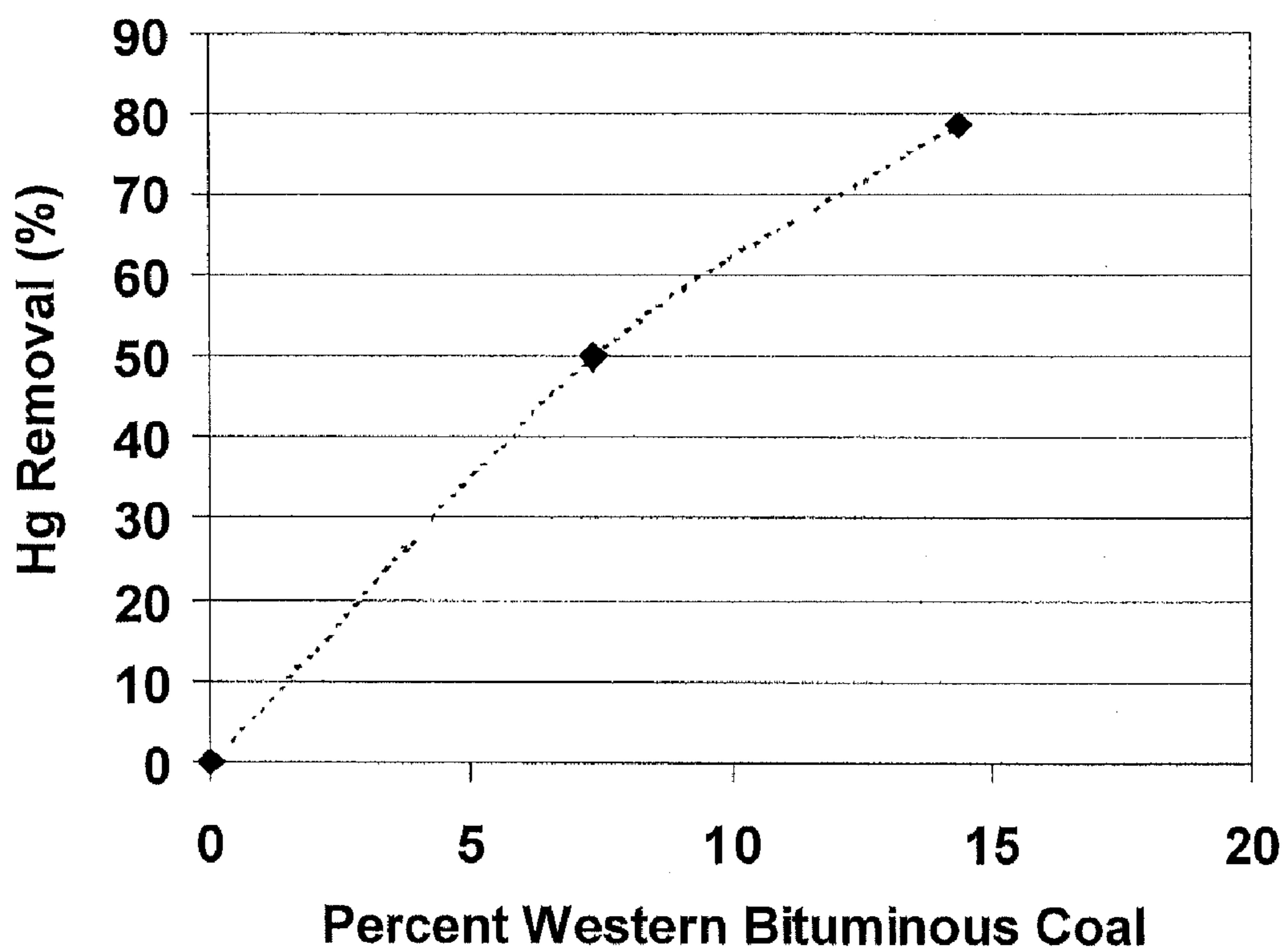
Figure 7. Results of Coal Blending Tests, Experiment #3
