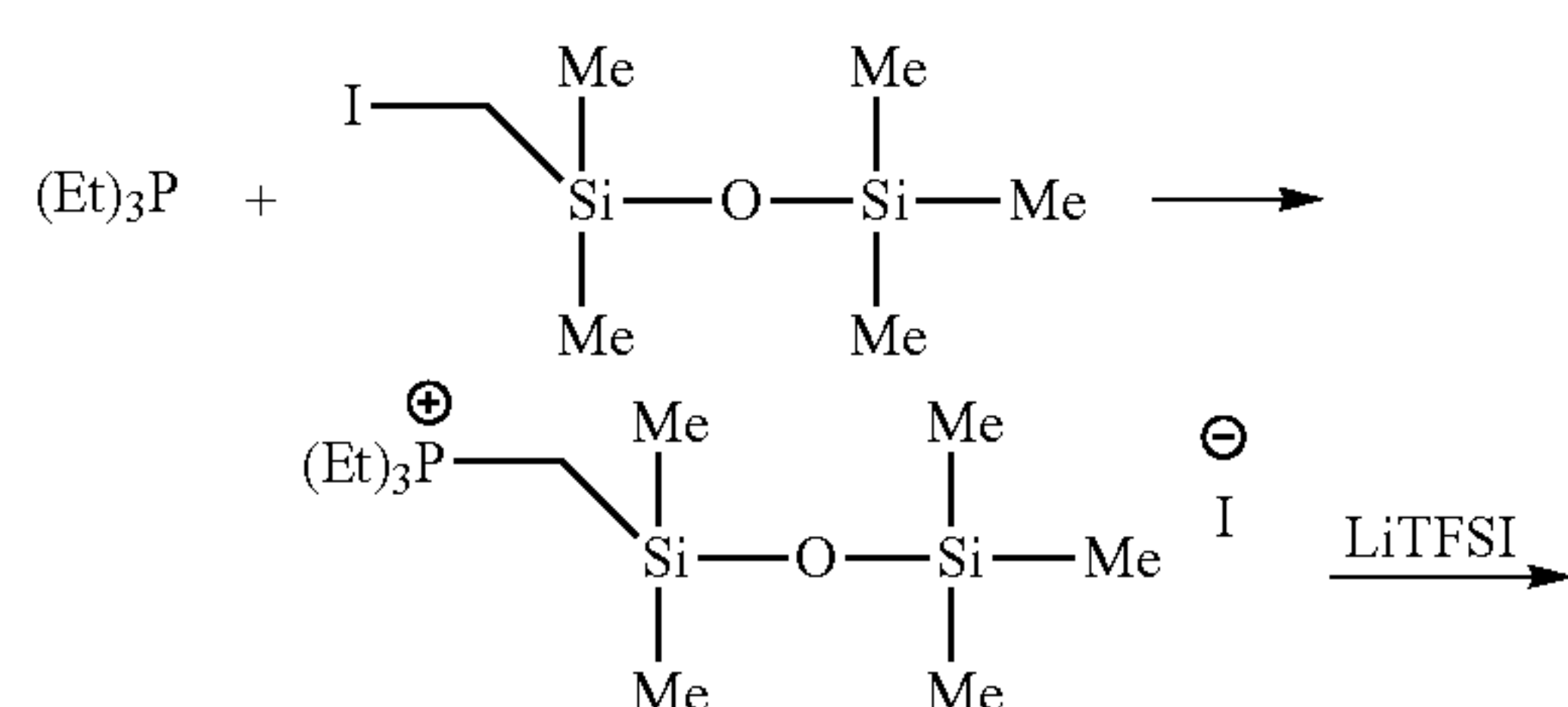
Scheme 1. Representative synthesis of functionalized ionic liquids IL1-I, IL1-TFSI, IL2-I, IL2-TFSI, IL3-Br and IL3-TFSI.
