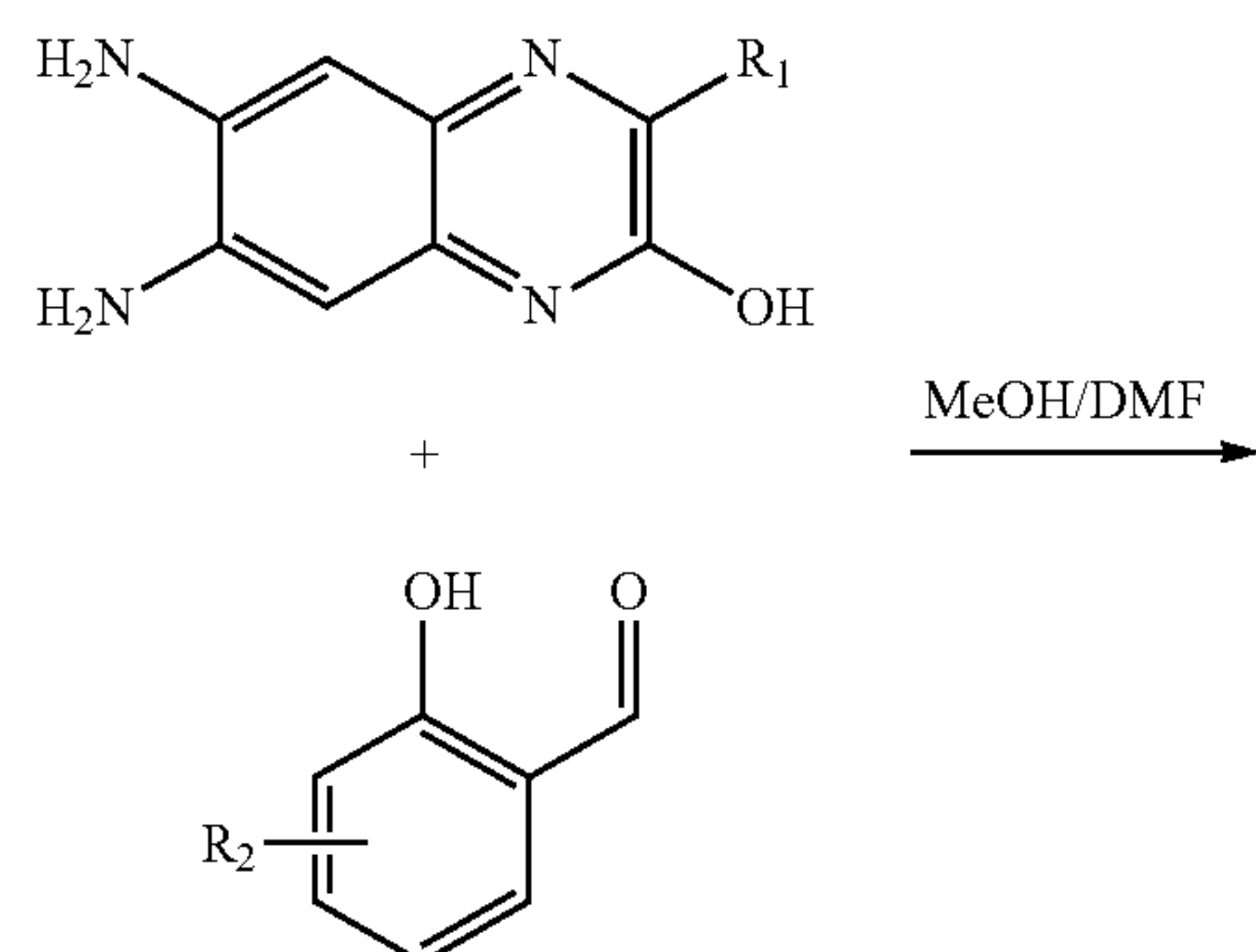
Scheme 4. Scheme depicting the synthesis of the 2-quinoxolinol salen ligands described within the text.
