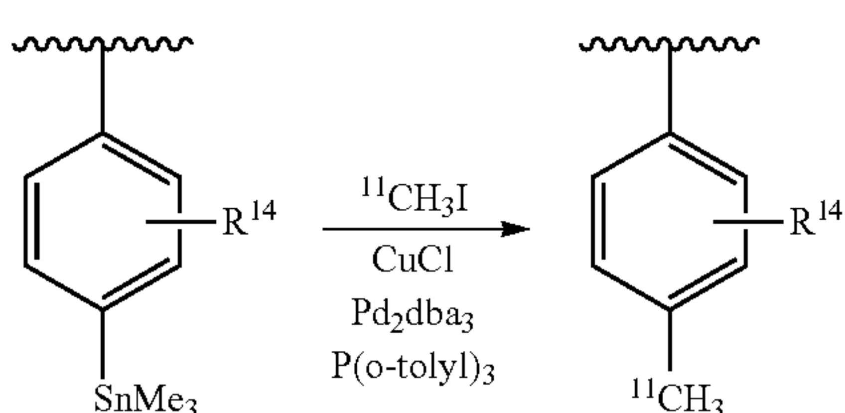
Scheme 14
