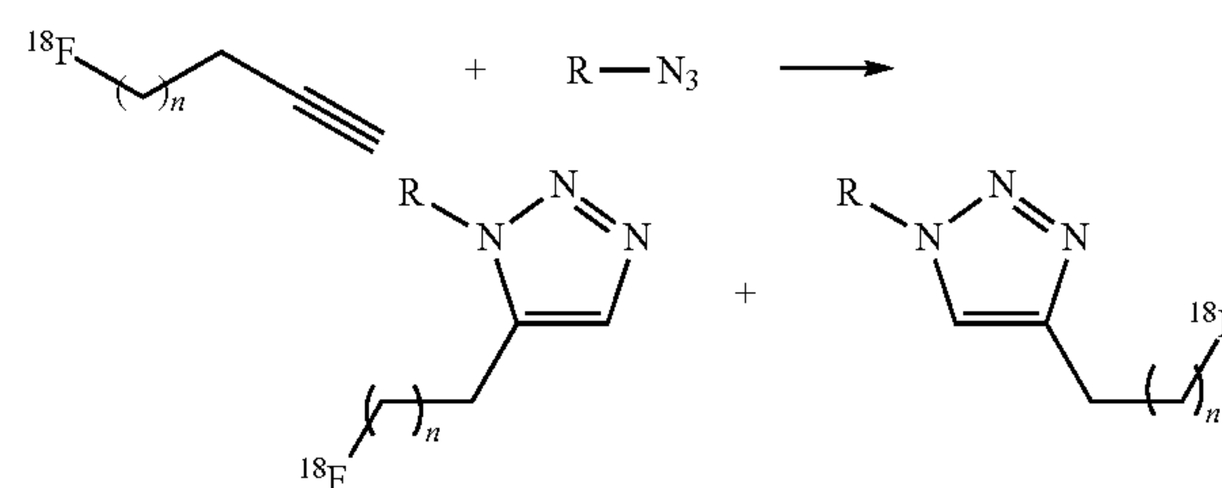
Scheme 17
