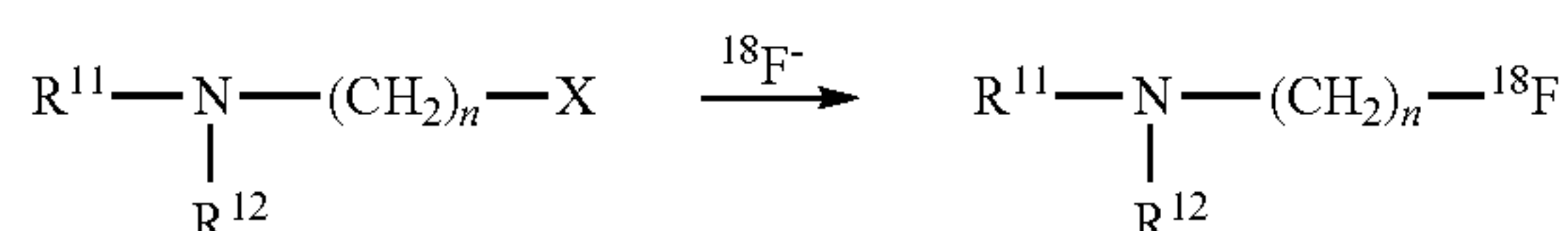
Scheme 12
