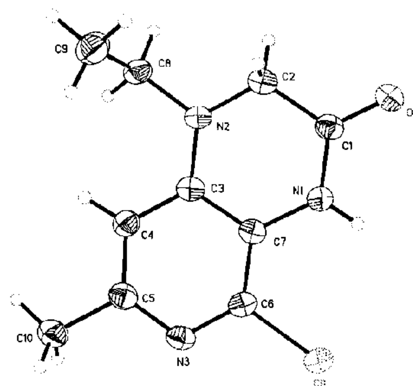
Figure 4. Thermal ellipsoid representation of the X-ray crystal structure of XXXIII .
