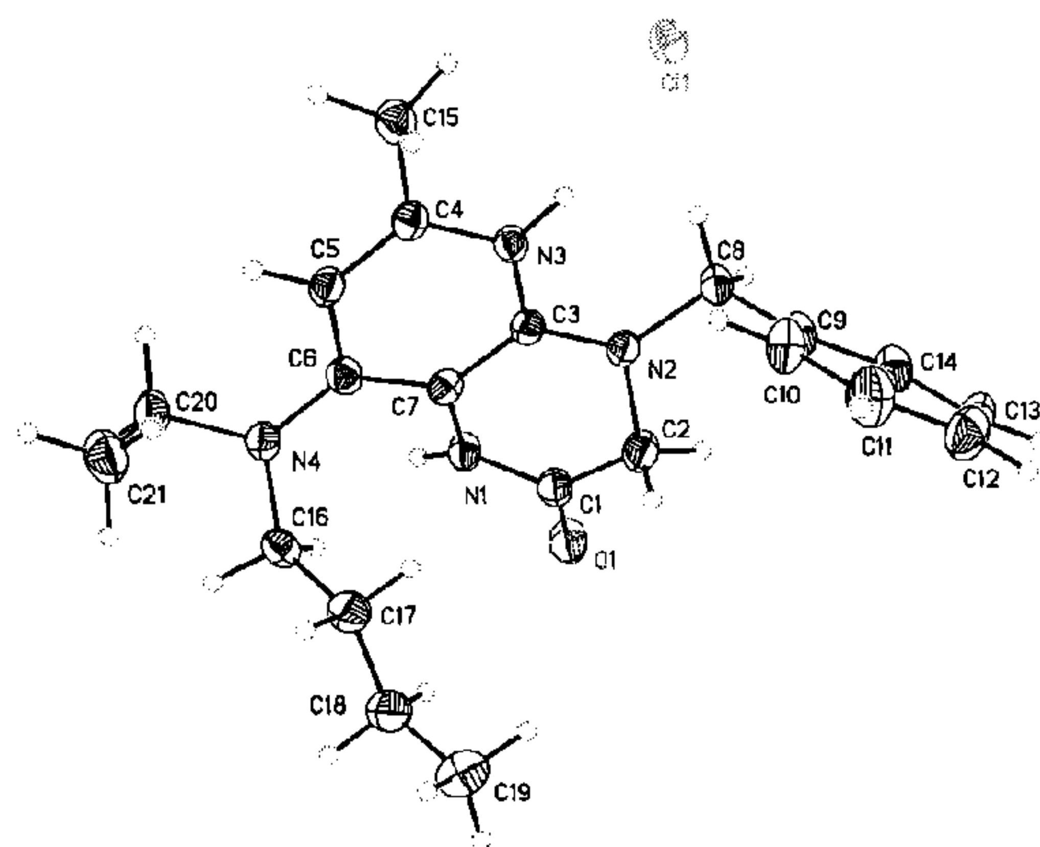
Figure 2. Thermal ellipsoid representation of the X-ray crystal structure of 8374•HCl .
