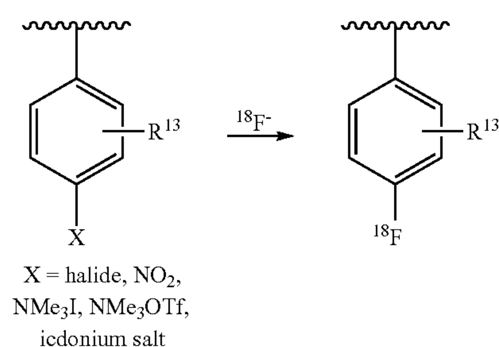
Scheme 13
