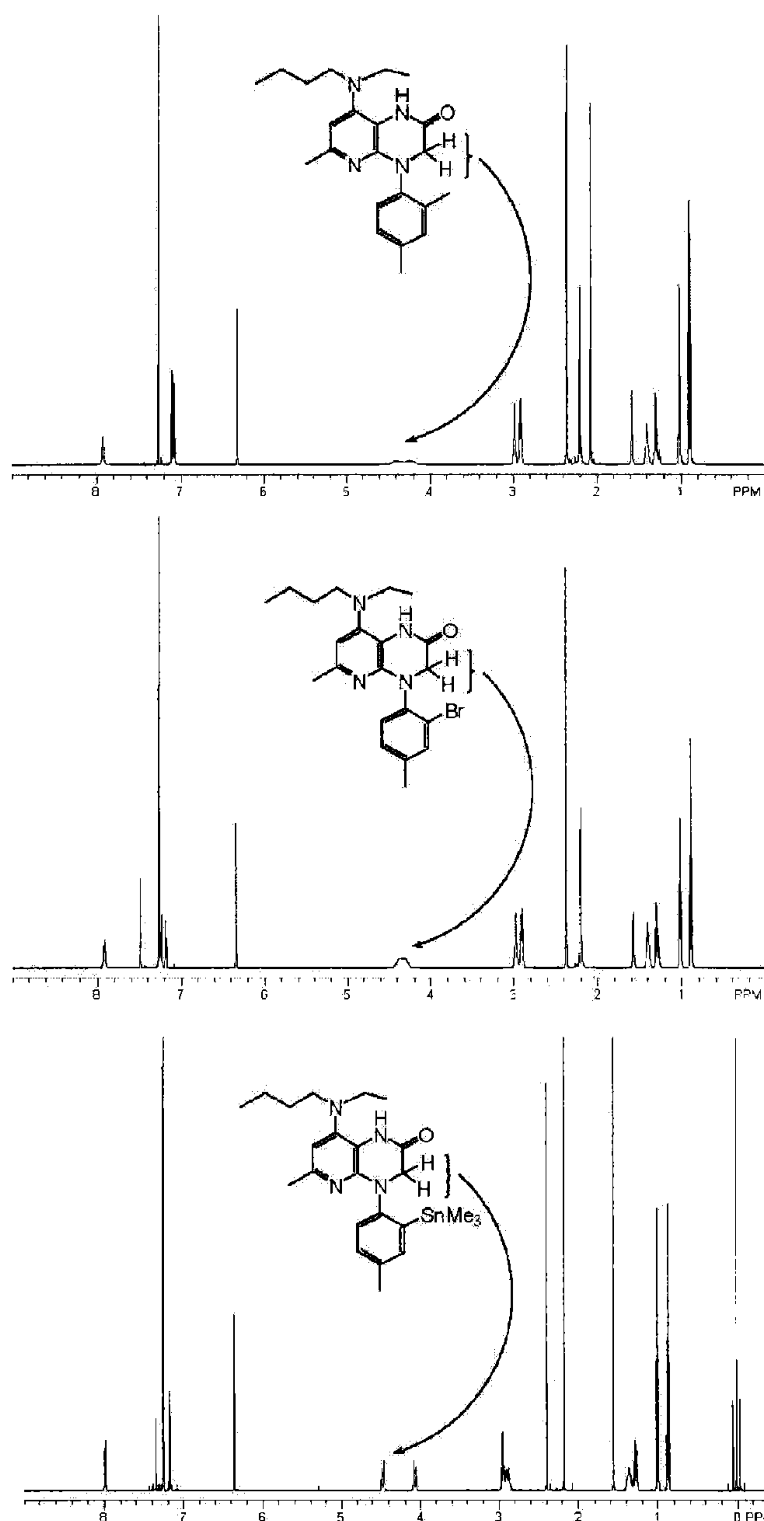
Figure 1. . 1 H NMR spectra (600 MHz, CDCl 3 ) of compounds 191 , 185 , and 190 demonstrating the existence of atropisomerism due to restricted rotation of the aniline ring.
