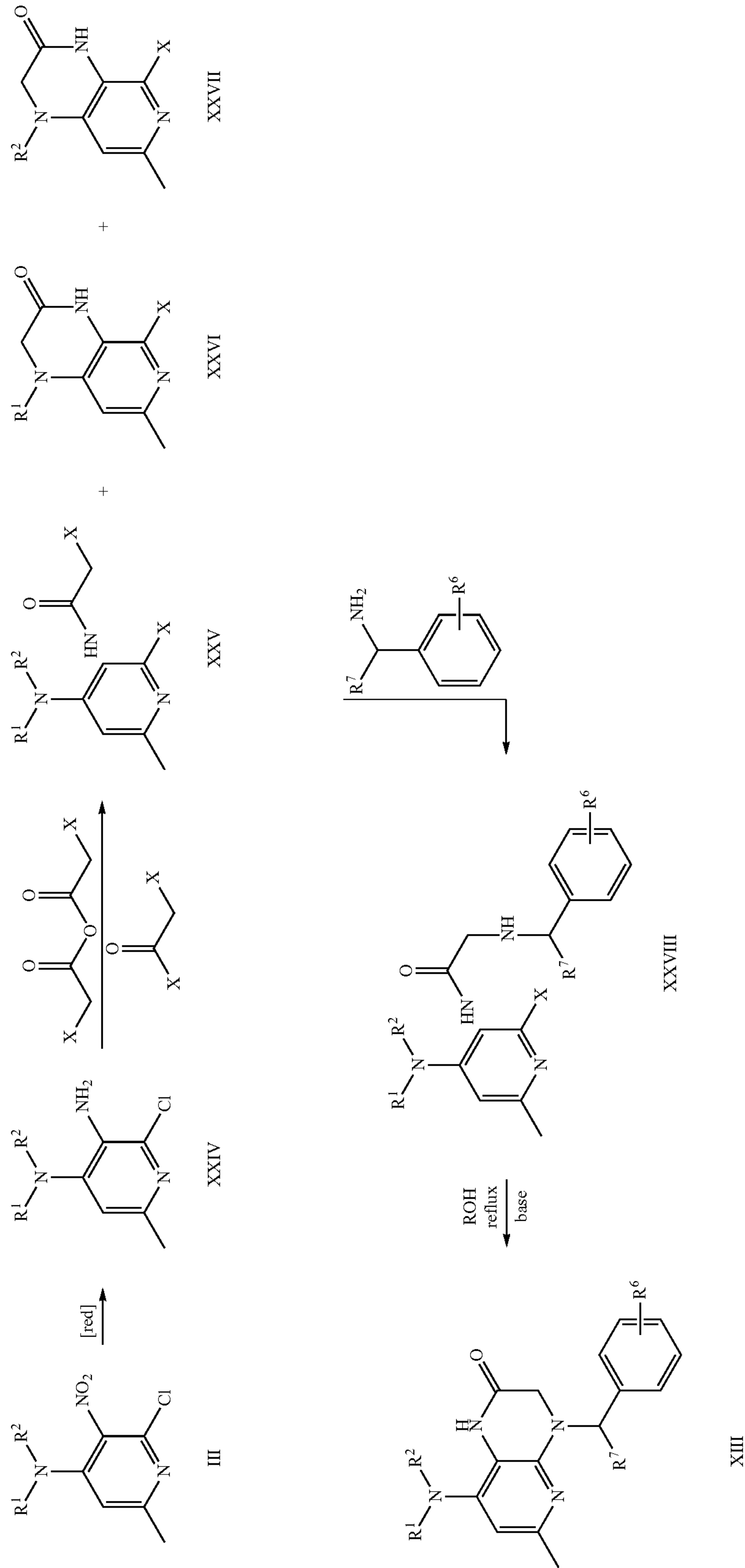
Scheme 6
