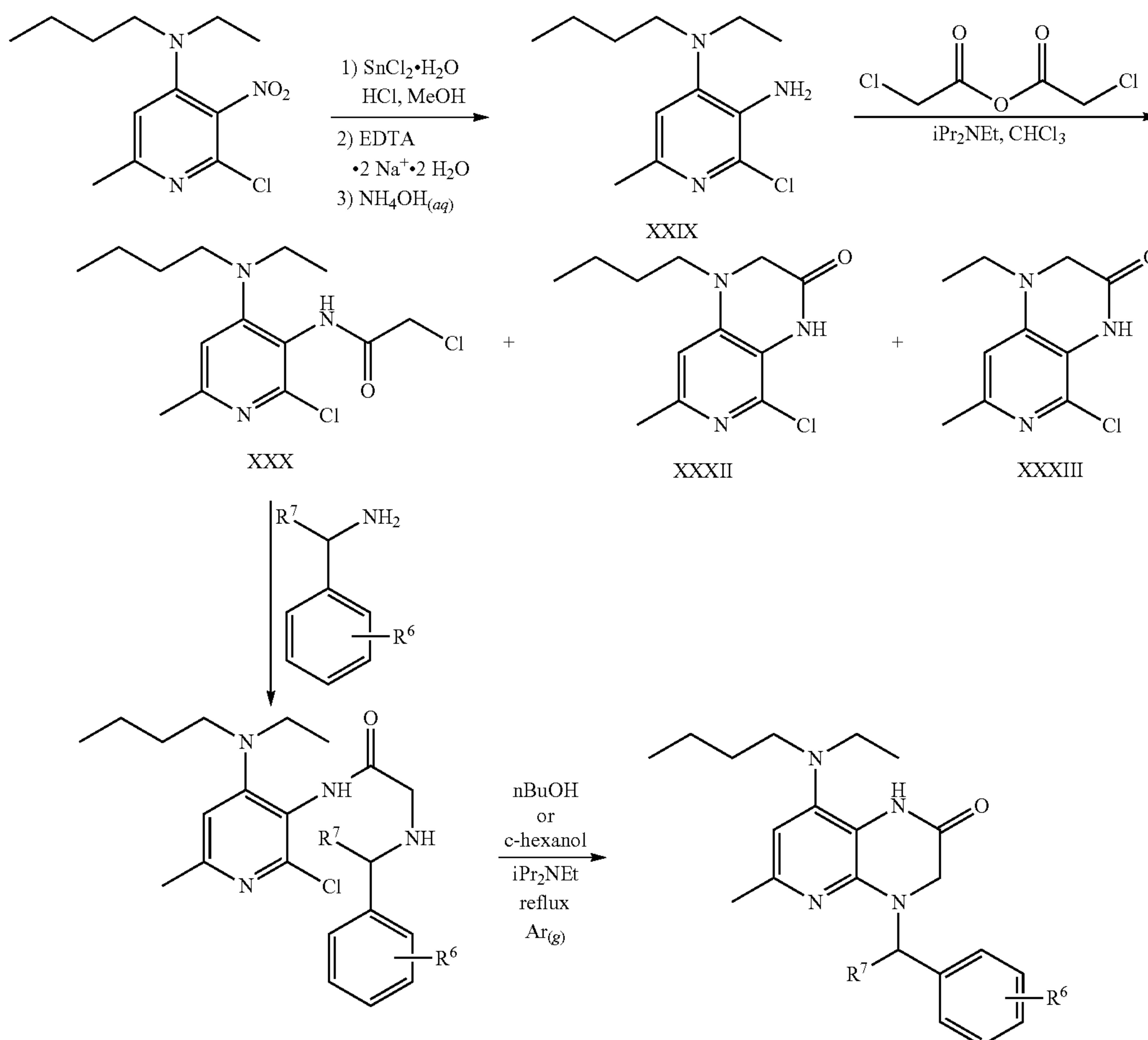
Scheme 23
