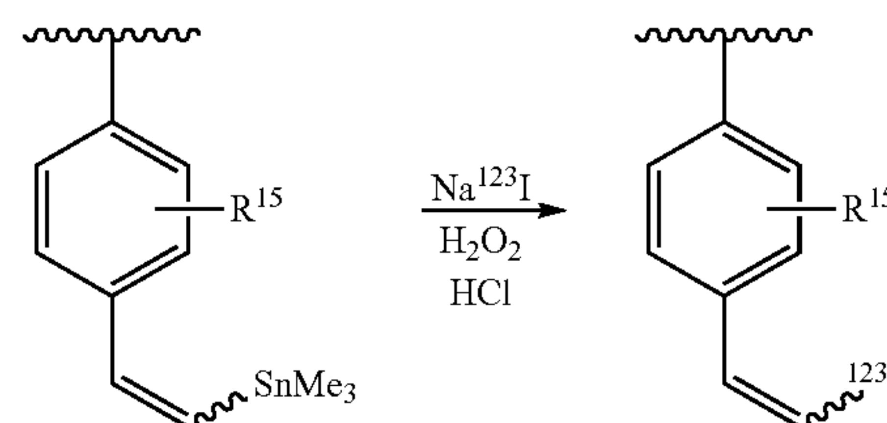
Scheme 15
