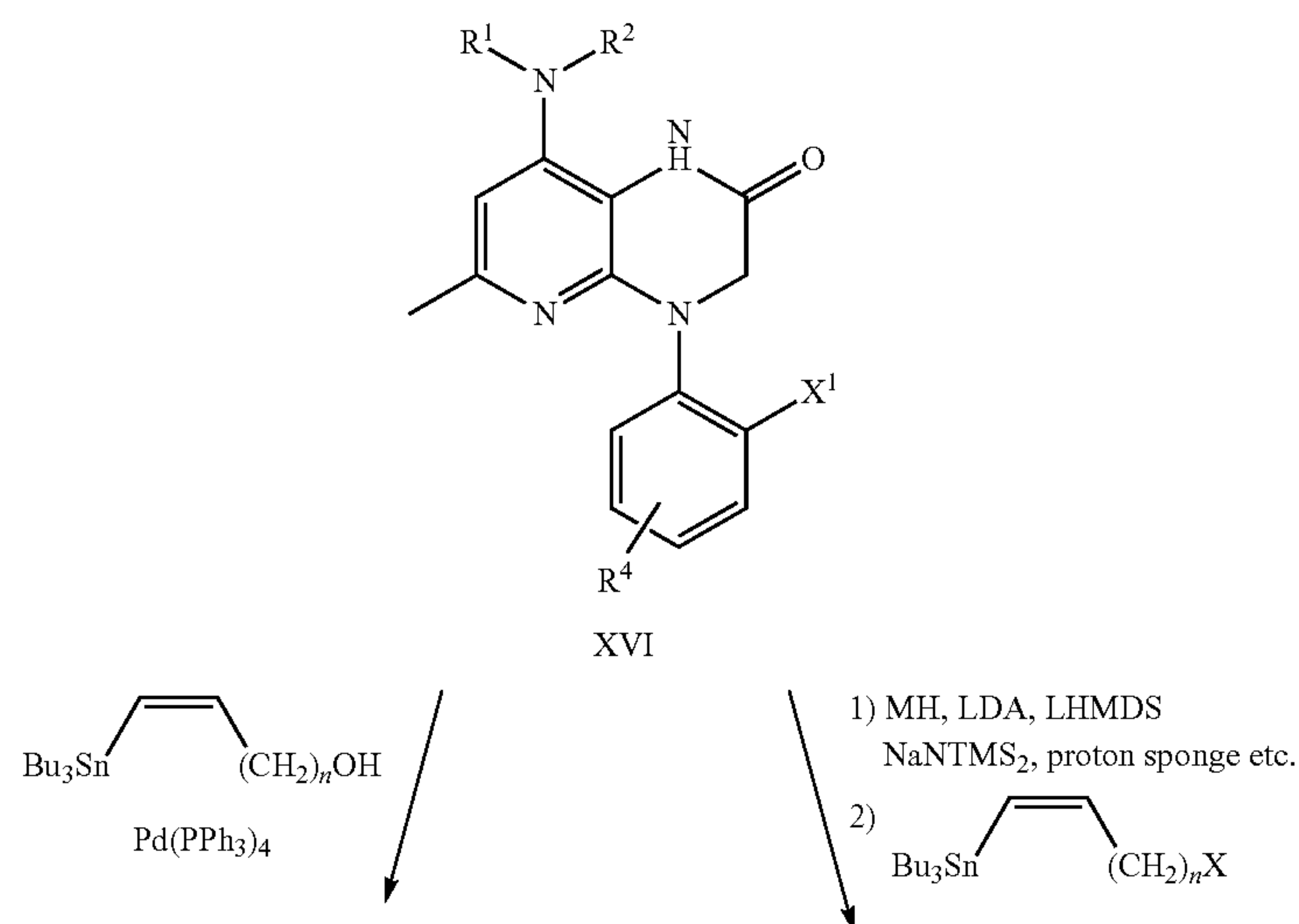
Scheme 4
