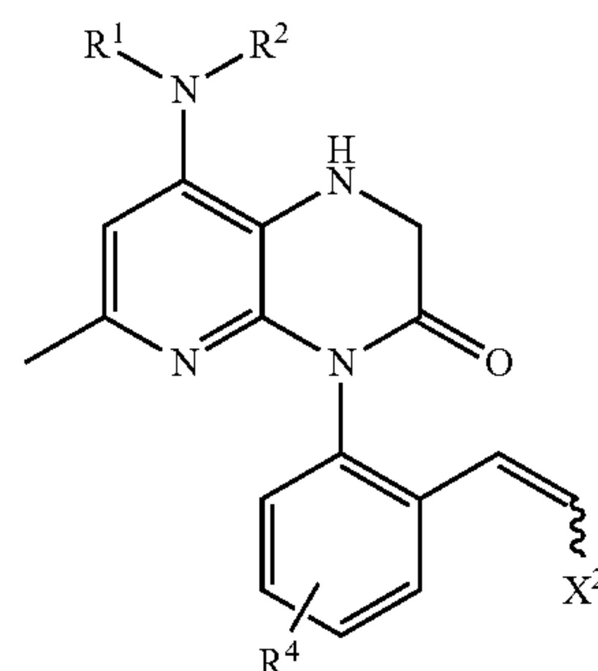
Substituent list for compounds of general structure XI.
