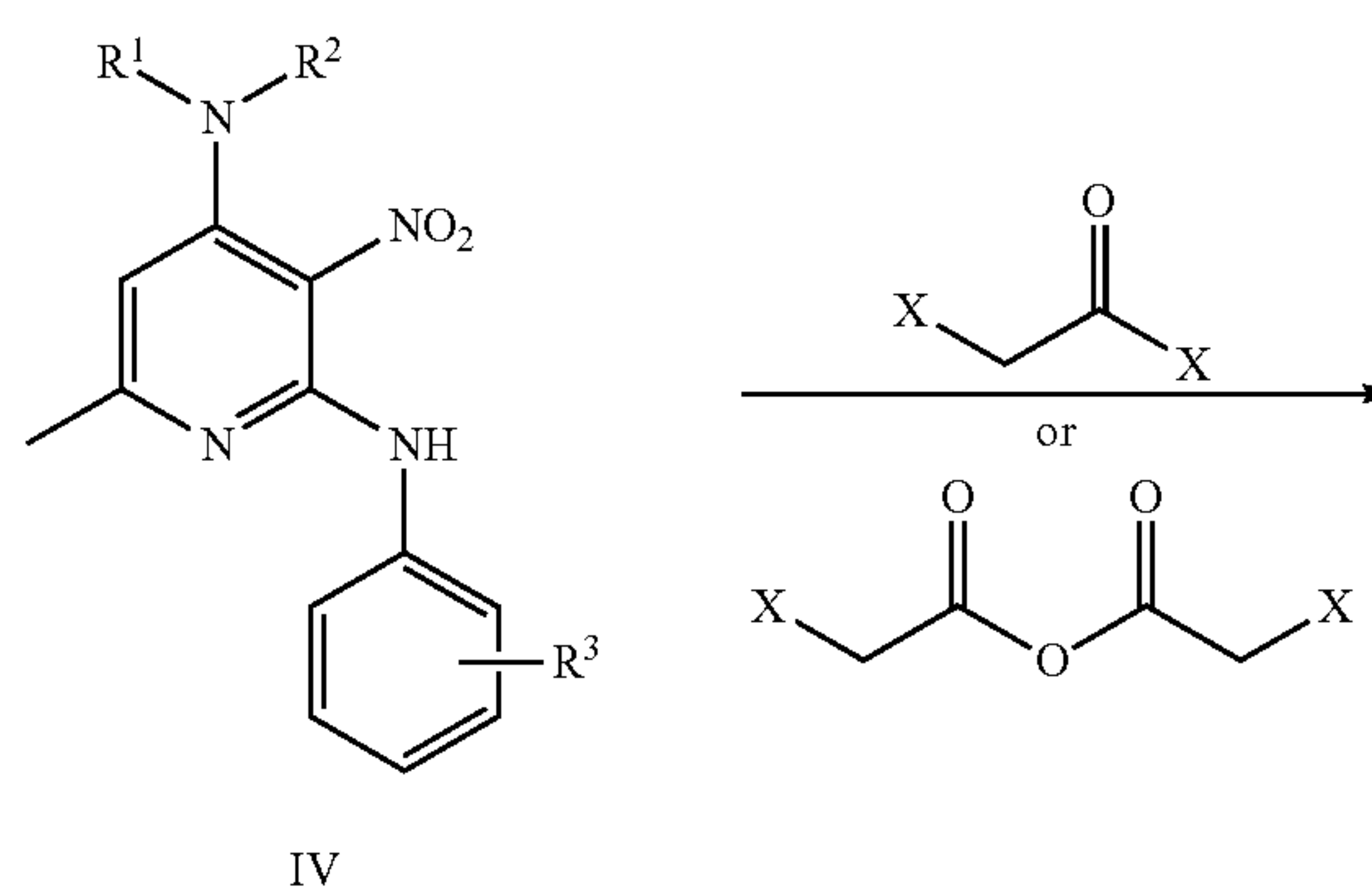
Scheme 5
