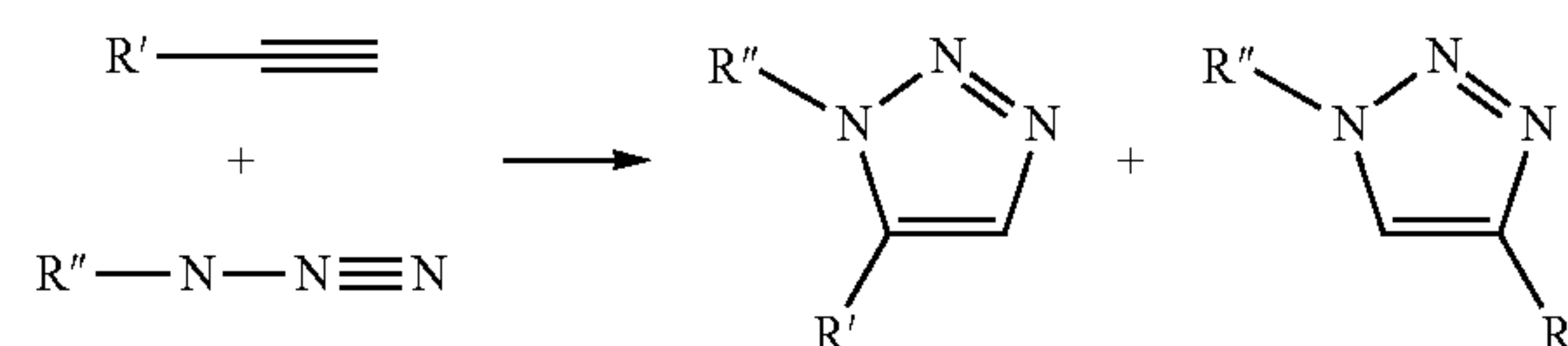
Scheme 16
