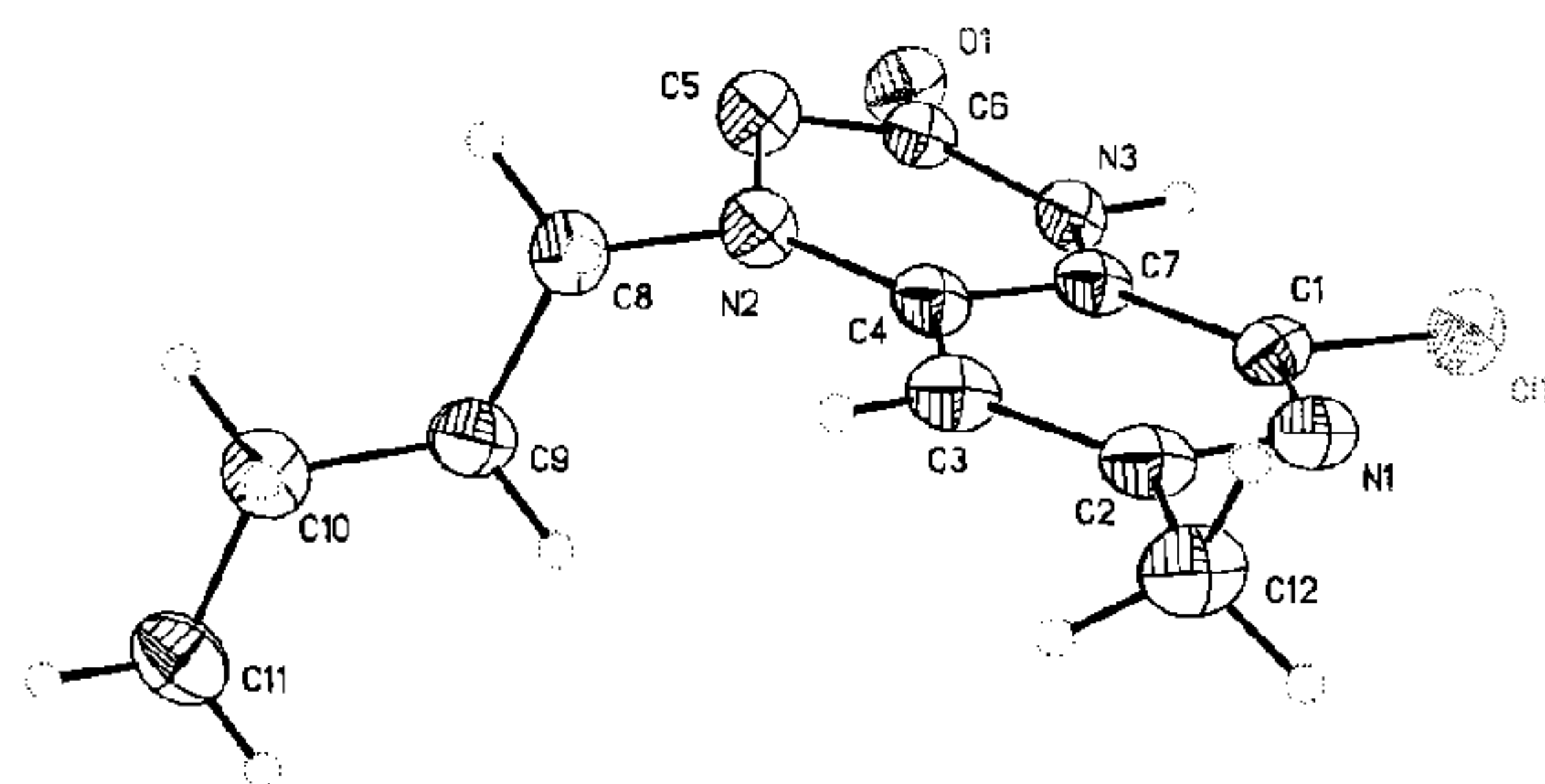
Figure 3. Thermal ellipsoid representation of the X-ray crystal structure of XXXII .
