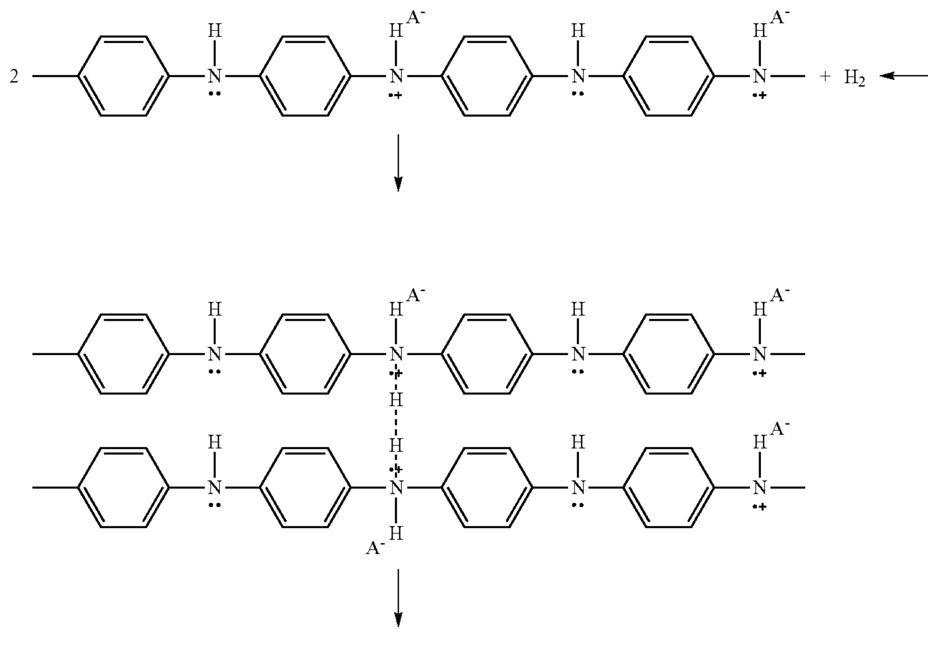
Scheme 1 Possible mechanism for hydrogen interaction with doped polyaniline where A^- represents the counteranion.
