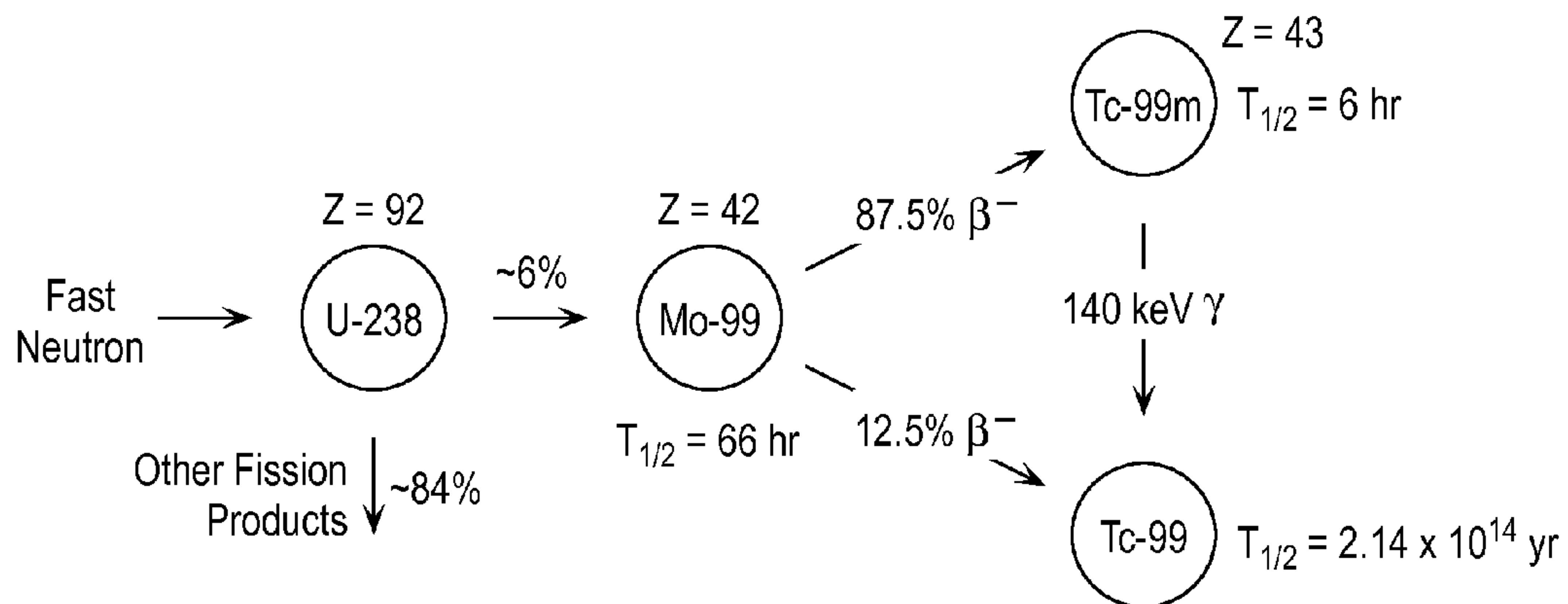
FIG. 2 (Prior Art)
