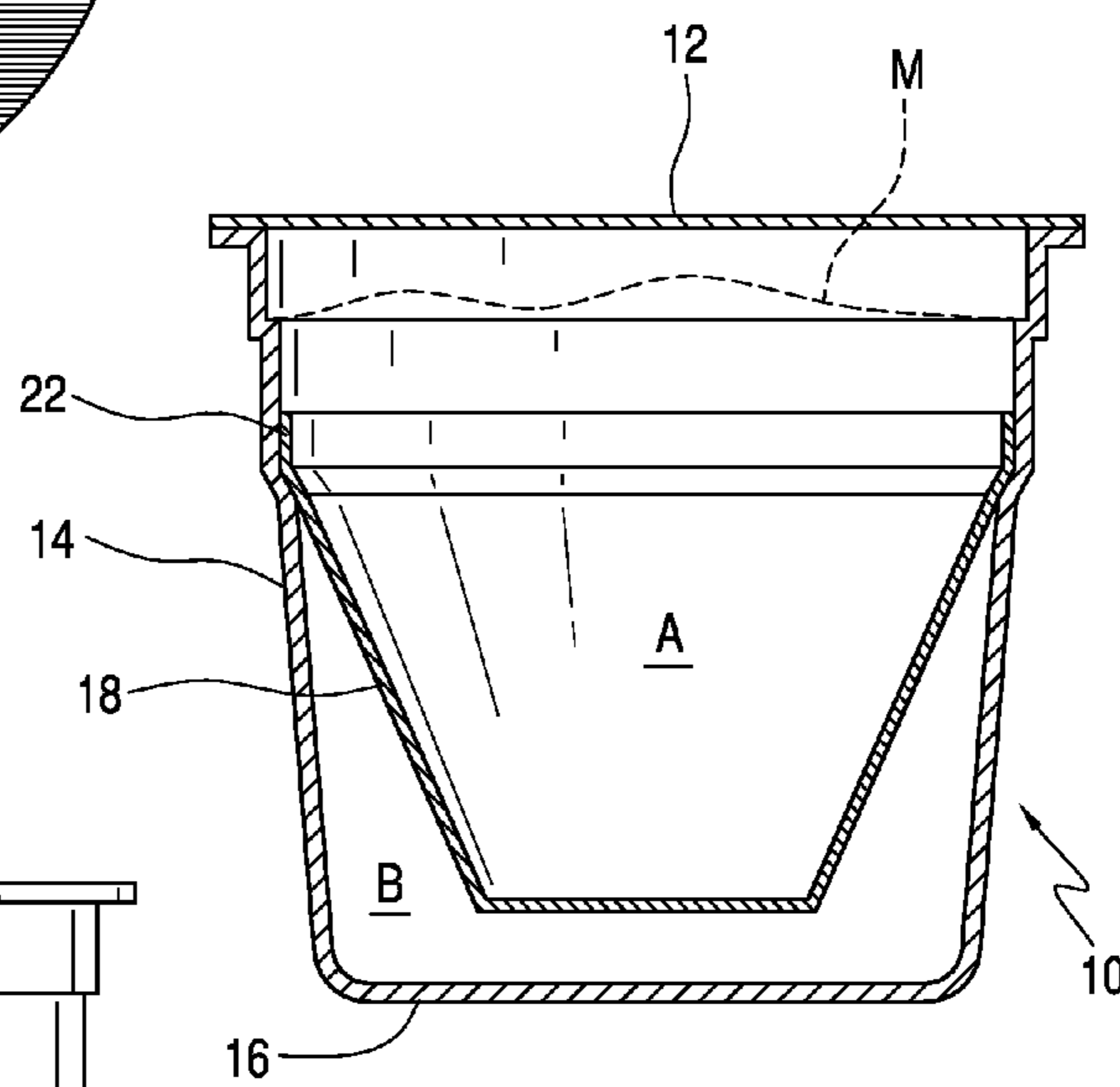
FIG. 3 PRIOR ART
