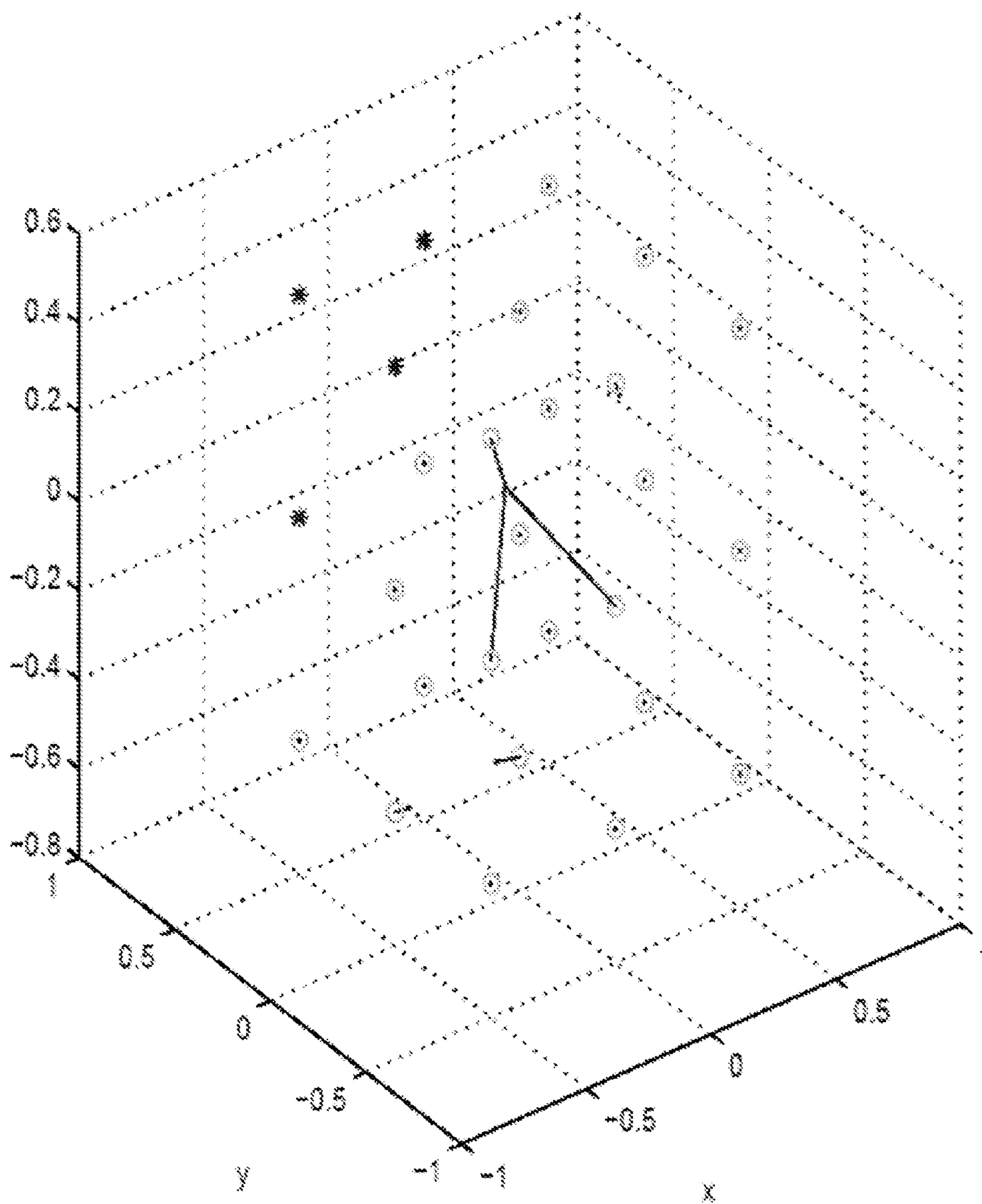
Estimated Sensor Locations in 3D without Geometric Routine
