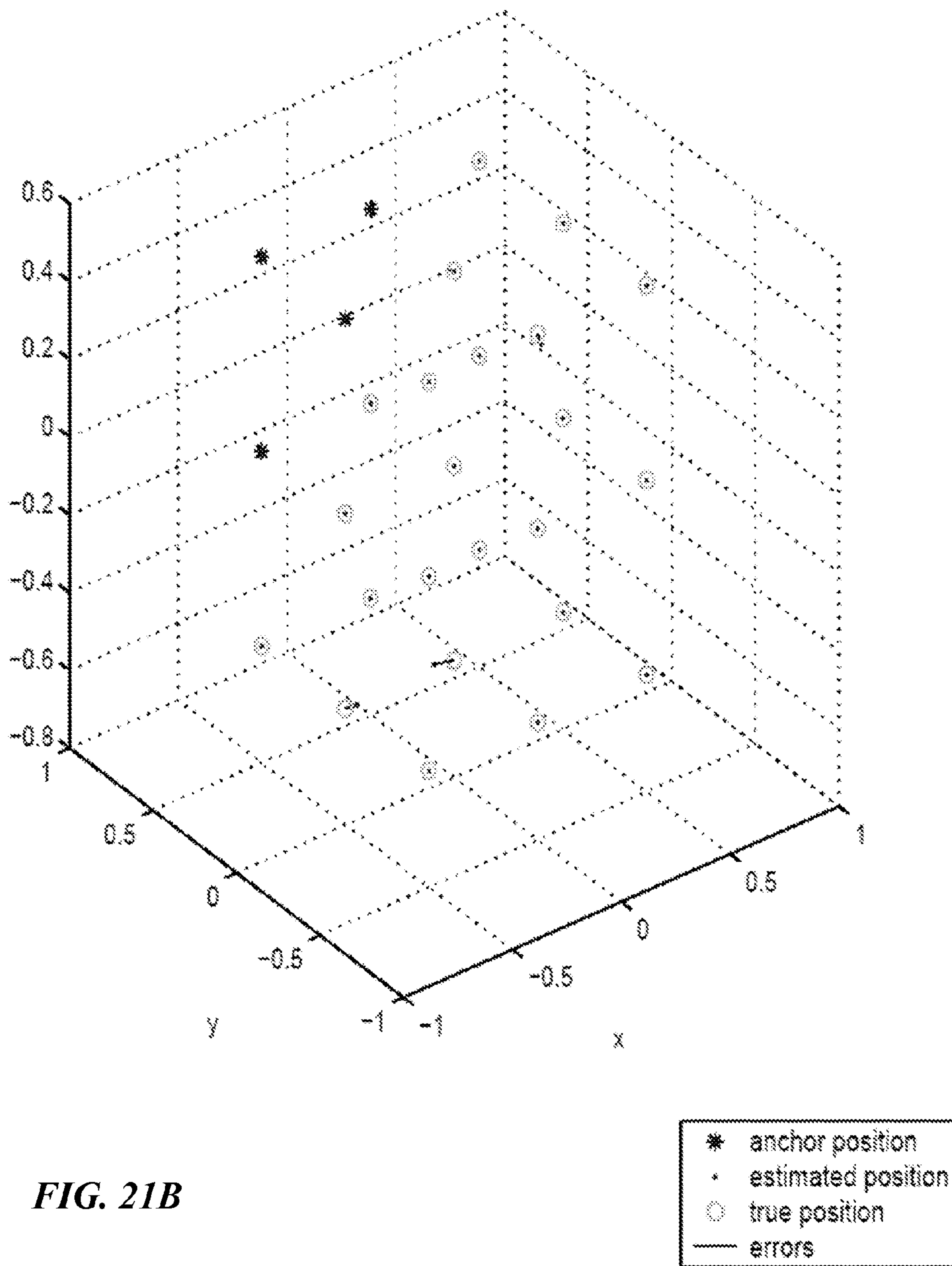
Estimated Sensor Locations in 3D with Geometric Routine
