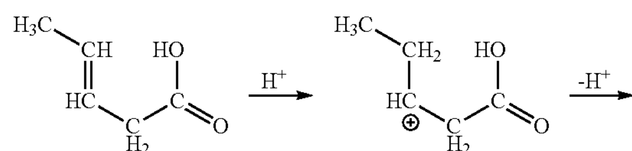
Scheme 2: Conversion of 3-pentenoic acid to 1-butene and \text{CO}_2
