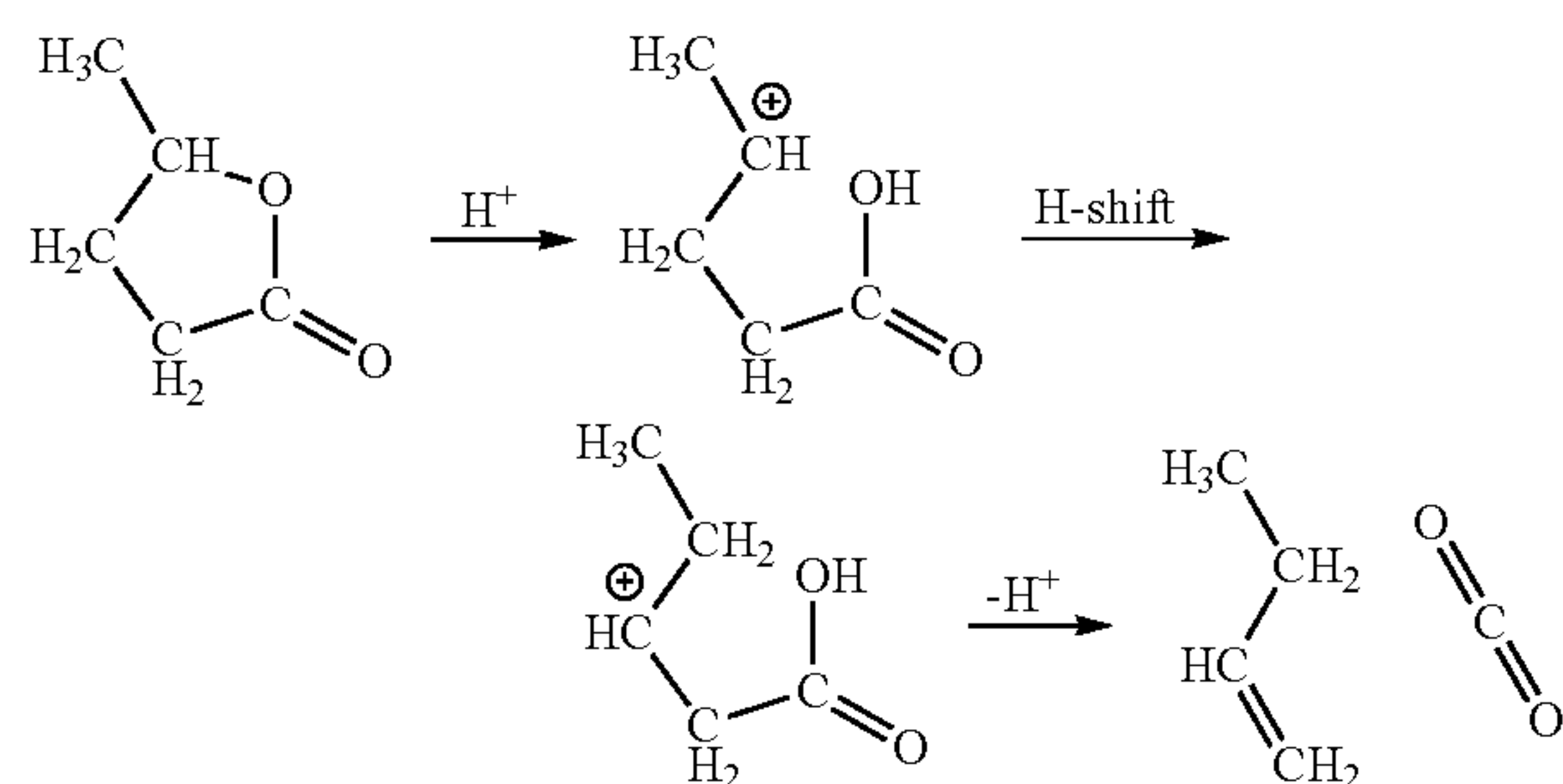
Scheme 1: Conversion of GVL to 1-butene and \text{CO}_2
