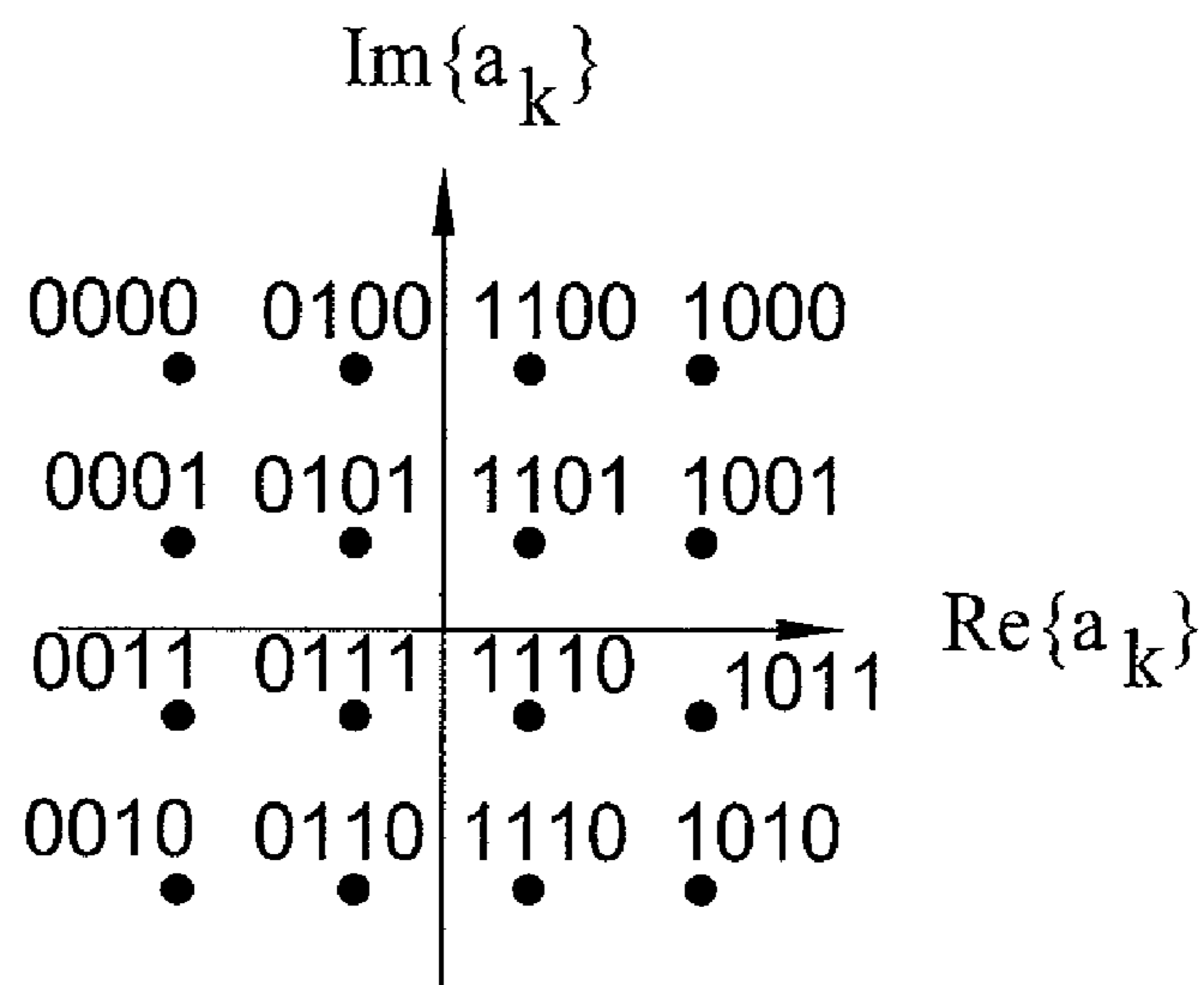
16-PSK 4 bits/symbol
