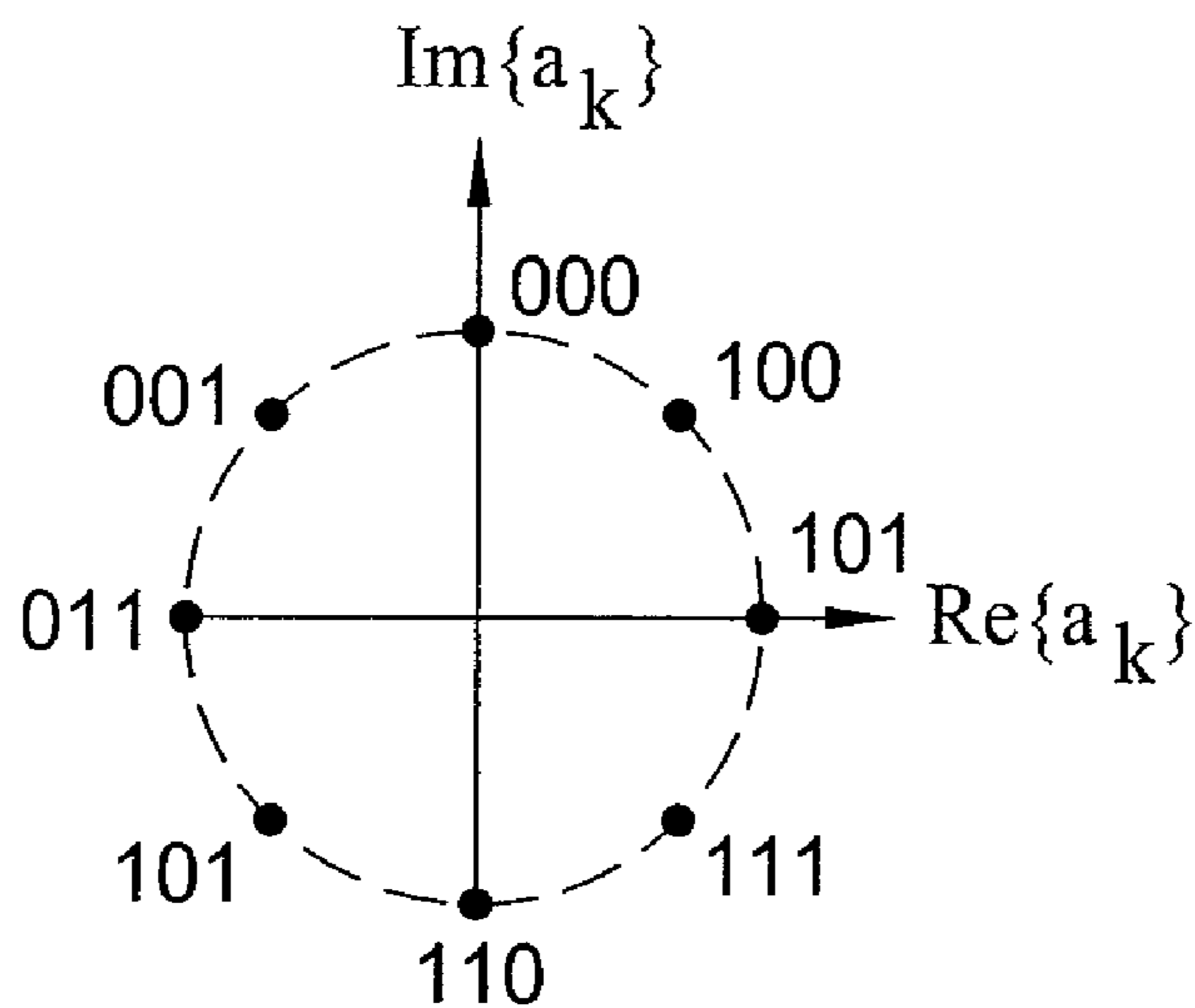
8-PSK 3 bits/symbol
