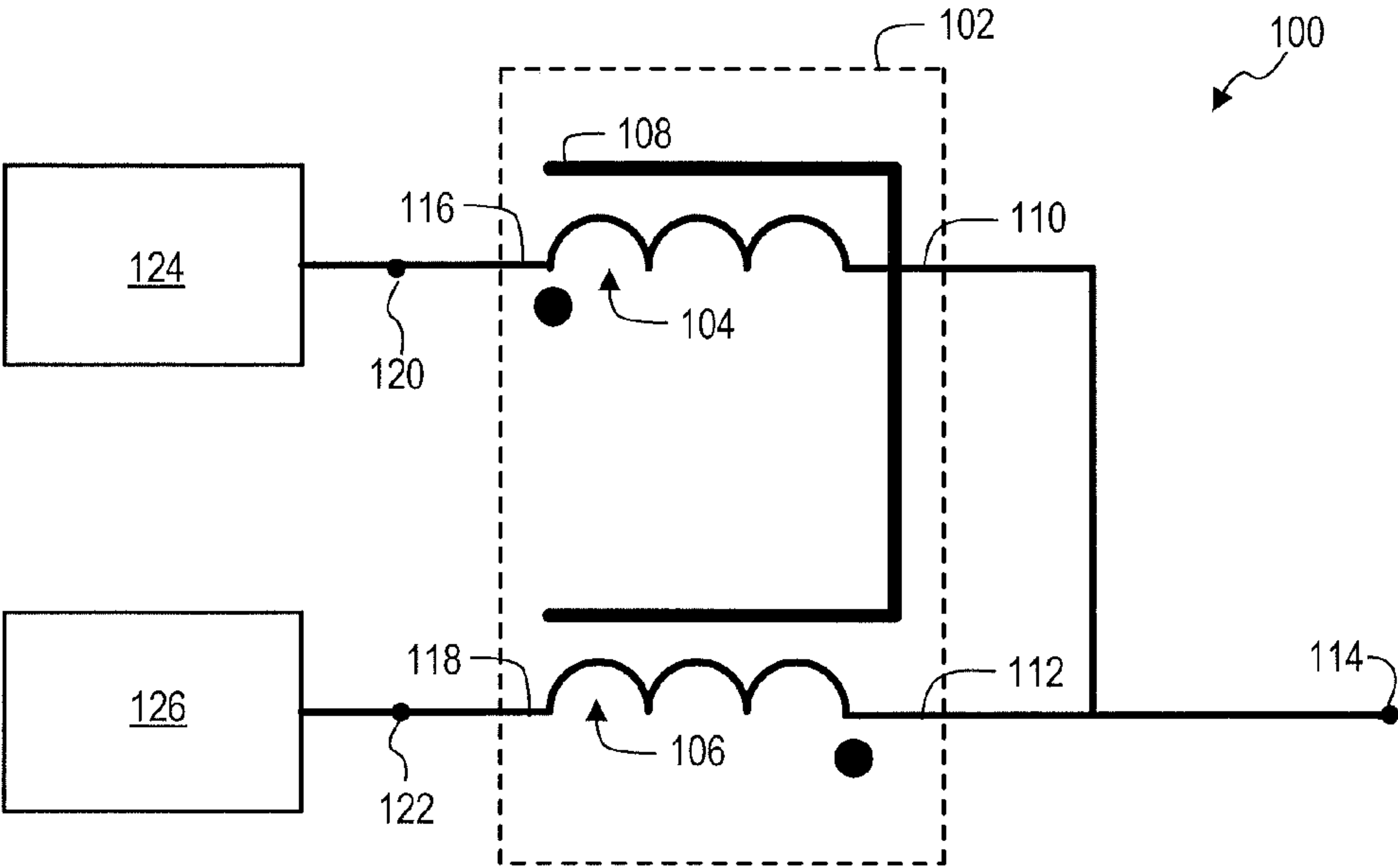
FIG. 1 (PRIOR ART)
