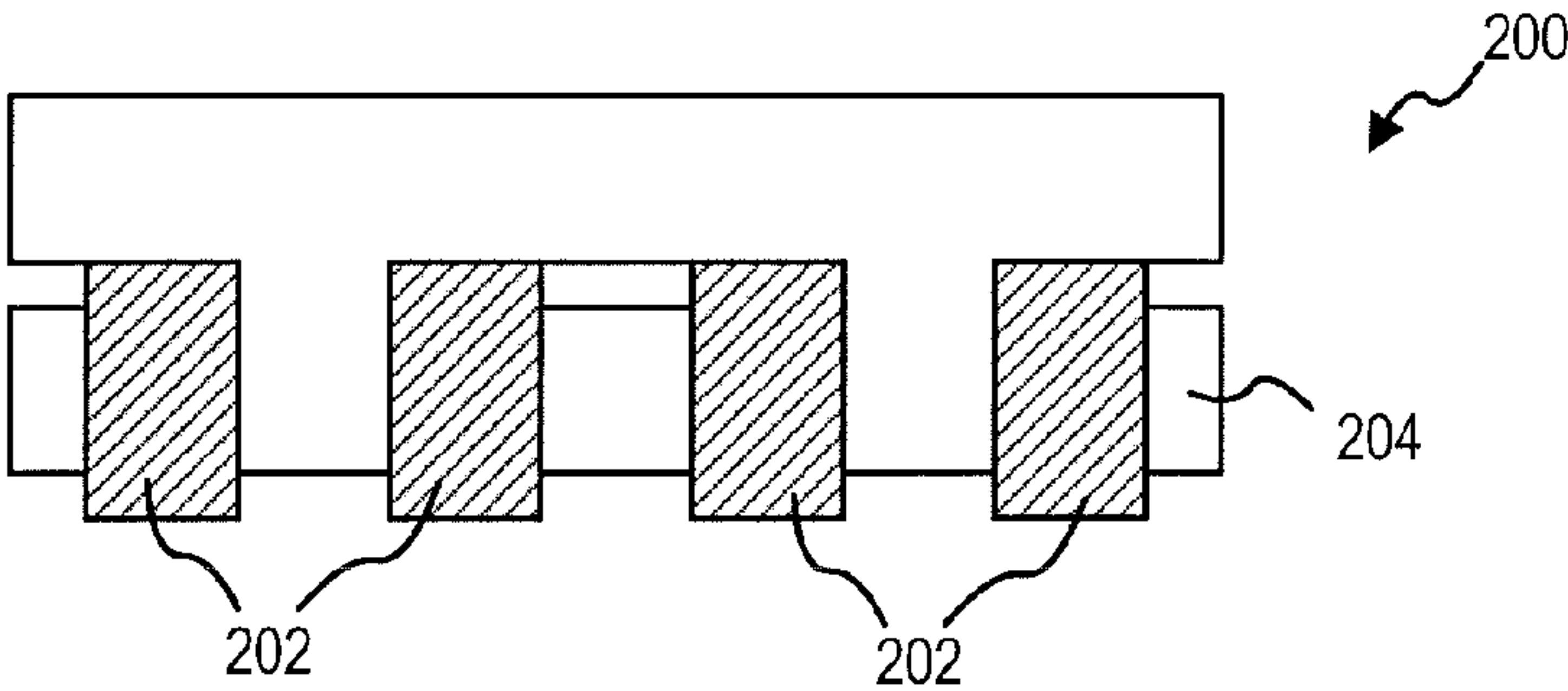
FIG. 2 (PRIOR ART)
