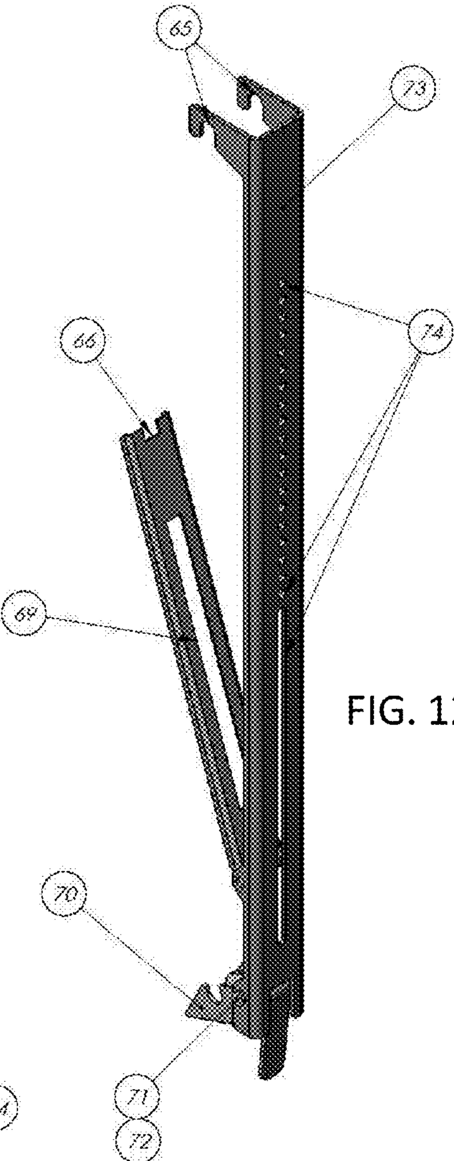
FIGURE 12 - LCD SUPPORT
