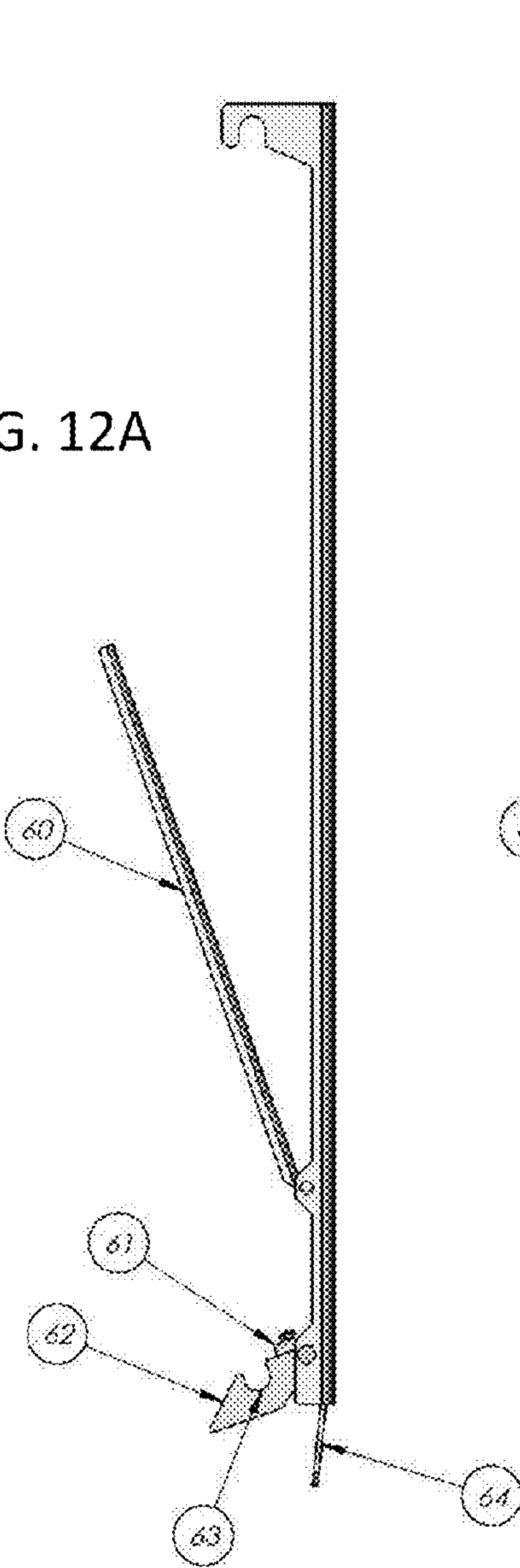
FIGURE 12 - LCD SUPPORT
