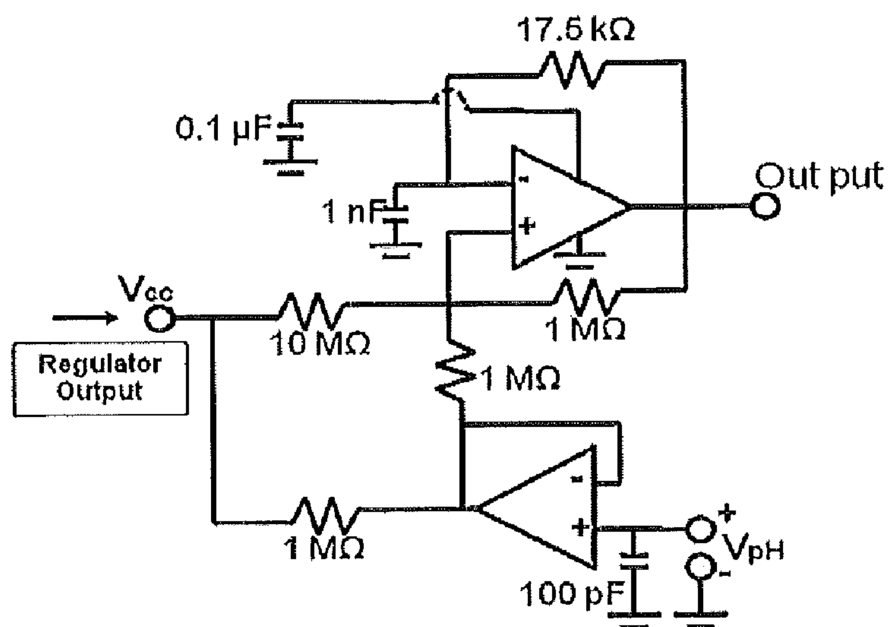
Figure 20 The relaxation oscillator design in the transponder.
