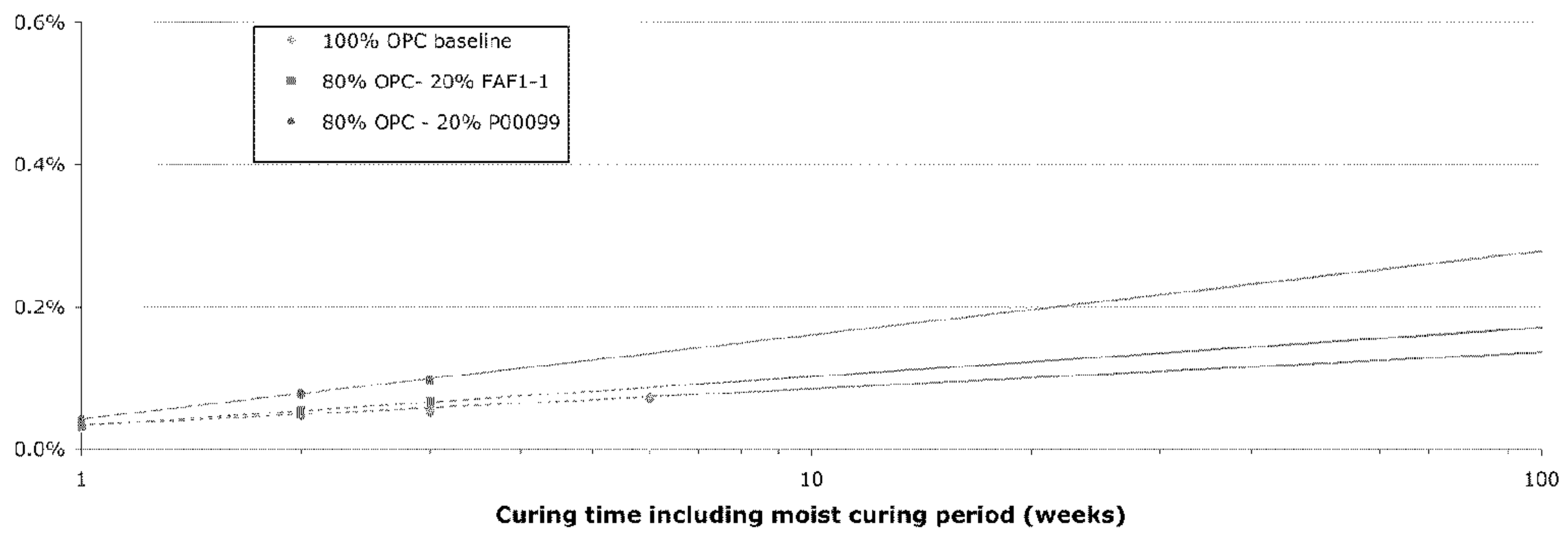
ASTM C596 - Drying shrinkage
