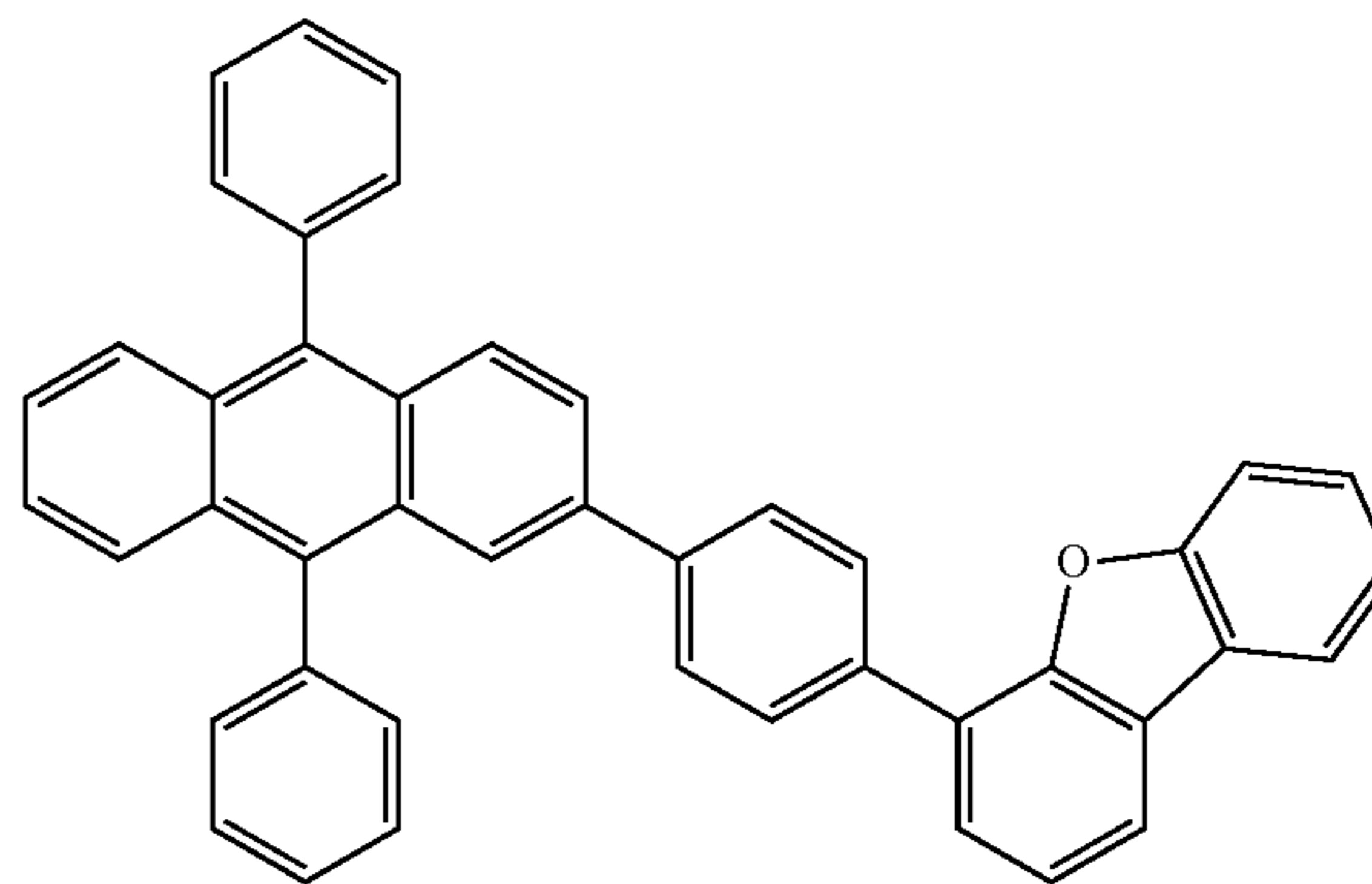
(2PDBFPA-II)
