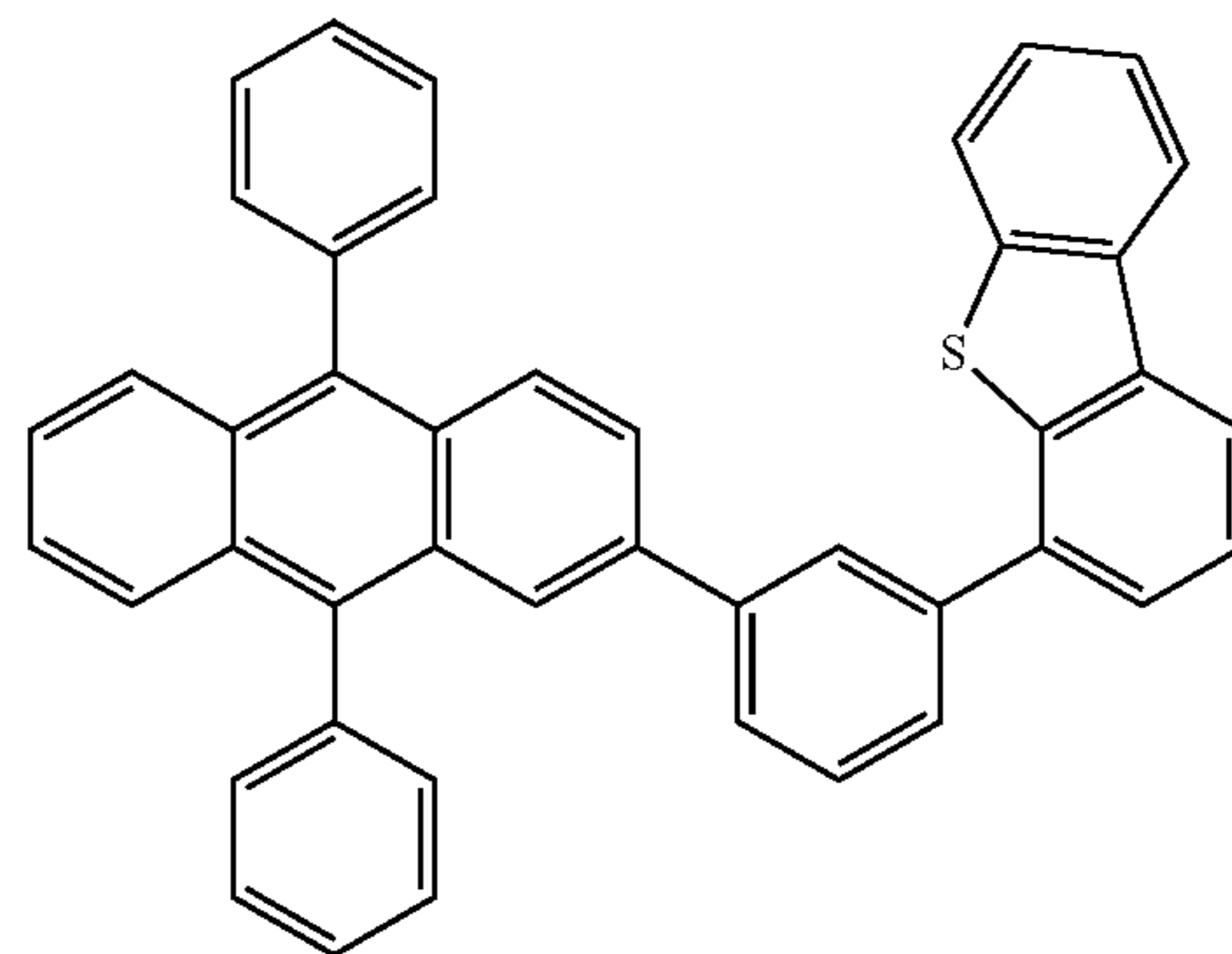
(2mPDBTPA-II)
