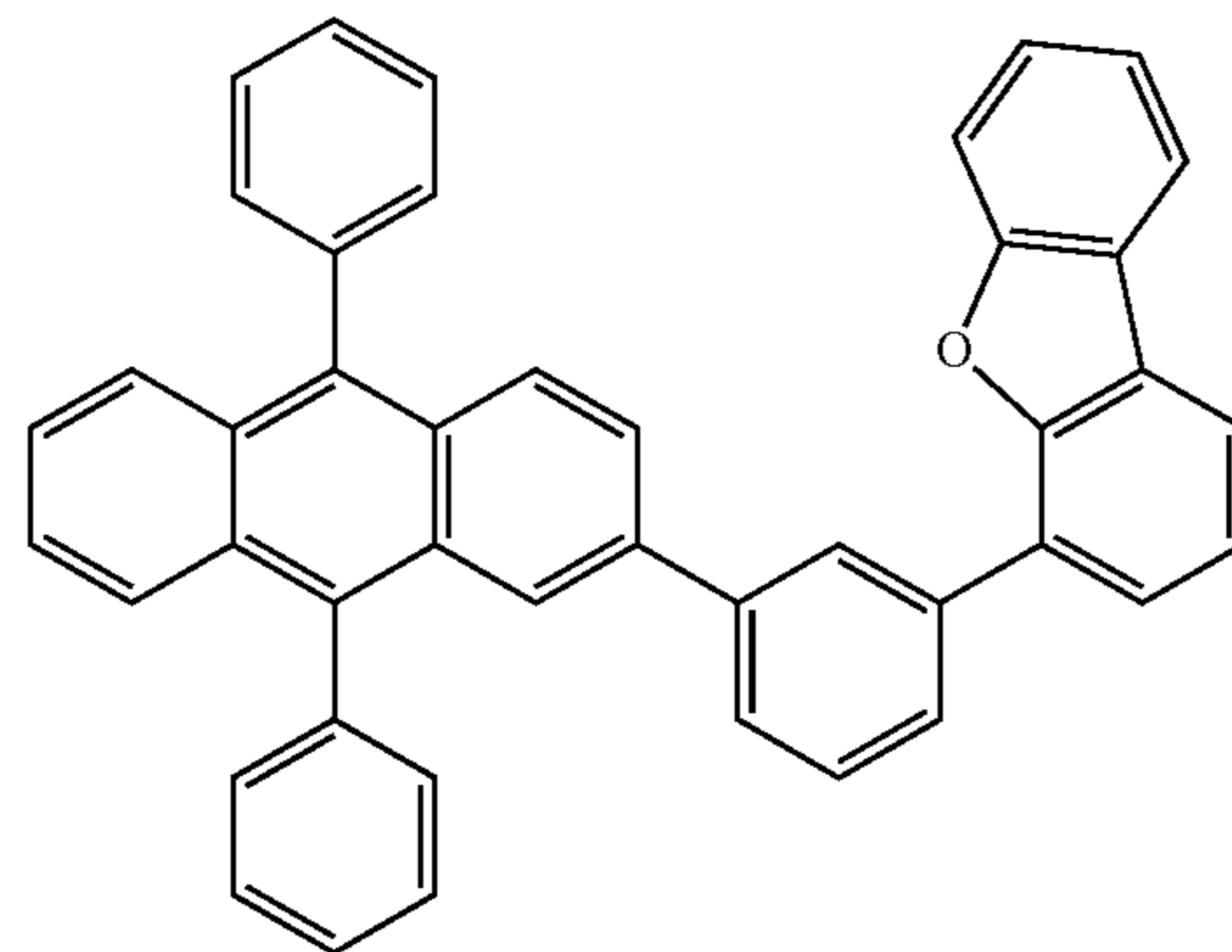
(2mPDBFPA-II)
