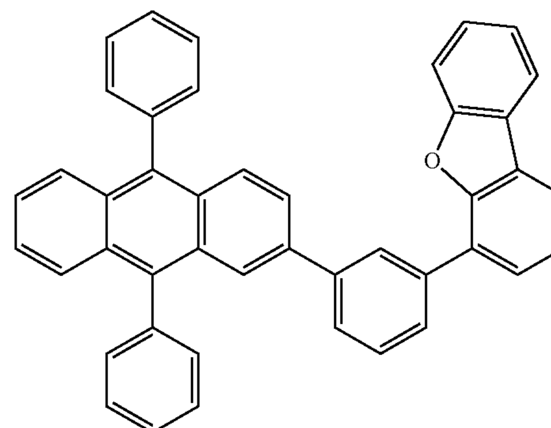
2mPDBFPA-II
