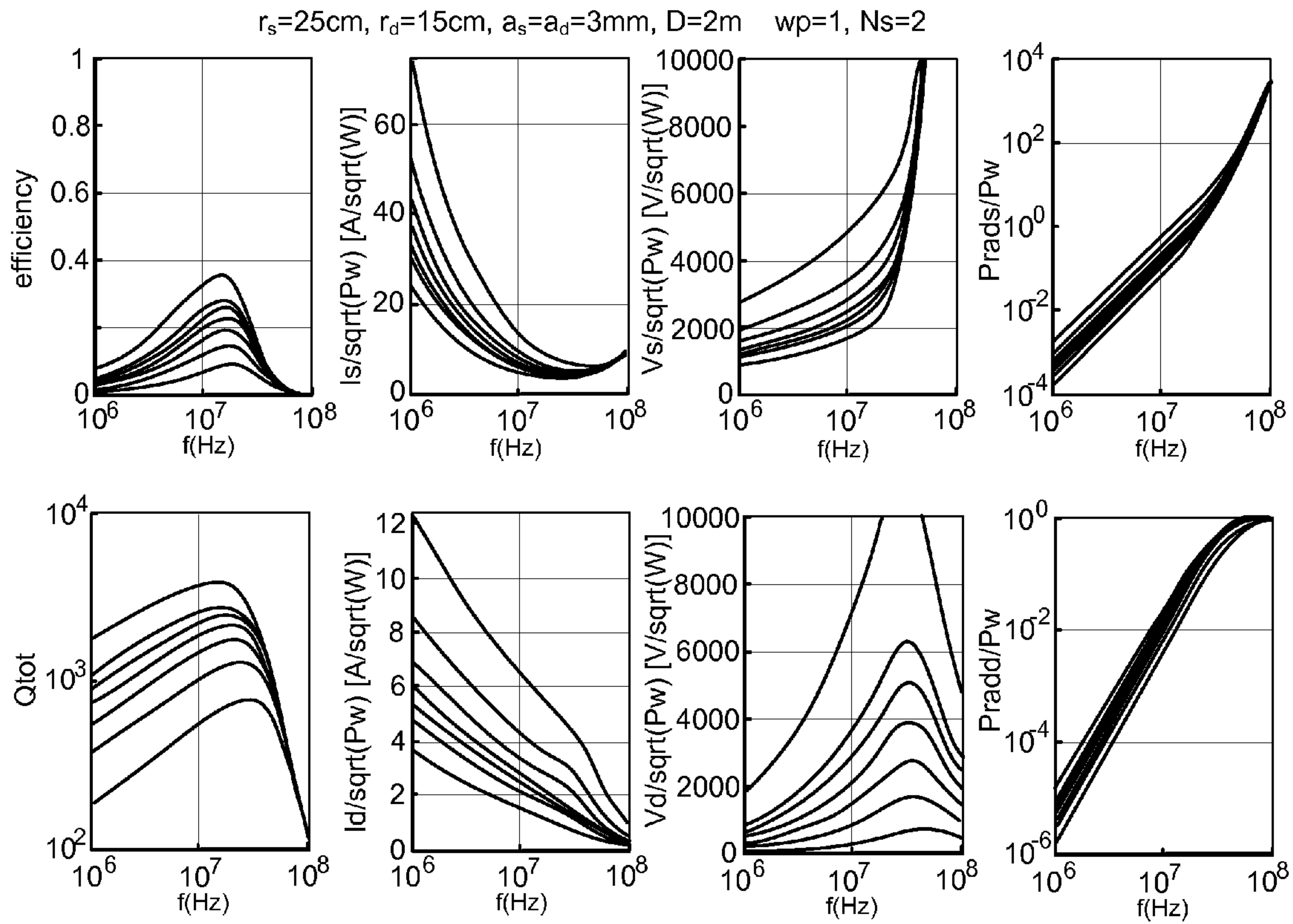
Efficiency, total (loaded) device Q, and source and device currents, voltages and radiated powers, normalized to 1Watt of output working power, as functions of frequency for a particular choice of source and device loop dimensions, w_p and N_s and different choices of N_d=1,2,3,4,5,6,10 (red, green, blue, magenta, yellow, cyan, black respectively)
