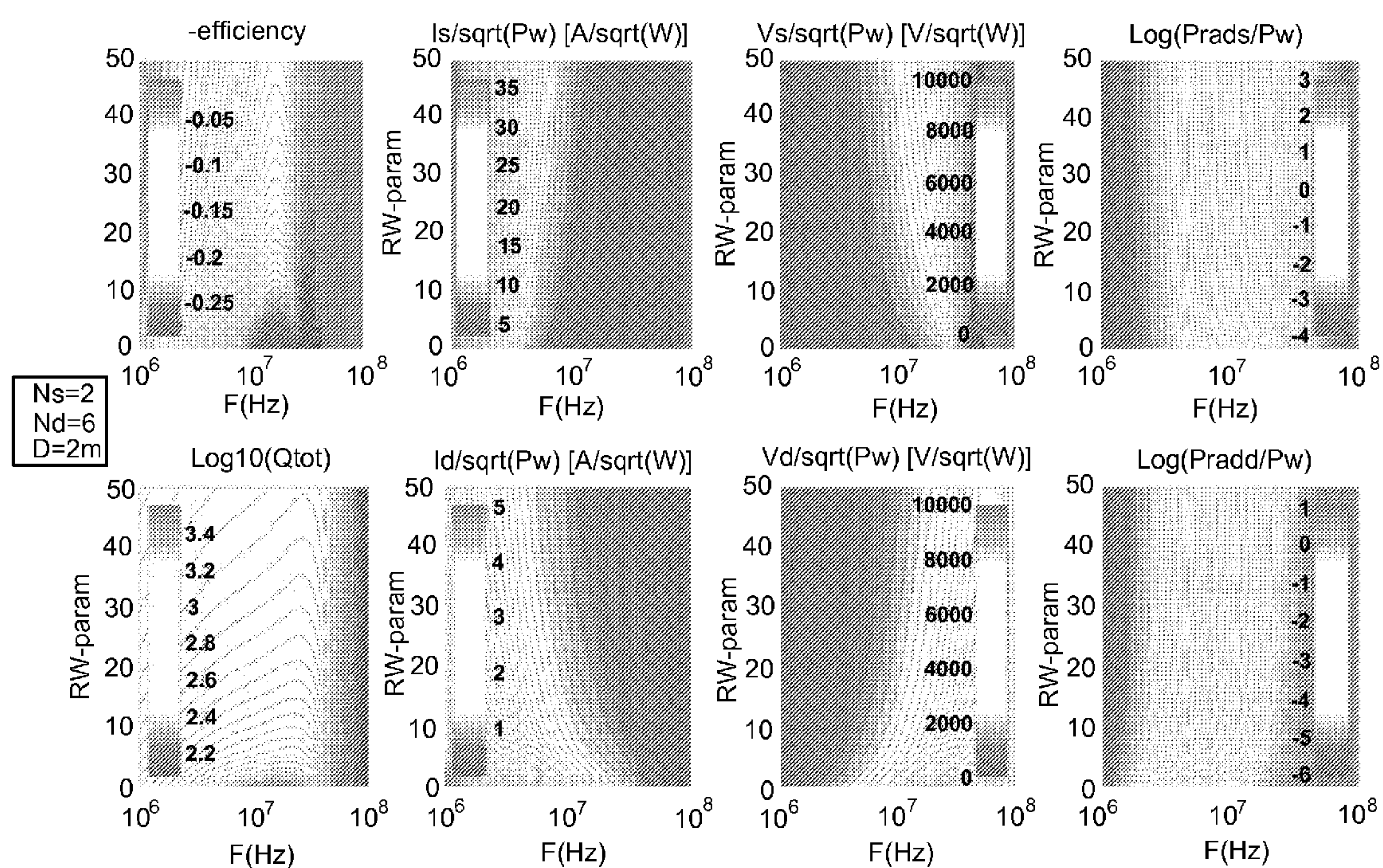
Efficiency, total (loaded) device Q , and source and device currents, voltages and radiated powers (normalized to 1Watt of output working power) as functions of frequency and w_p for a particular choice of source and device loop dimensions, and number of turns N_s and N_d .
