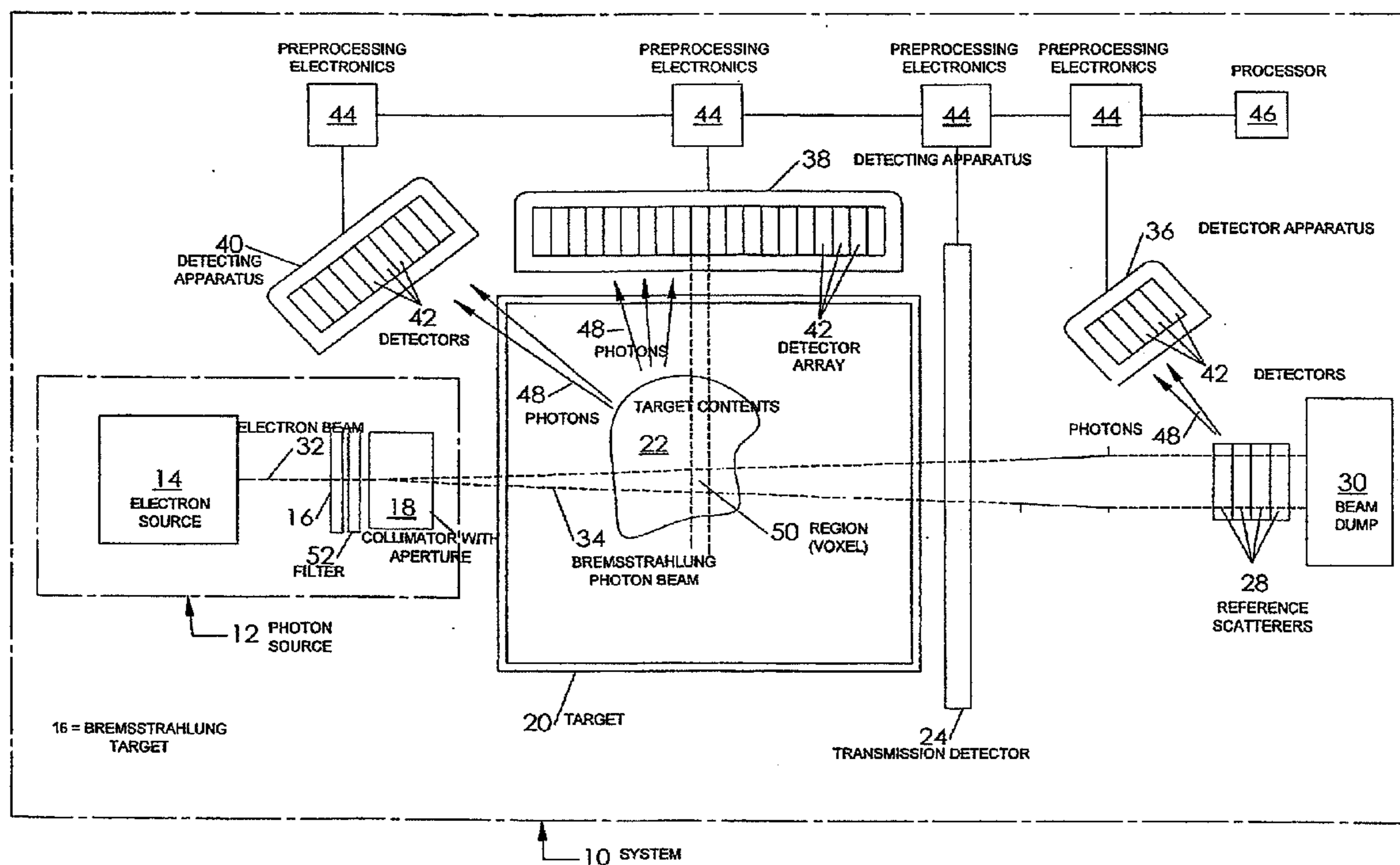
Schematic representation of Nuclear Resonance Fluorescence Scattering
