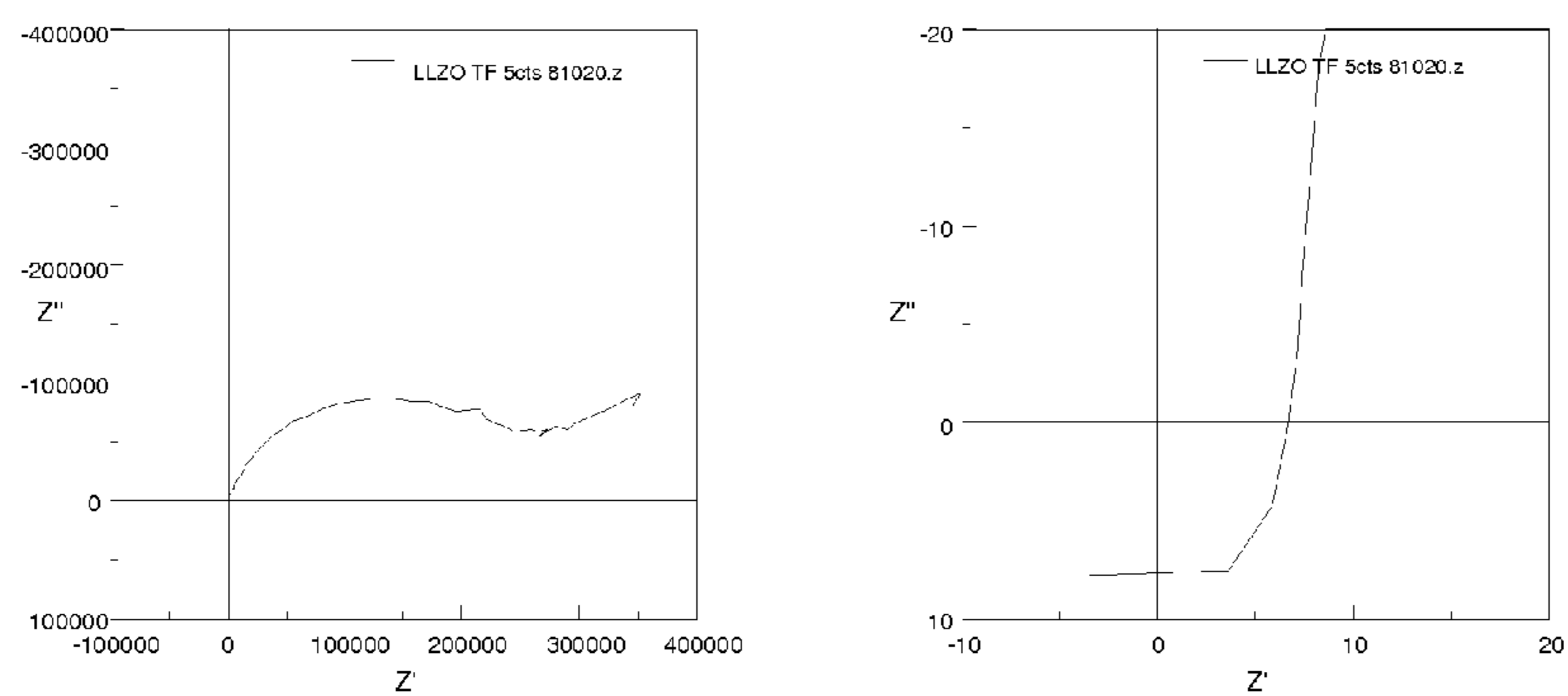
Electrochemical Impedance Spectroscopy (EIS) spectra of amorphous LLZO film Nyquist Plots Full spectrum (left): Real axis intercept (right), Magnification of Full Spectrum
