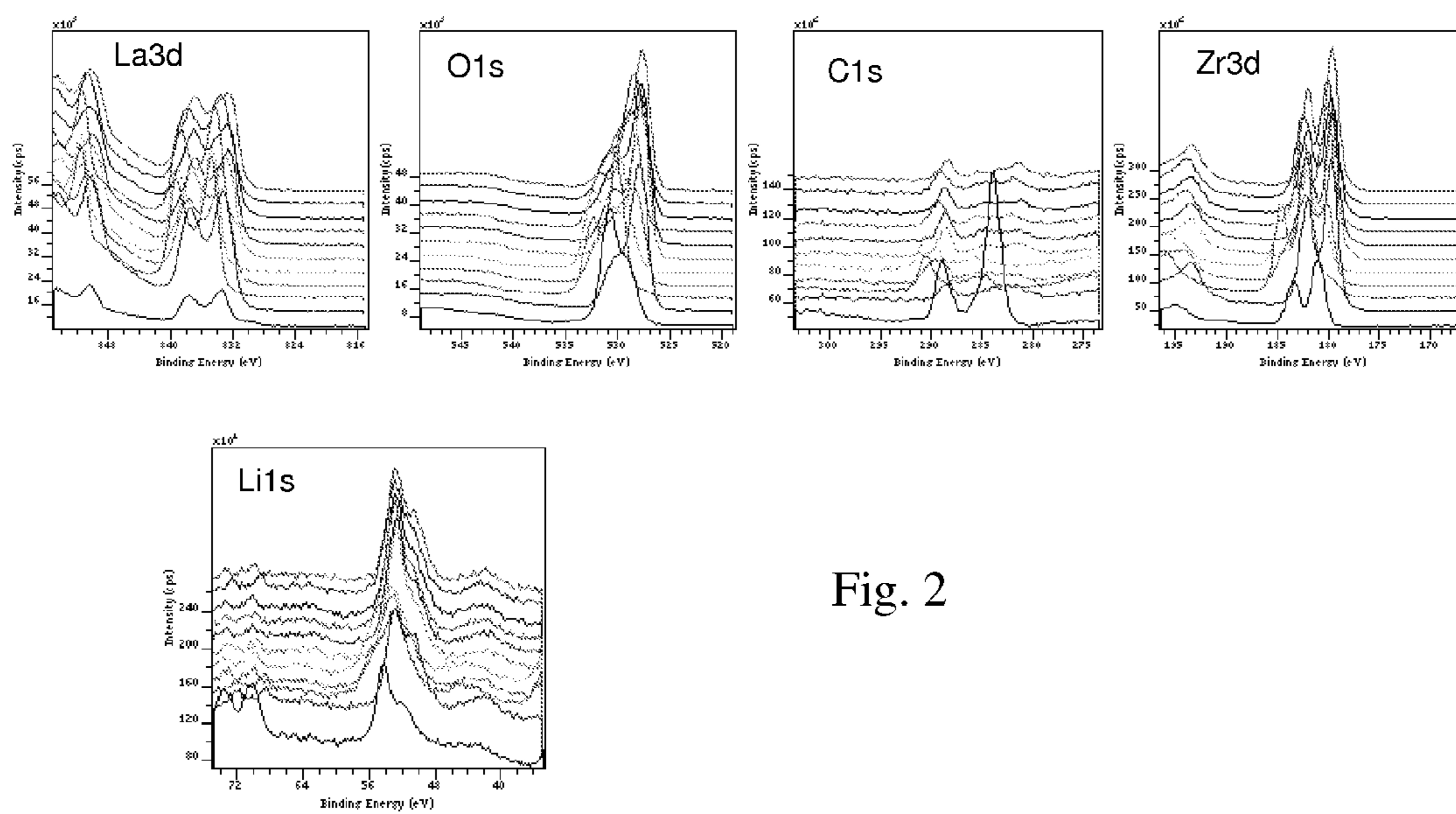
XPS Spectra Graphs For Atomic Species Constituting Sample Amorphous LLZO Film
