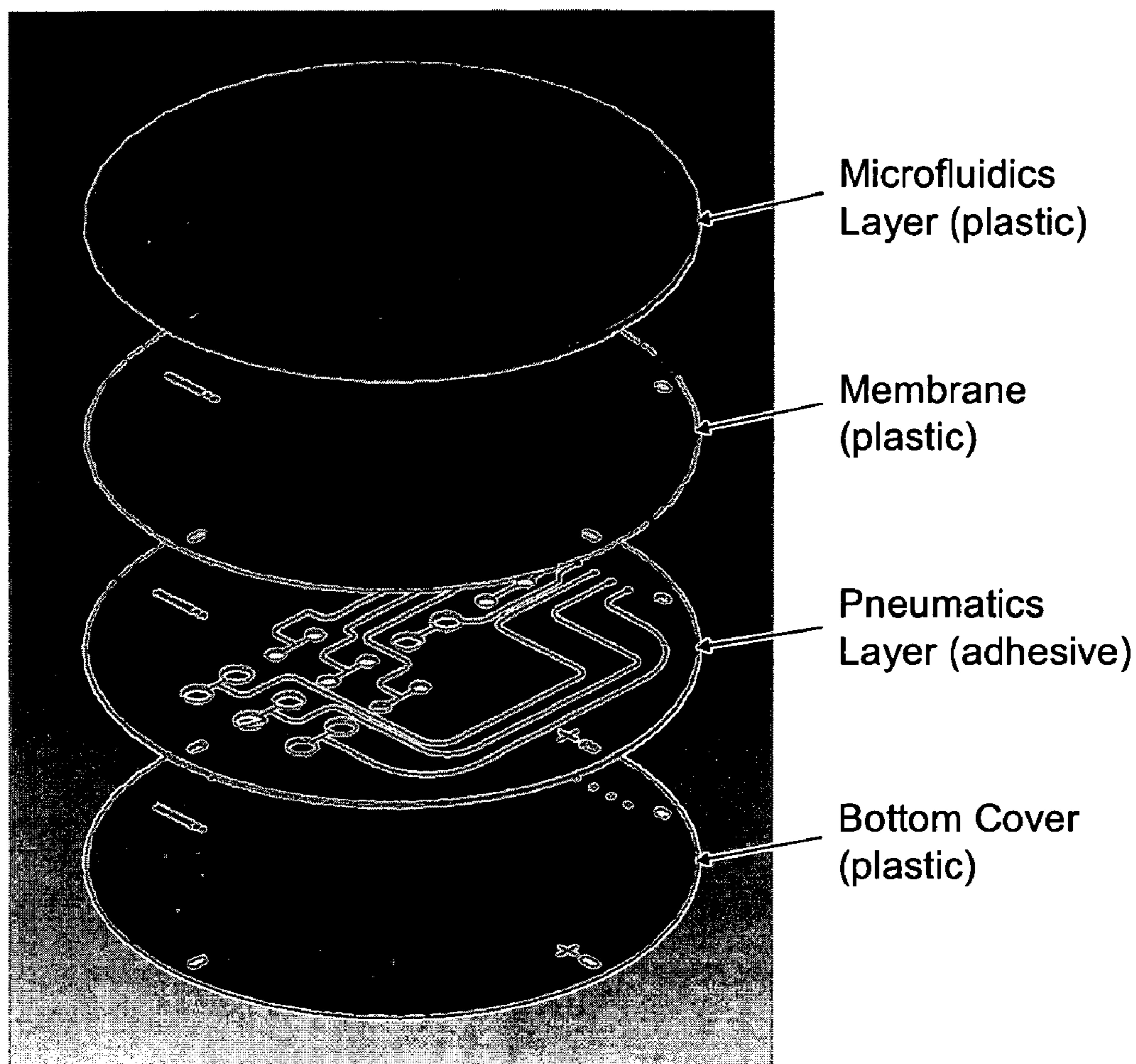
Figure 34. Hybrid plastic microchip.
