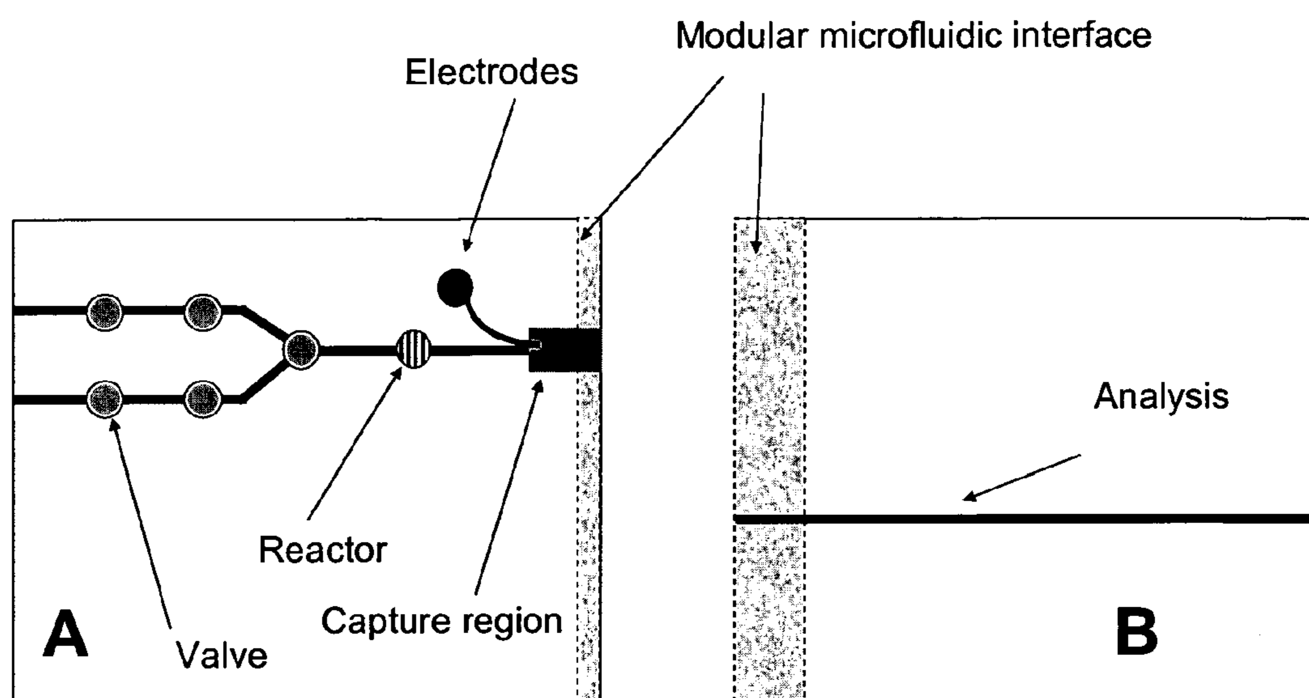
Figure 14. Capturing the sample for improved injection.
