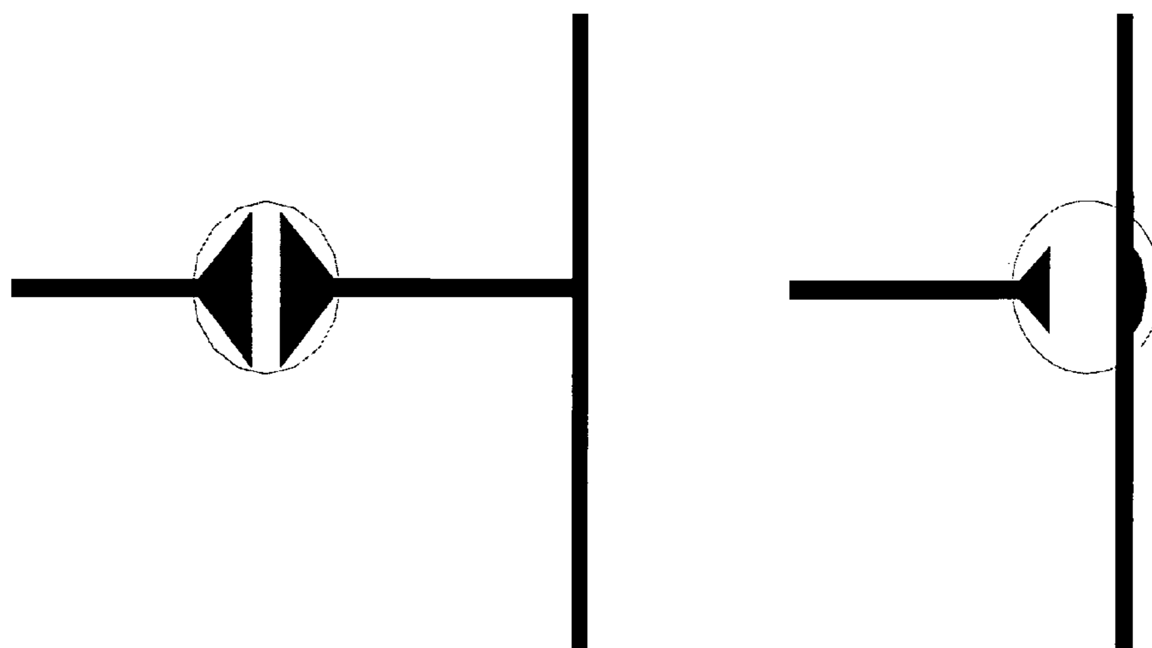
Figure 25. Use of flow through valve to eliminate dead volume at an intersection. Conventional MOV valve (left) intersection is less than ideal because it contains a section of dead volume, the section between the valve and the intersection of the tow channel is dead volume. The Flow Through valve system (right) eliminates this dead volume.
