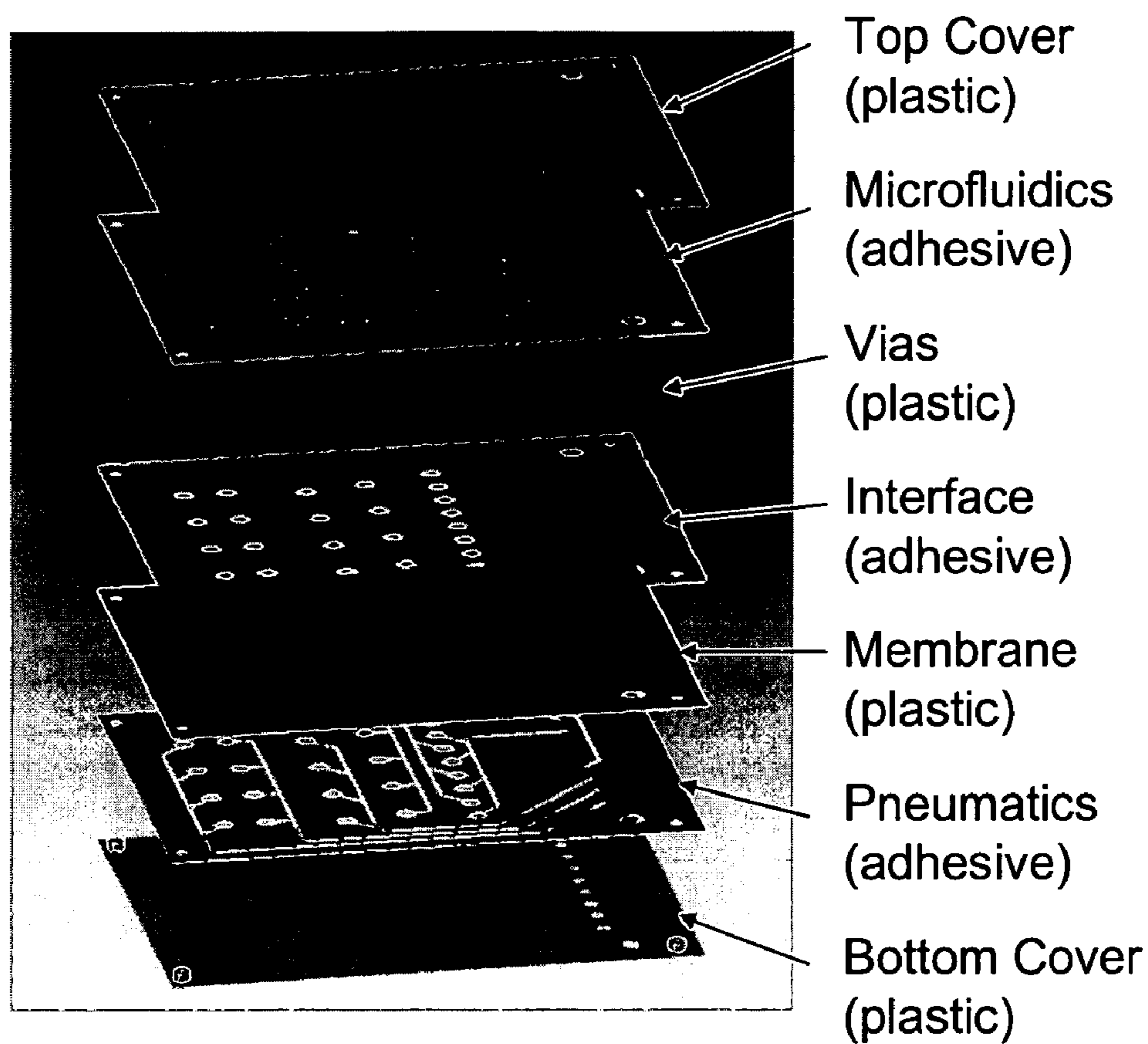
Figure 38. An embodiment of the adhered chip construction.
