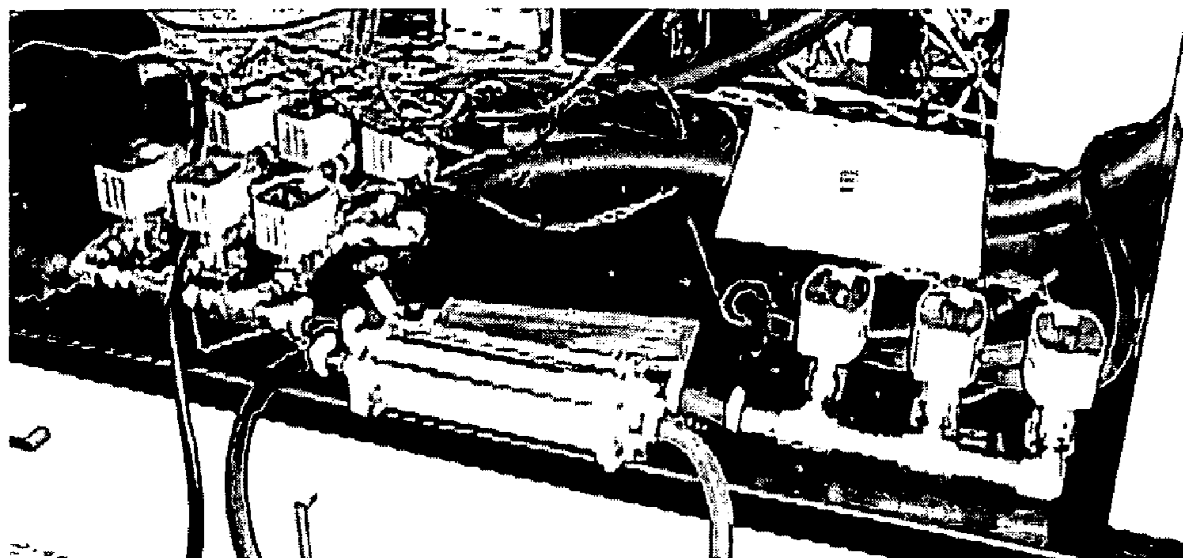
Figure 62. Circulating water thermal cycling. Three sets of three valves flank the reaction chamber.
