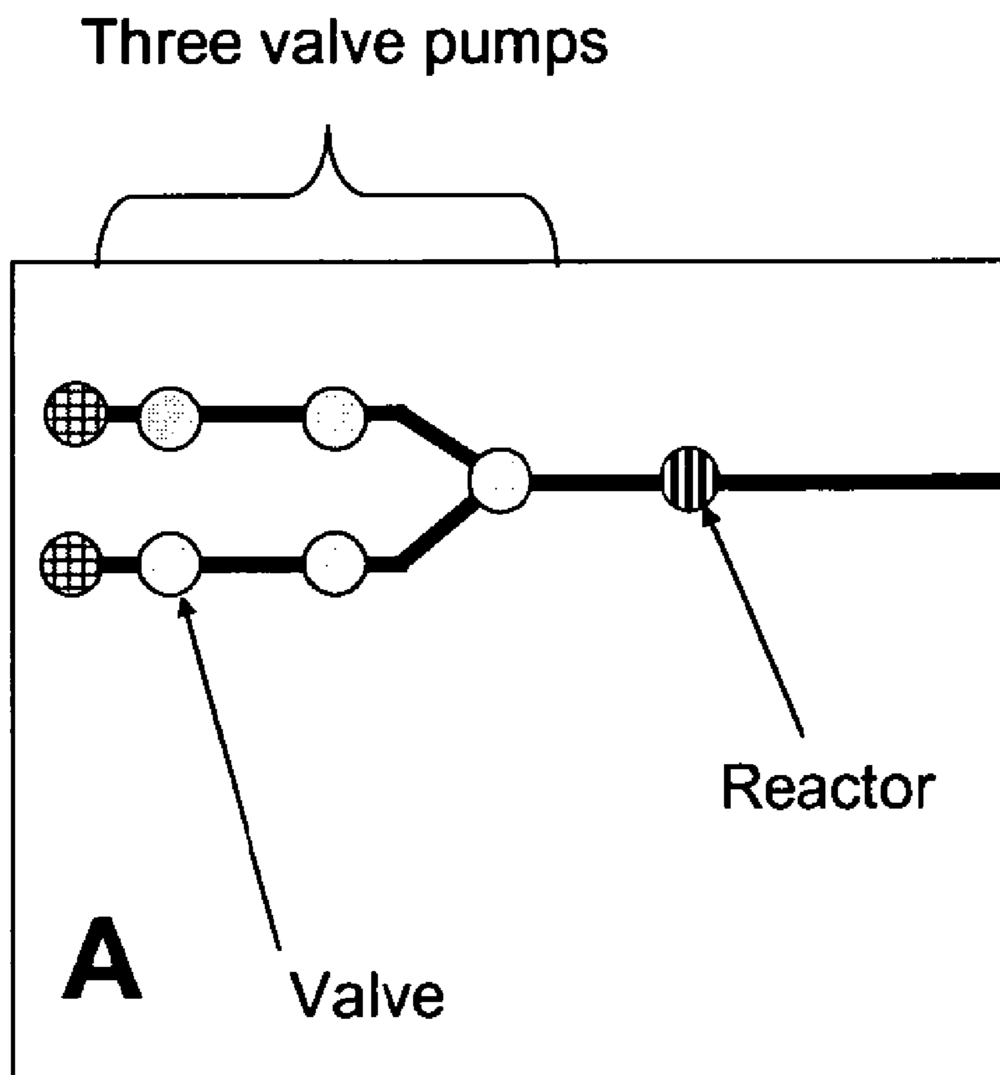
Figure 9. Mixing with reactor and moving the sample to an edge.
