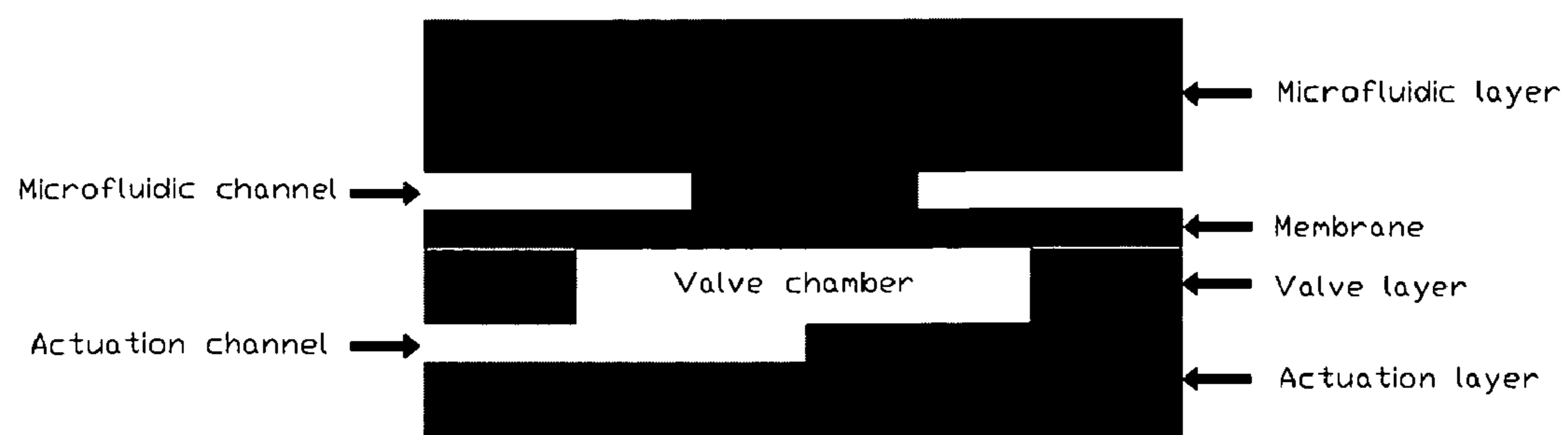
Figure 44. Cross section of a four layer valve. The valve layer allows multiple air and microfluidic crossings without cross-talking between channels.
