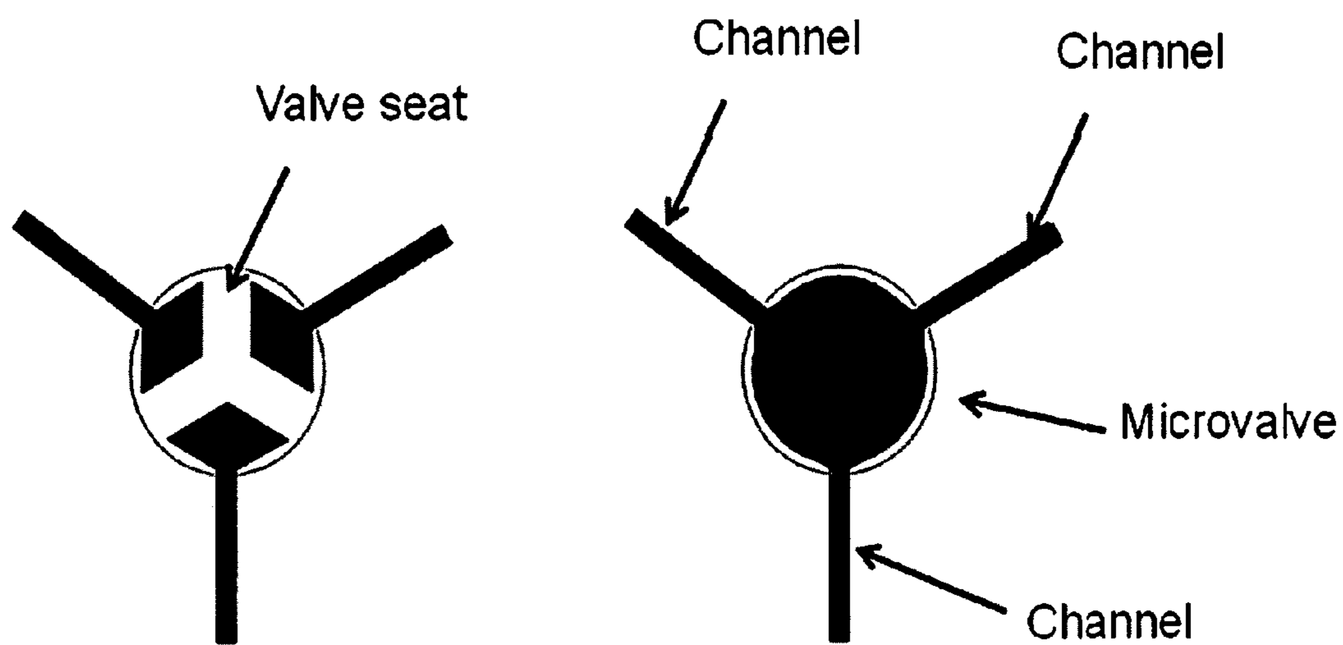
Figure 23. Y-valve in closed (left) and open (right) configuration. This valve allows for segregation of channels when desired. The valve could also aid in the mixing of reagents.
