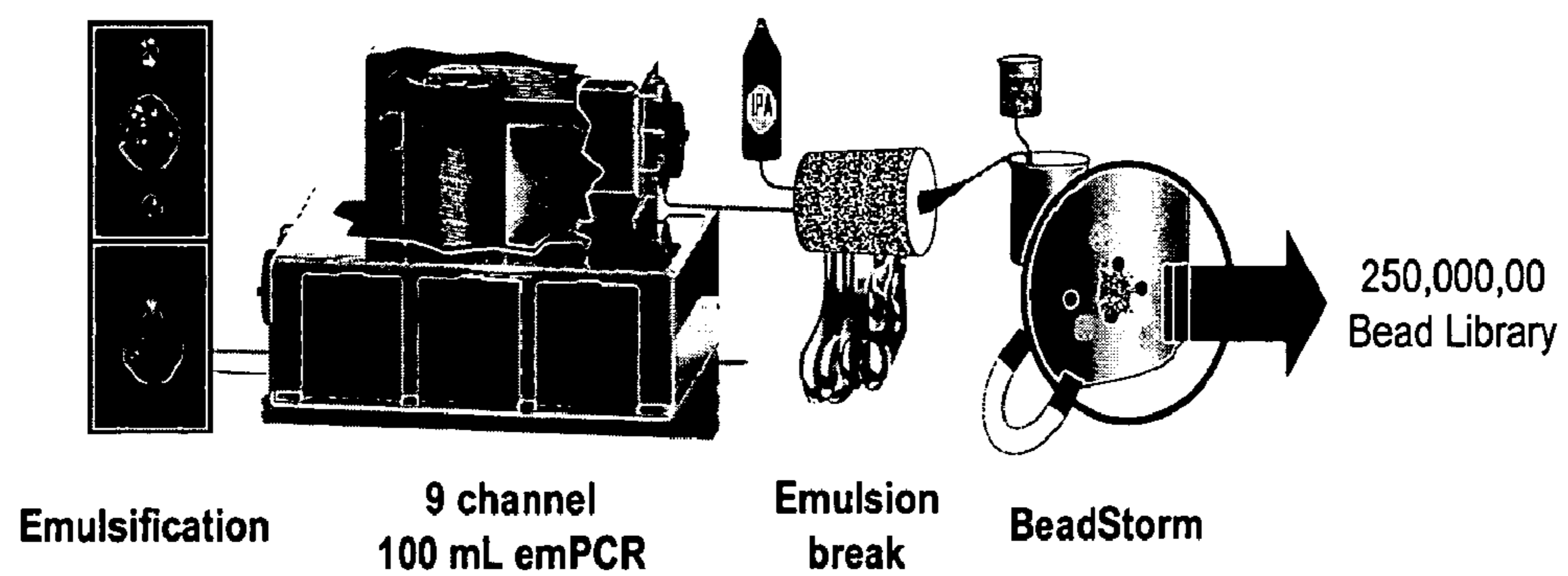
Figure 61. emPCR amplification.
