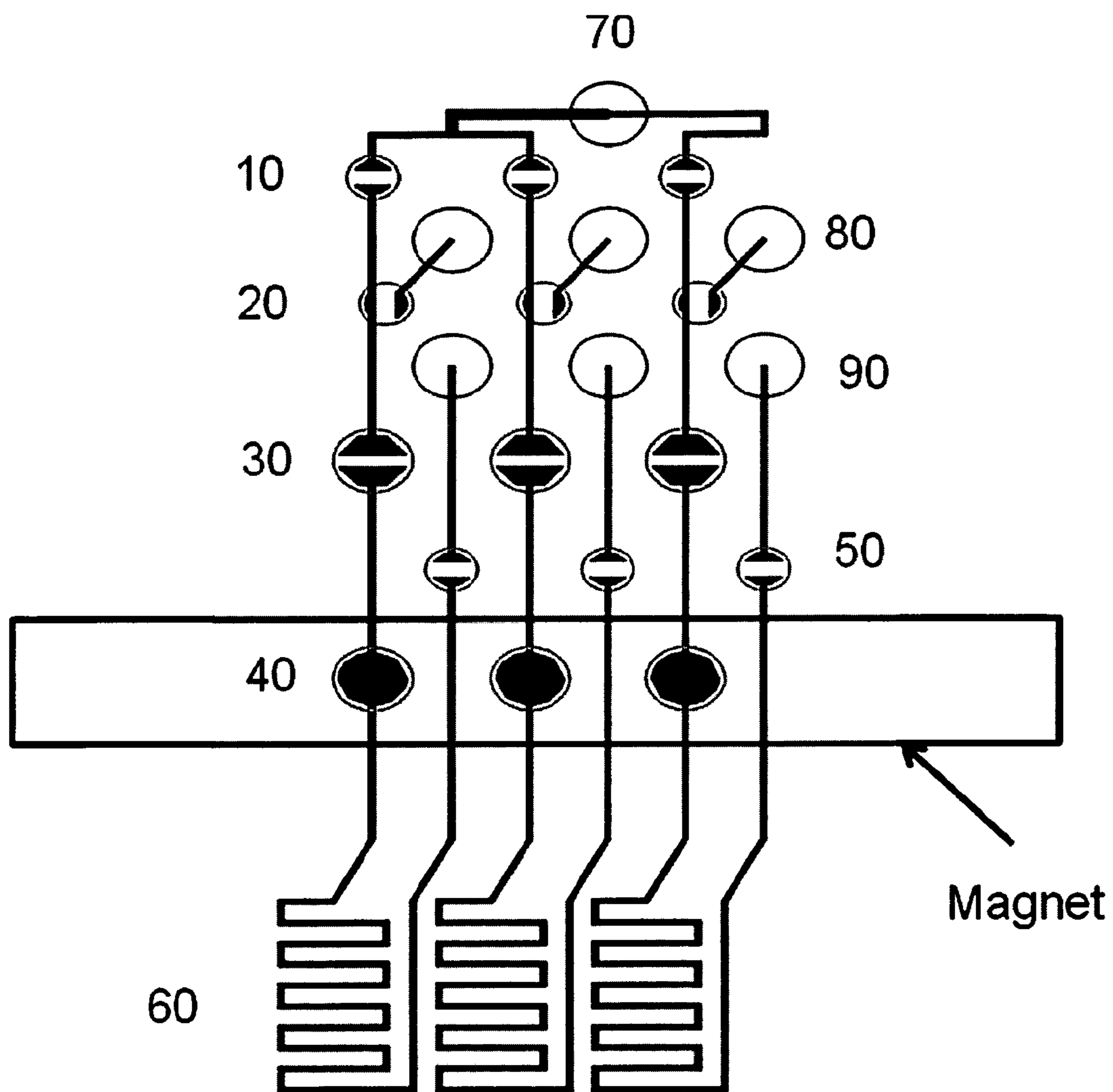
Figure 32. Compact Integrated design.
