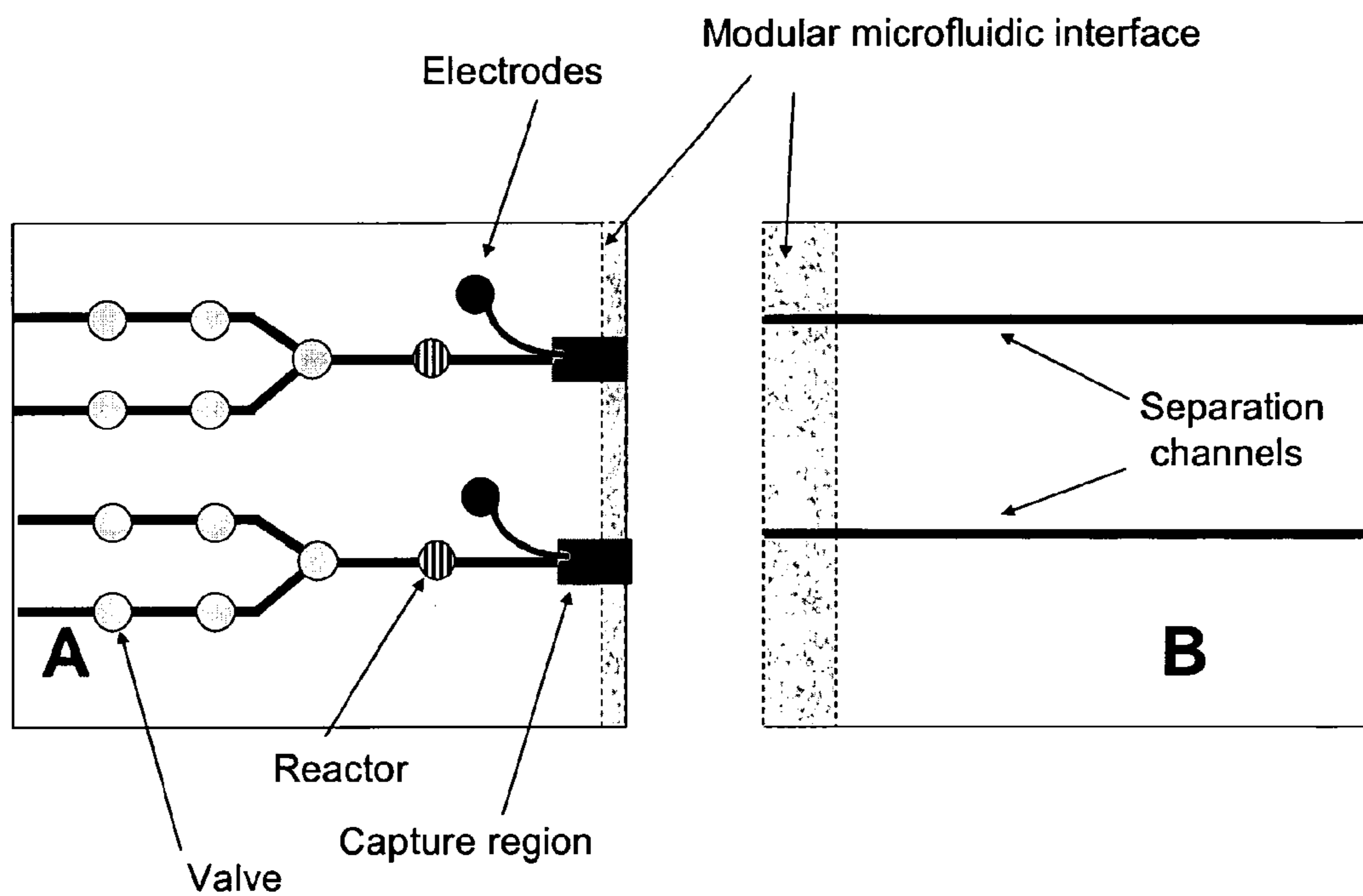
Figure 15. Multiple channels of sample preparation and analysis.
