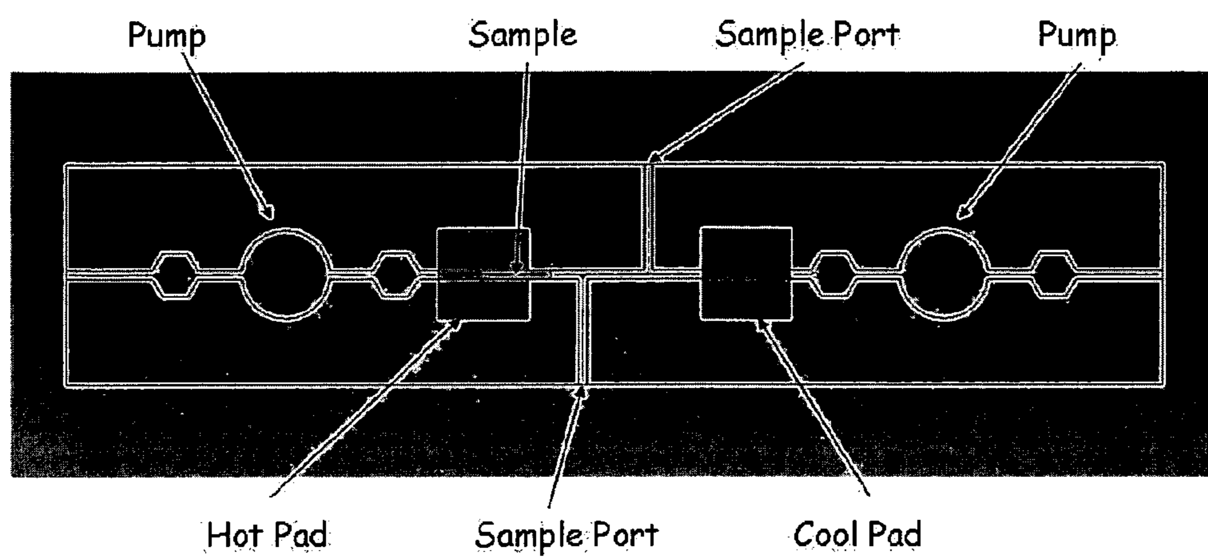
Figure 49: Alternative concept using an immiscible fluid on either side of the sample so the sample does not go through the pumps.
