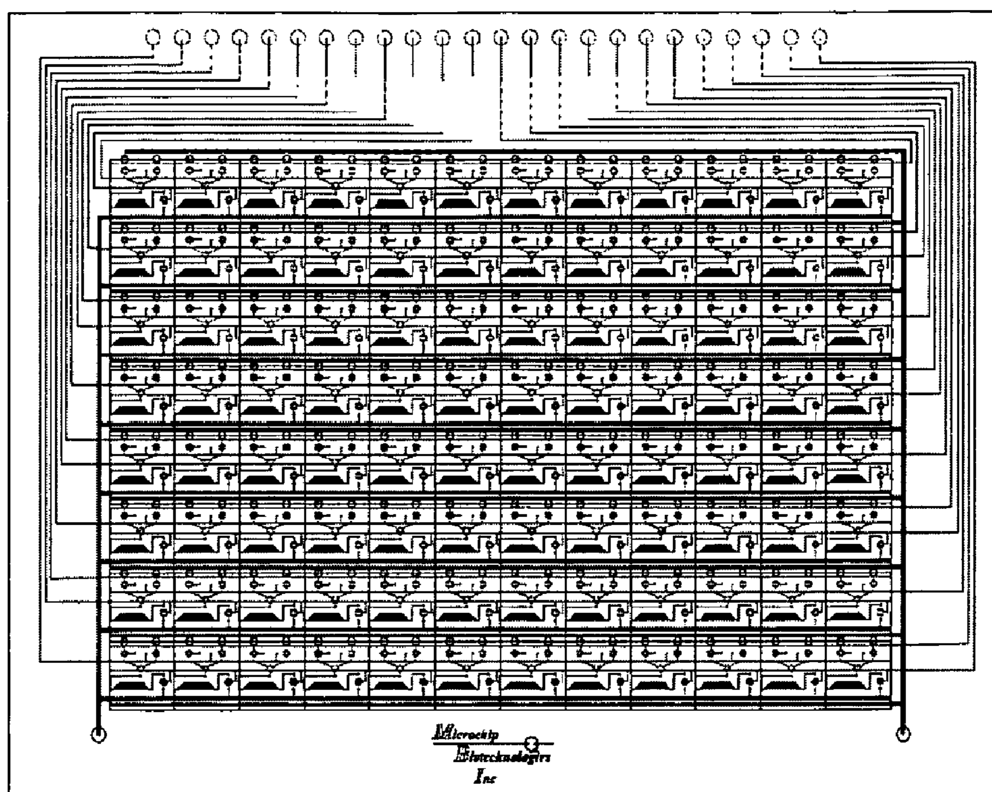
Figure 59. 96 ligation circuits. The red 16 lines are pneumatics. The blue lines are microfluidics.
