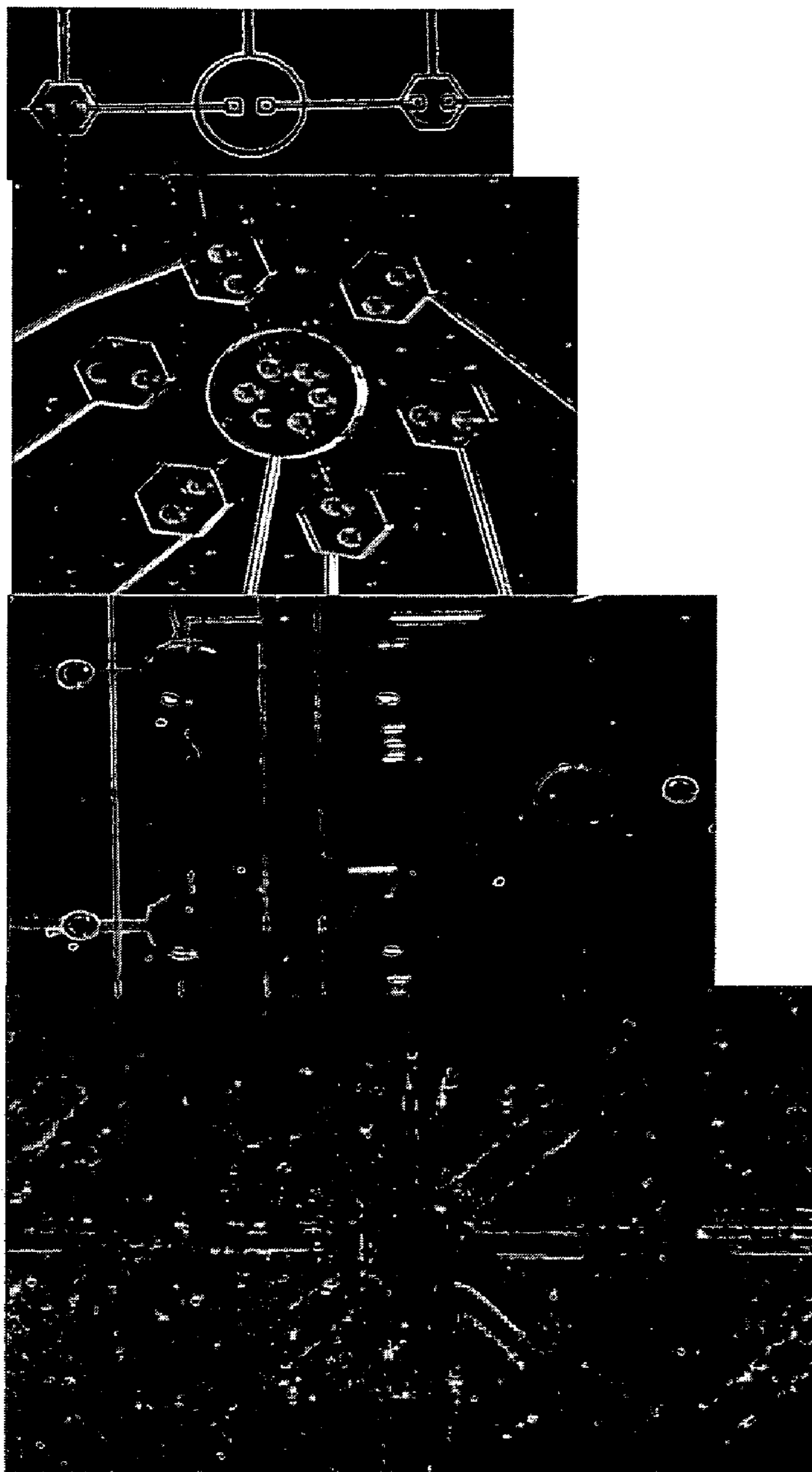
Figure 3. MOV devices from top to bottom: valve, router, mixer, bead capture.
