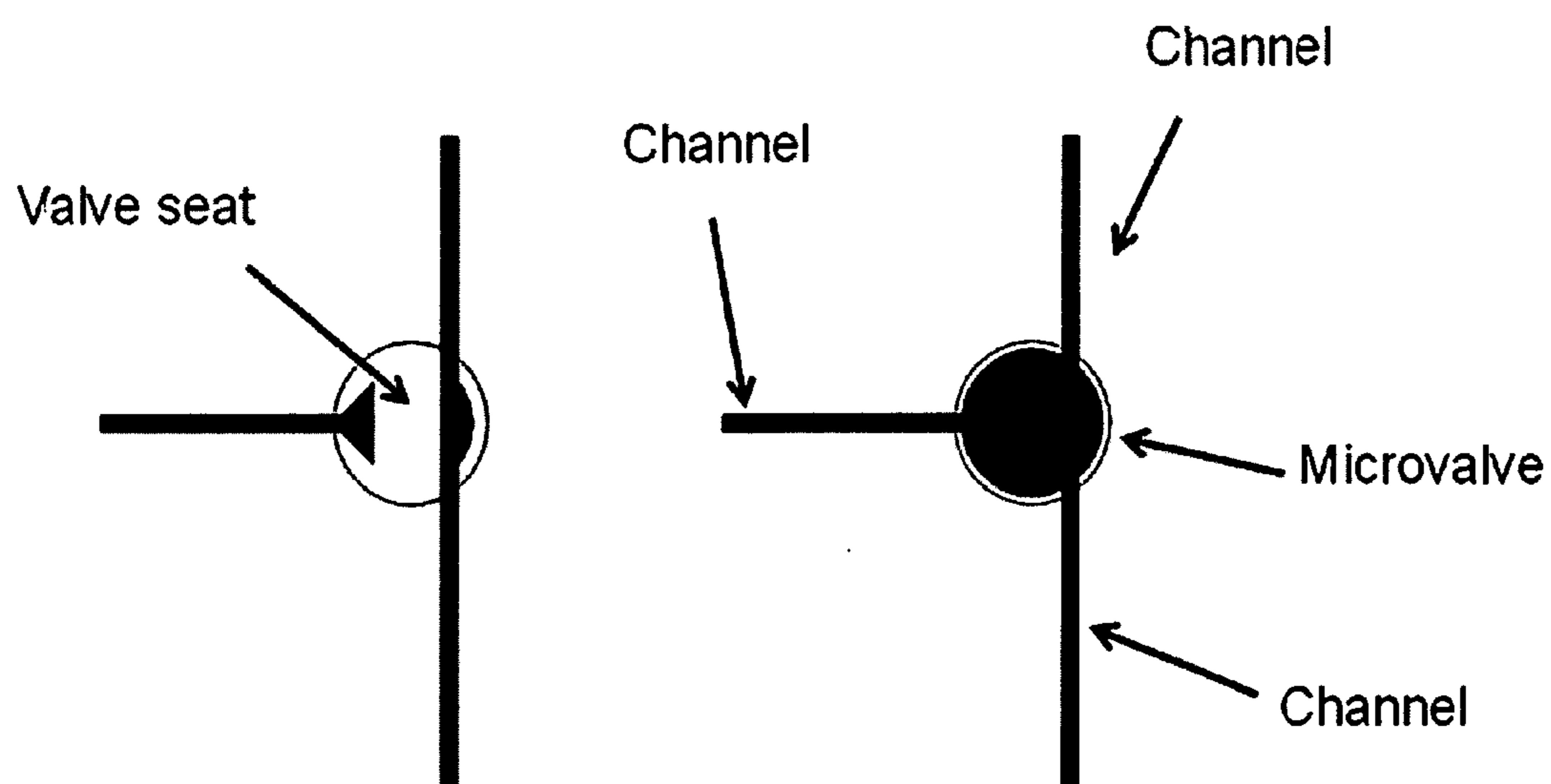
Figure 24. Flow through MOV valve. Closed configuration (left) allows for movement of fluid in the vertical channel while isolated from the horizontal channel. When in an open configuration (right), the channel can flow into one another.
