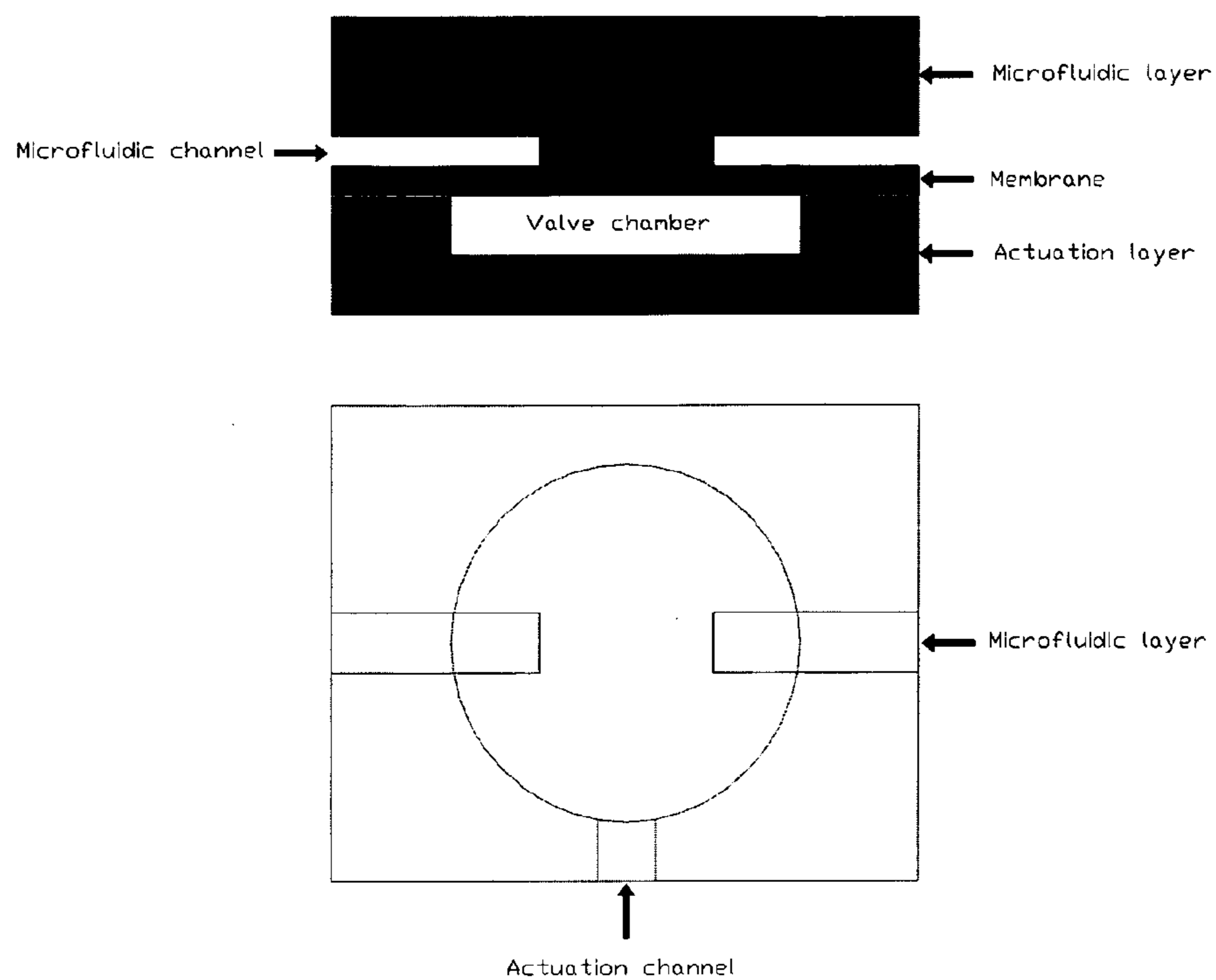
Figure 42: Structure of a valve fabricated on a three layer plastic laminated microfluidic chip.
