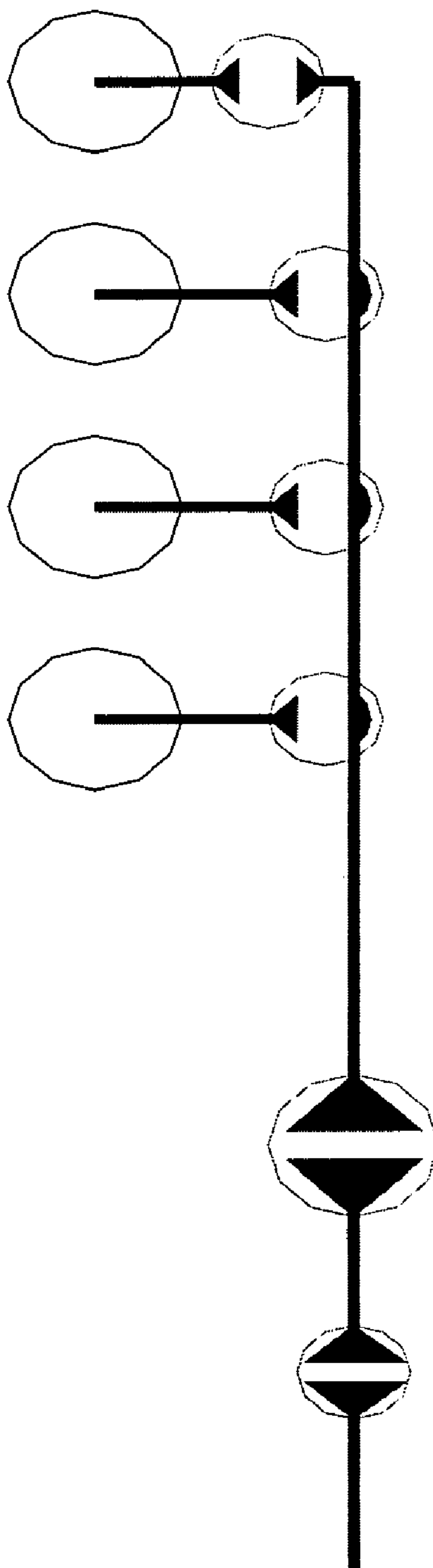
Figure 30. Reagent delivery system using a single set of pumping valves.
