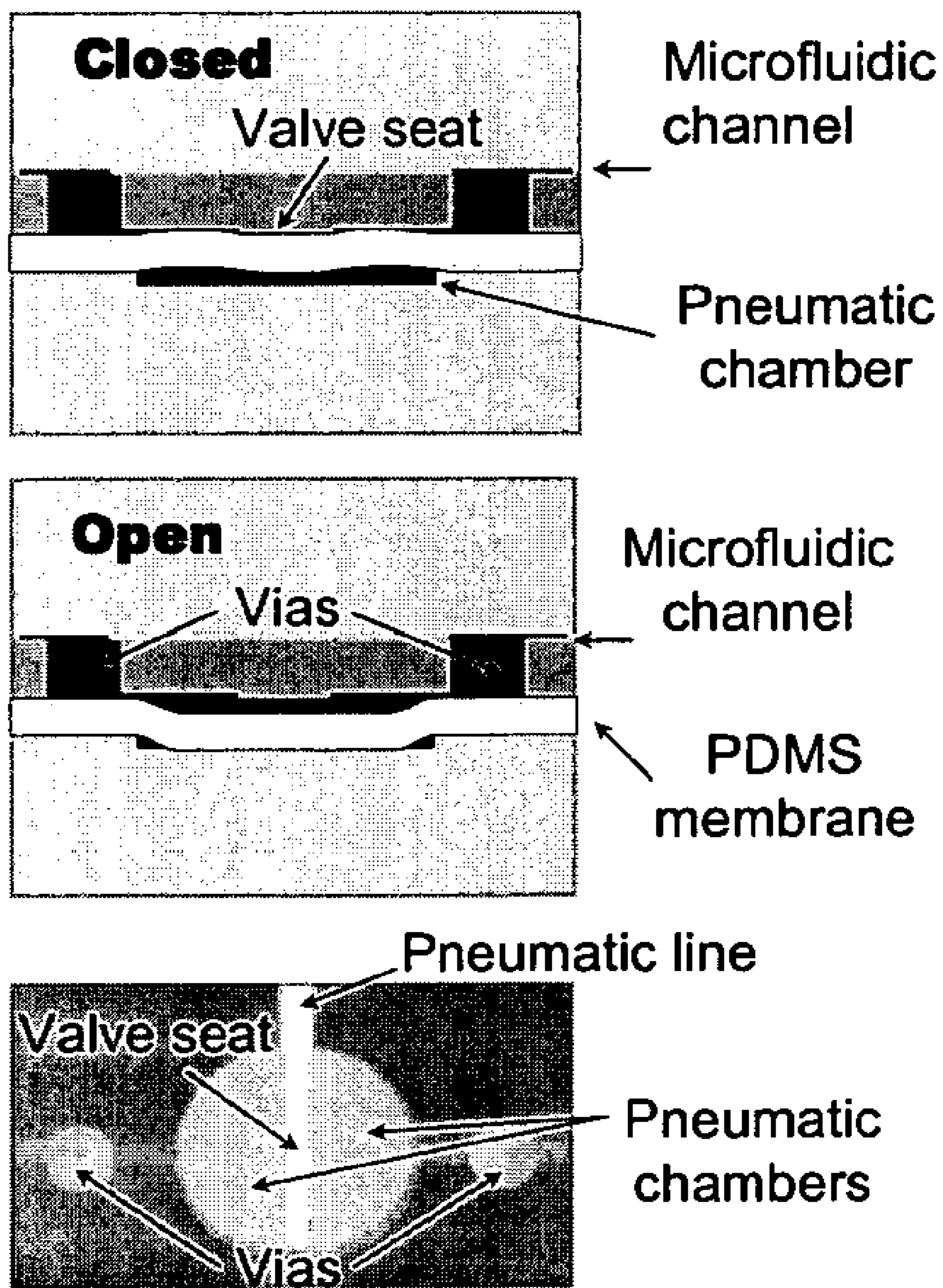
Figure 2. MOV valve.
