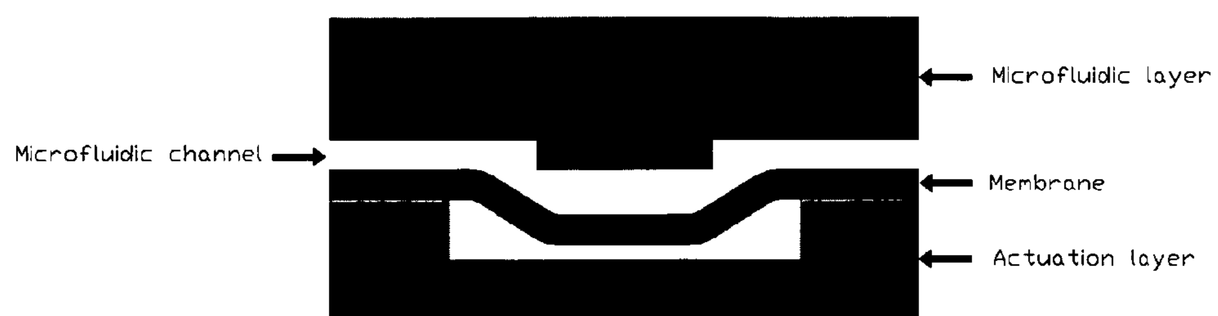
Figure 43. Cross section of a normally open valve obtained by inflating the membrane during the lamination.
