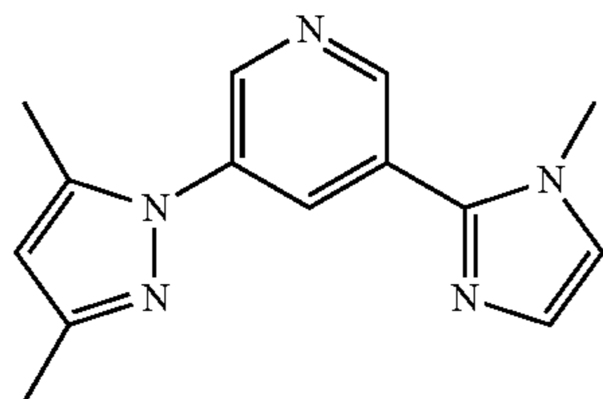
DMPz-Py-IMz
