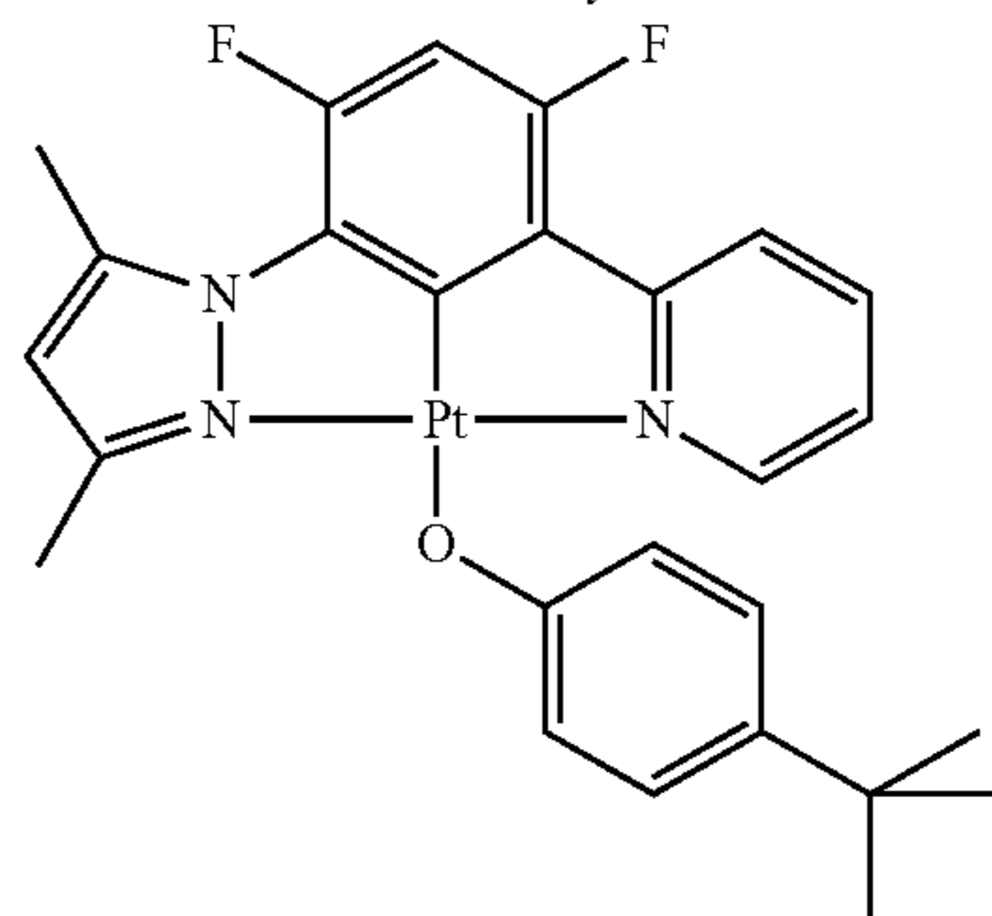
DMPz-DFPh-Py-PtOPhBu
