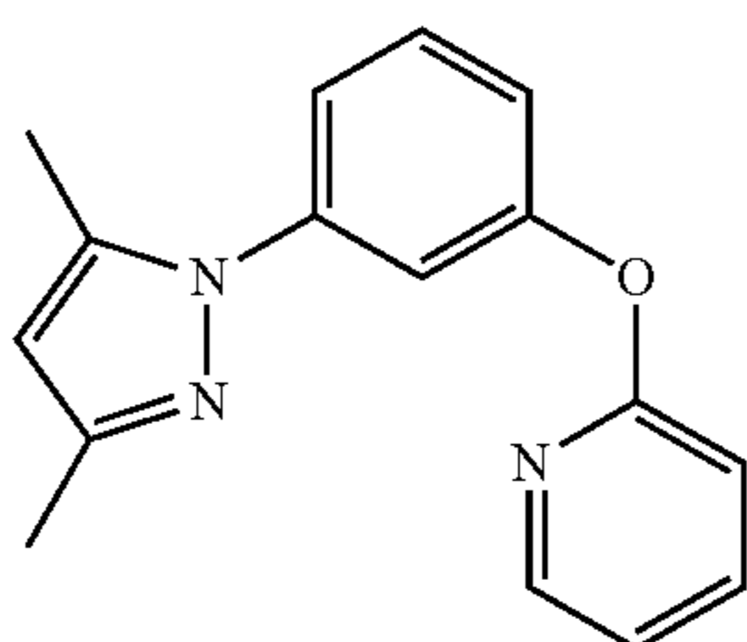
DMPz-Ph-O-Py
