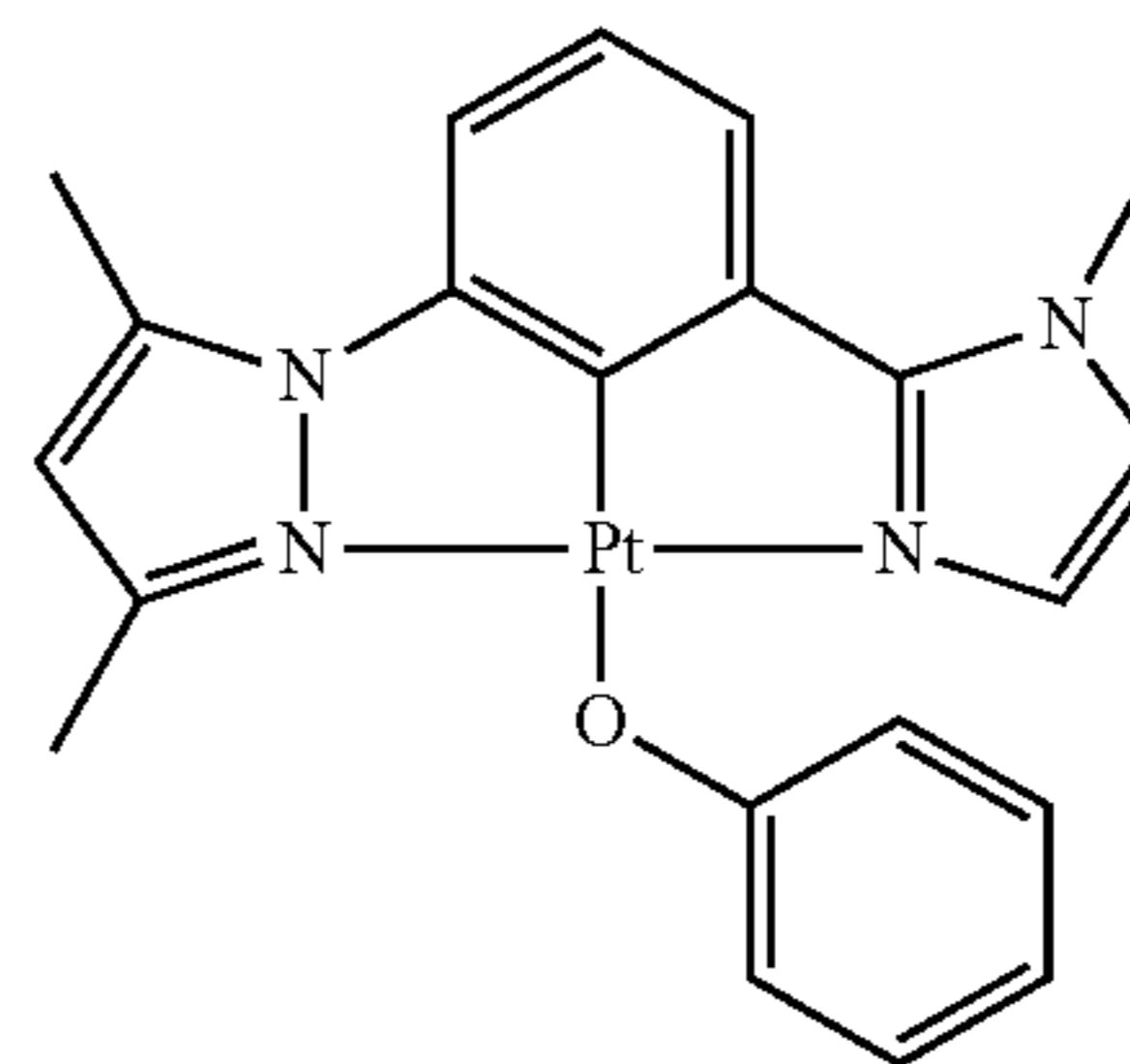
DMPz-Ph-MIz-PtOPh
