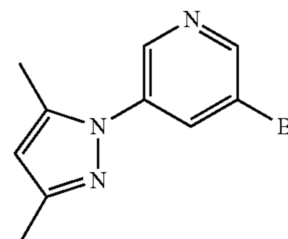
DMPz-Py-Br
