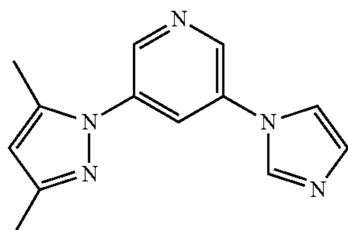
DMPz-Py-Iz
