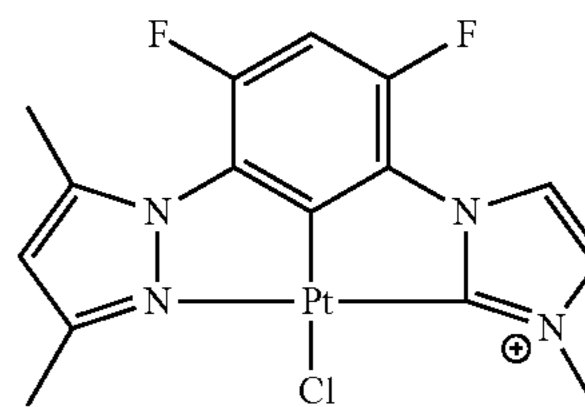
DMPz-Ph-MIzCb-PtCl
