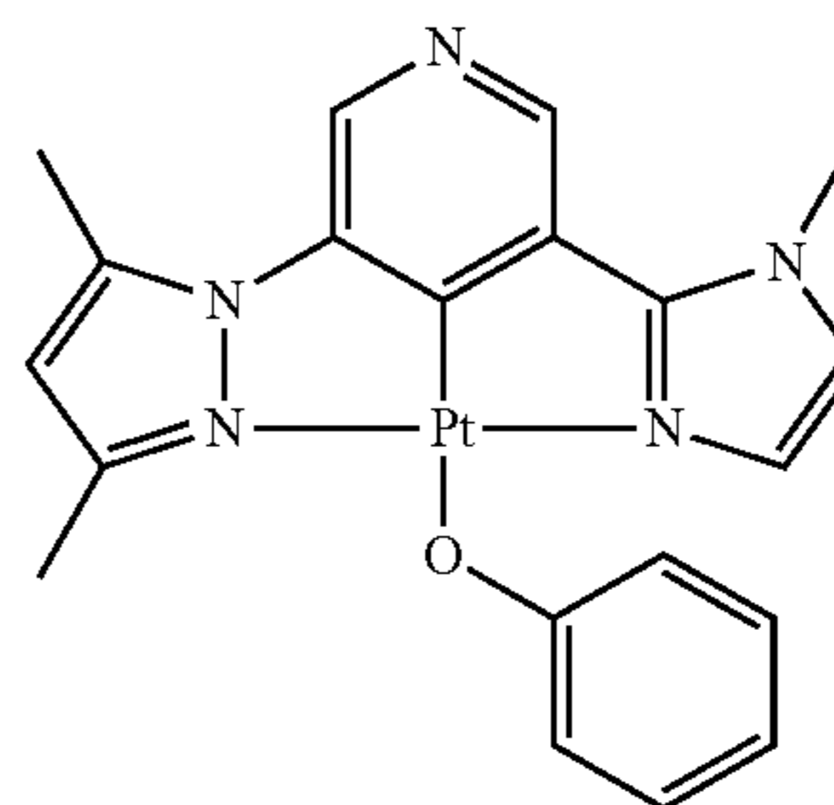
DMPz-Py-MIz-PtOPh
