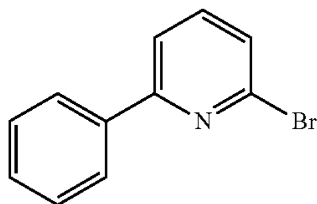
Ph-Py-Br
