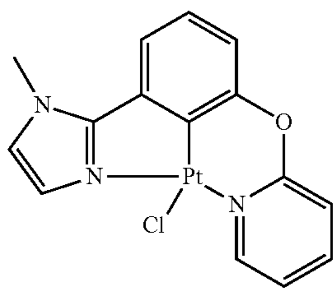
MIz-Ph-O-Py-PtCl
