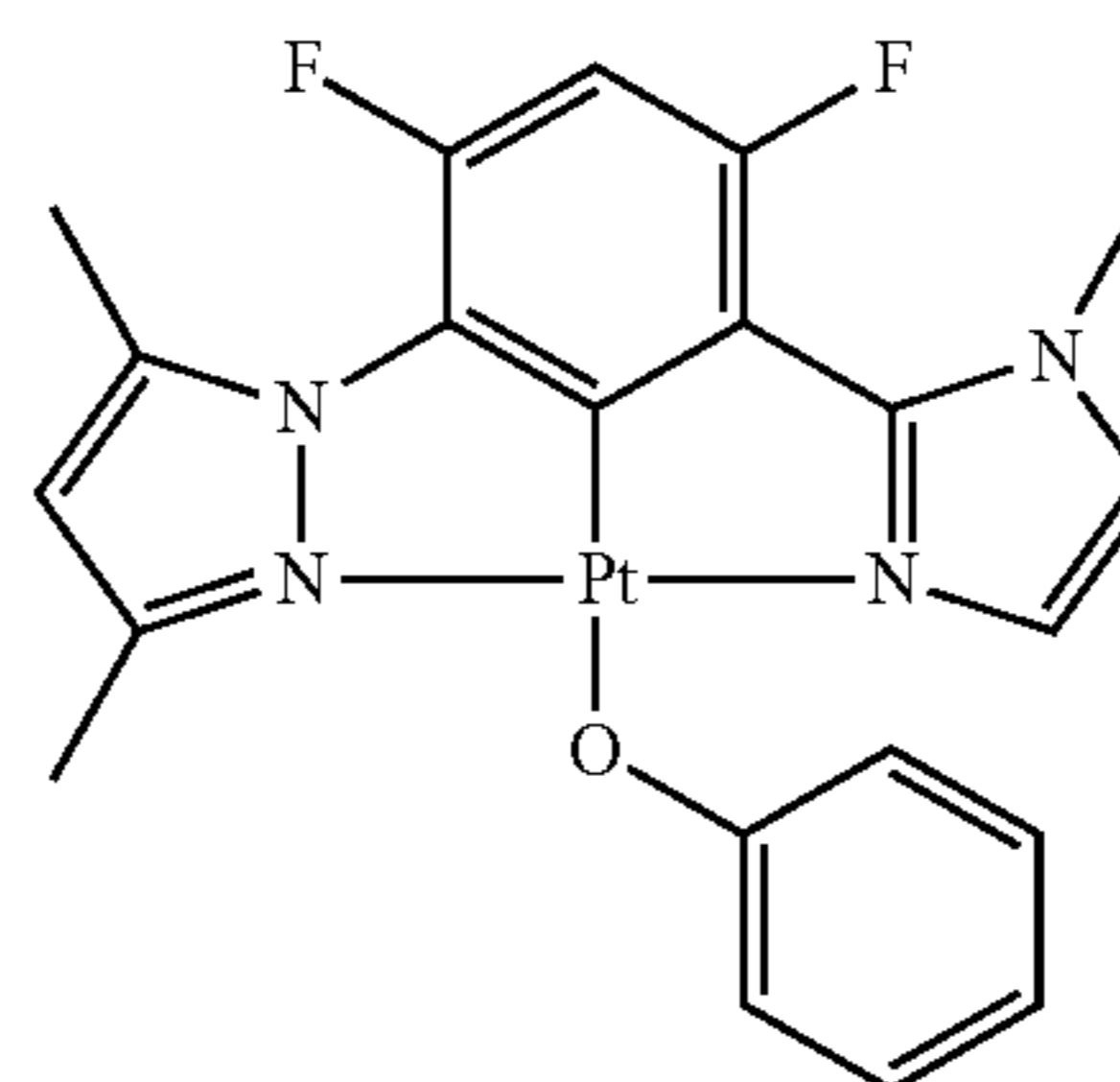
DMPz-DFPh-MIz-PtOPh
