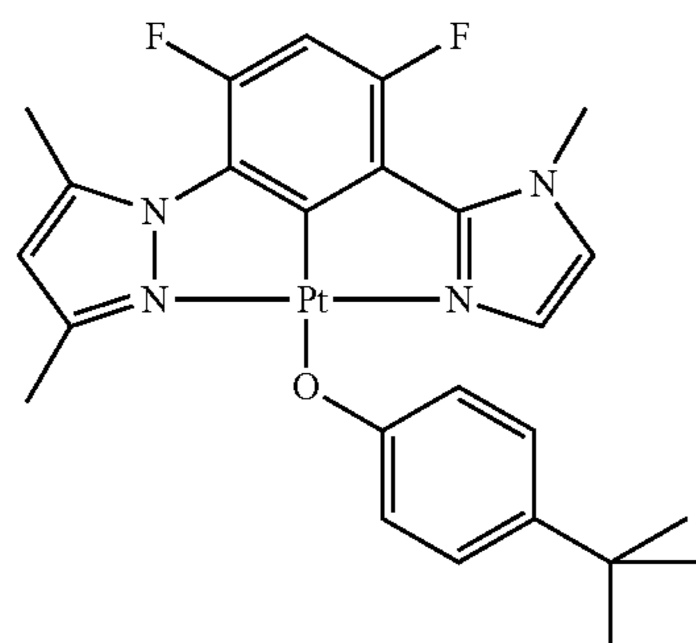
DMPz-DFPh-MIz-PtOPhBu
