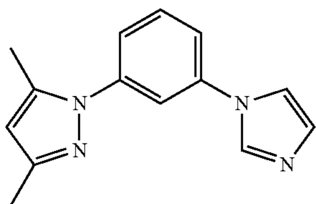
DMPz-Ph-Iz
