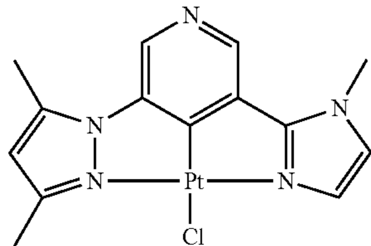
DMPz-Ph-MIz-PtCl
