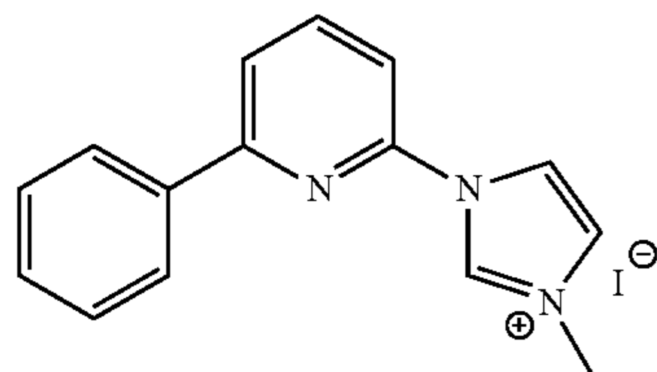
Ph-Py-IMIz
