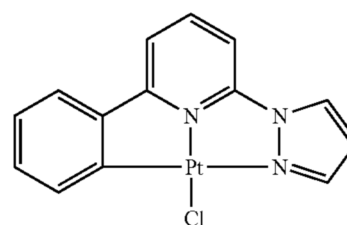
Ph-Py-Pz-PtCl
