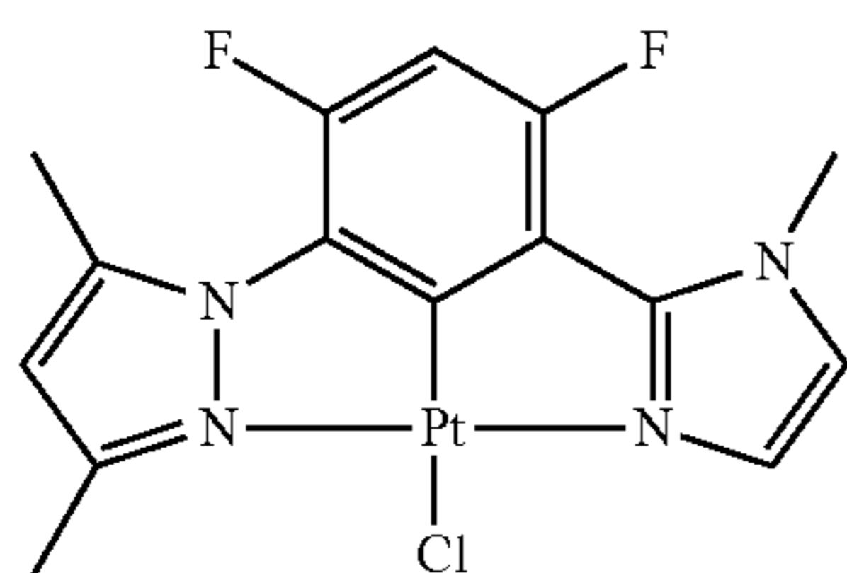
DMPz-DFPh-MIz-PtCl
