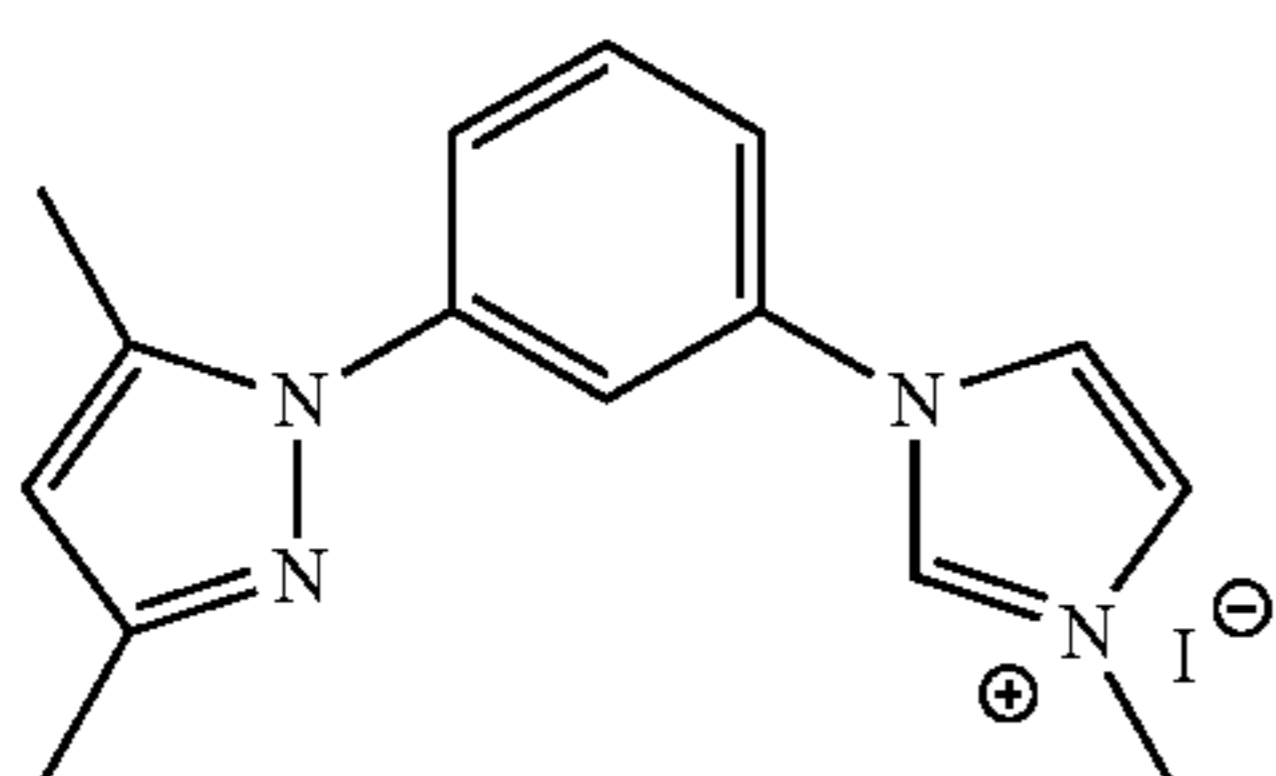
DMPz-Ph-IMIz
