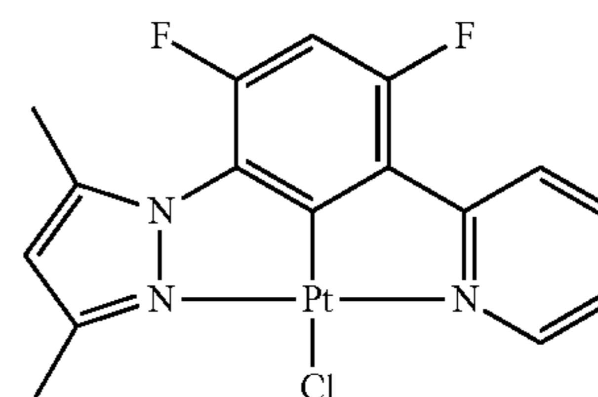
DMPz-DFPh-Py-PtCl
