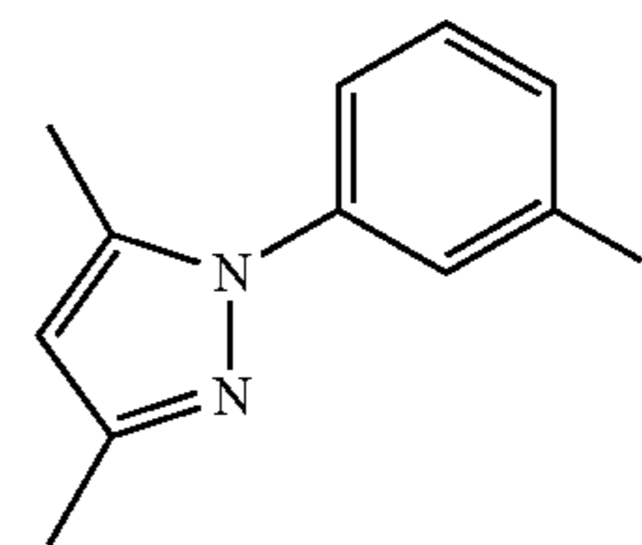
DMPz-Ph-I
