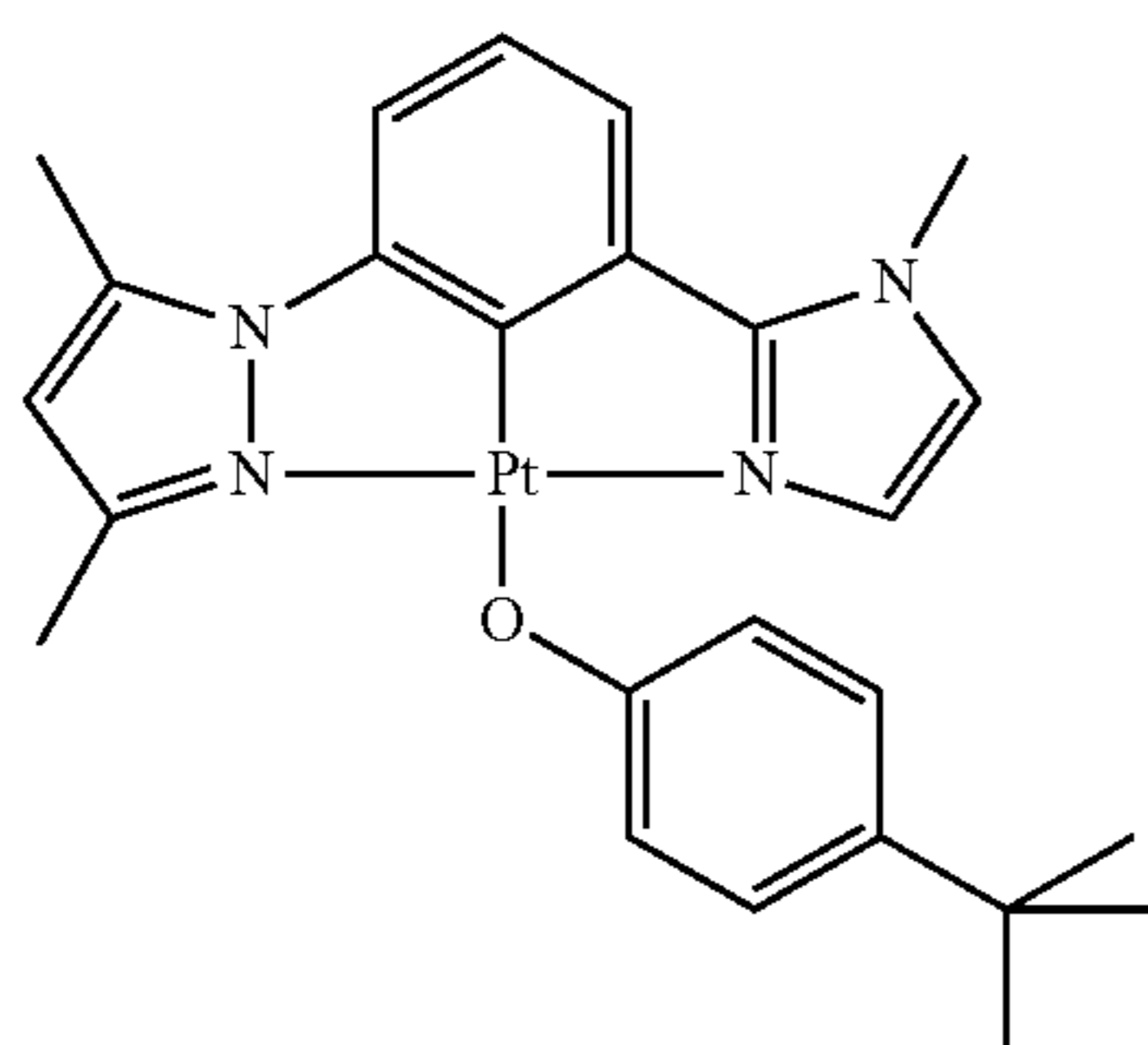
DMPz-Ph-MIz-PtOPhBu
