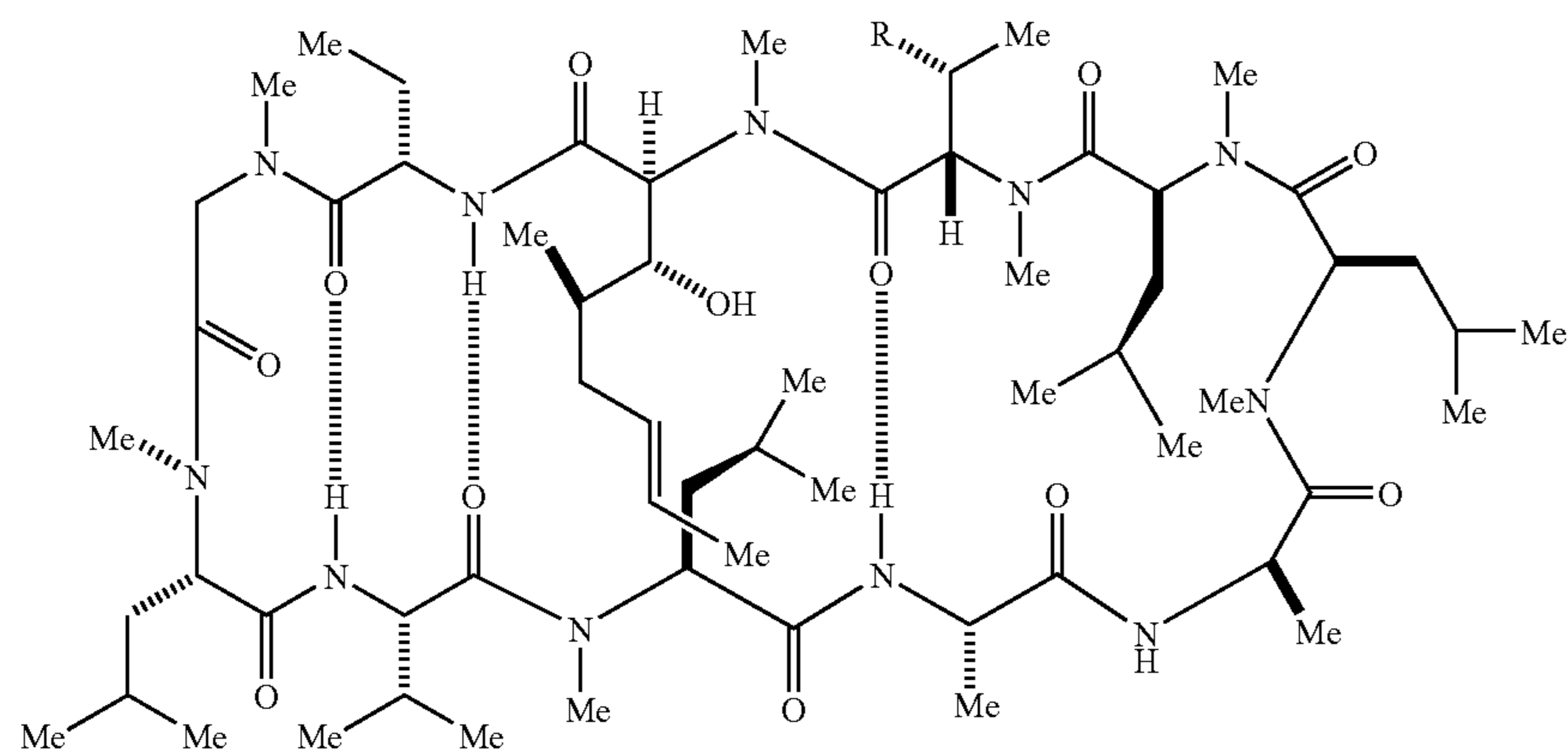
1 (R = Me): CsA 2 (R = Me): Modified [MeVal 11 ]CsA
