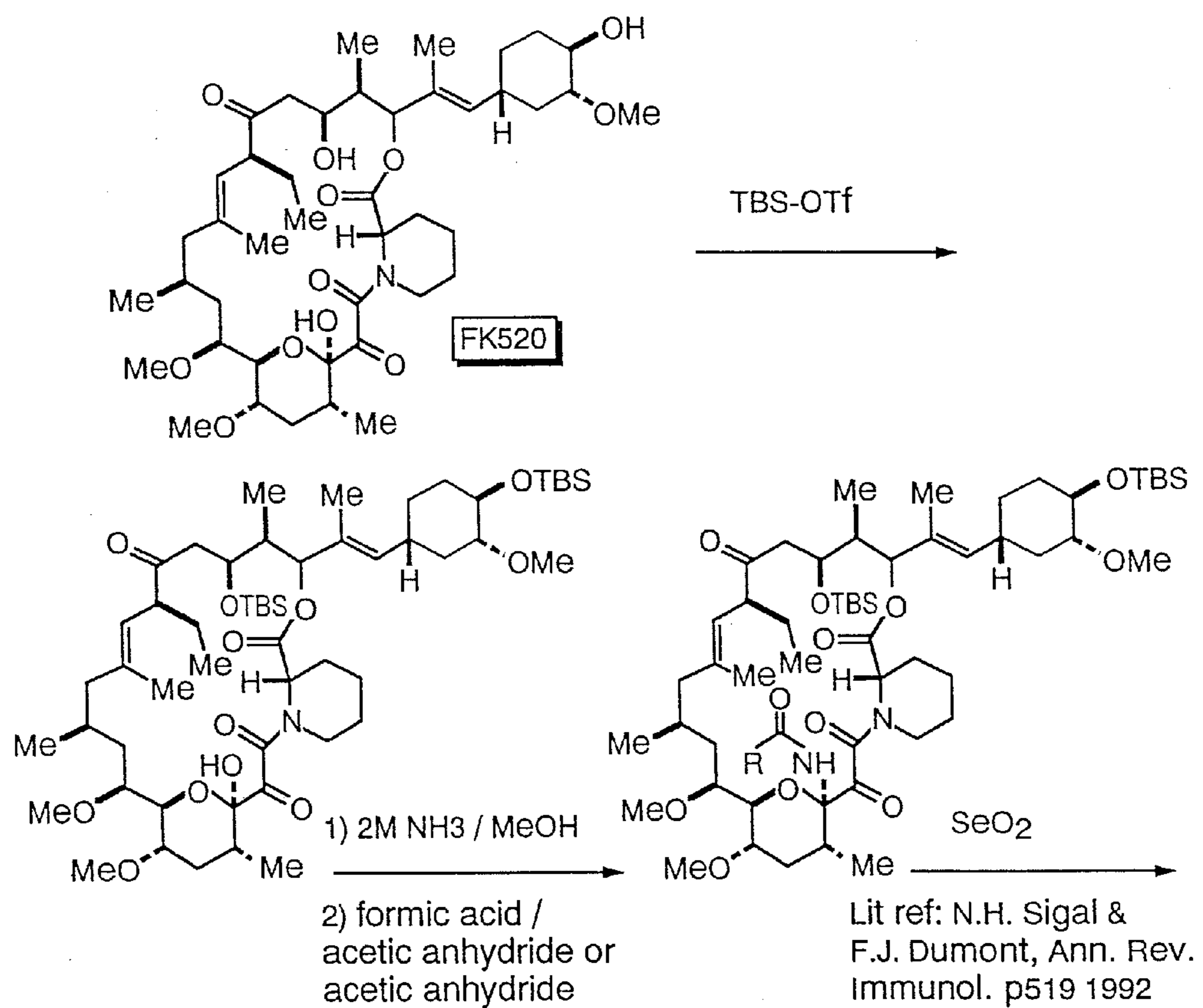
Scheme 2: Synthesis of Dimers
