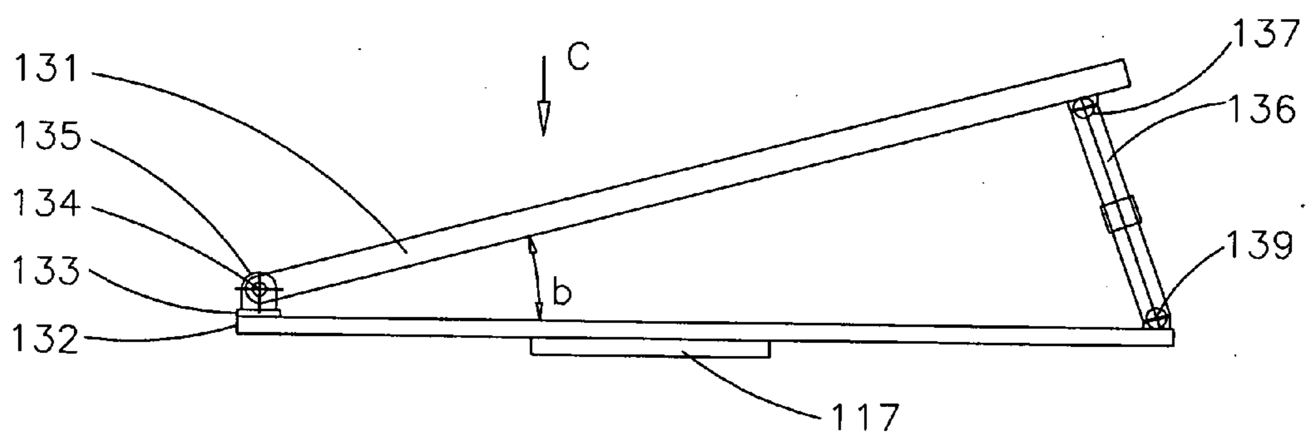
FIG. 13 (SECTION X-Y)
