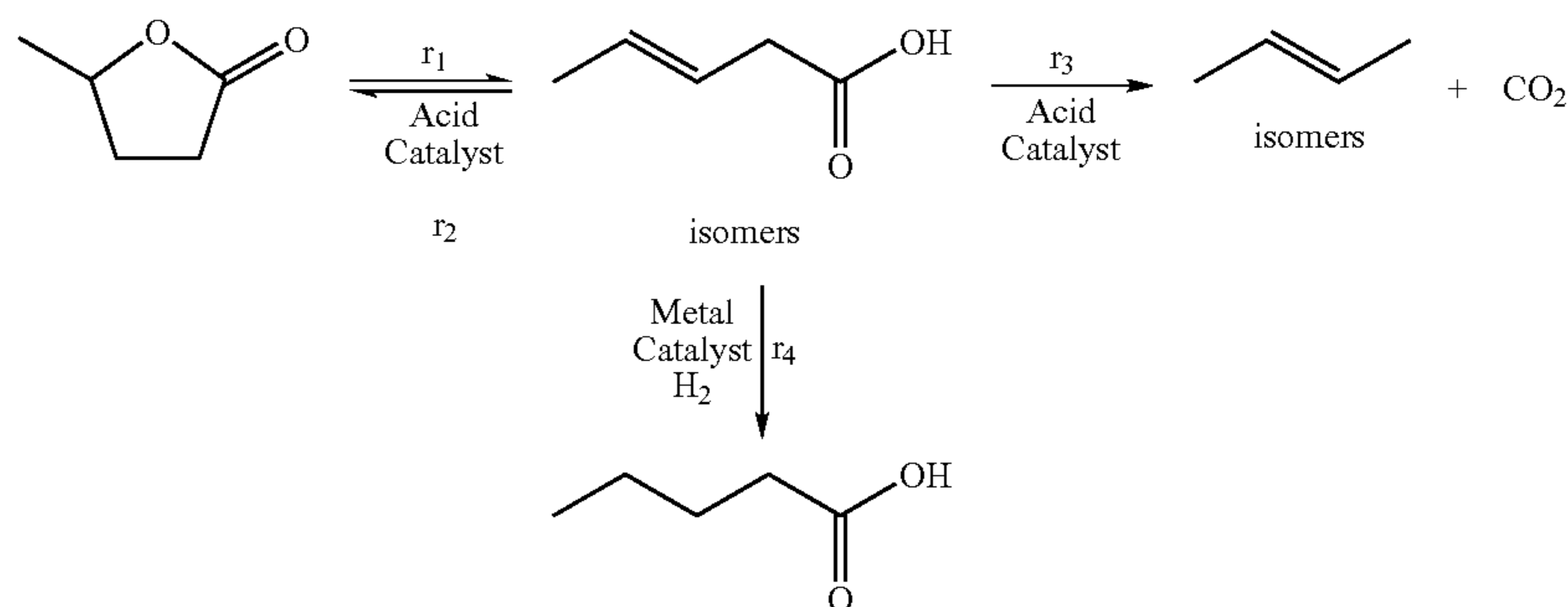
Scheme 3. Reactive pathway model
