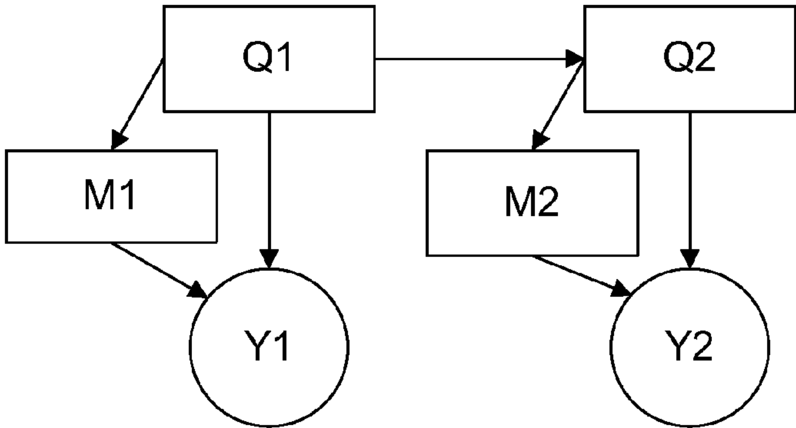
HMM with mixture of Gaussians output Fig. 3
