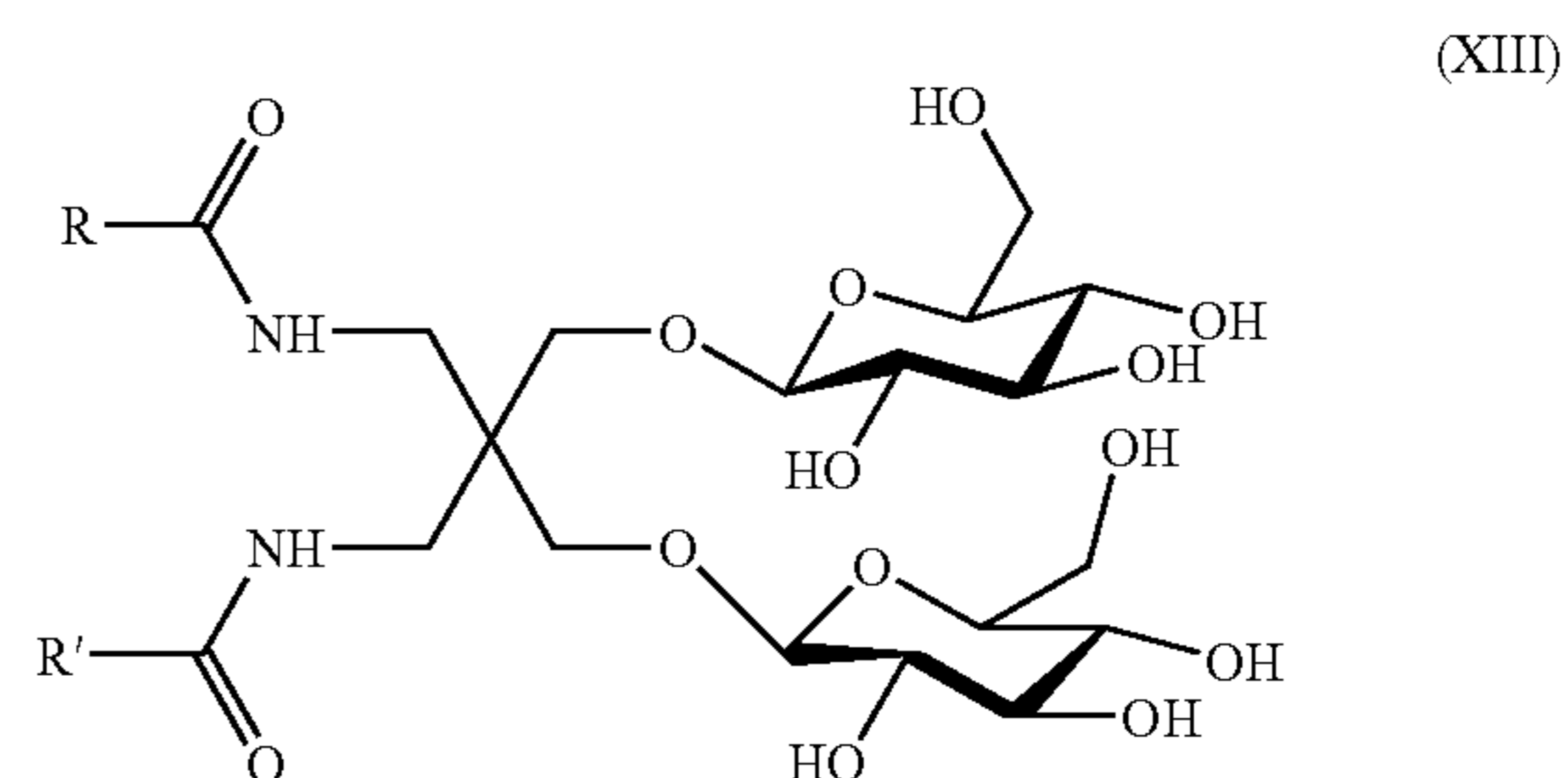
Scheme E. GNG Amphiphiles
