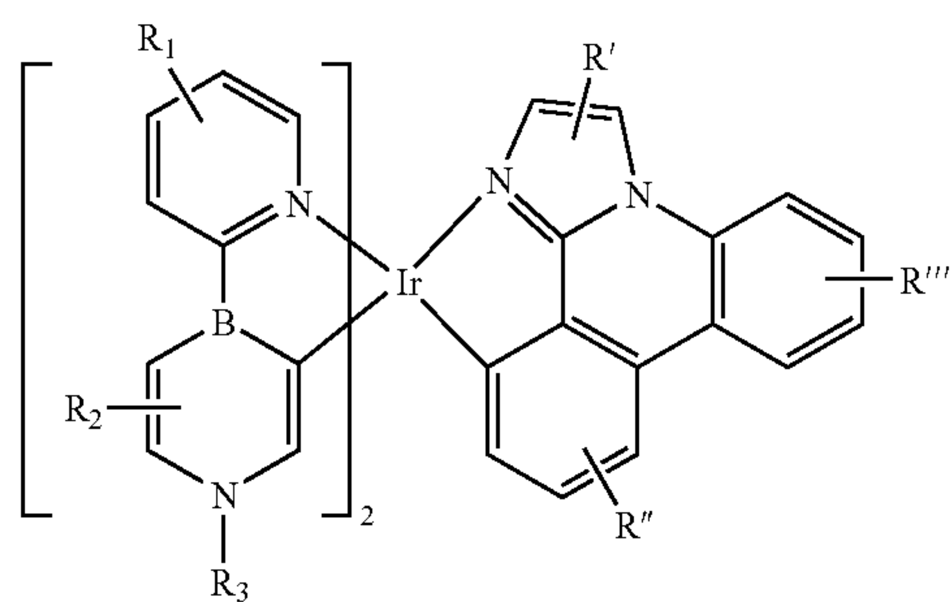
Compound 162G
