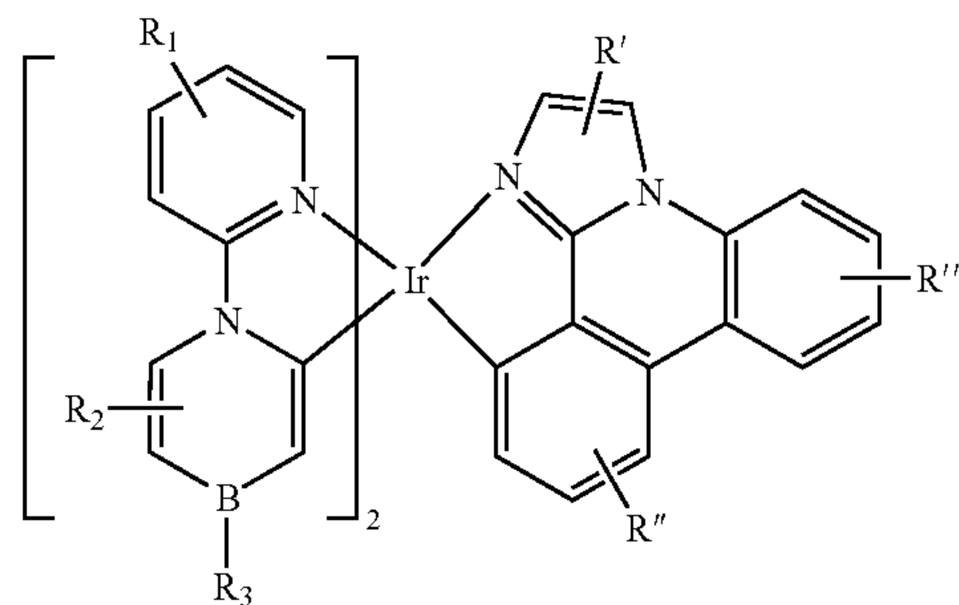
Compound 149G
