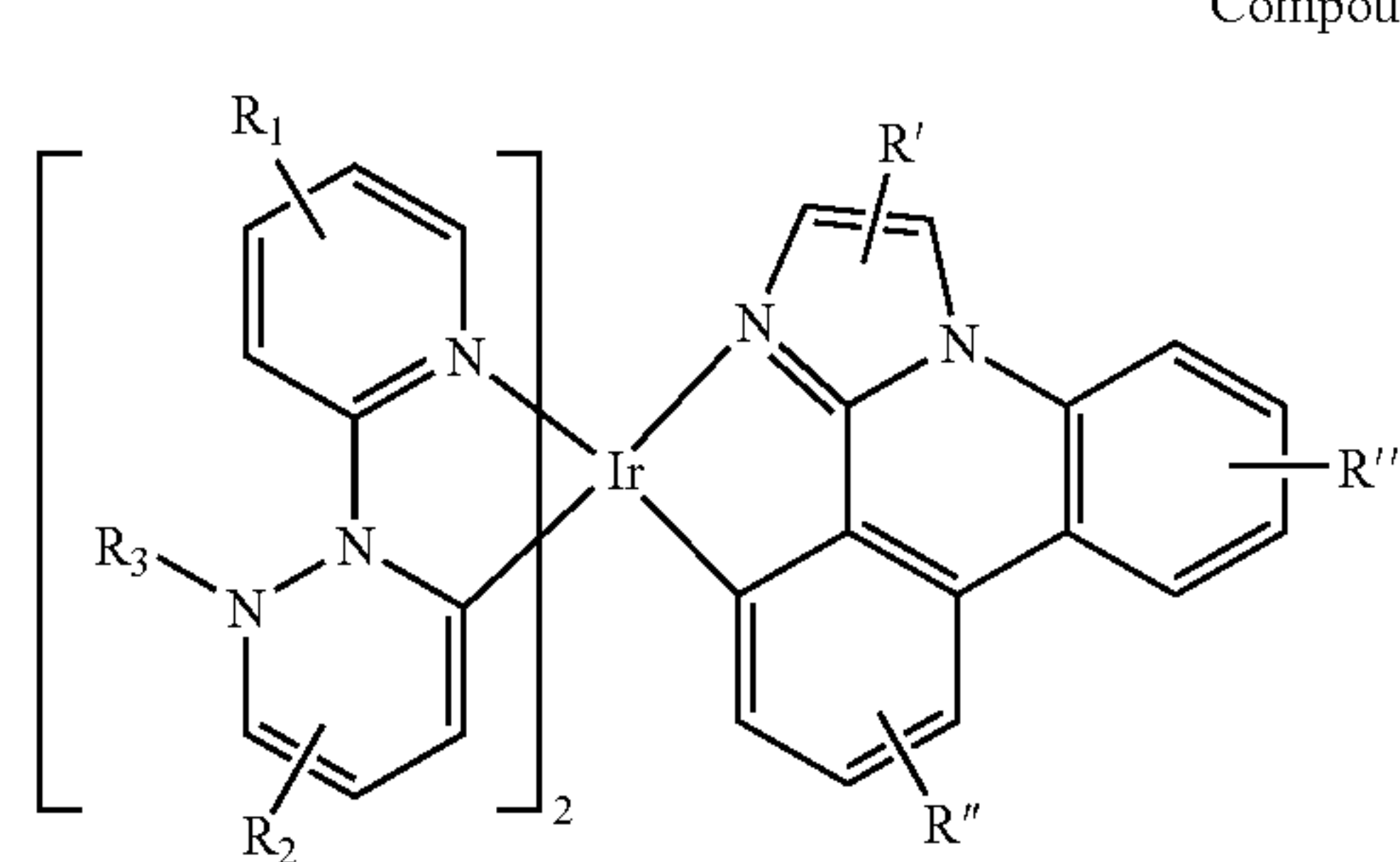
Compound 123G
