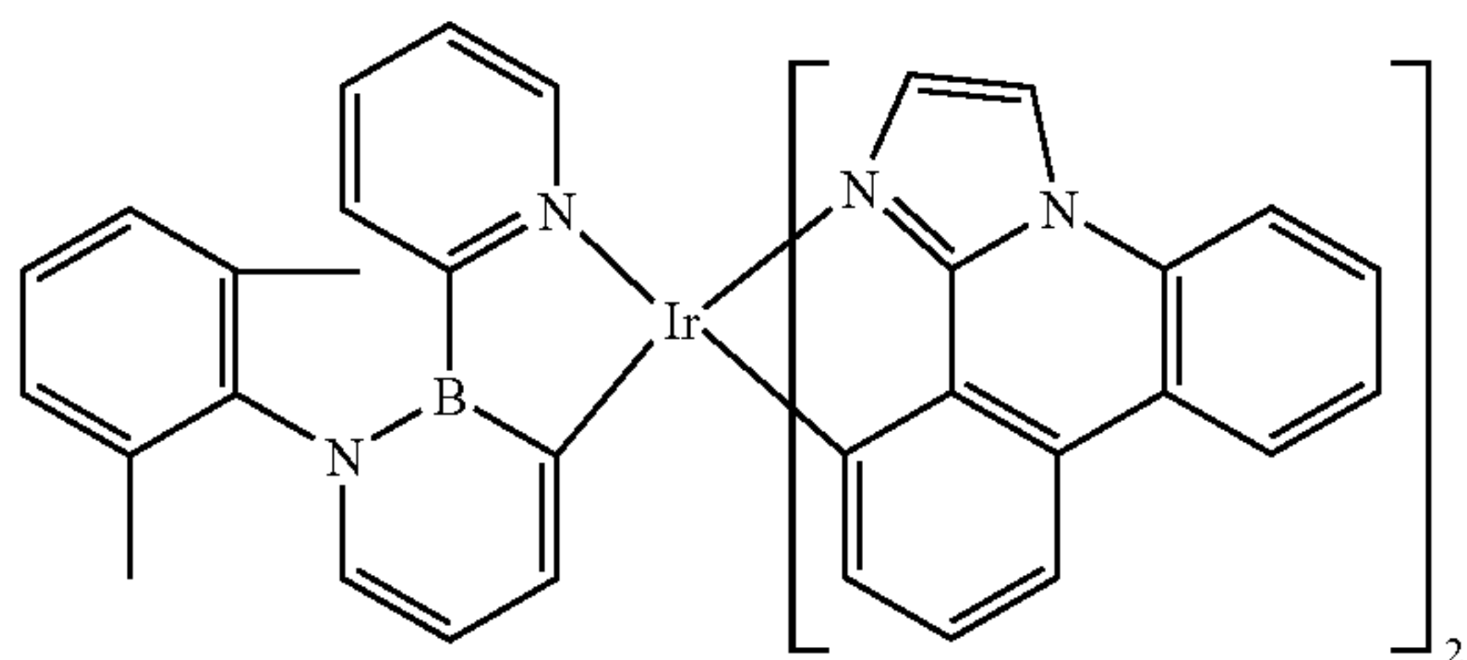
Compound 125
