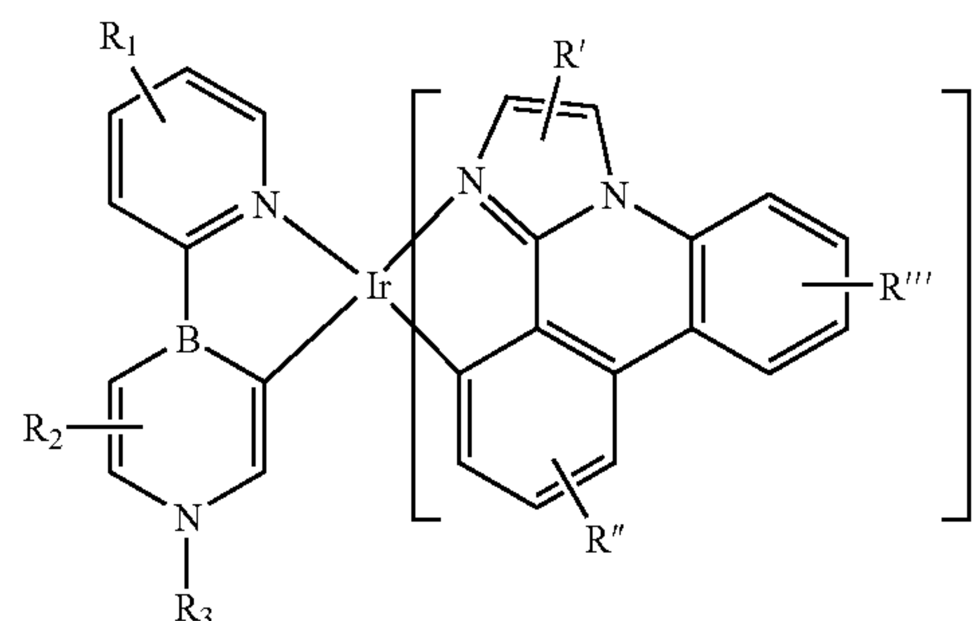
Compound 163G
