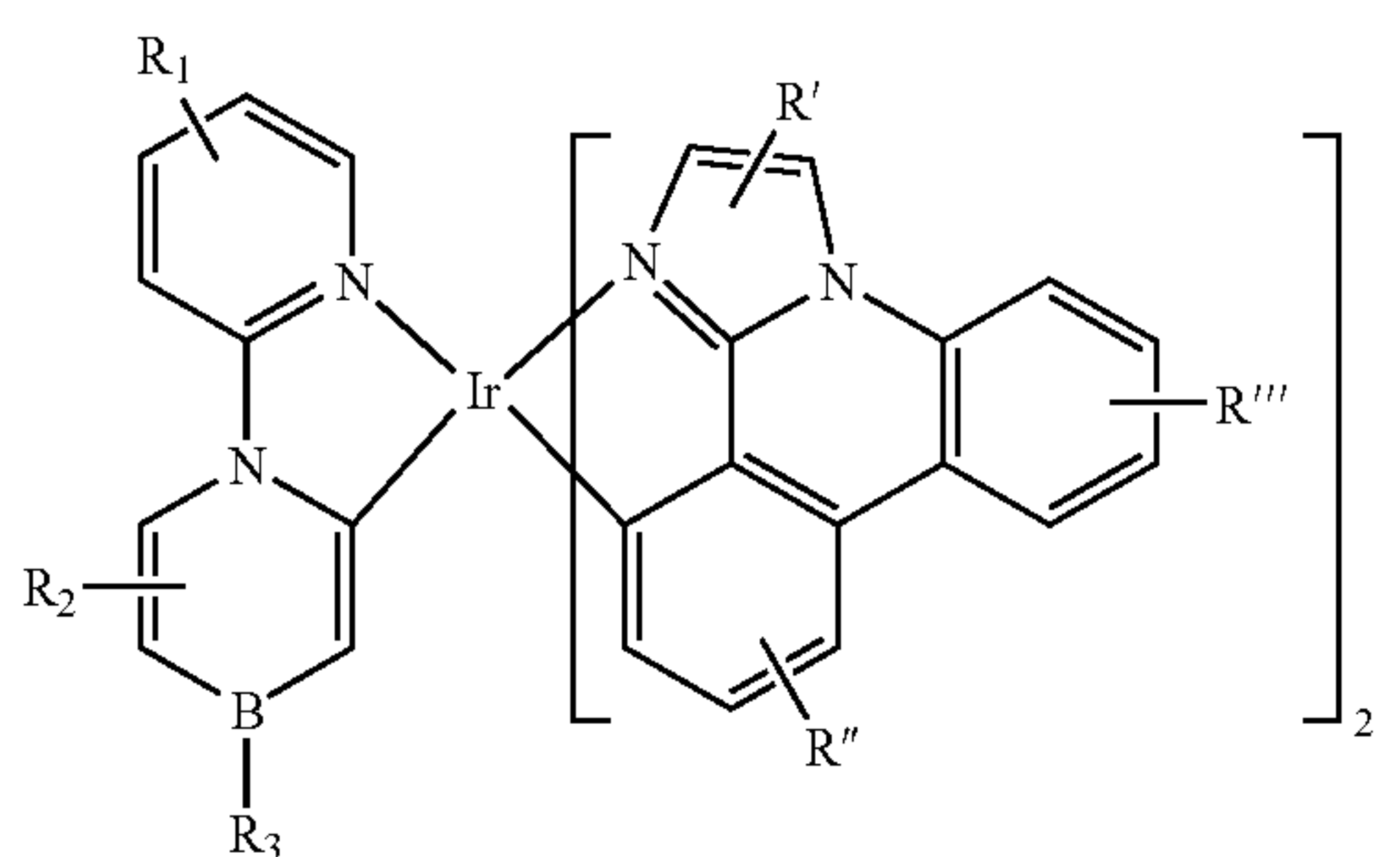
Compound 150G
