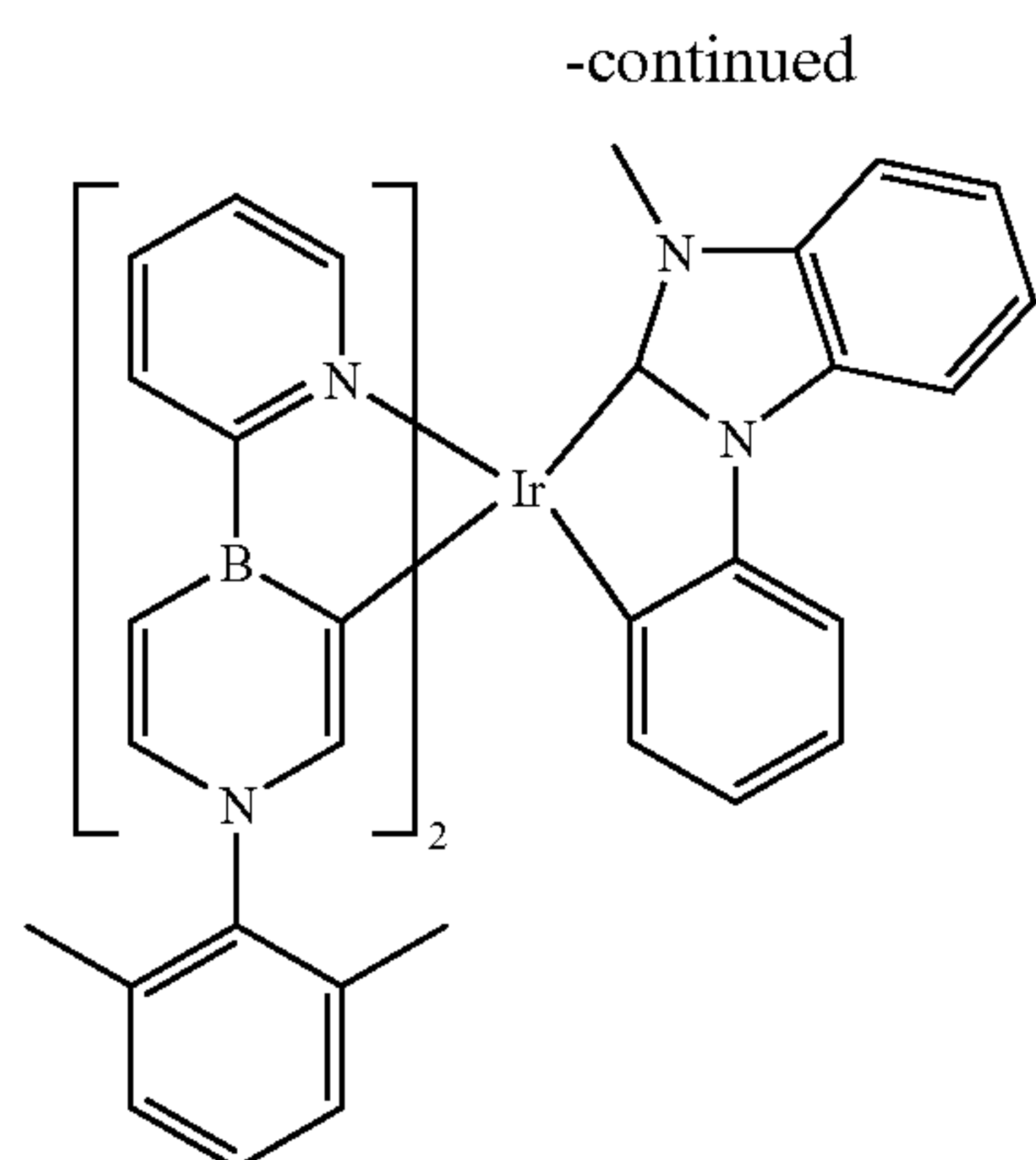
Compound 166
