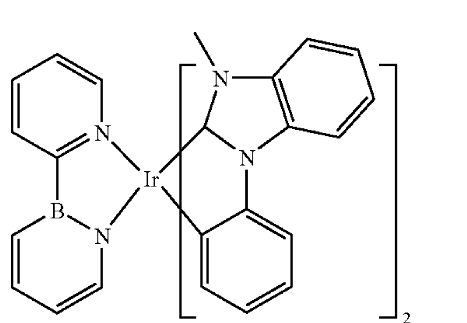
Compound 141
