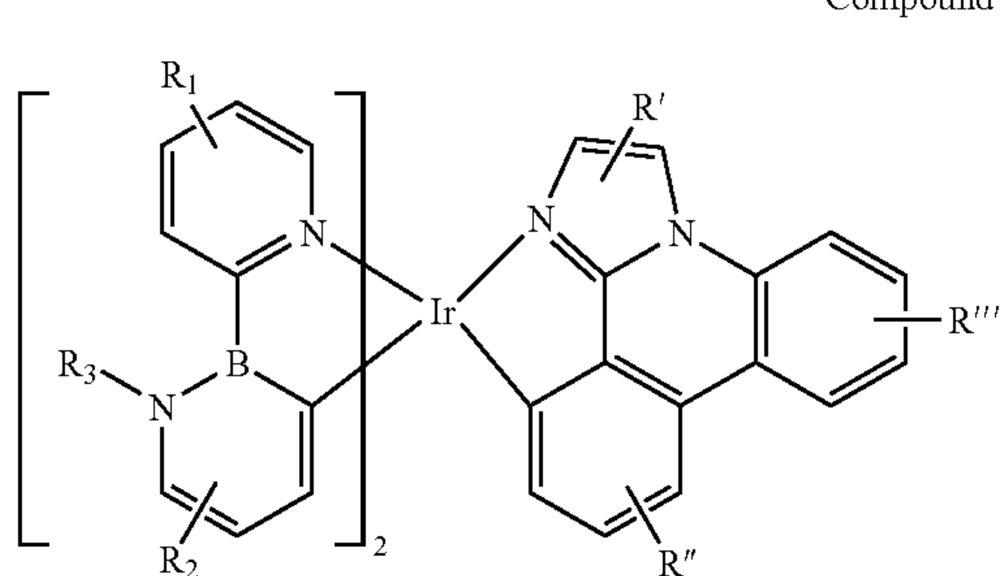
Compound 123G
