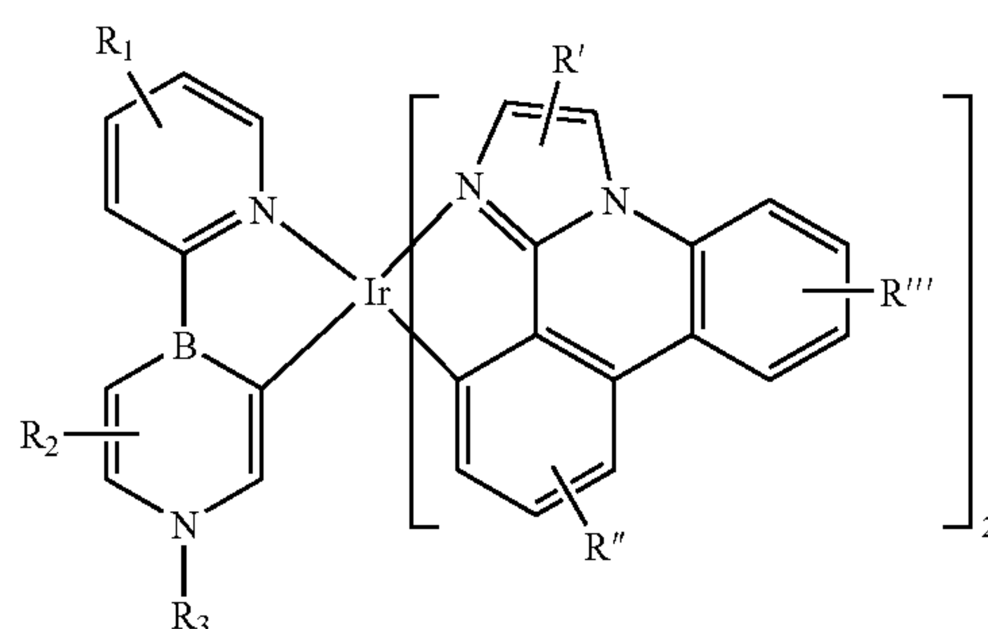
Compound 163G
