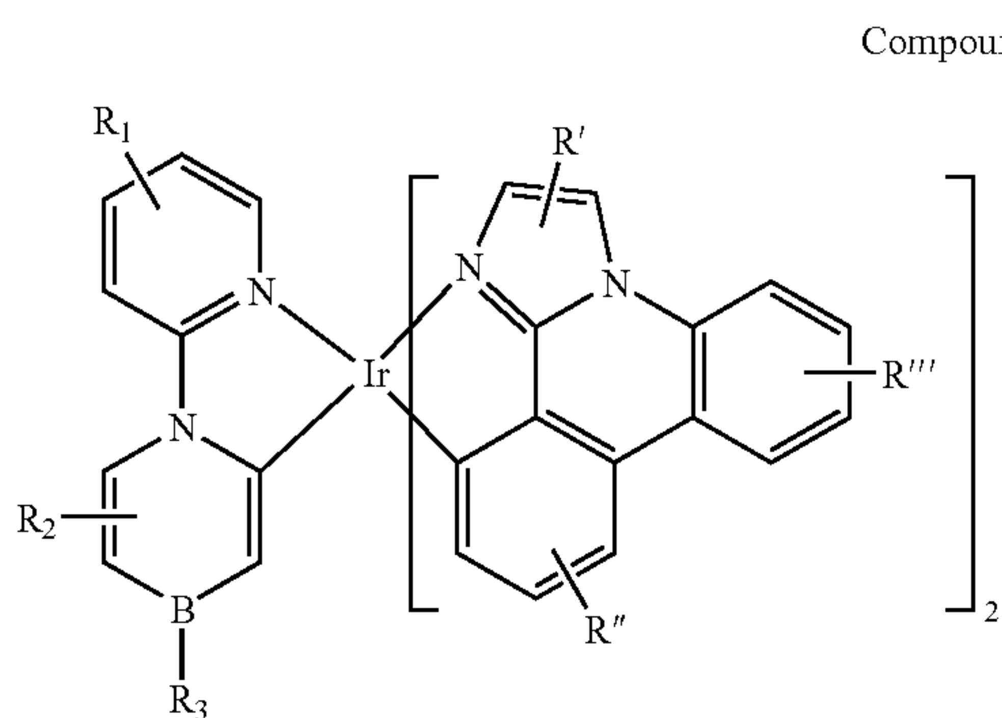
Compound 151G
