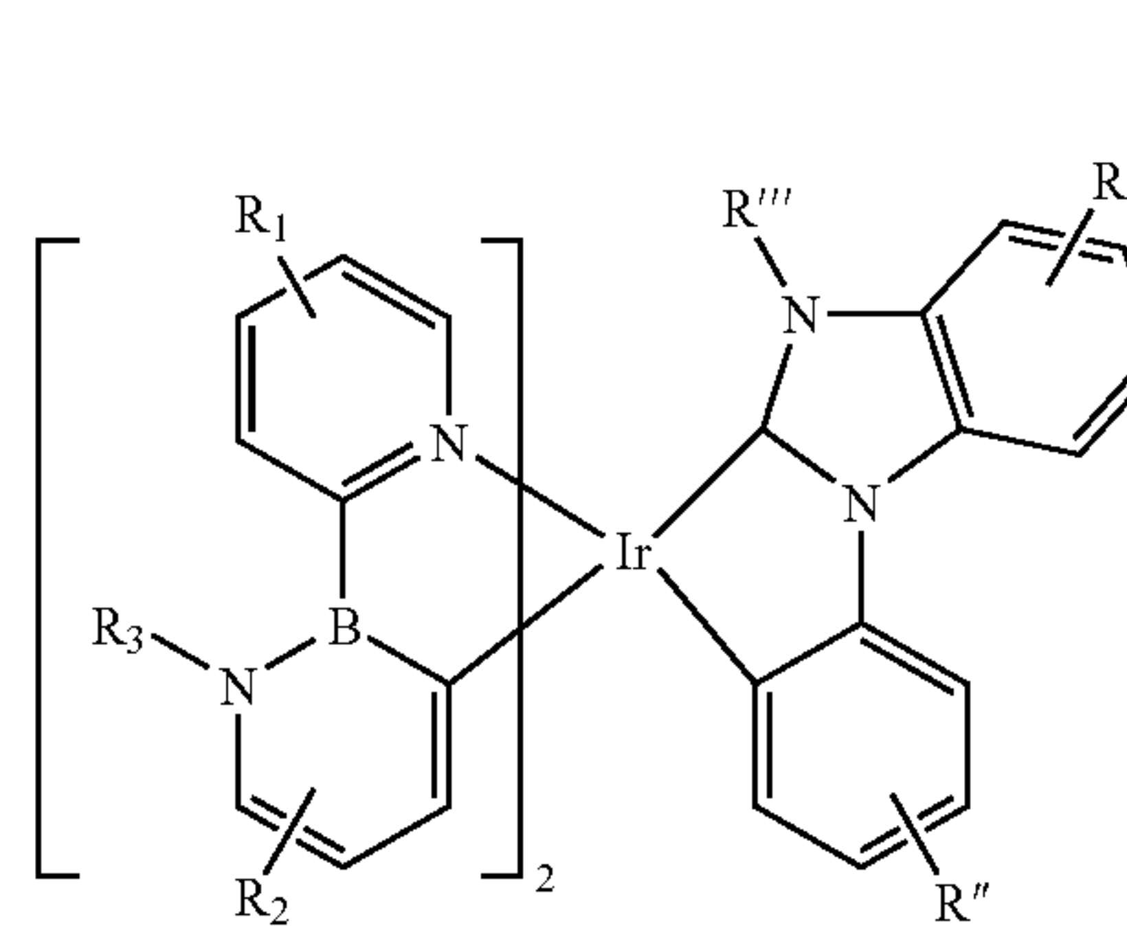
Compound 127G
