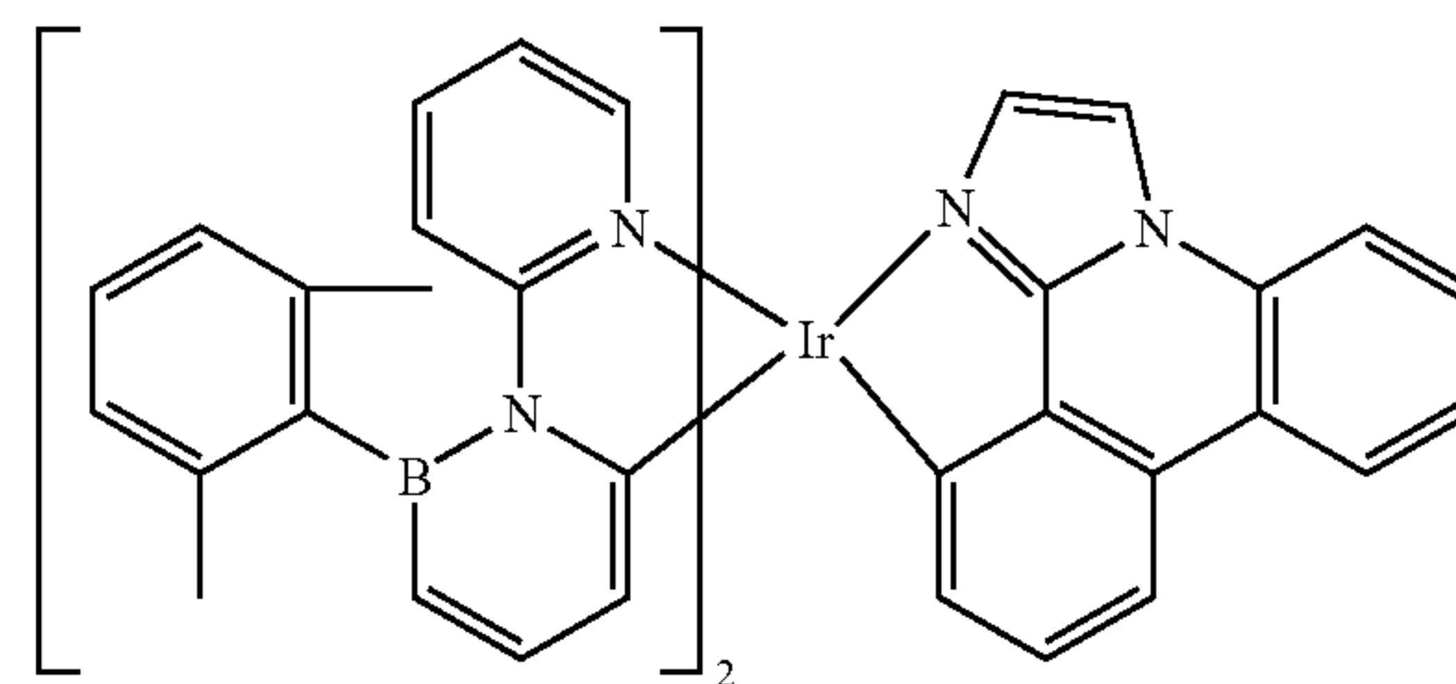
Compound 97
