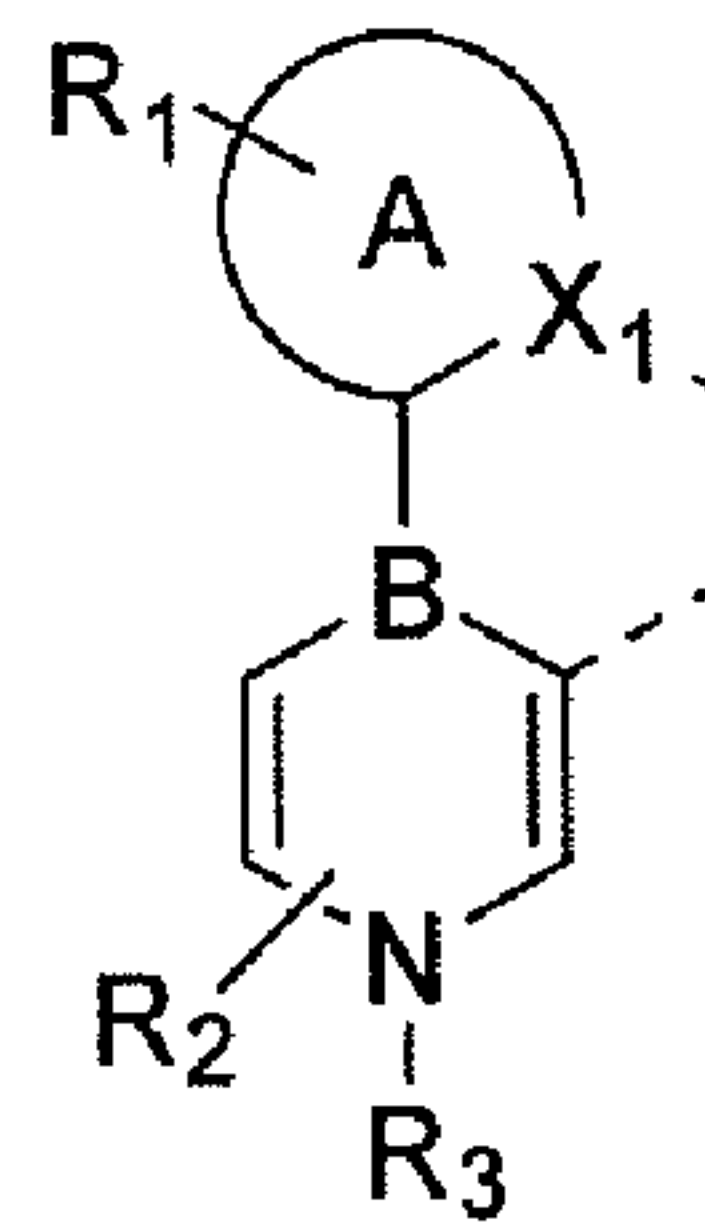
Compound 28
