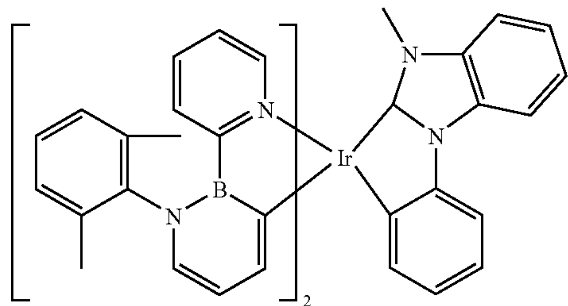
Compound 128
