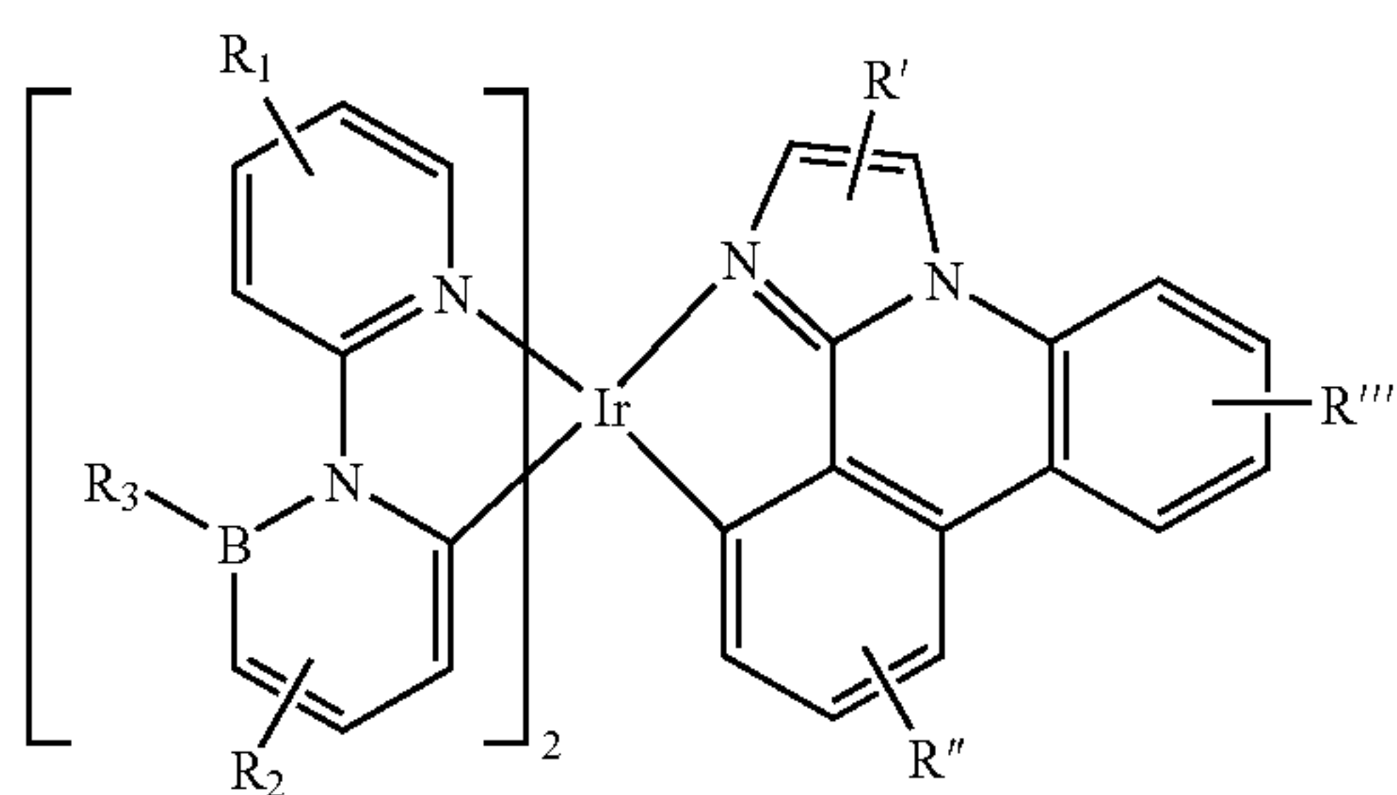
Compound 98G
