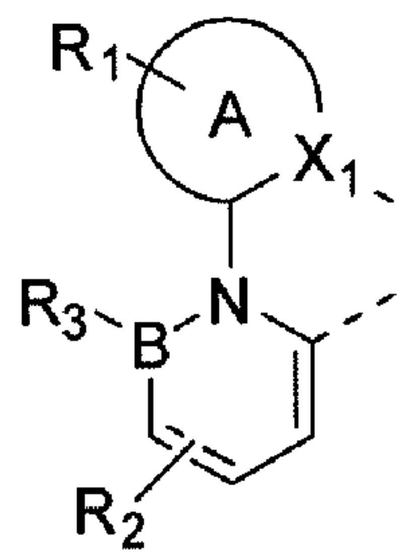
Compound 12
