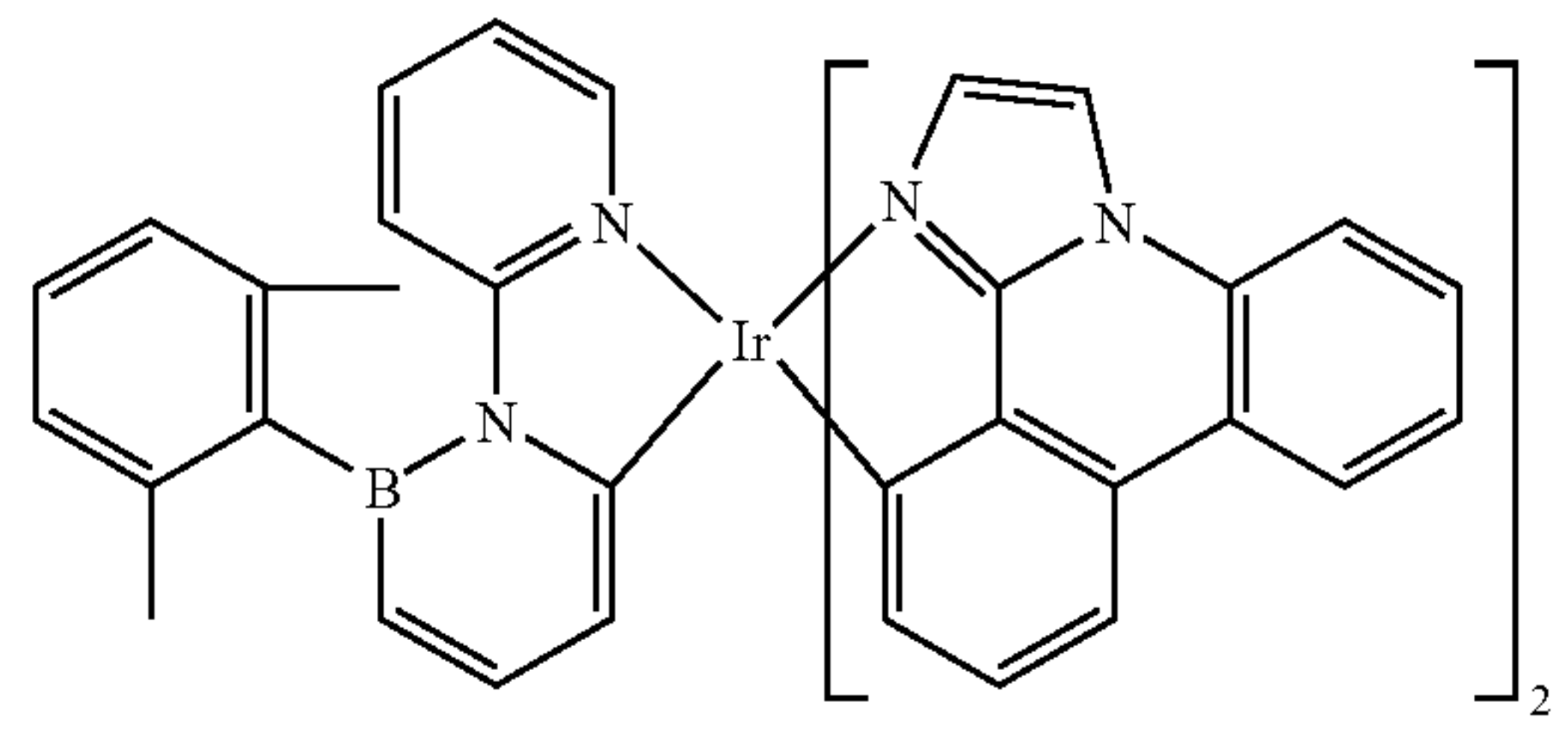
Compound 98
