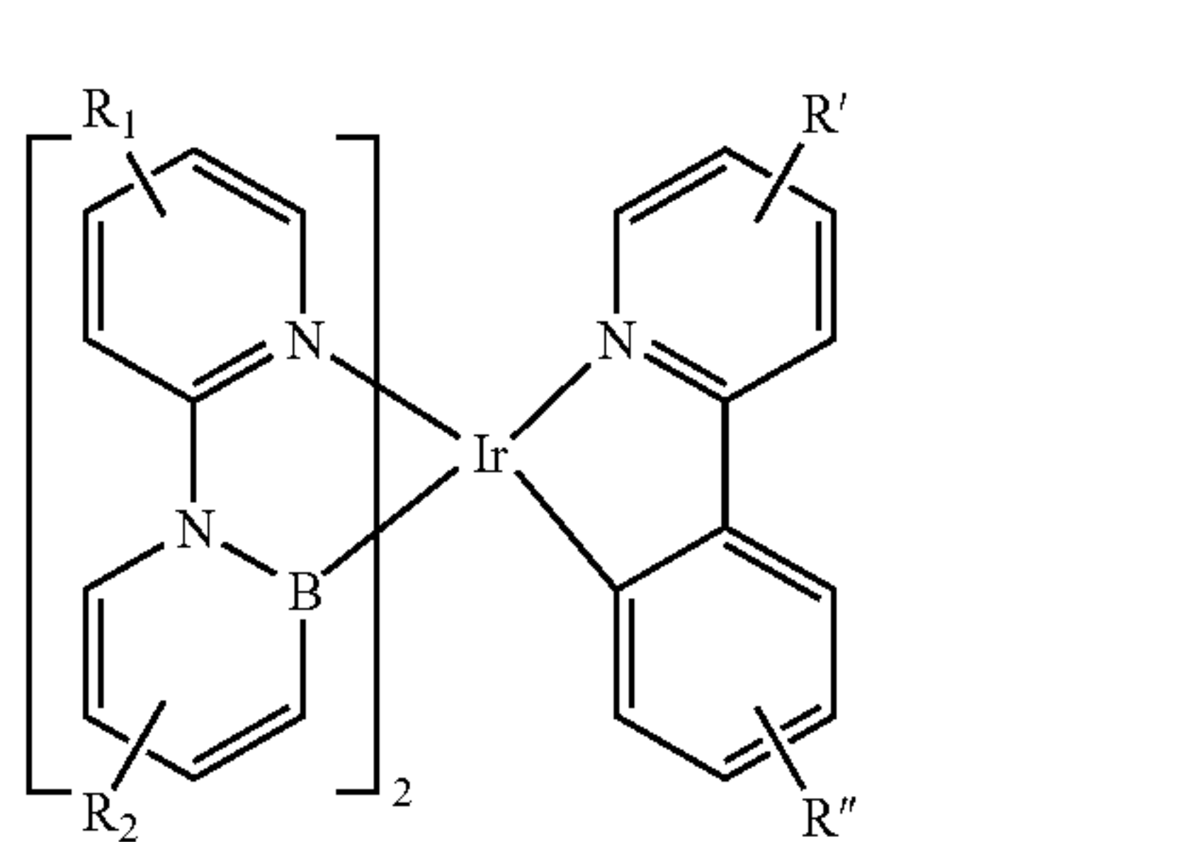
Compound 103G
