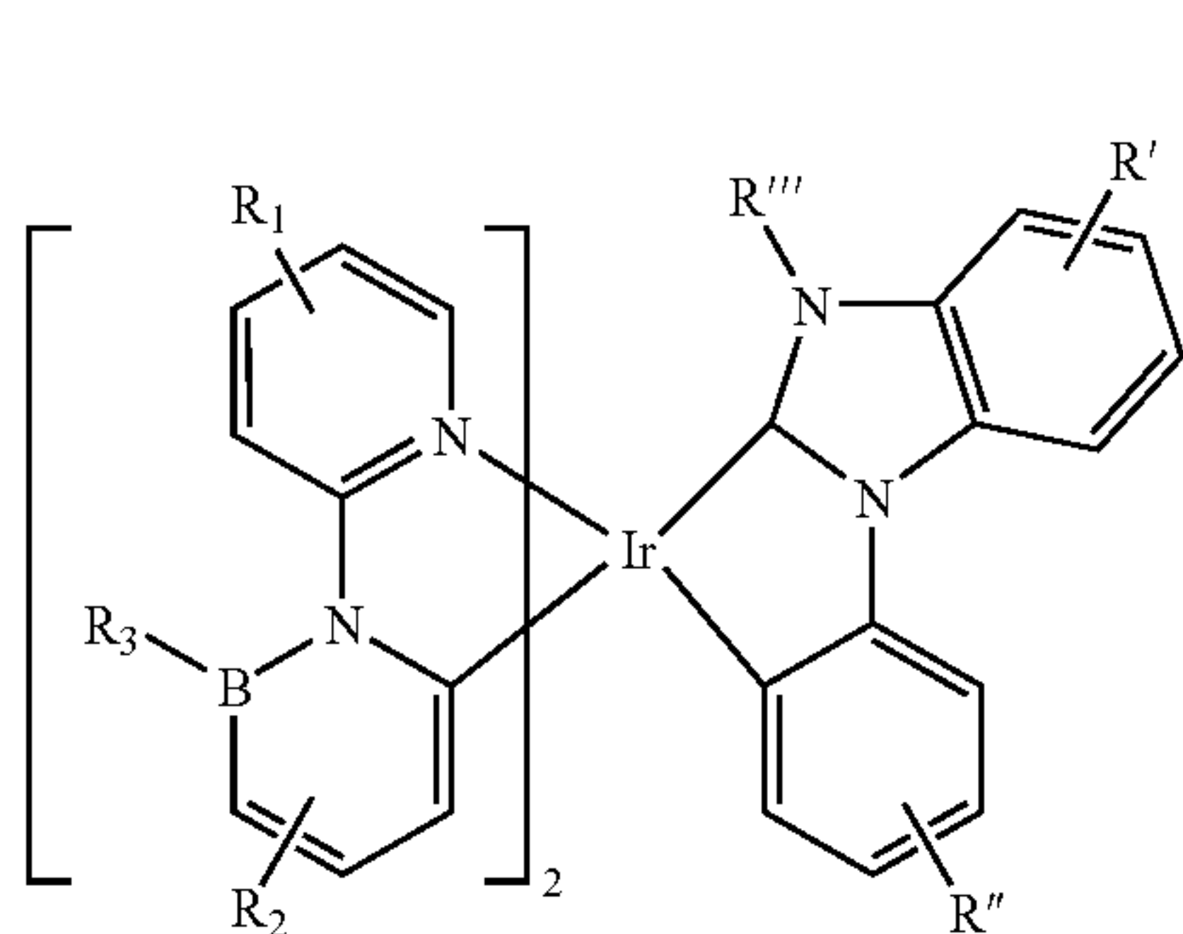
Compound 101G
