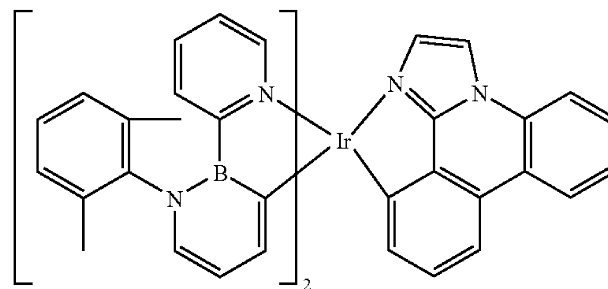
Compound 123
