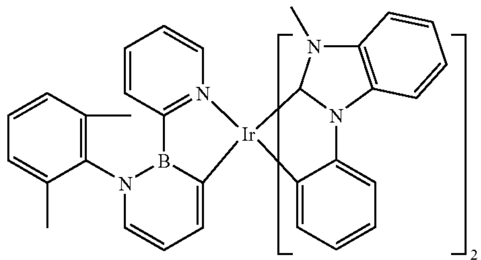
Compound 129
