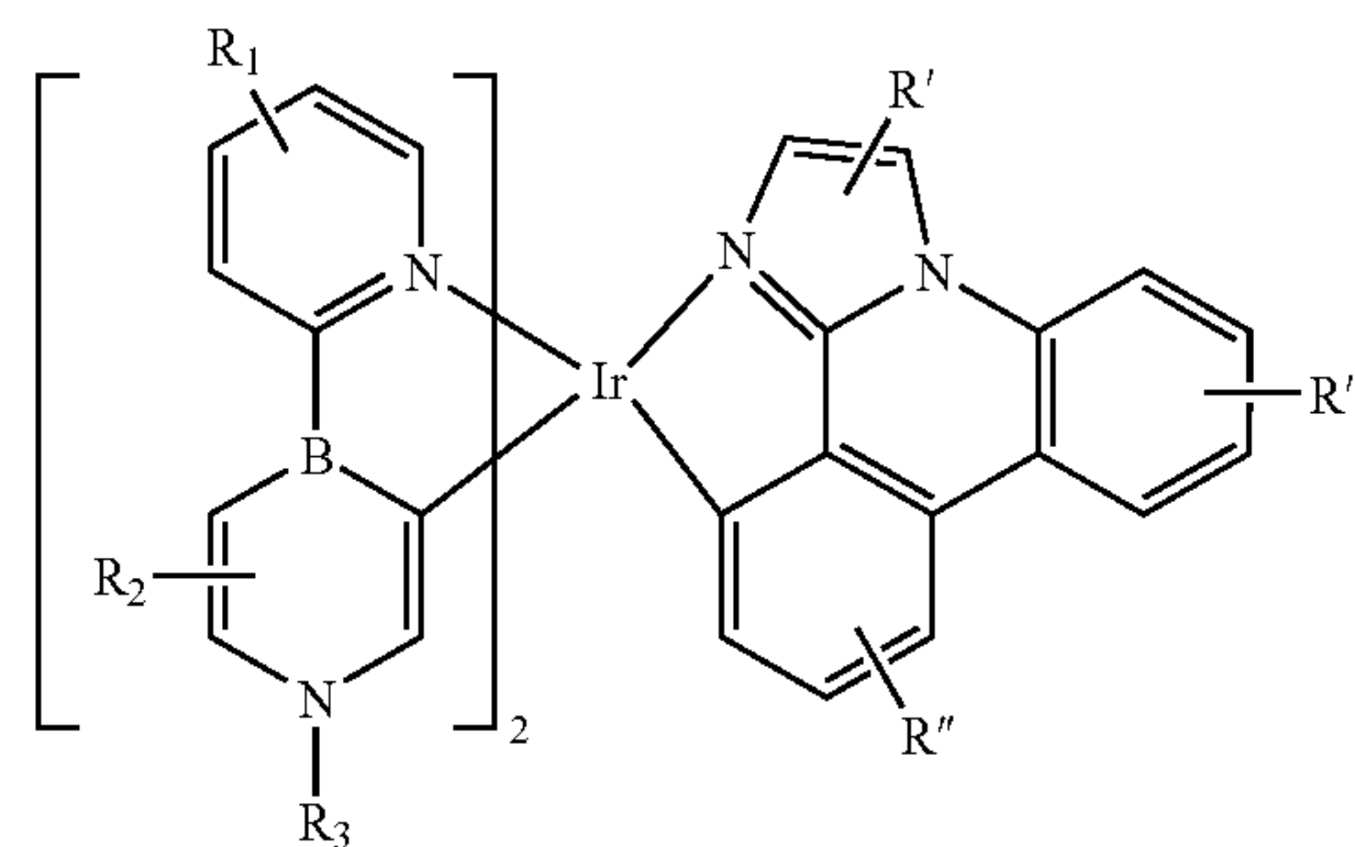
Compound 162
