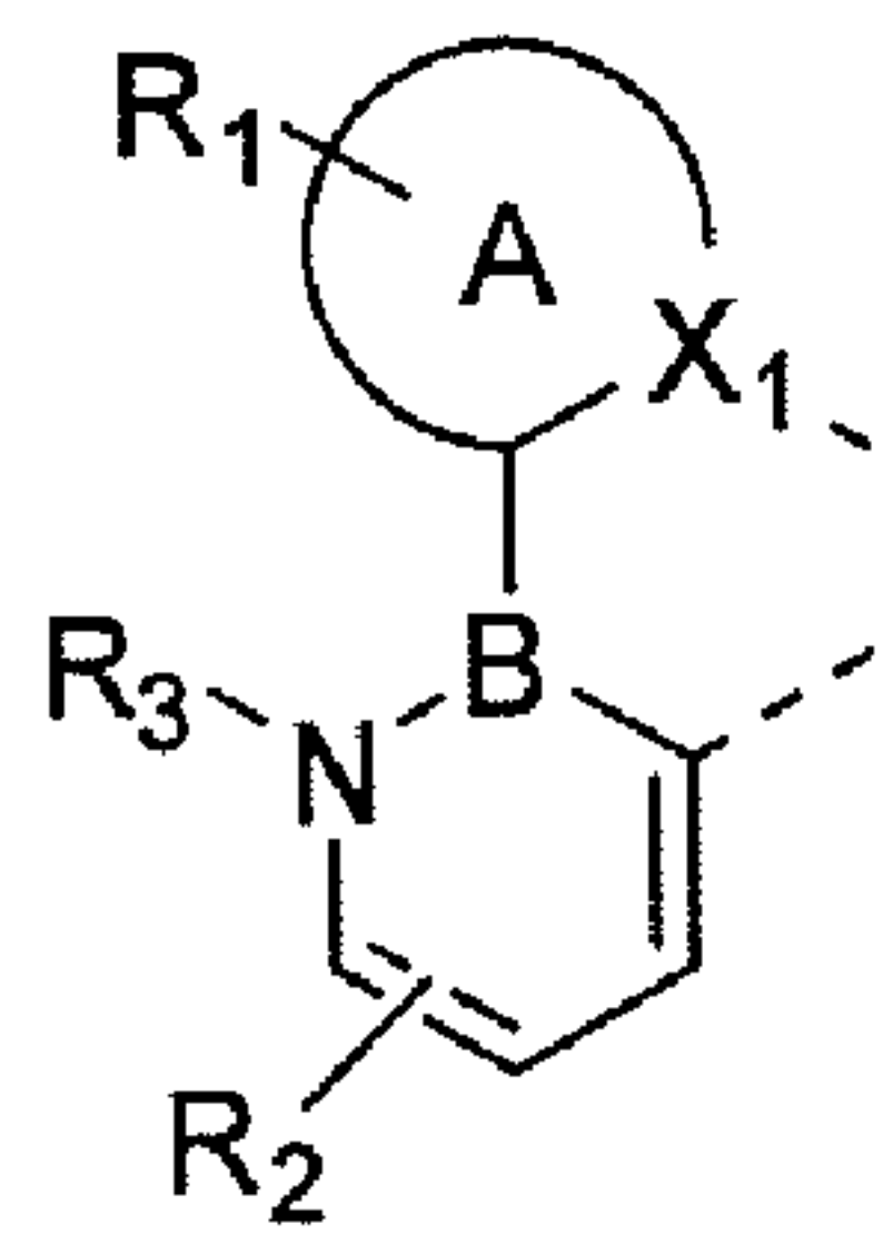
Compound 6
