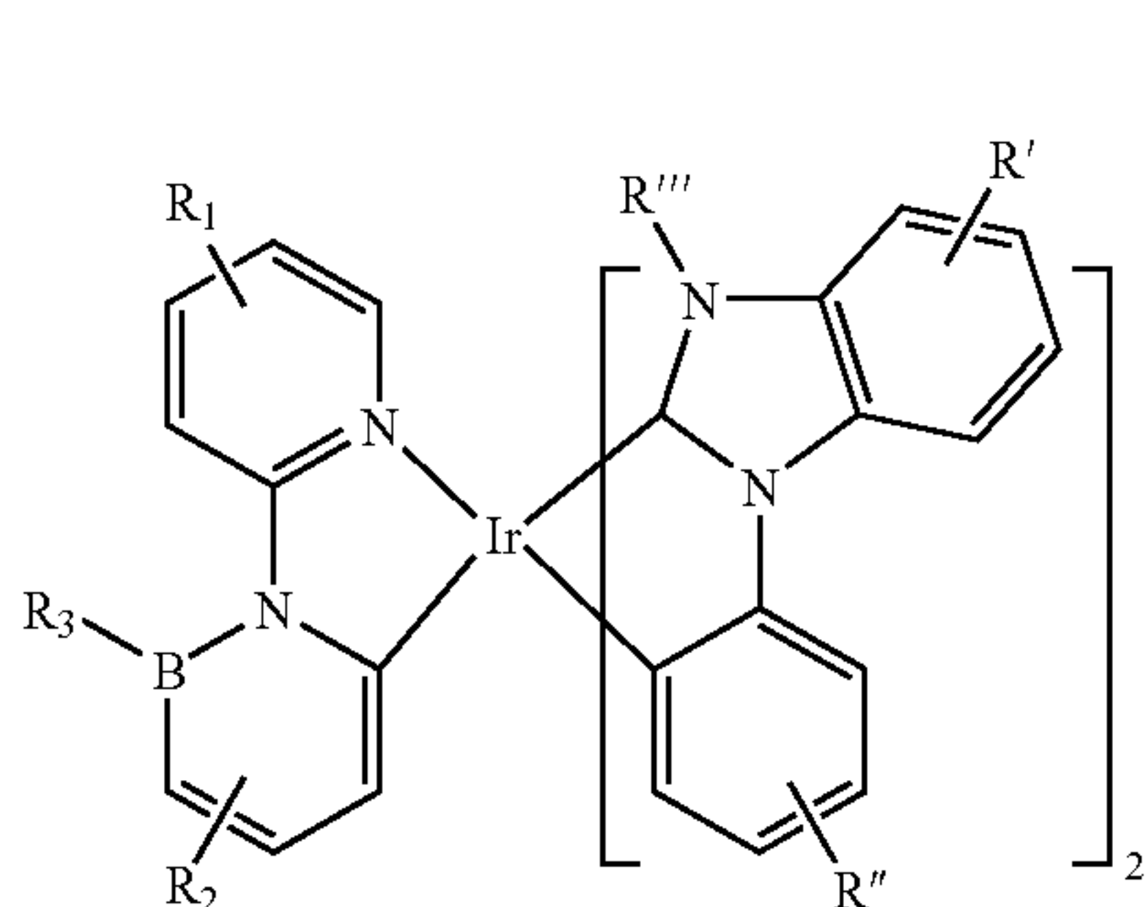
Compound 102G
