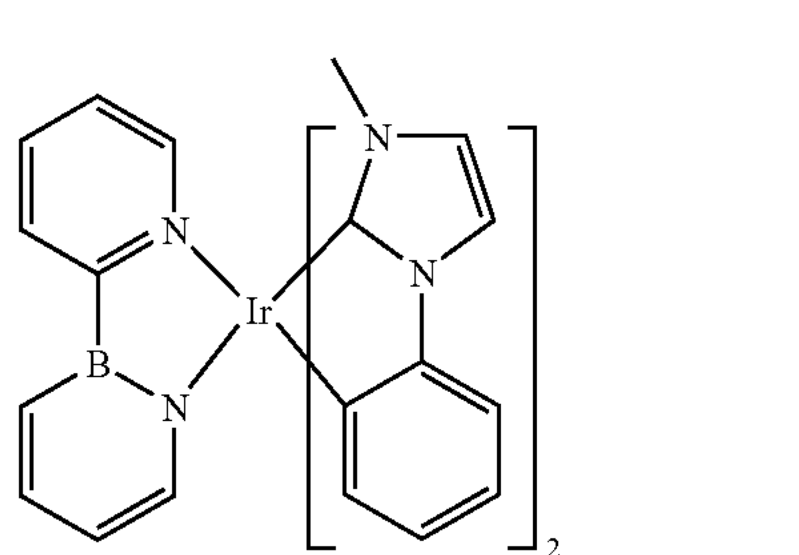
Compound 139
