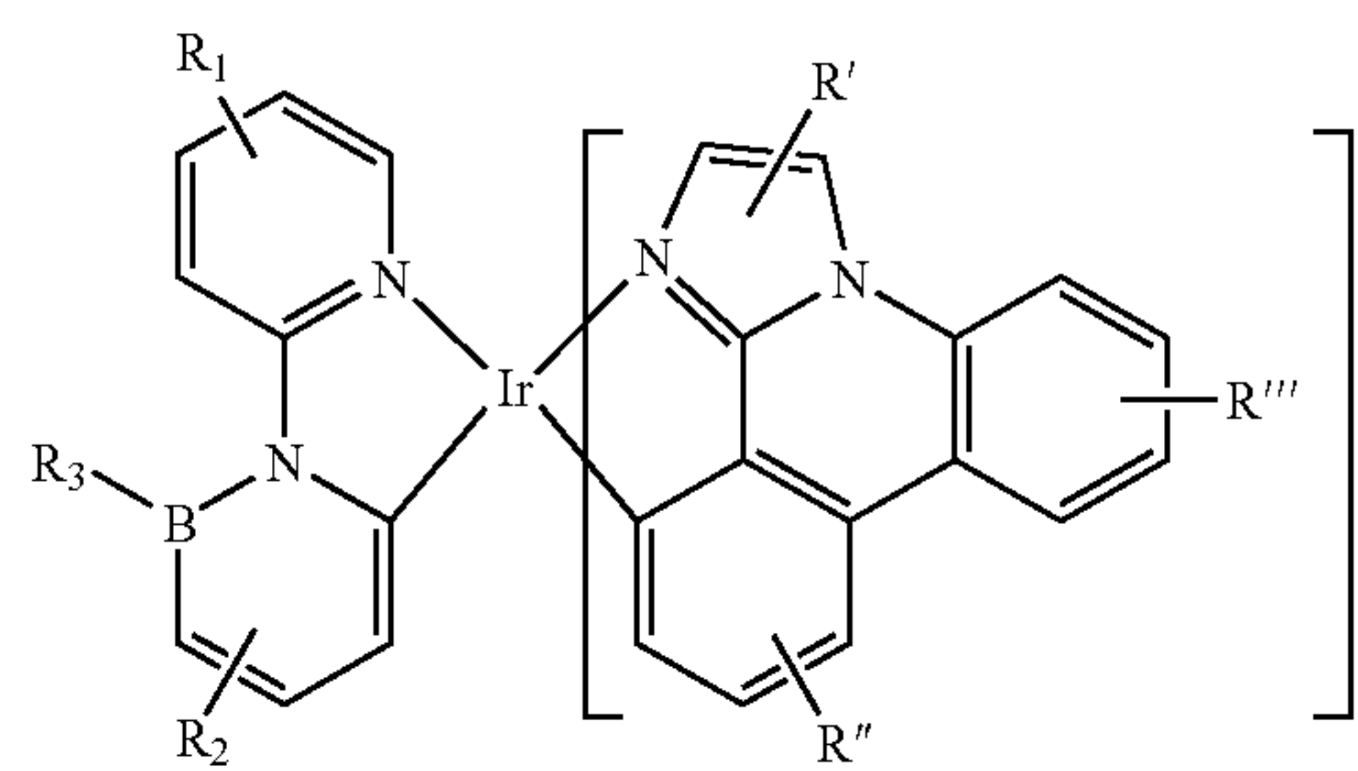
Compound 98G
