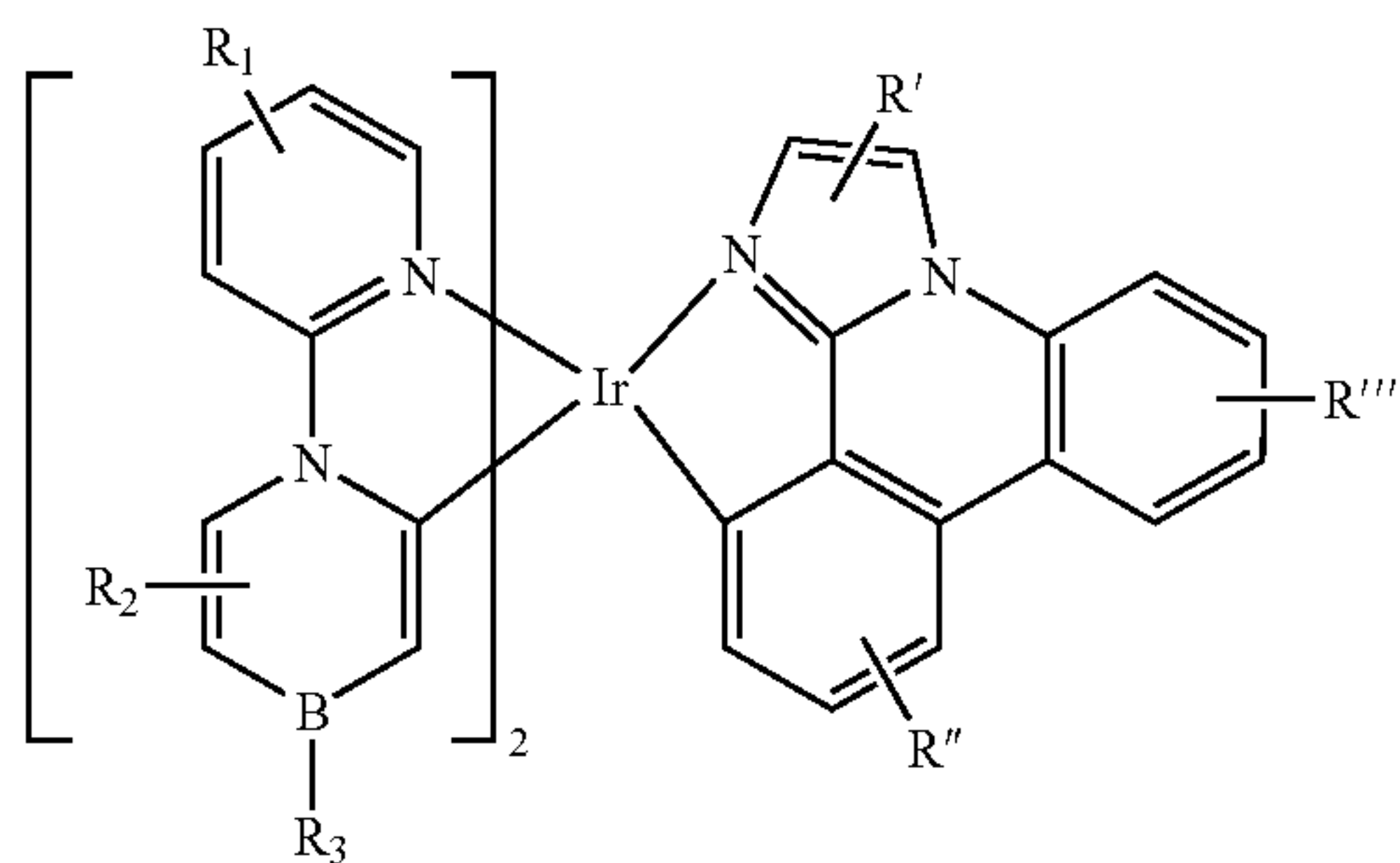
Compound 149G
