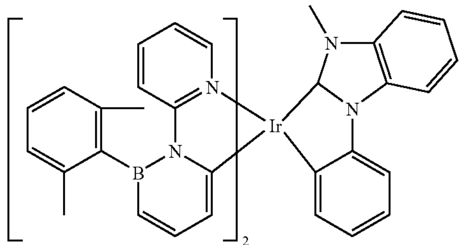
Compound 102
