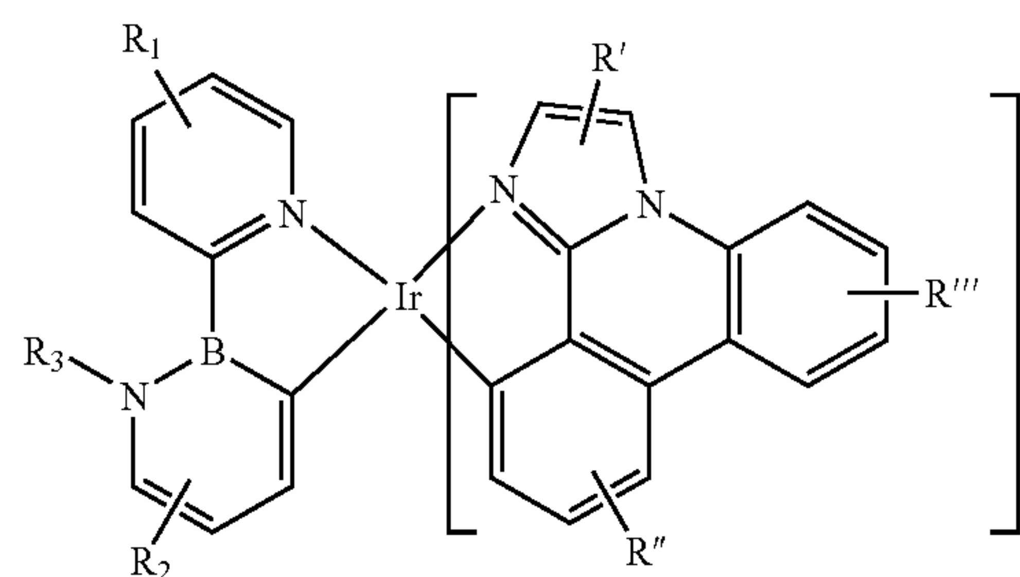
Compound 124G
