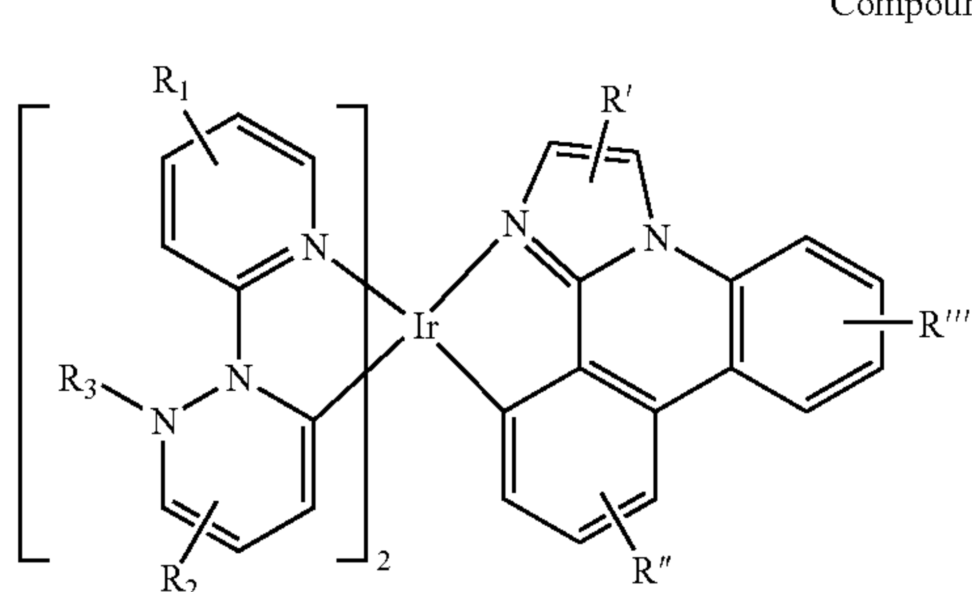
Compound 123G
