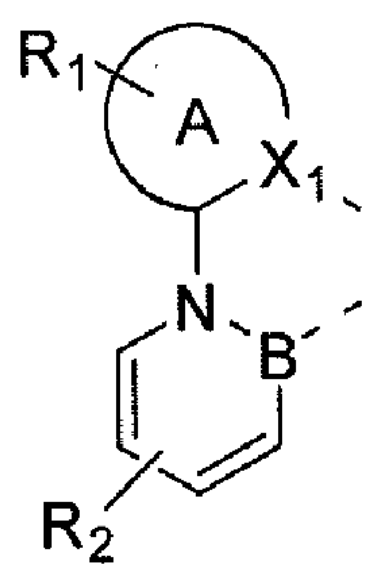
Compound 1
