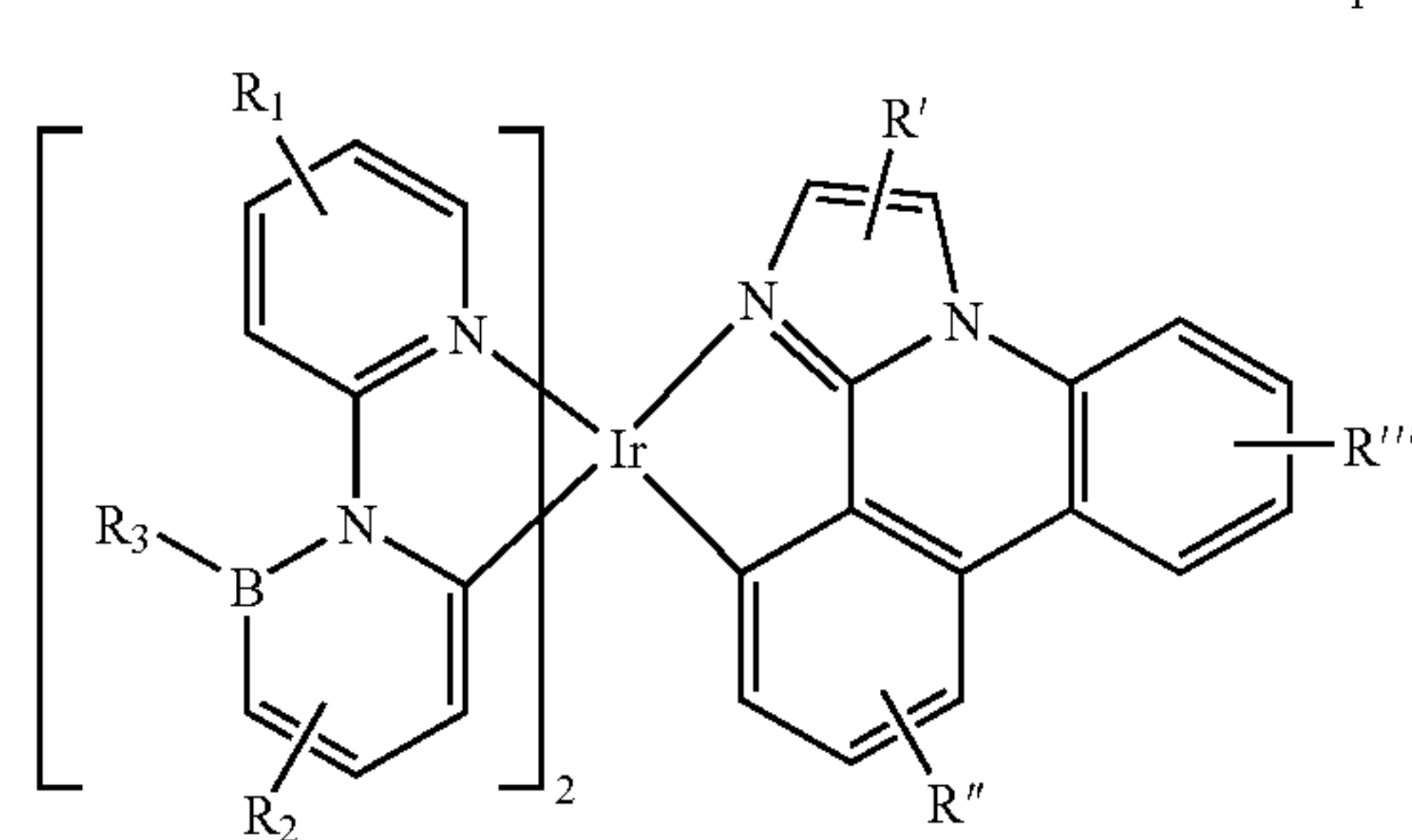
Compound 98G
