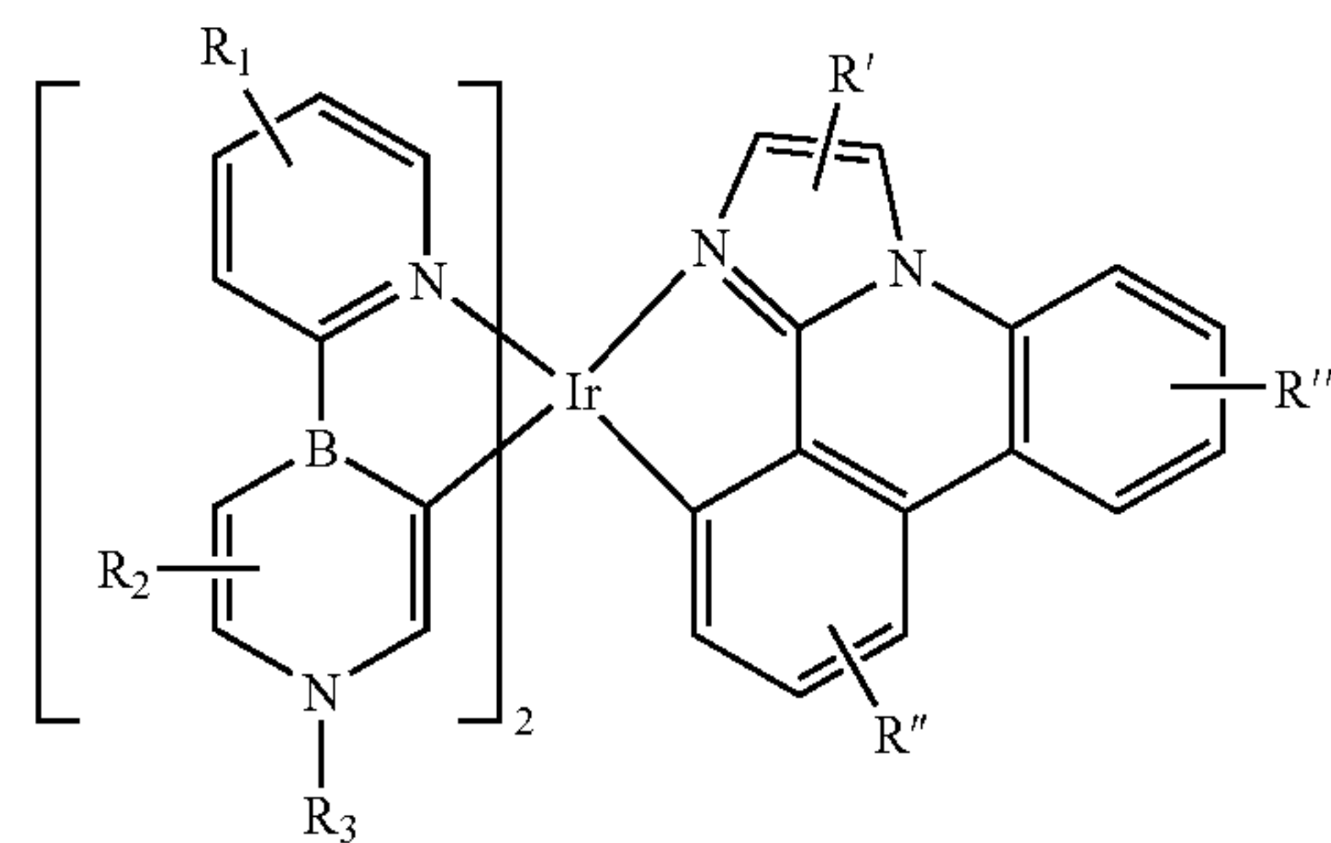
Compound 162G
