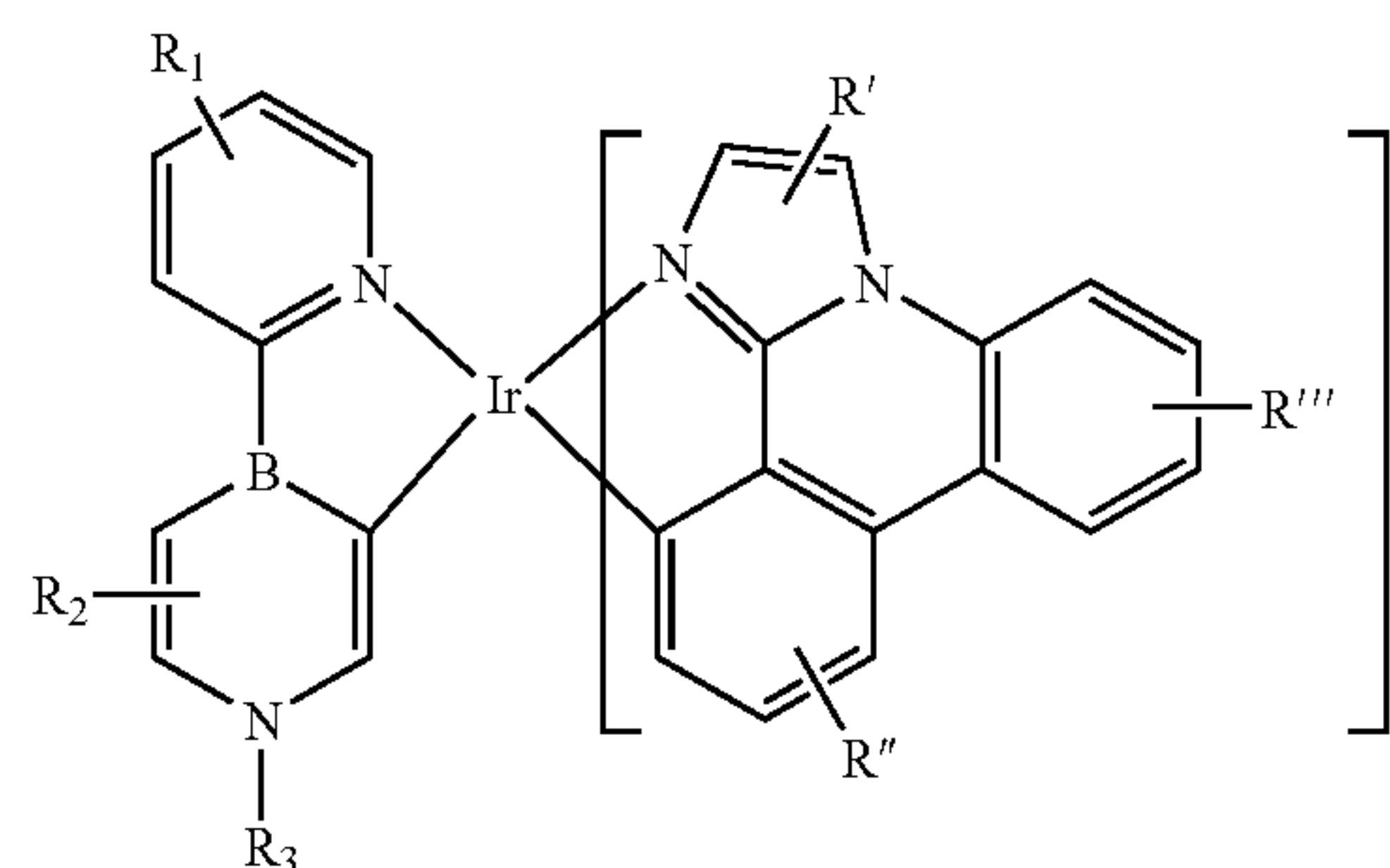
Compound 163
