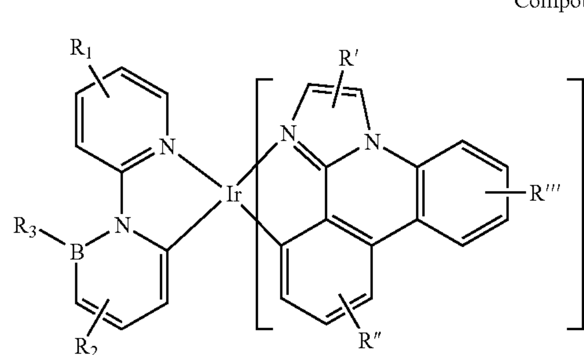
Compound 98G
