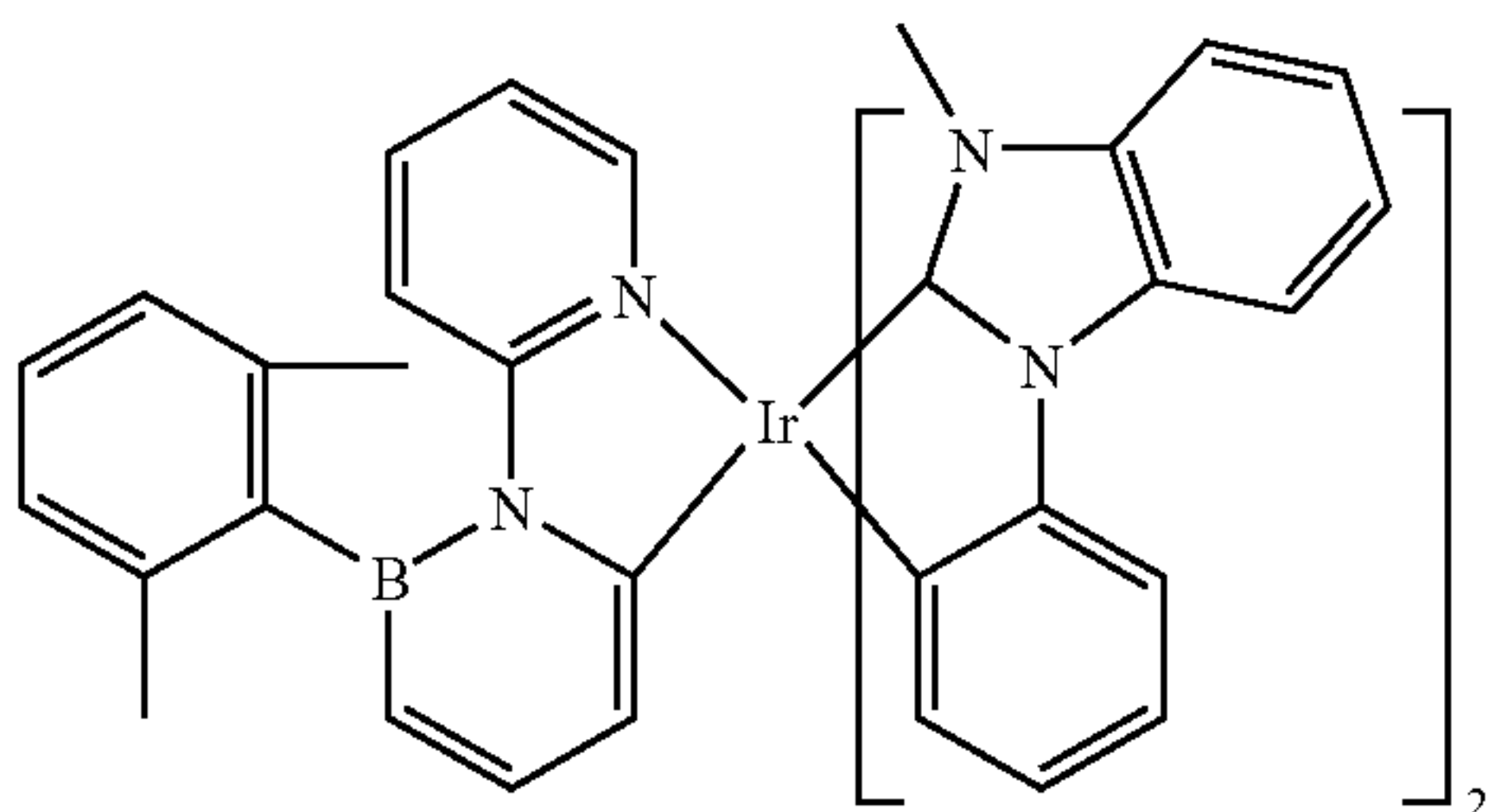
Compound 103
