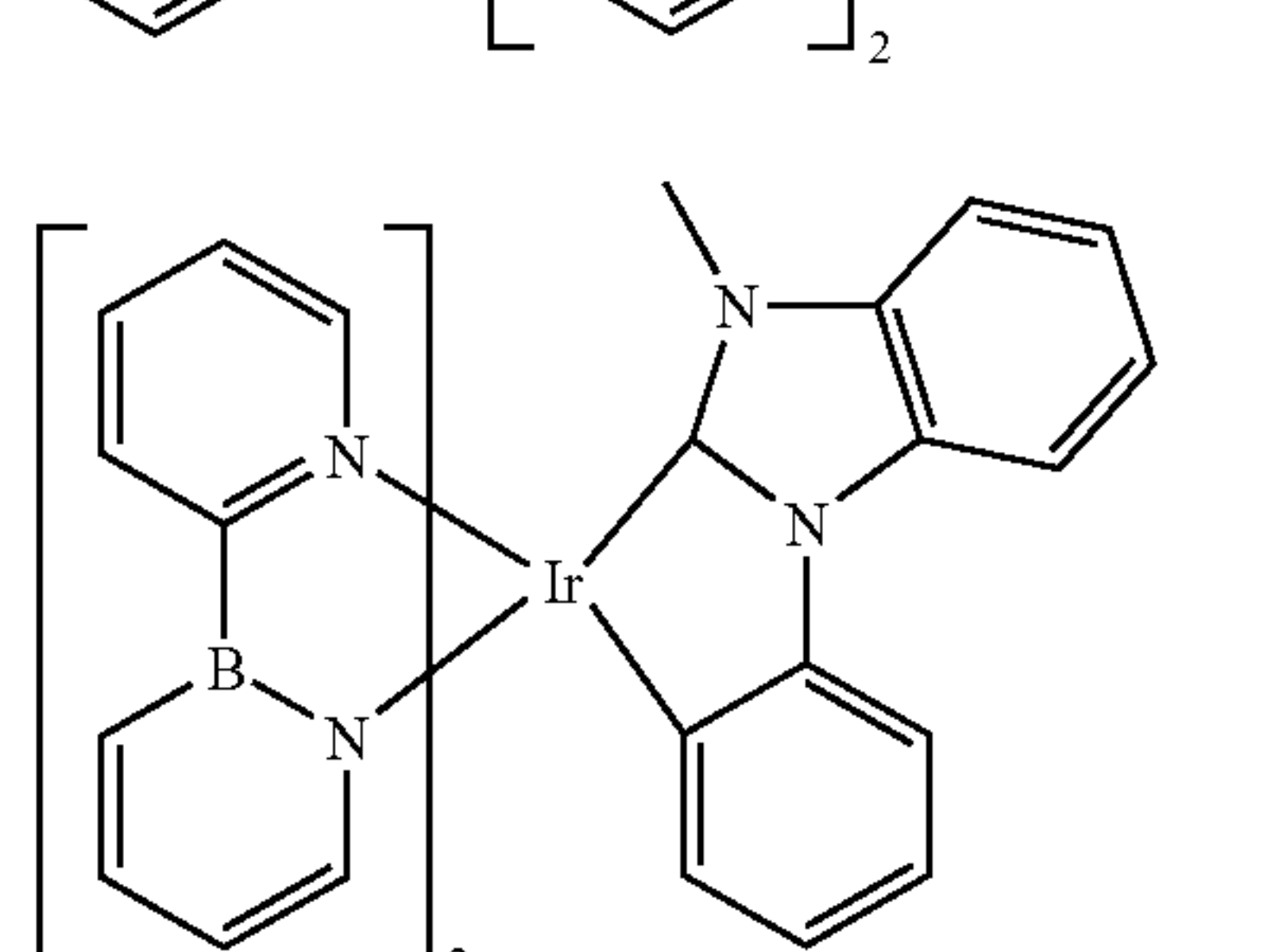
Compound 140
