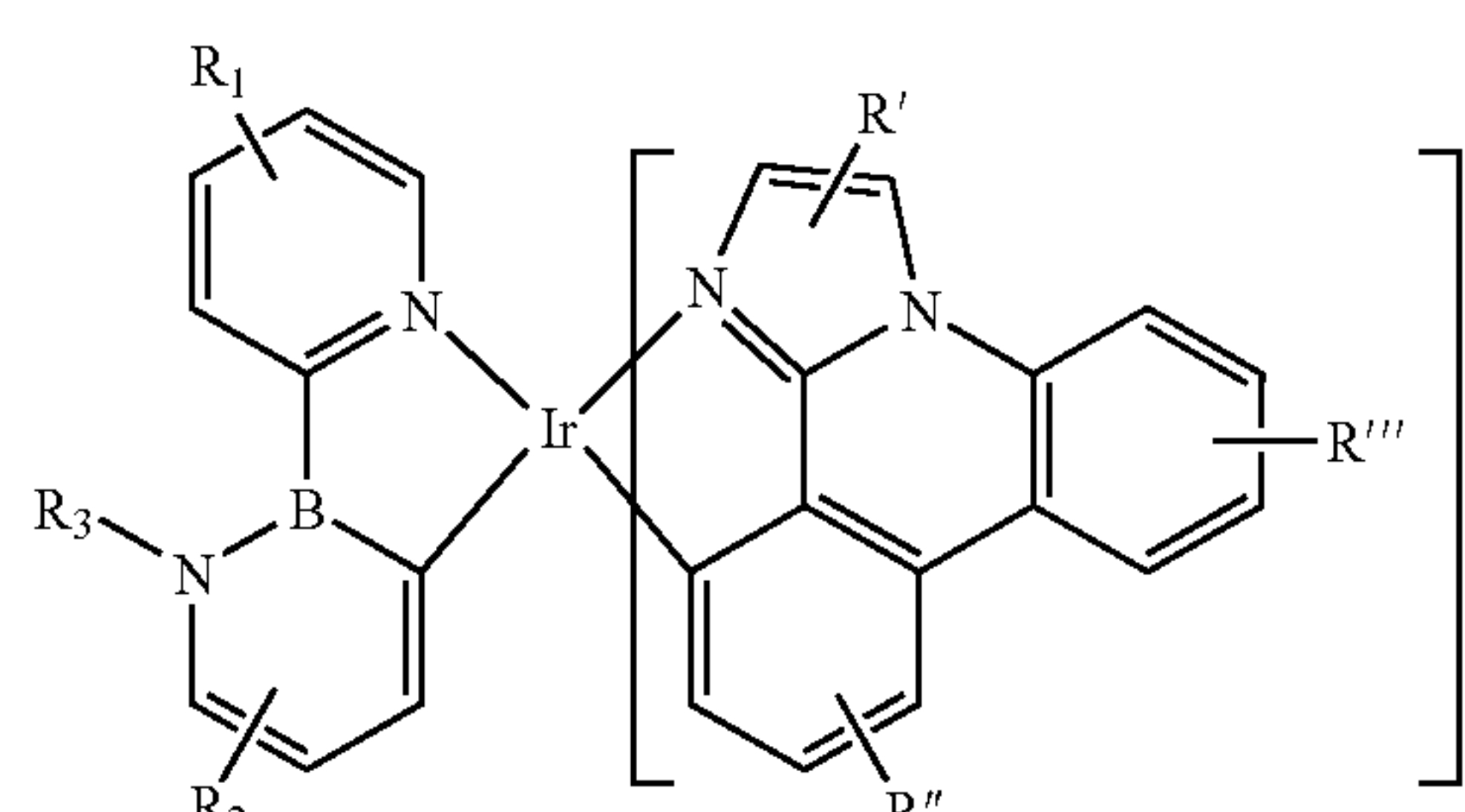
Compound 124G
