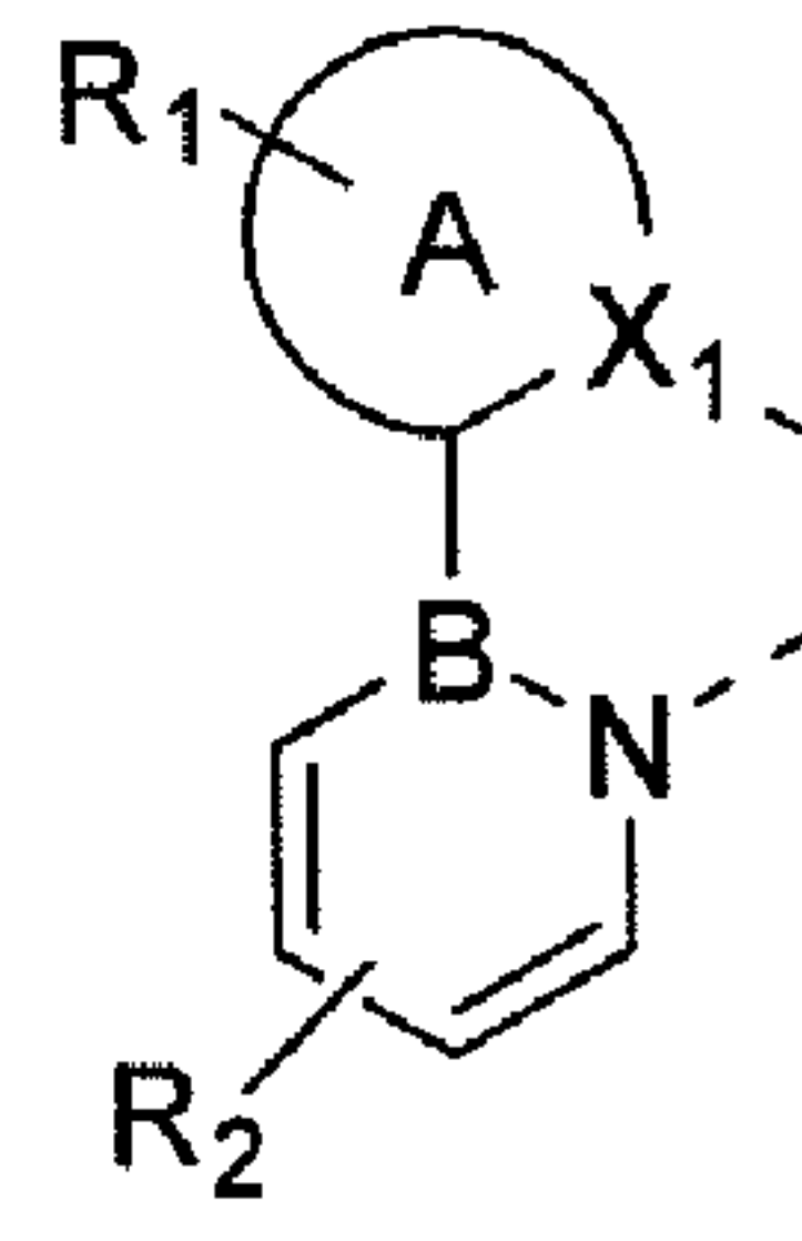
Compound 7
