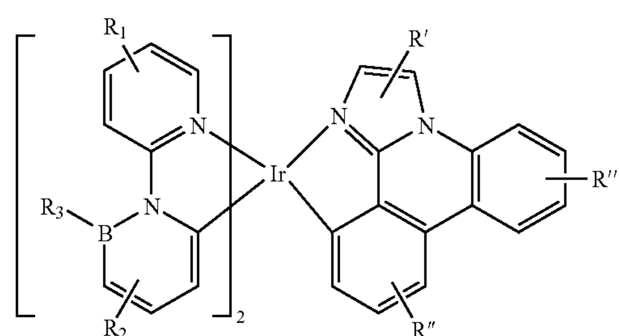
Compound 98G
