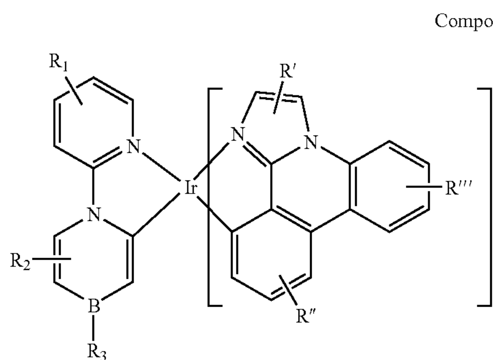
Compound 151G
