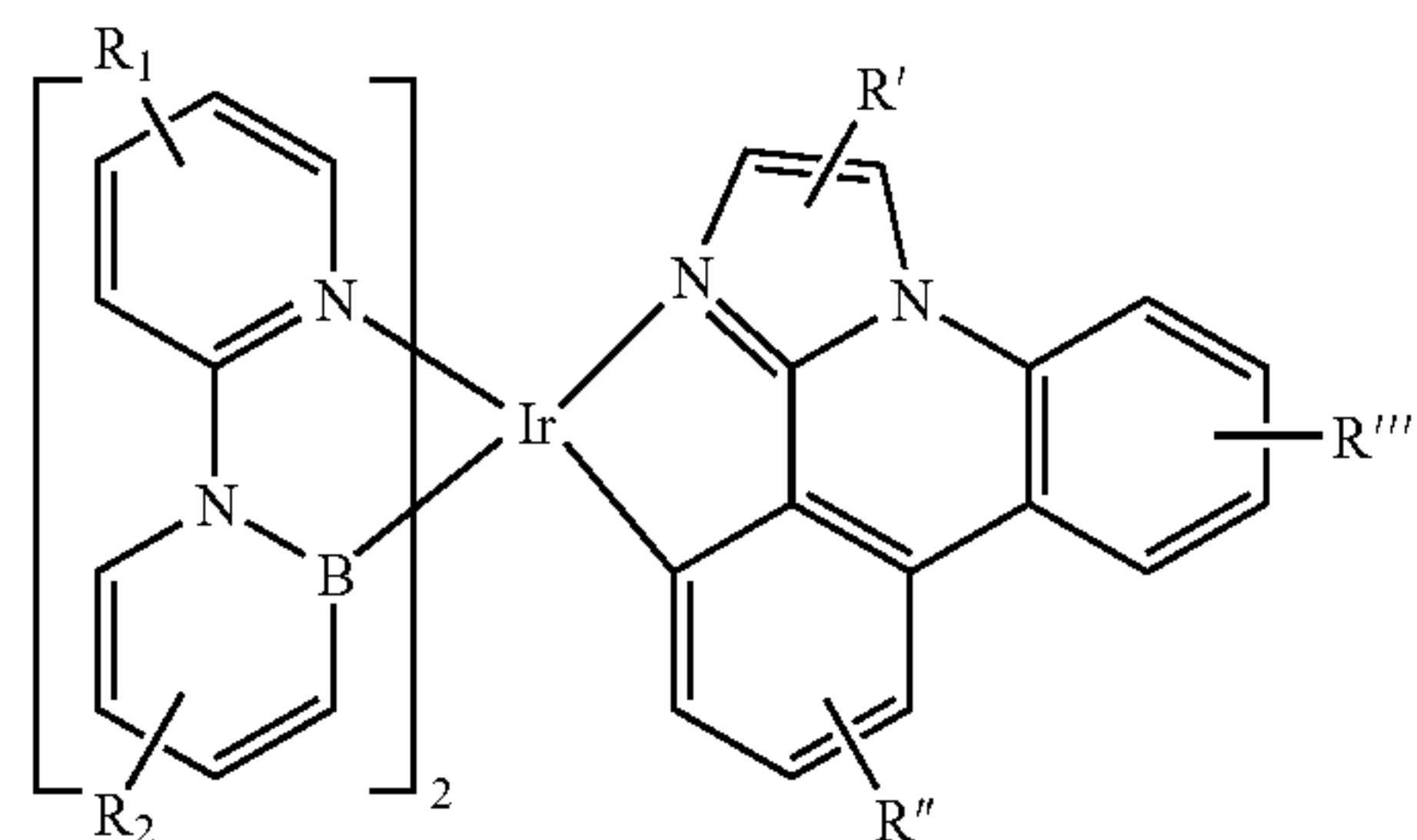
Compound 111G
