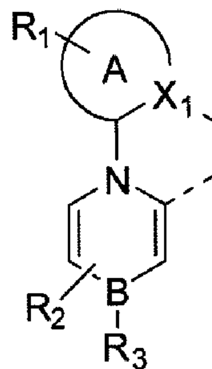
Compound 25
