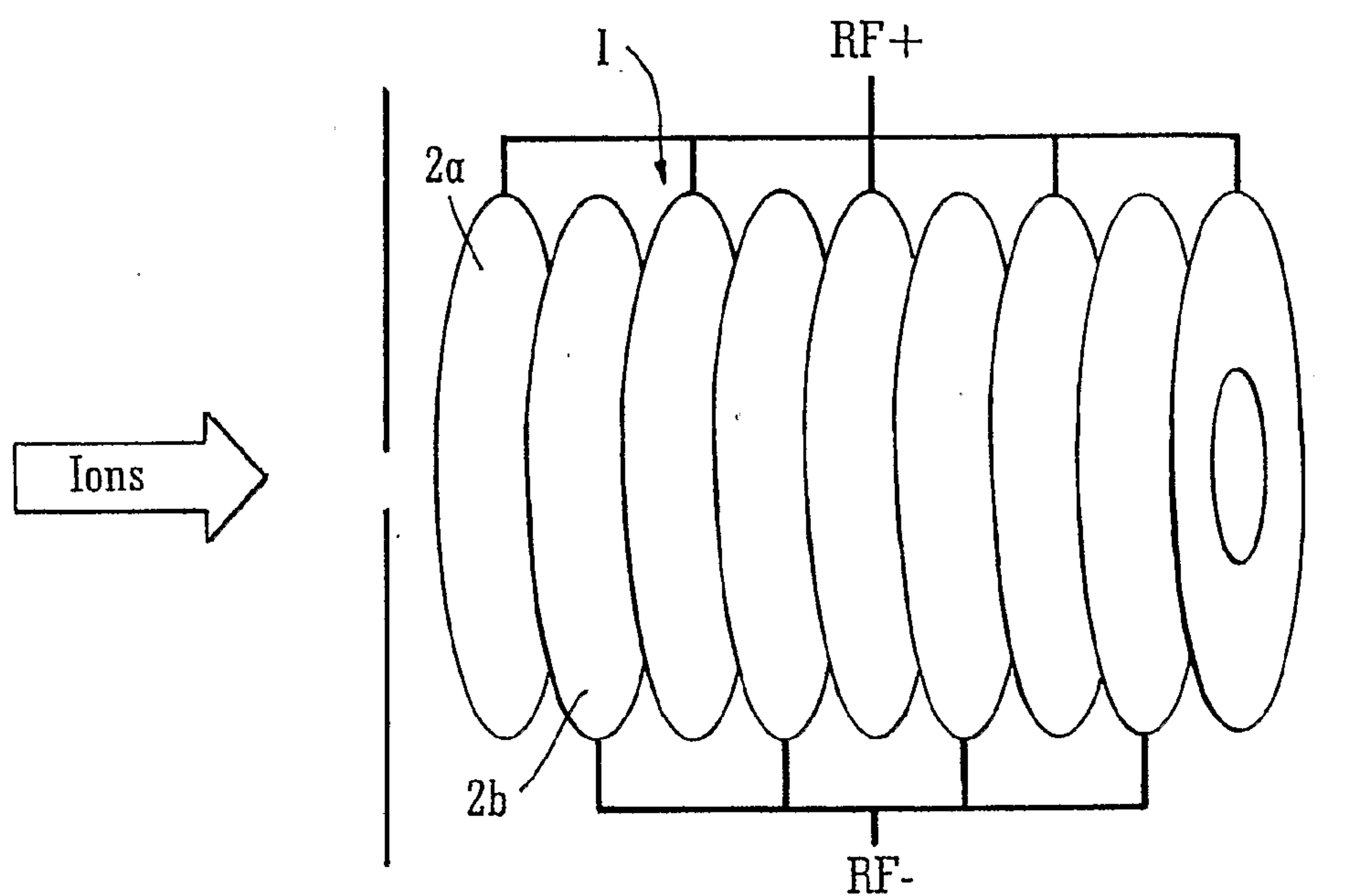
FIG. 1 PRIOR ART
