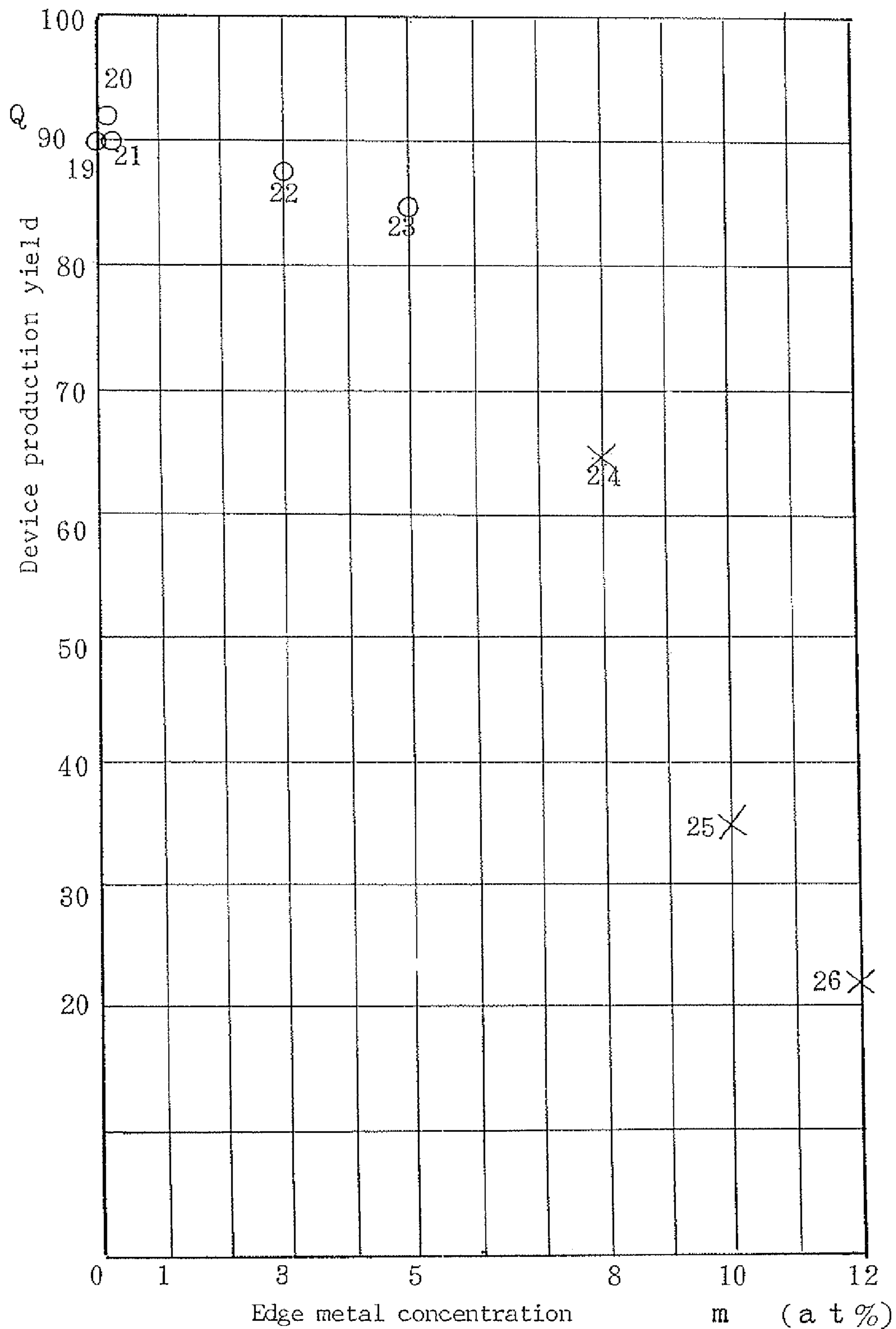
Metal Concentration and device production yield
