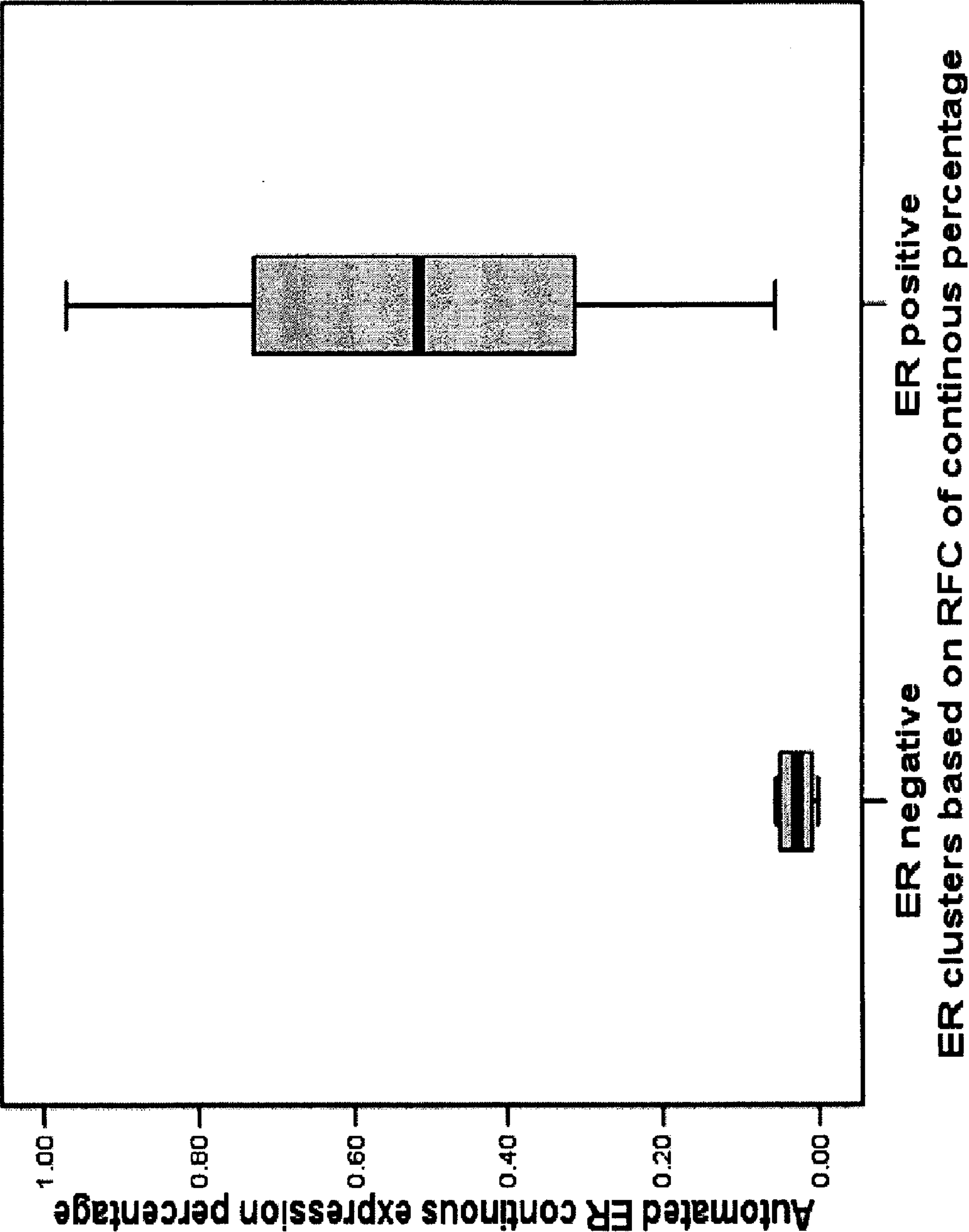
ER clusters based on RFC of continous percentage ER negative ER positive Figure 4C
