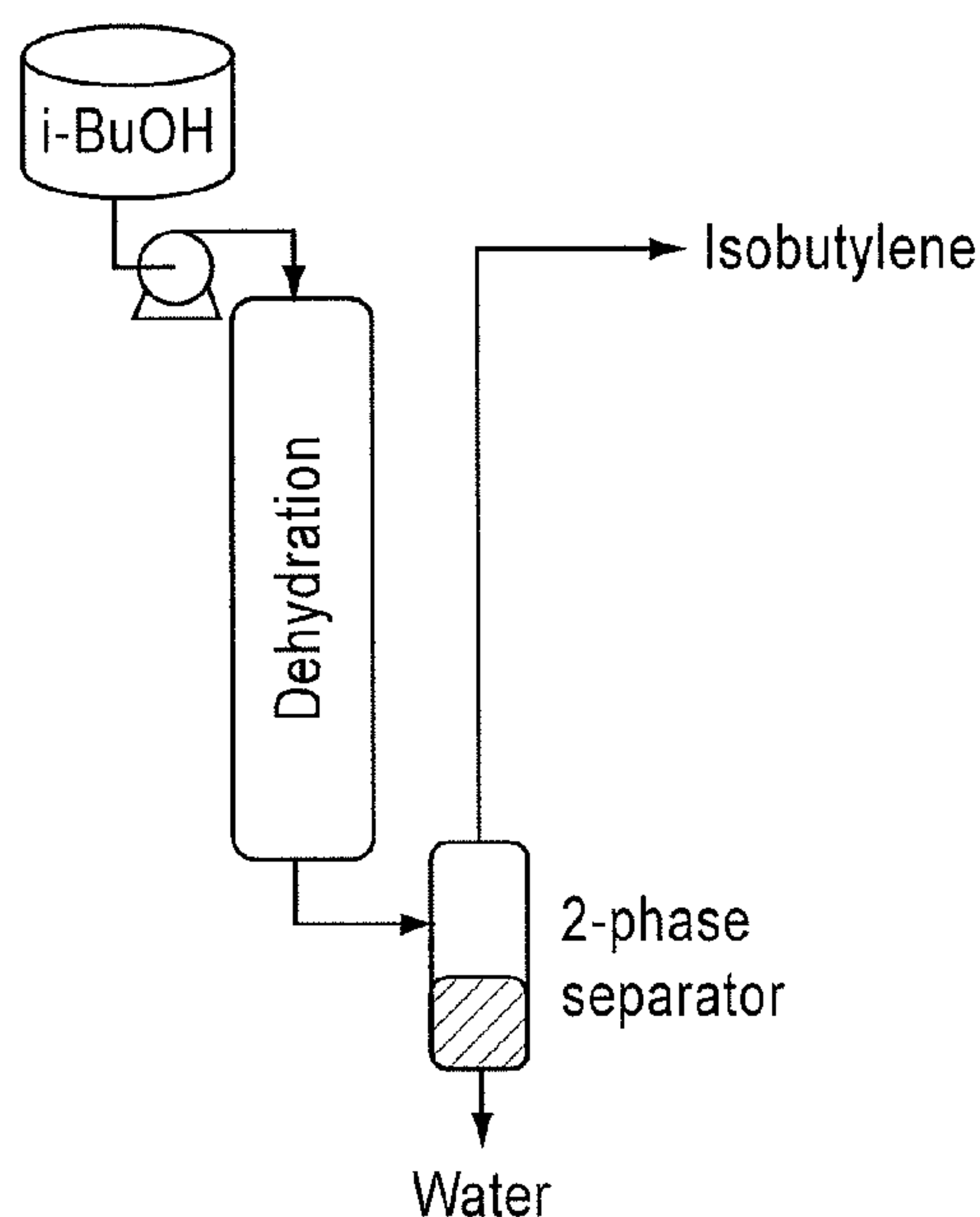
Dehydration Reactor Schematic
