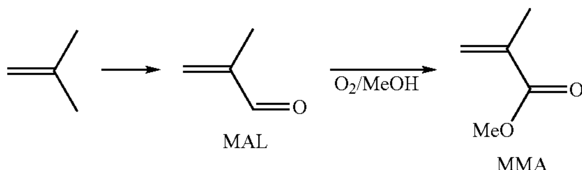
Scheme 9:
