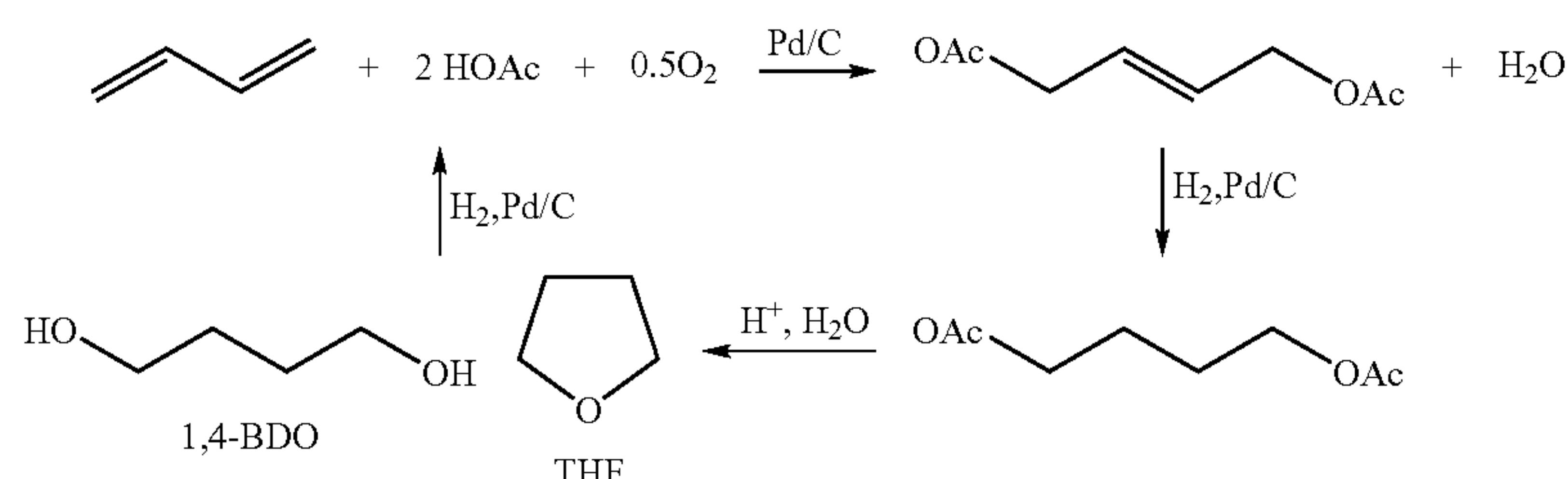
Scheme 1:
