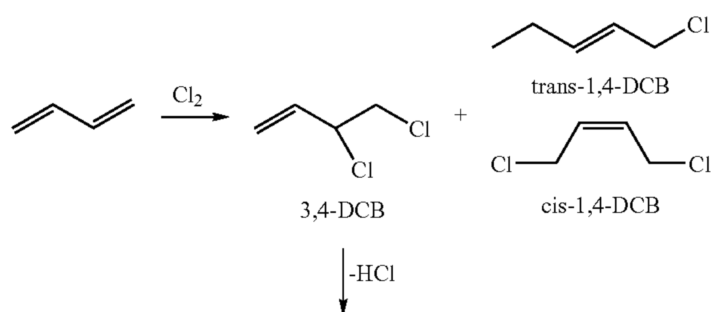
Scheme 4:
