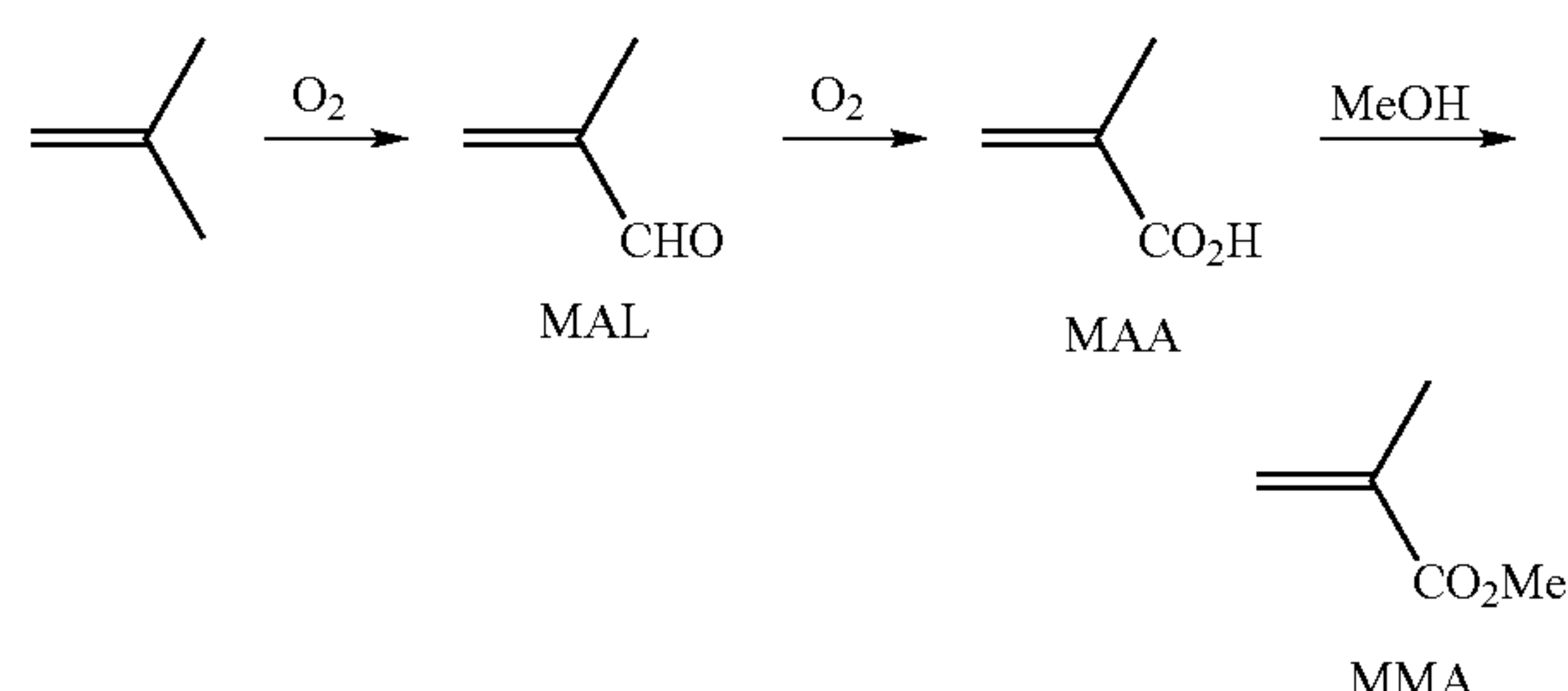
Scheme 8:
