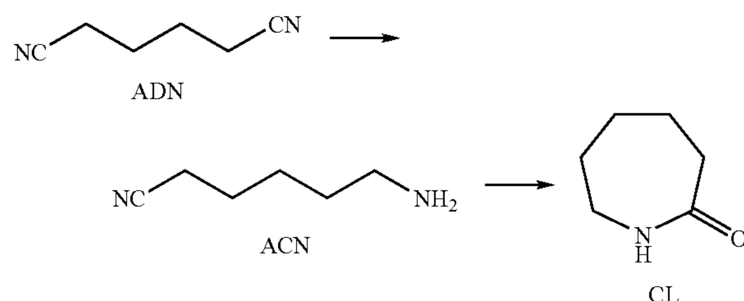
Scheme 6:
