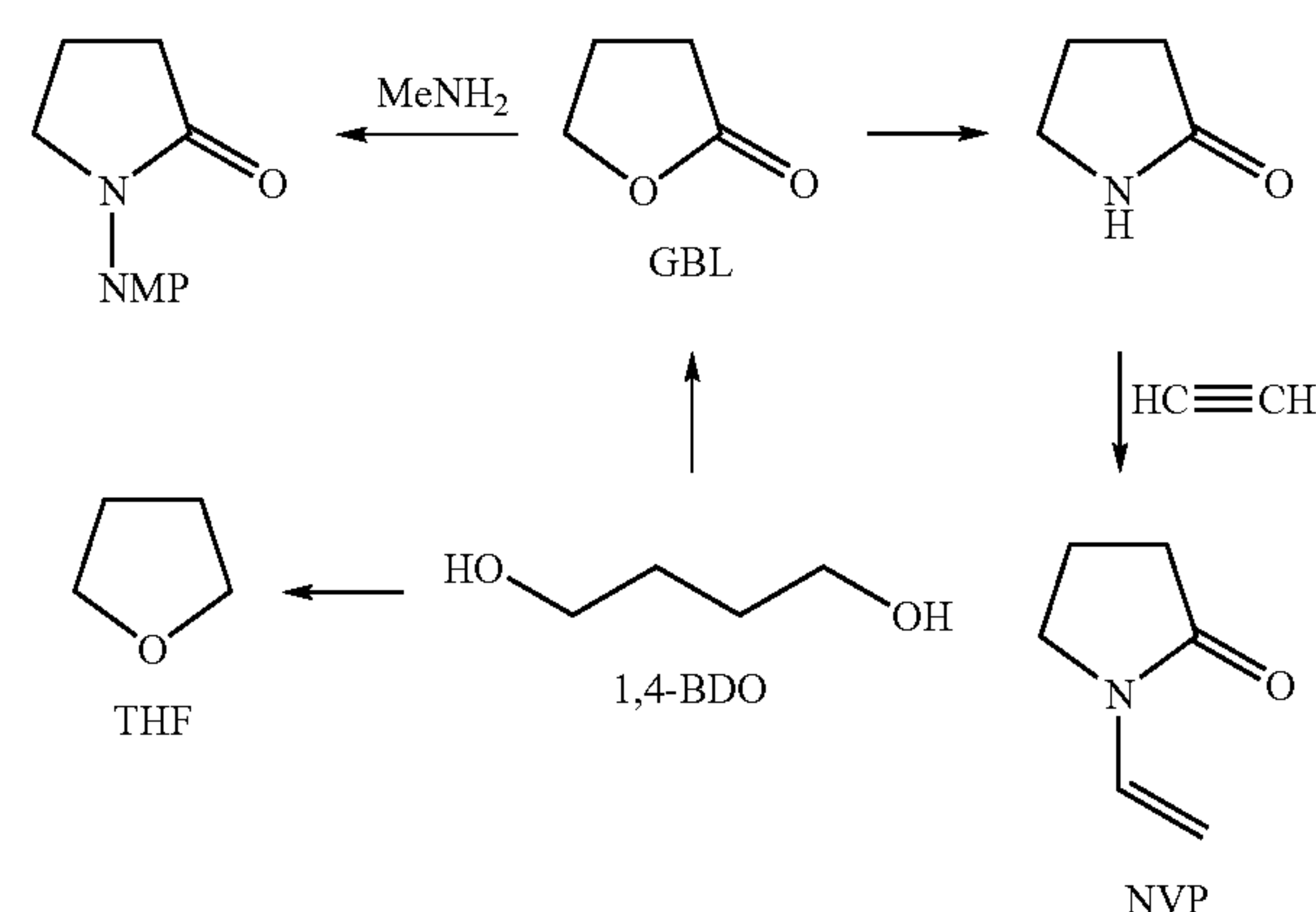
Scheme 2:
