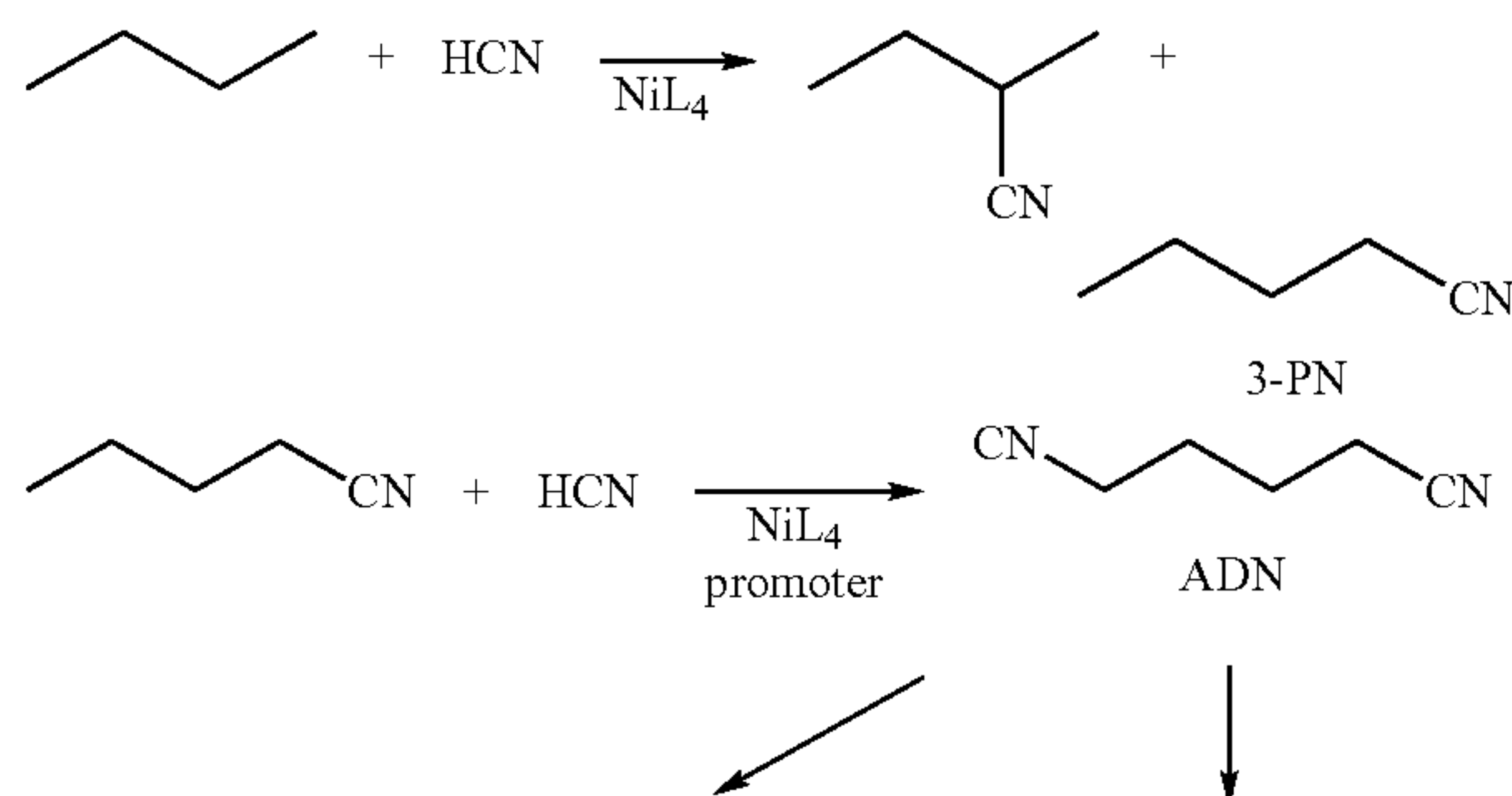
Scheme 5:
