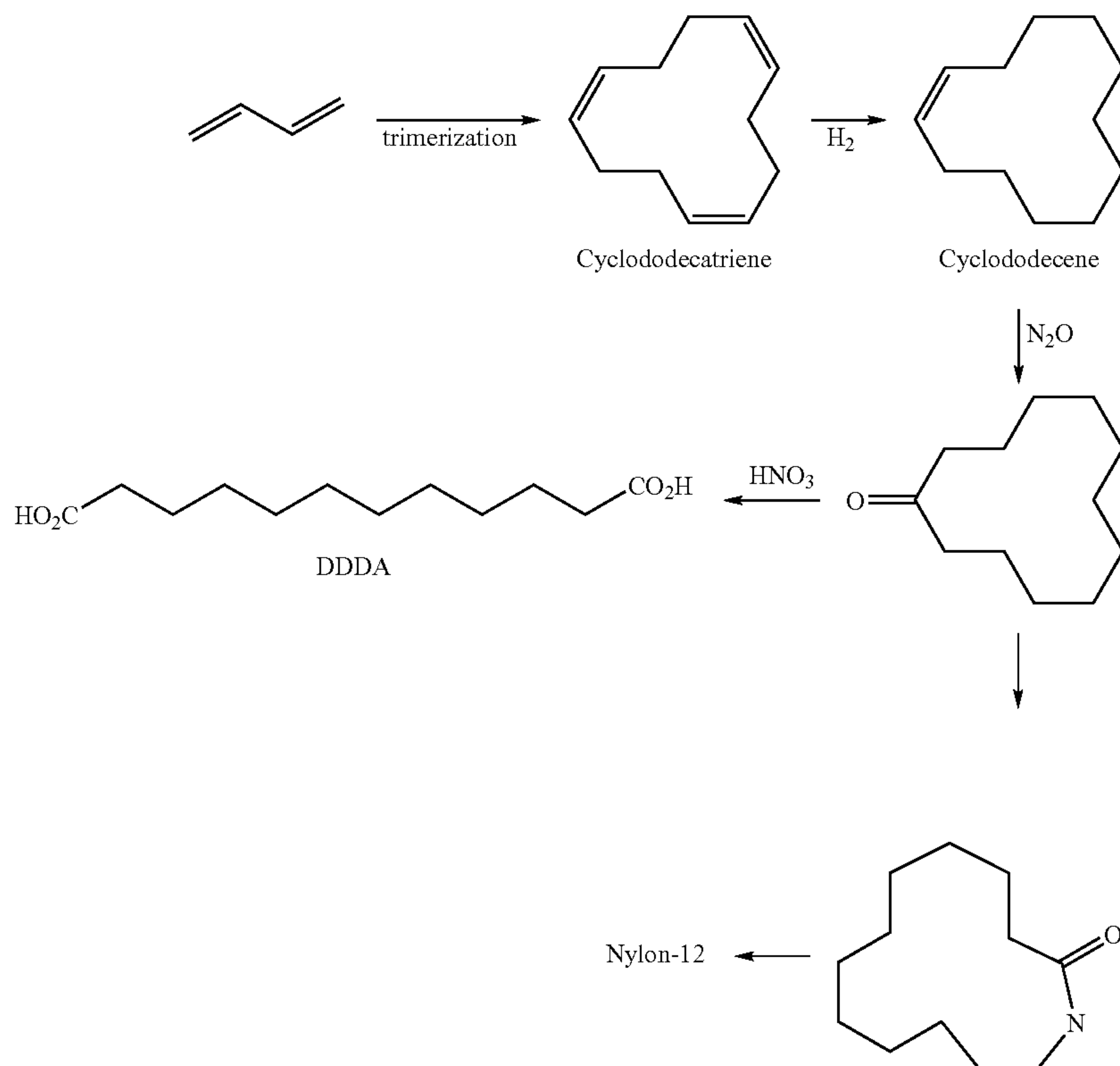
Scheme 3:
