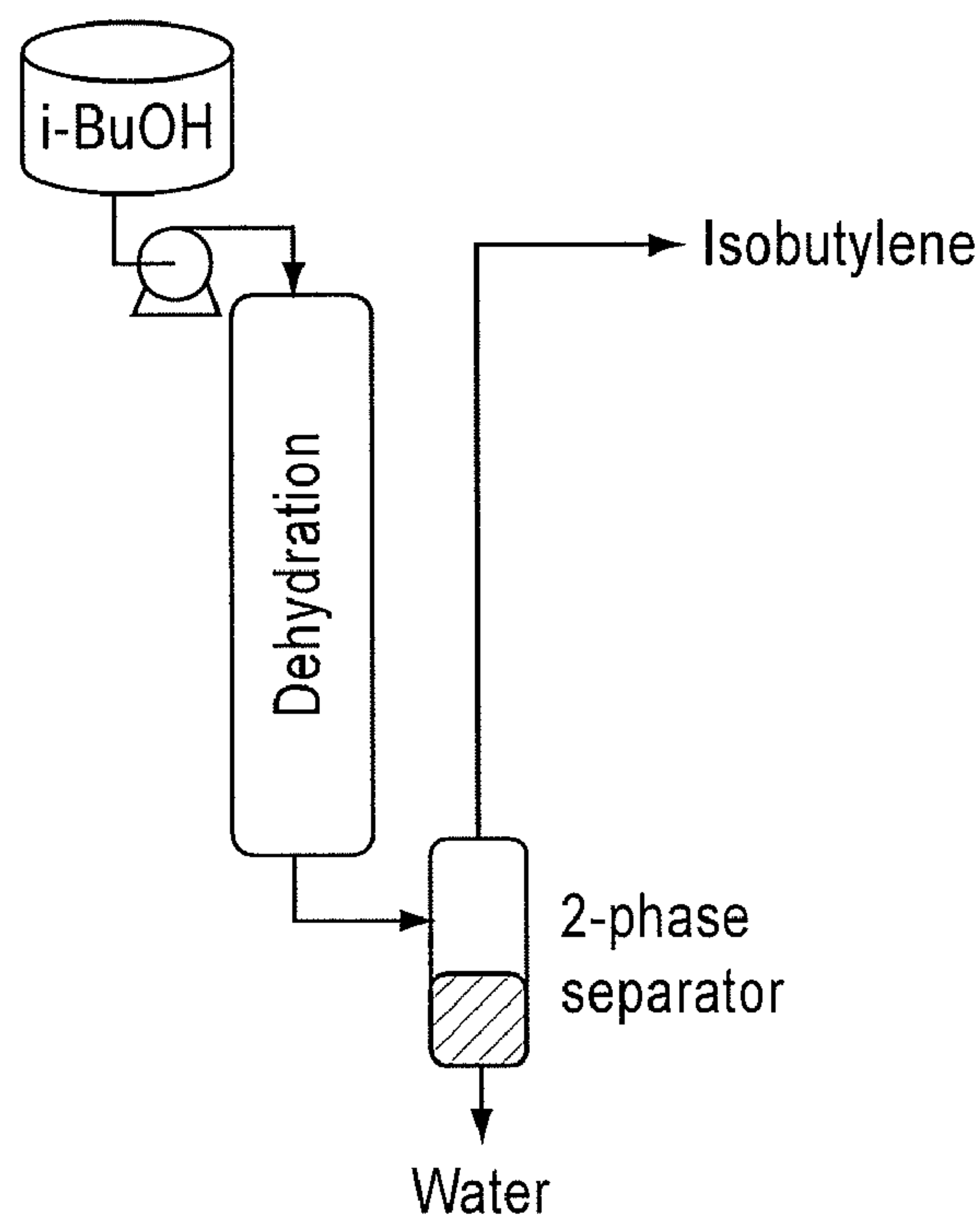
Dehydration Reactor Schematic
