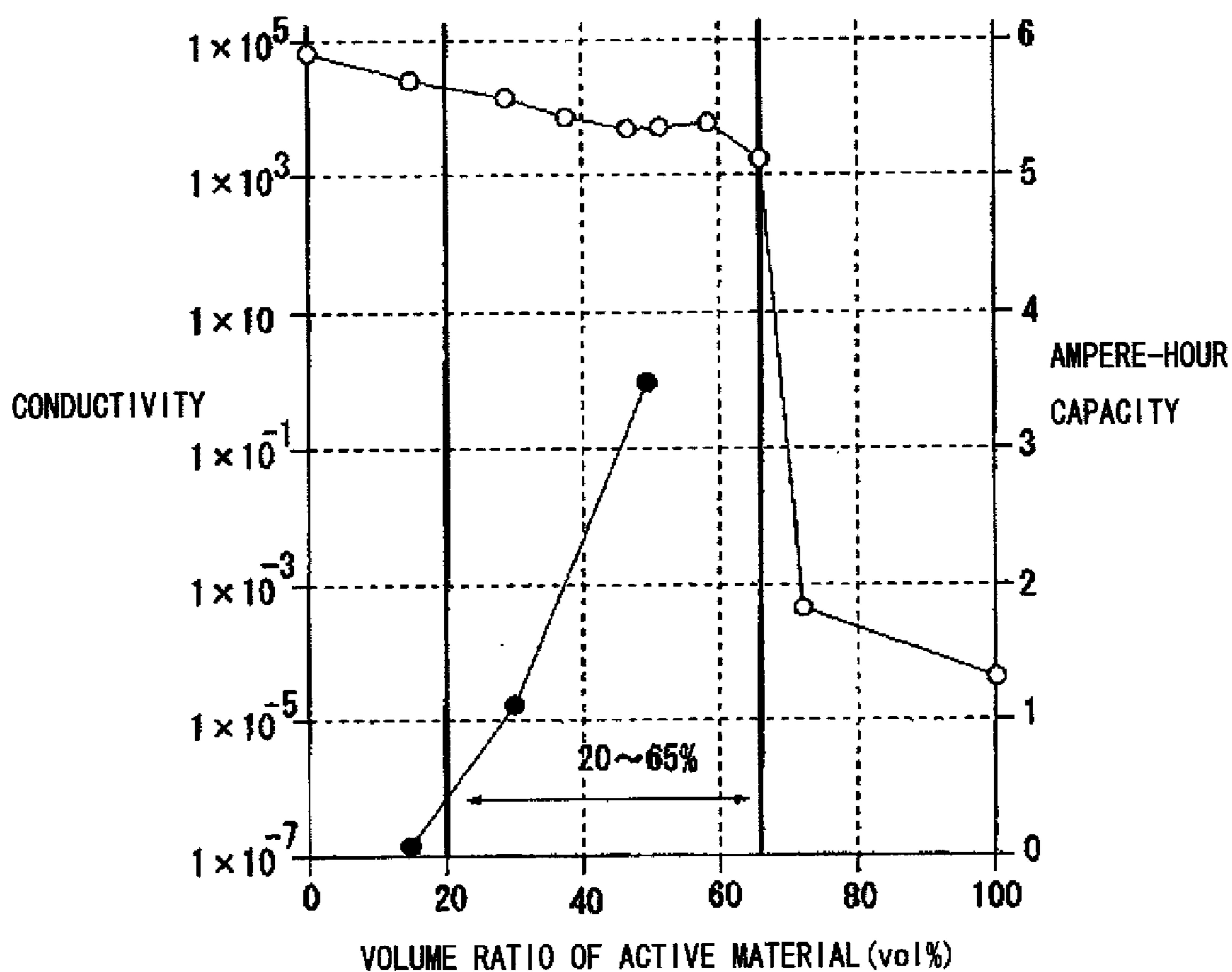
ELECTRIC CONDUCTIVITY AND AMPERE-HOUR CAPACITY VS. VOLUME RATIO BETWEEN POSITIVE ACTIVE MATERIAL AND CONDUCTIVE MATERIAL
