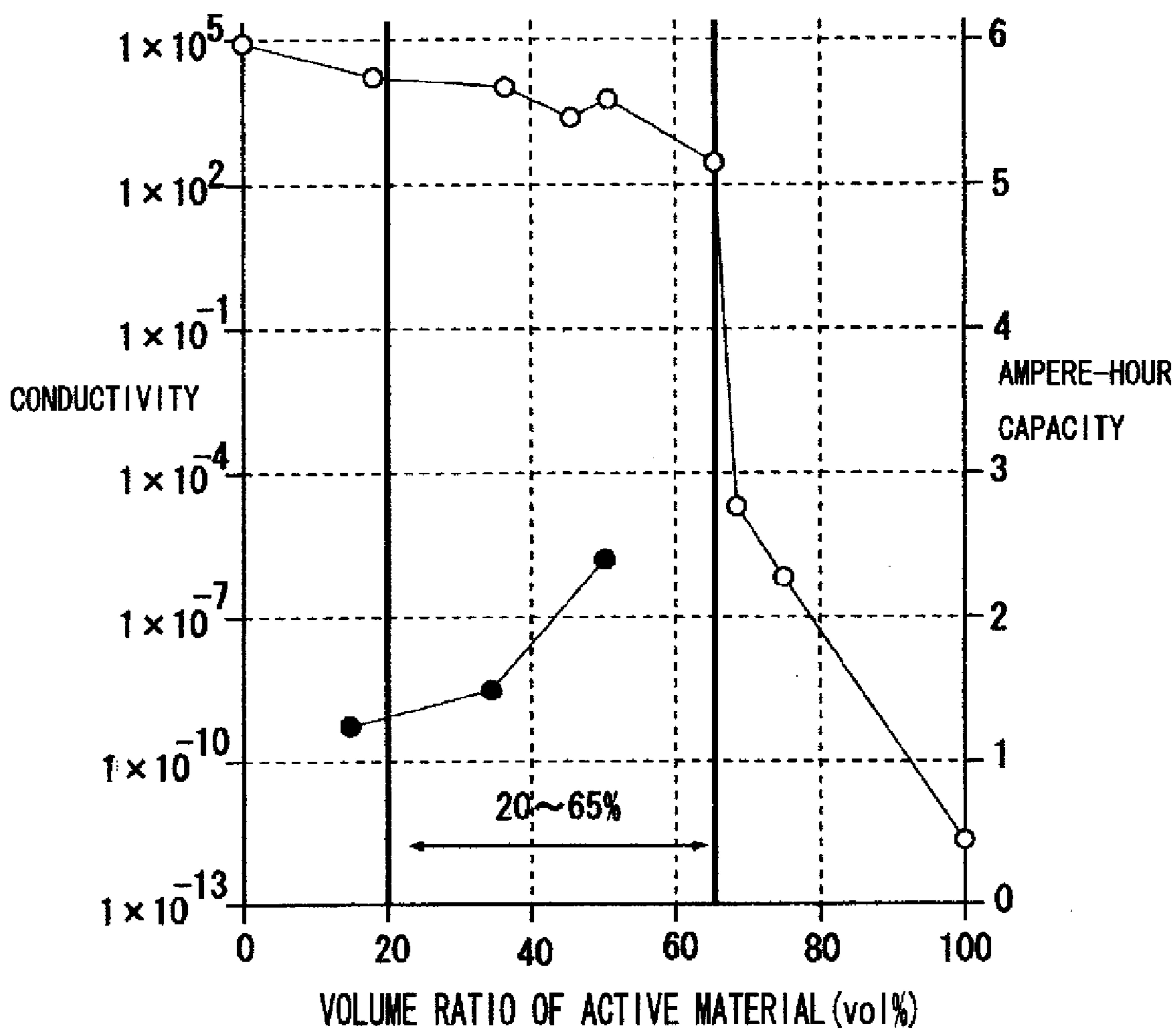
ELECTRIC CONDUCTIVITY AND AMPERE-HOUR CAPACITY VS. VOLUME RATIO BETWEEN NEGATIVE ACTIVE MATERIAL AND CONDUCTIVE MATERIAL
