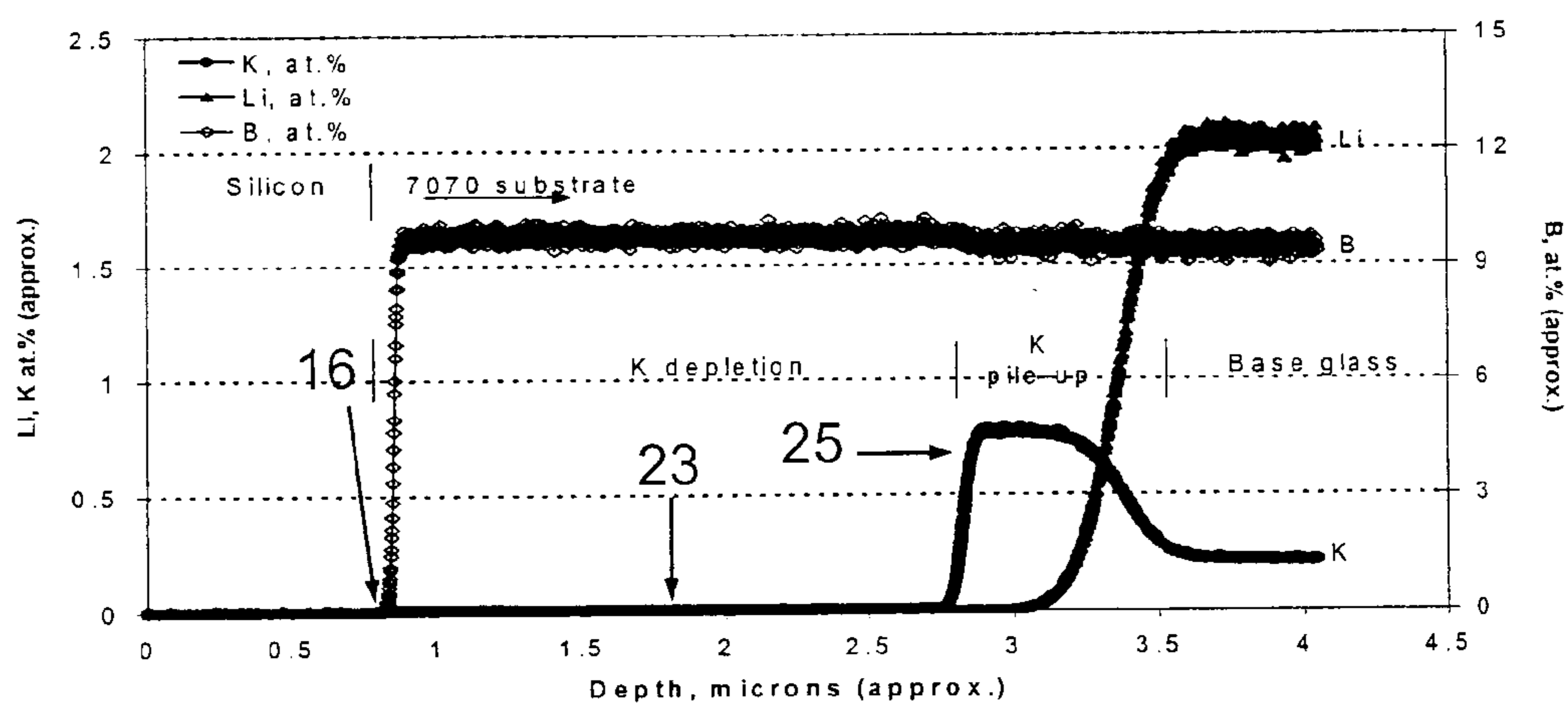
ToF-SIMS DEPTH PROFILE OF Si/7070 (RE-FIRED)
