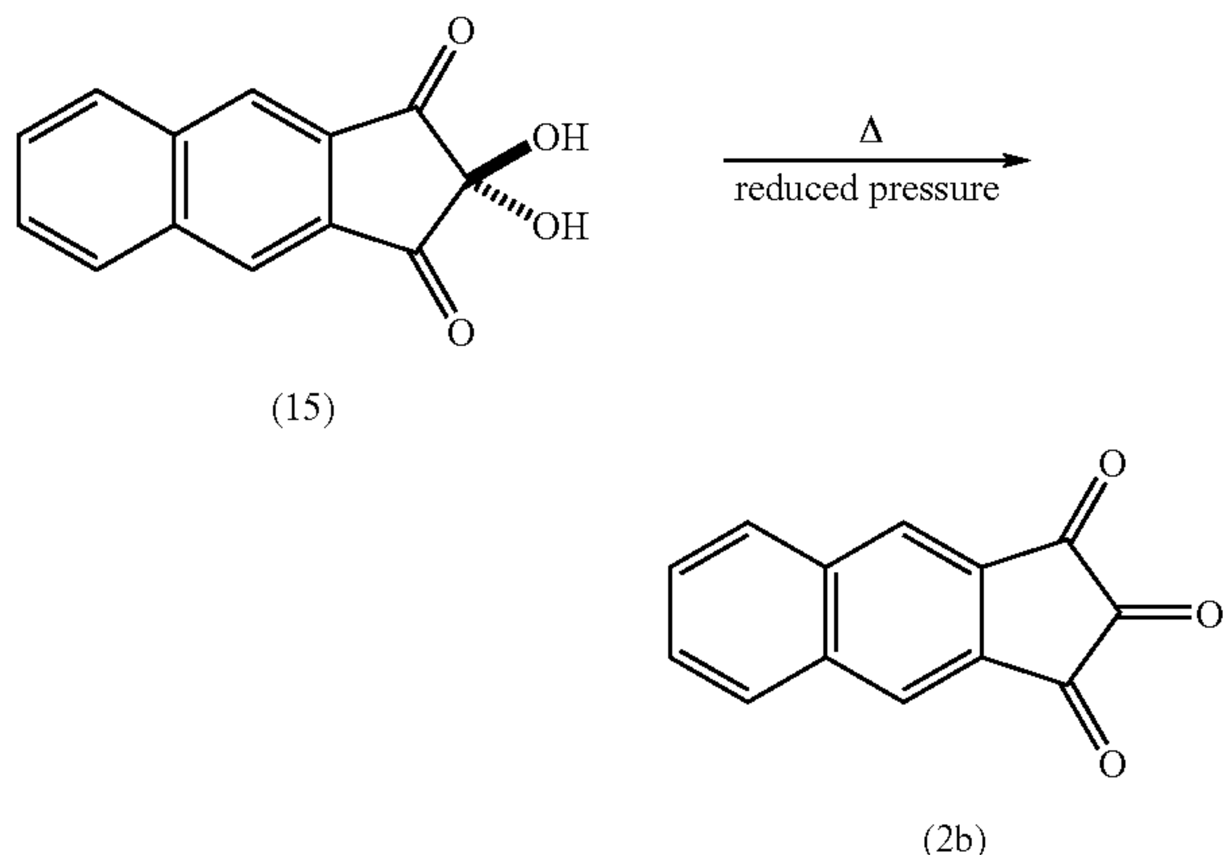
[Chemical Formula 17]
