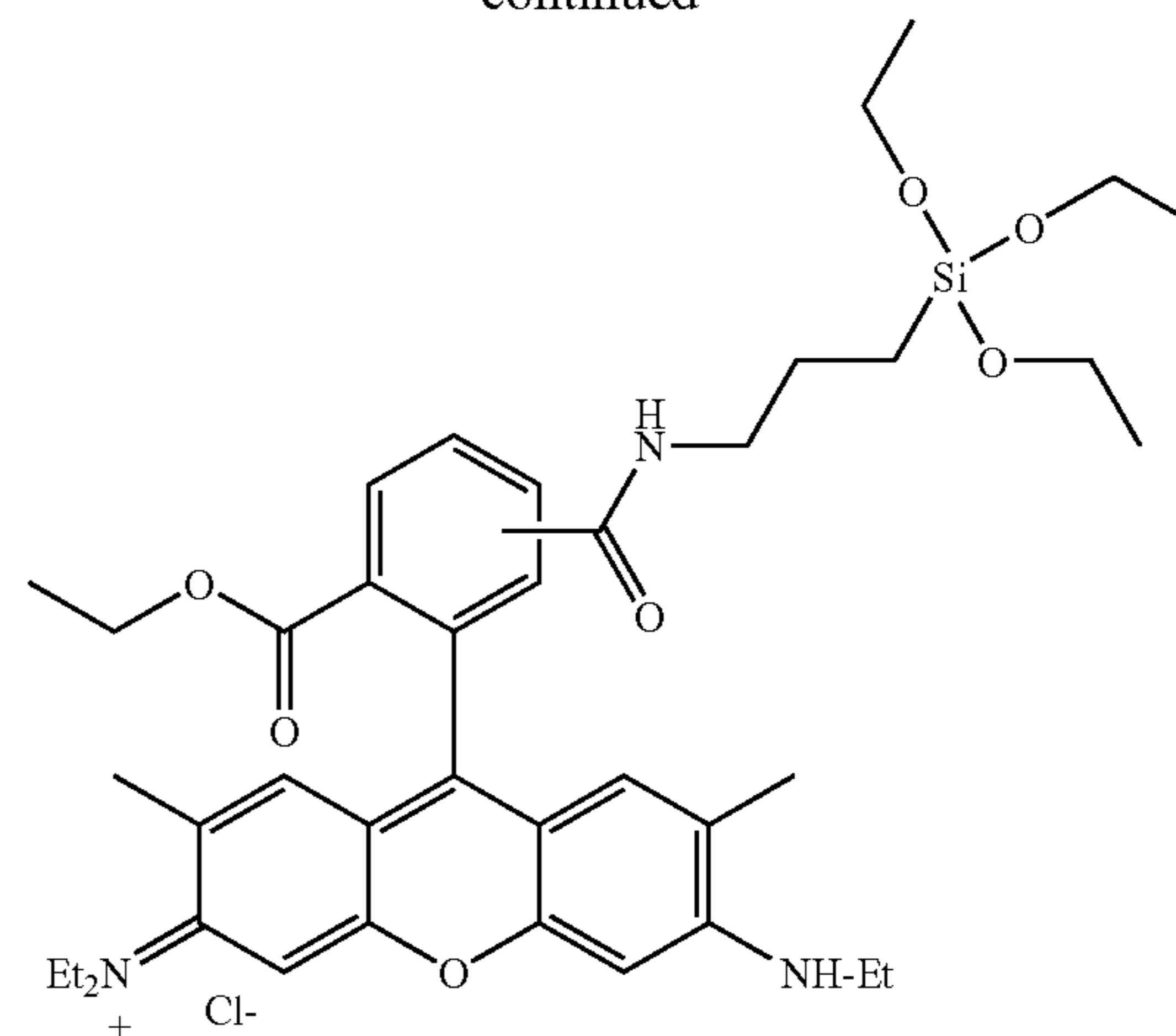
Rhodamine 6G-silane derivative 5-(and-6)-Carboxyrhodamine 6G Succinimidyl ester
