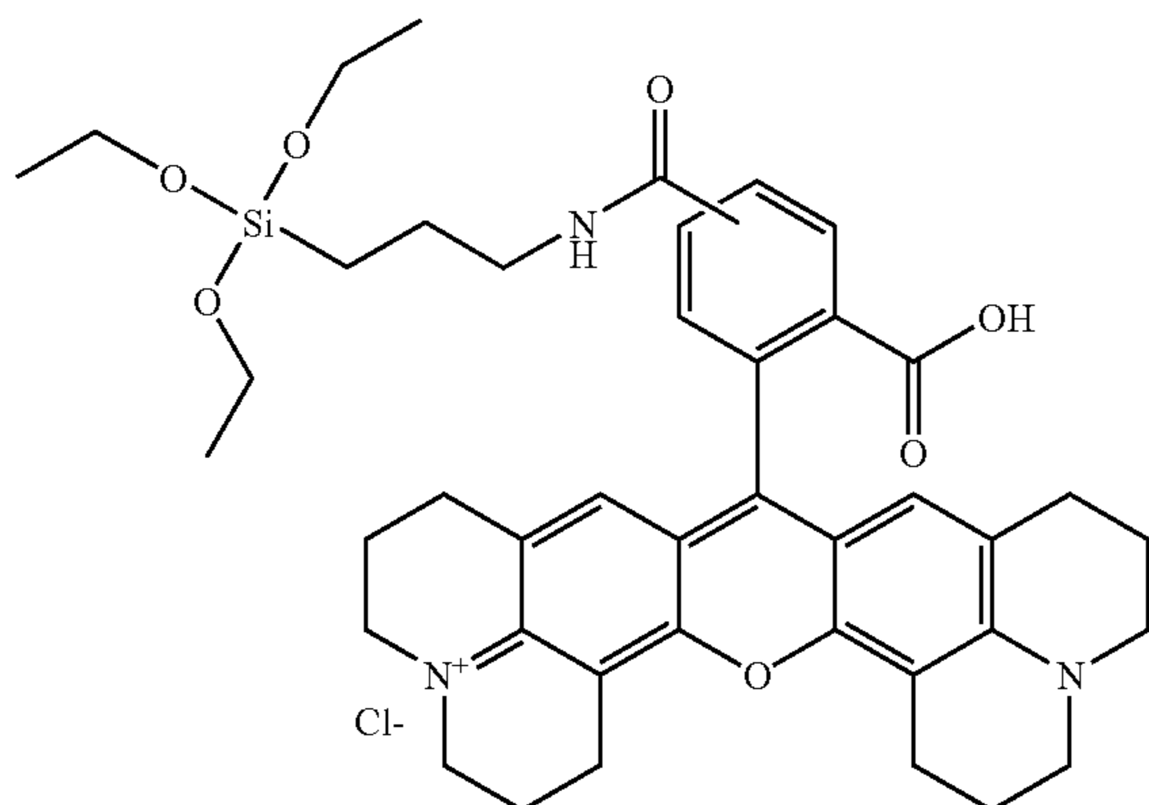
ROX-silane derivative obtainable from: 5-(and-6)-carboxy-X-rhodamine succinimidyl ester
