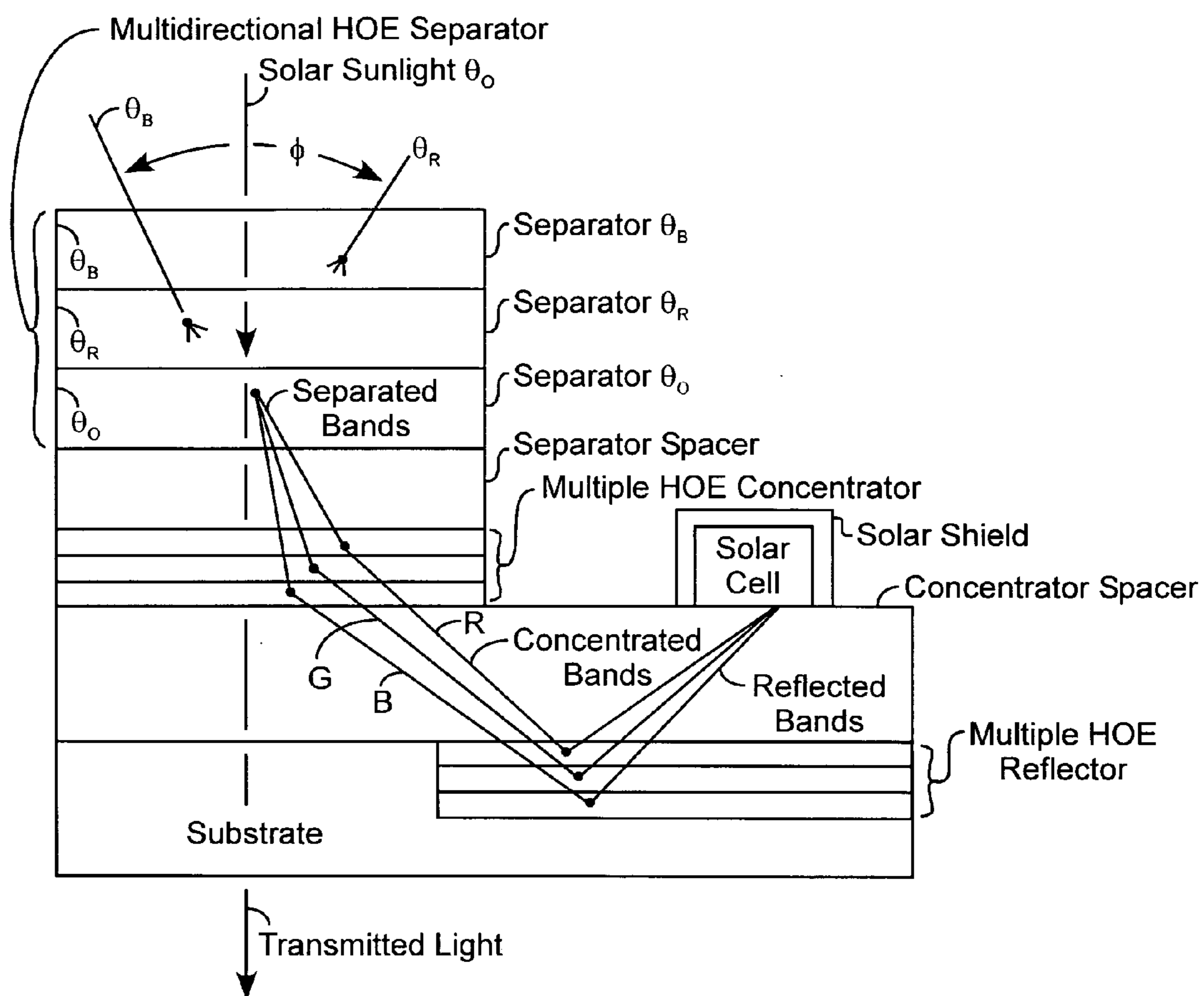
MULTIDIRECTIONAL MULTIPLE HOE SOLAR CONCENTRATOR
