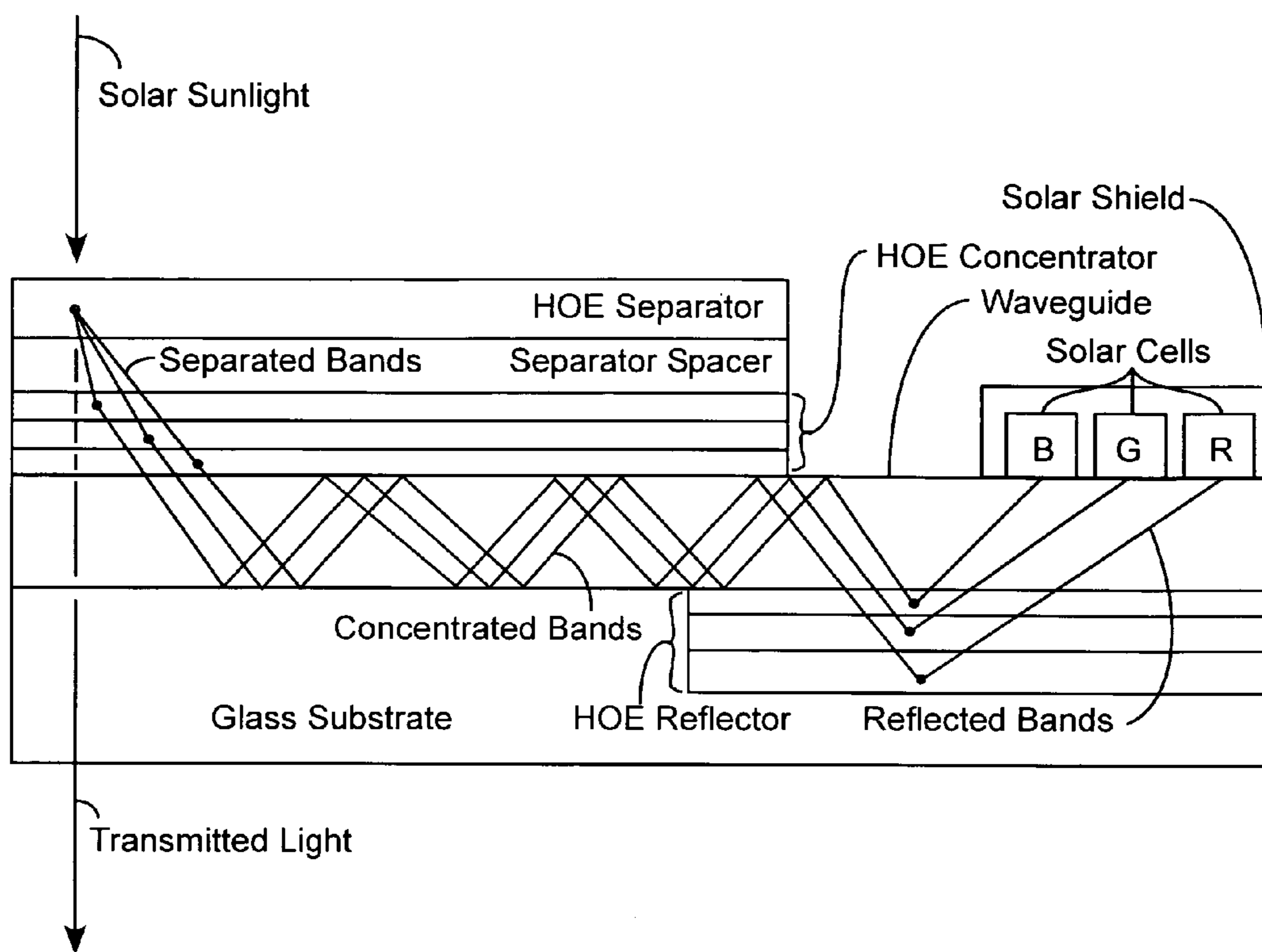
MULTIPLE HOE WAVEGUIDE SERIAL SOLAR CONCENTRATOR
