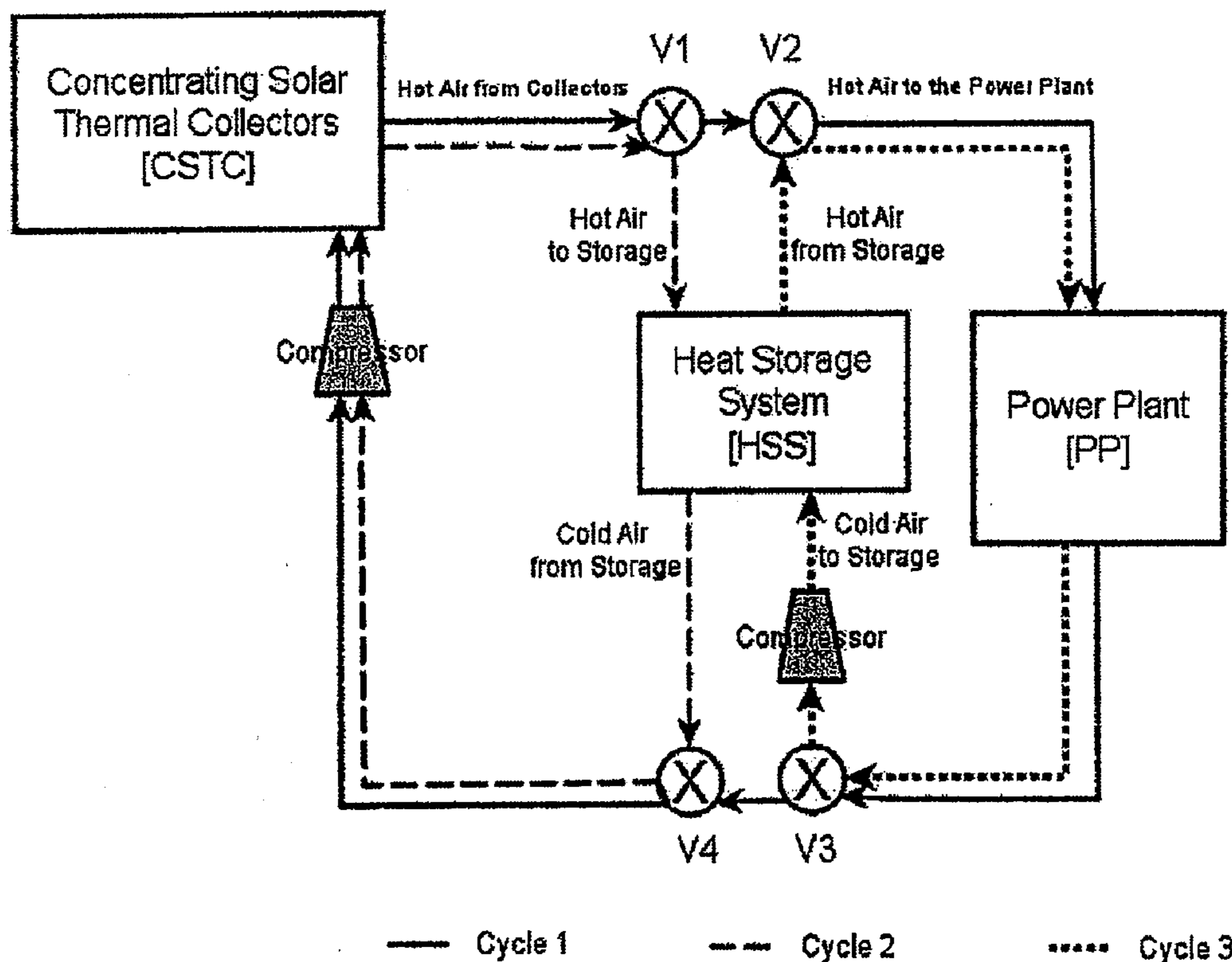
Concentrated Solar Energy with Heat Storage Capability
