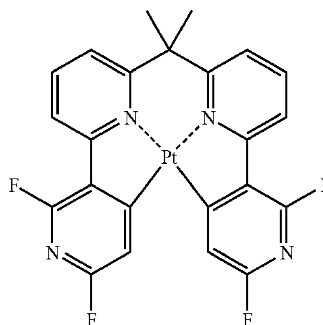
-continued D-4
