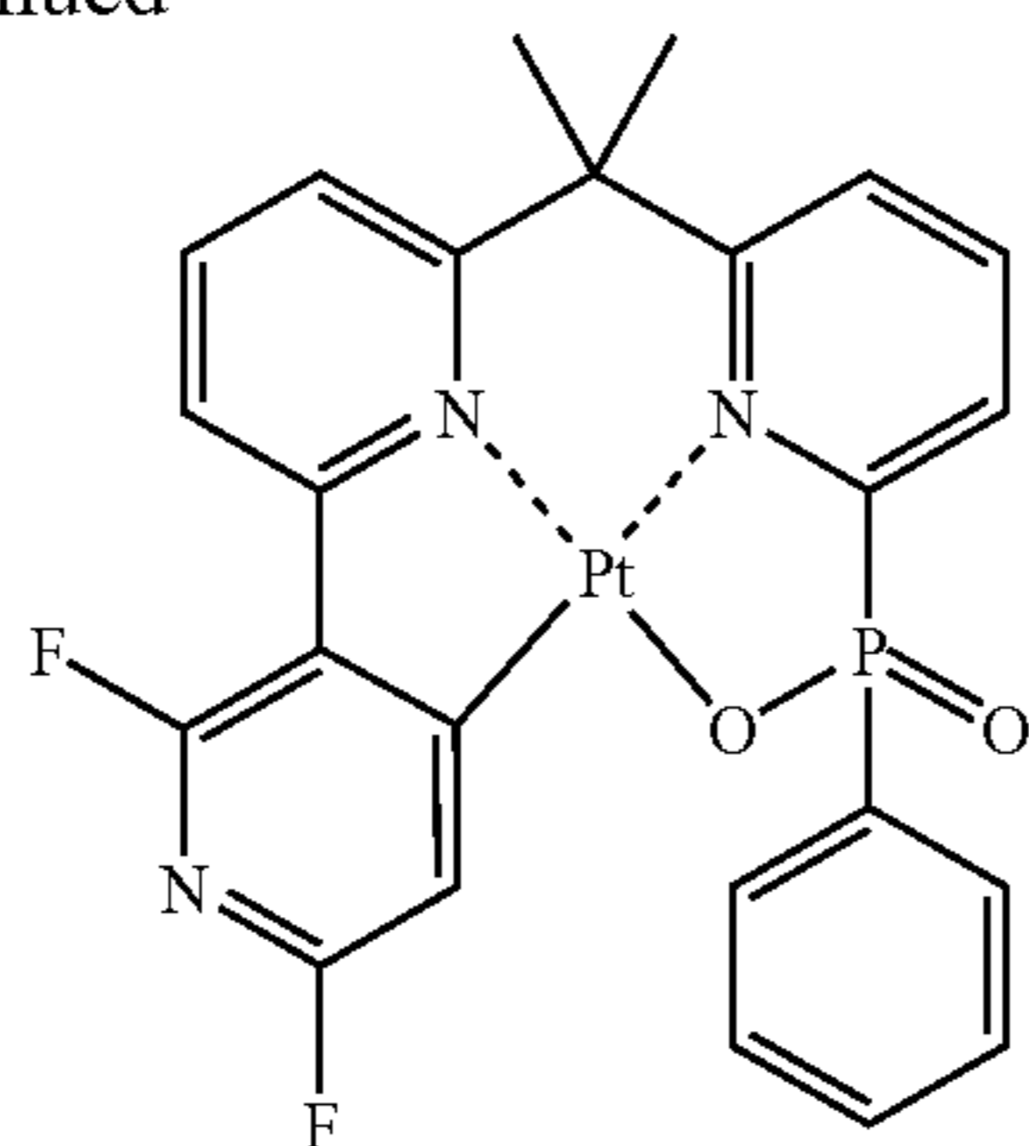
Exemplified compound 3
