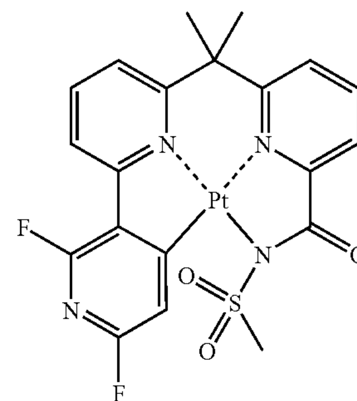
Exemplified compound 2
