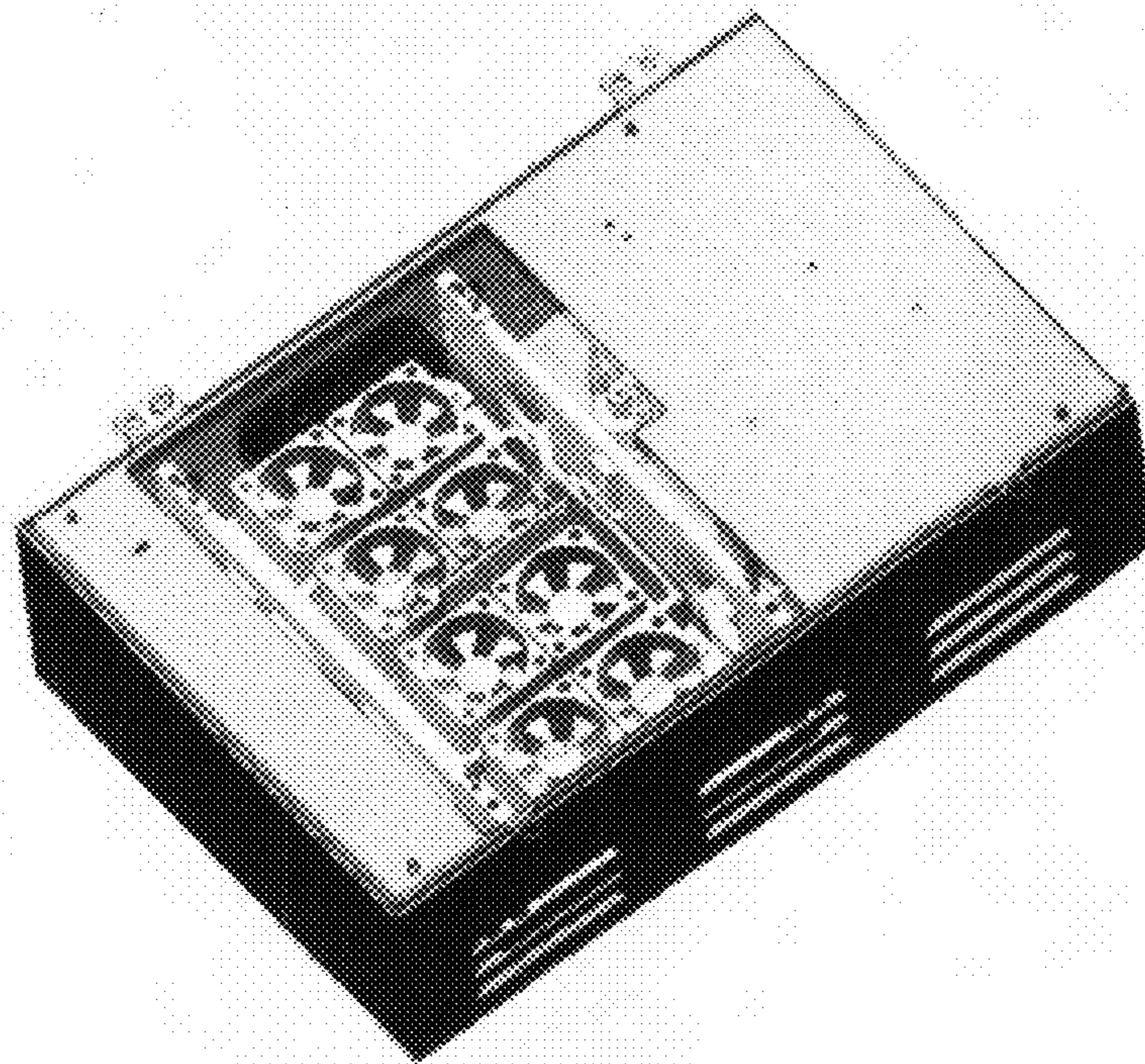
Thermal control element: bottom view
