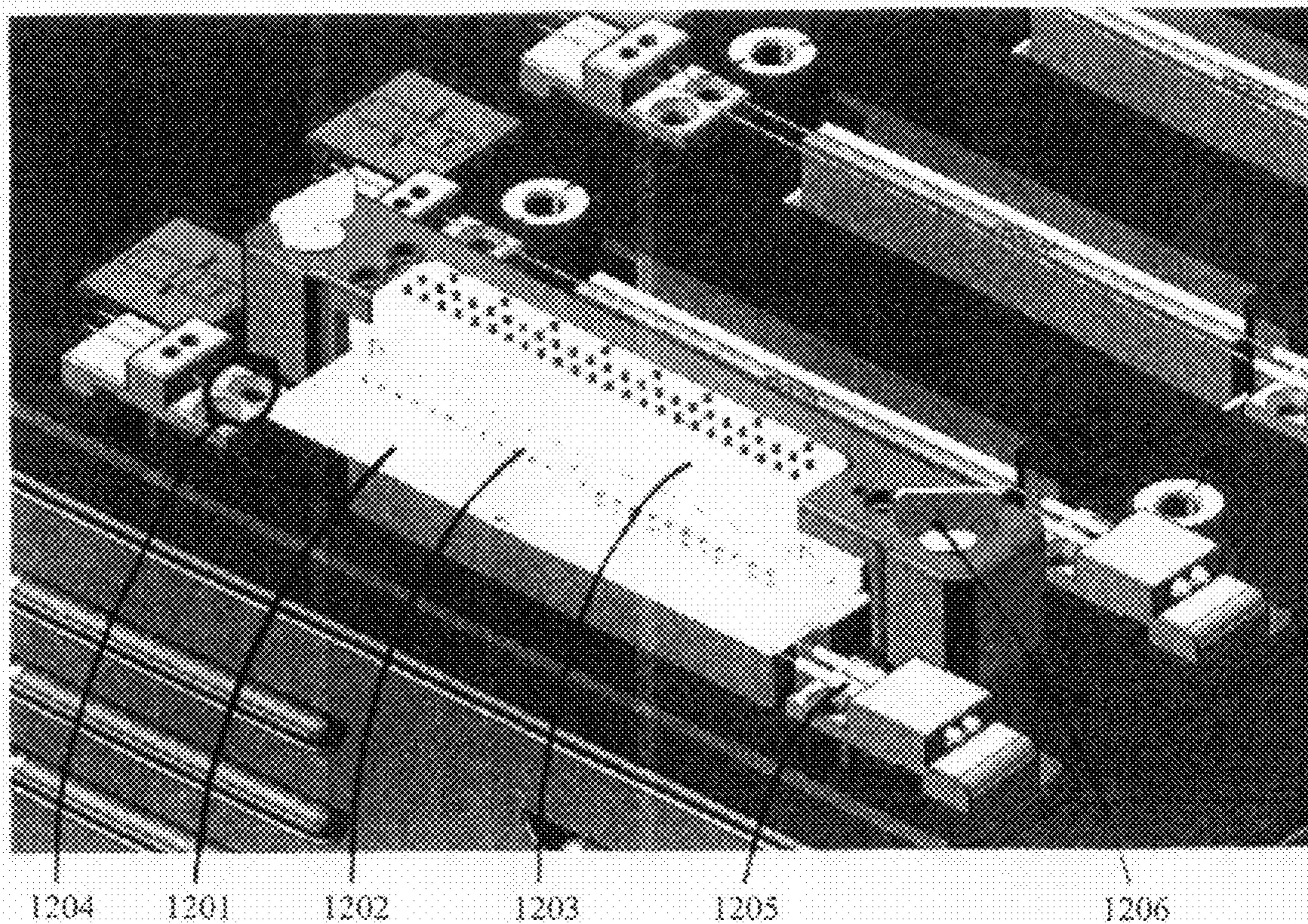
Microfluidic chip device attached to one station of thermal control element
