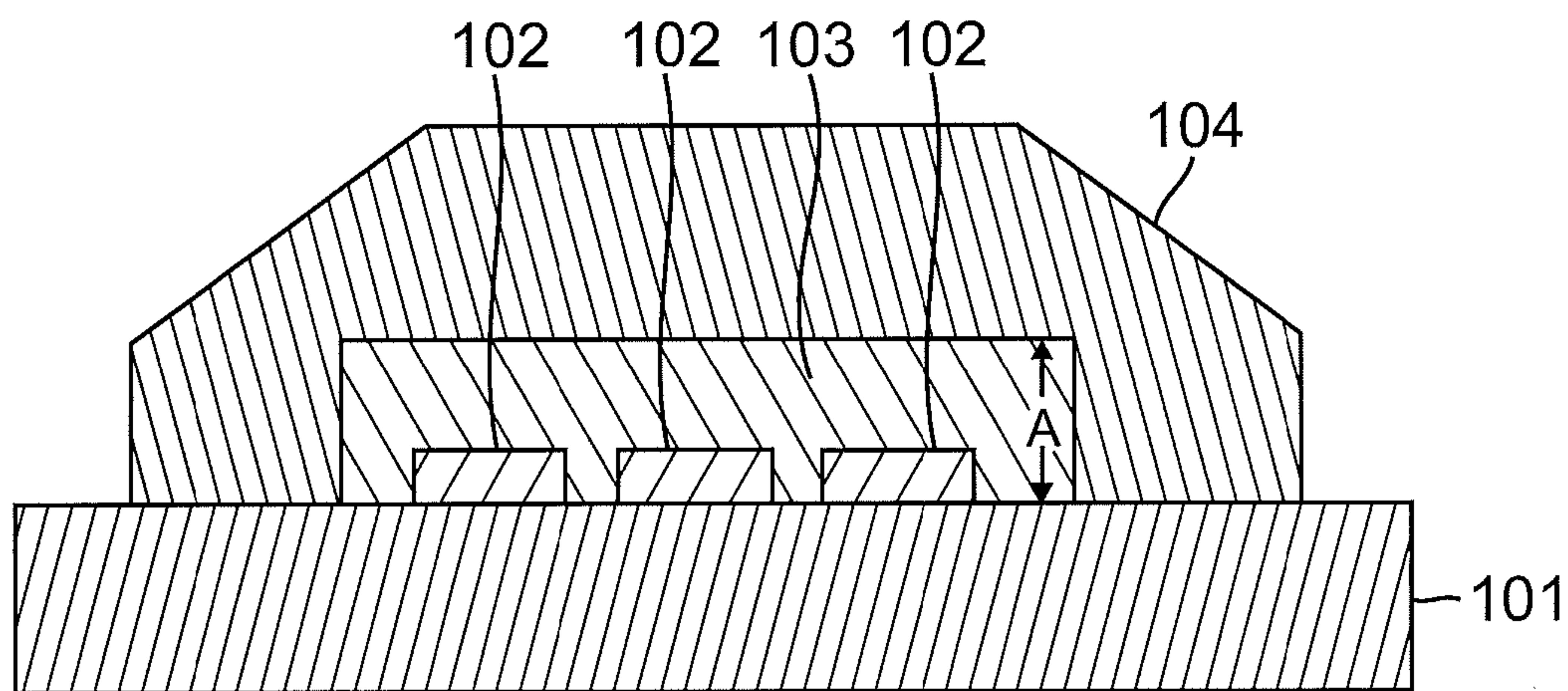
FIG. 1 (Prior art)
