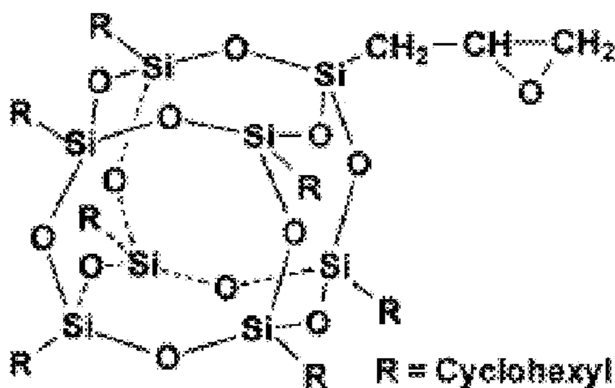
Monofunctional POSS Molecule
