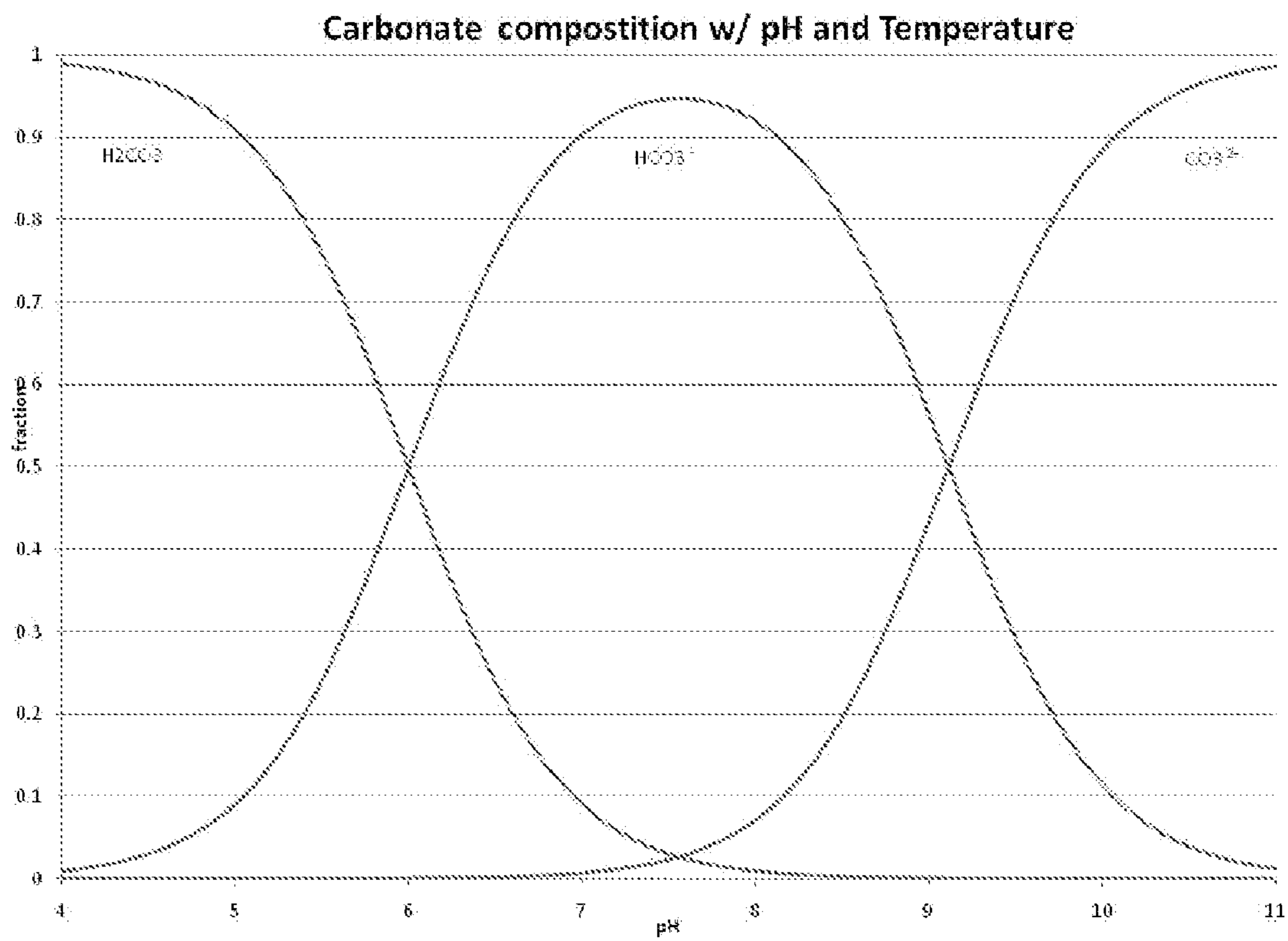
Carbonate/Bicarbonate speciation in H_2O v. pH at 25 °C.
