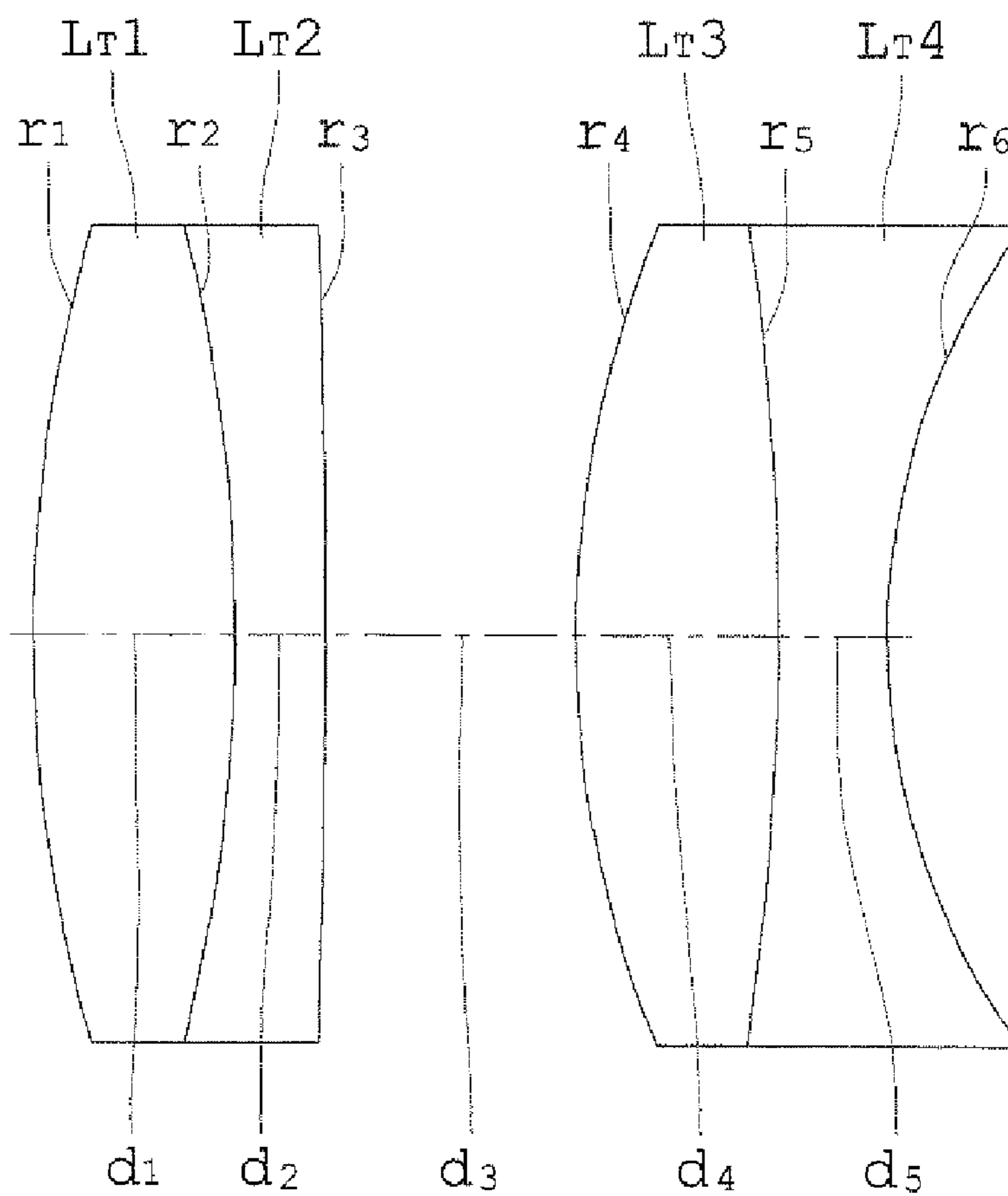
EMBODIMENT 11 TUBE LENS : f_{TL}=280\text{mm}
