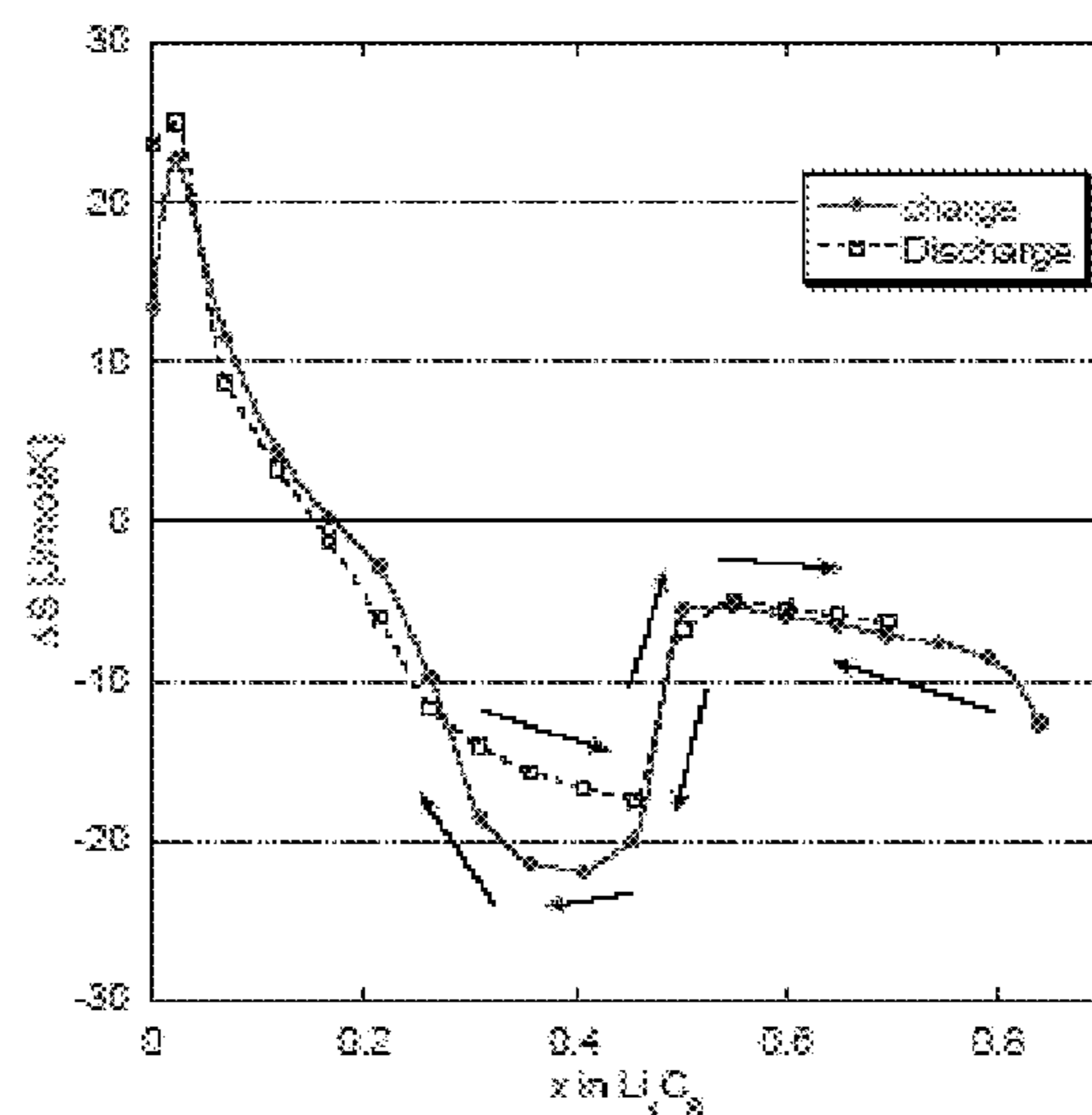
Entropy of Li intercalation during charge and discharge of coke HTT at 2500°C
