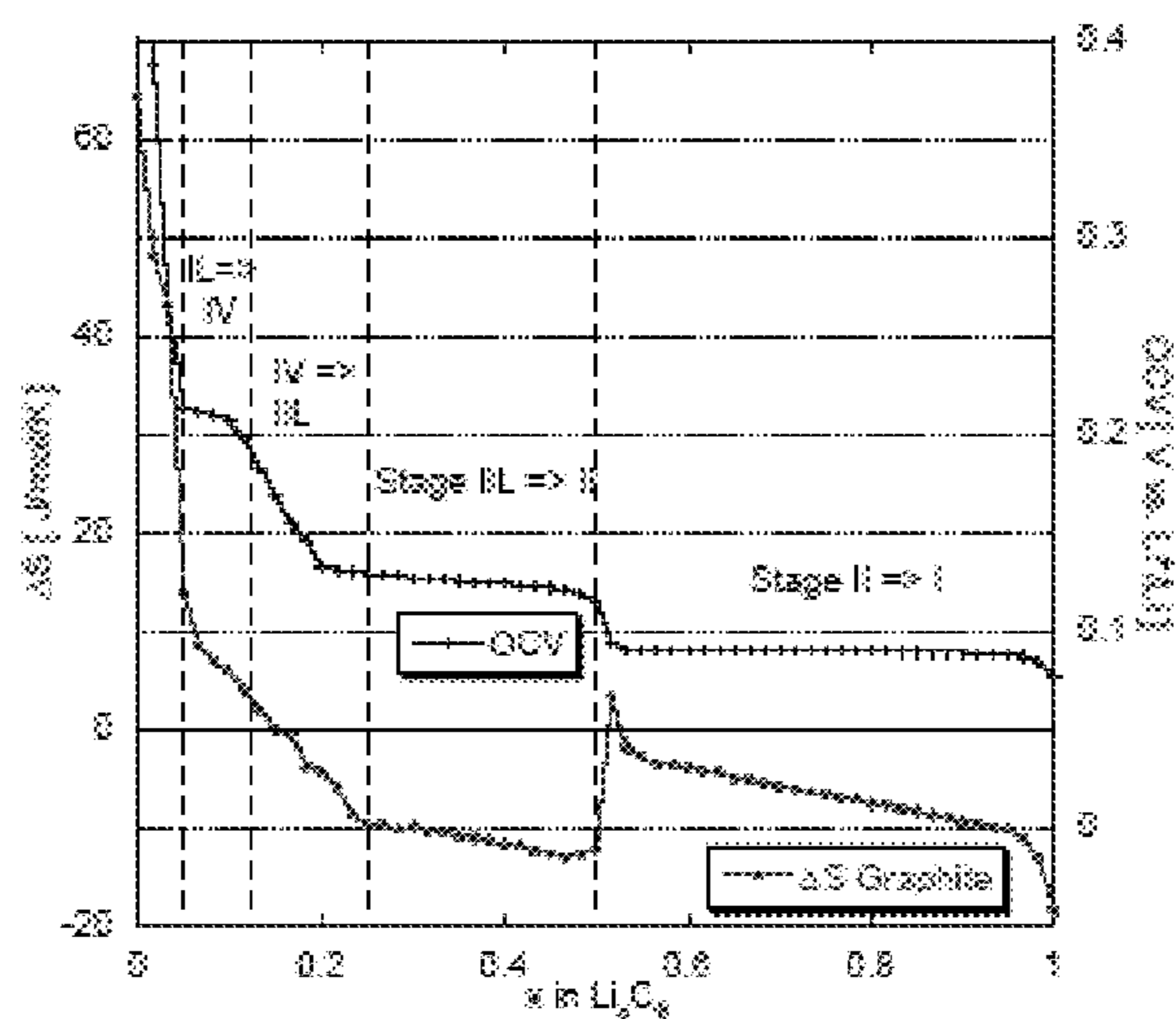
Entropy of intercalation and OCV during insertion
