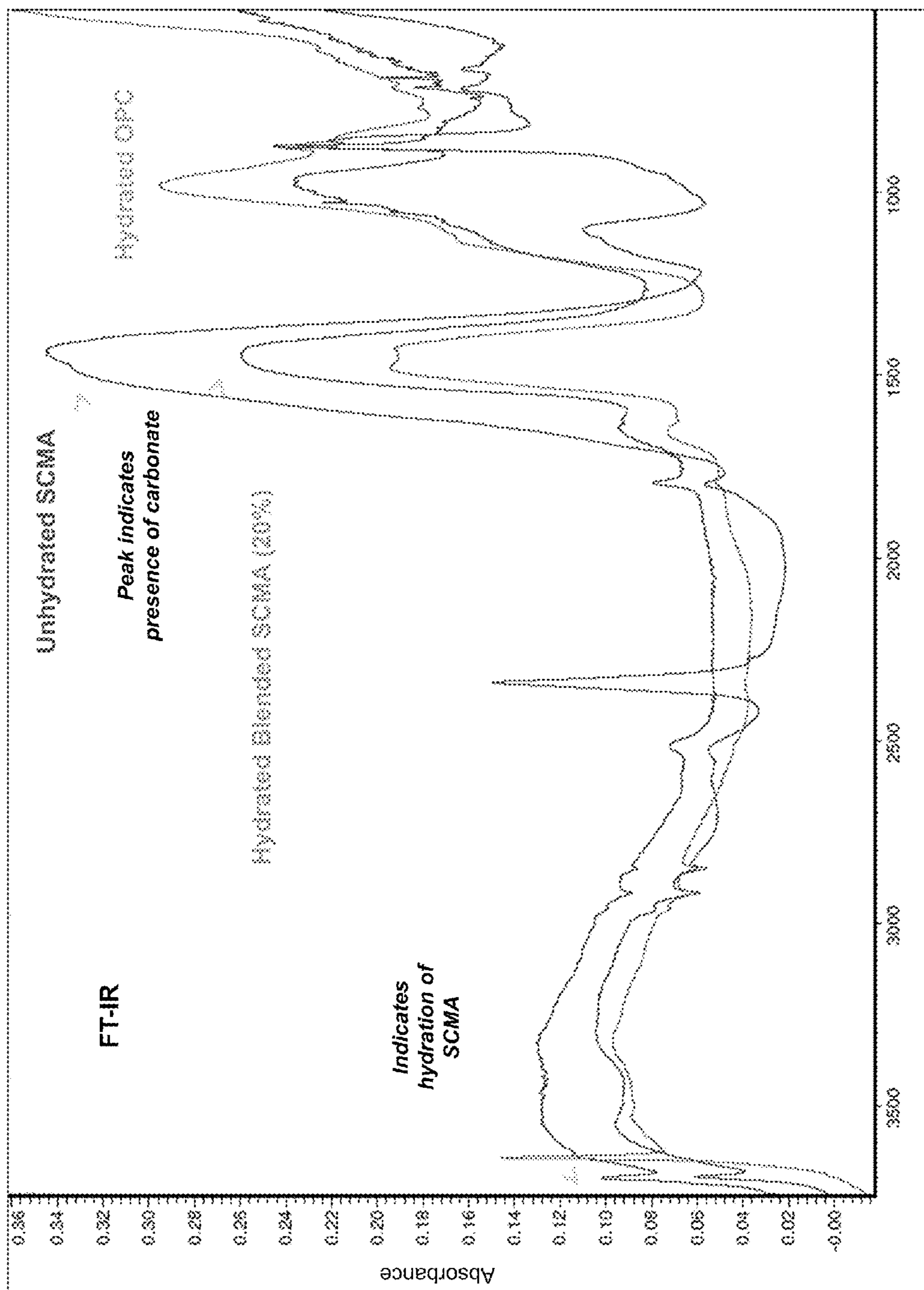
Wavenumbers (cm -1 )
