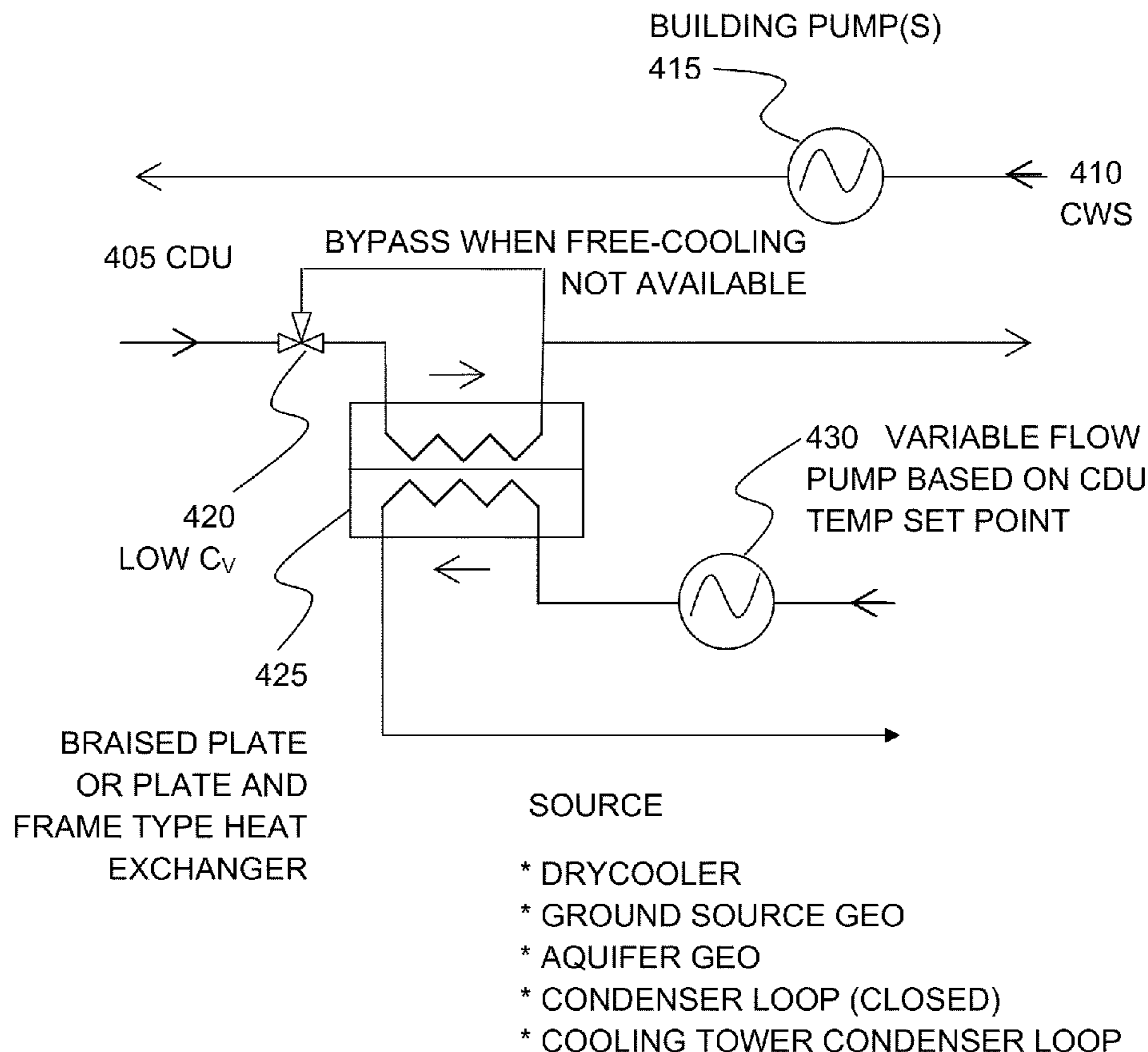
Indirect Flow Embodiment
