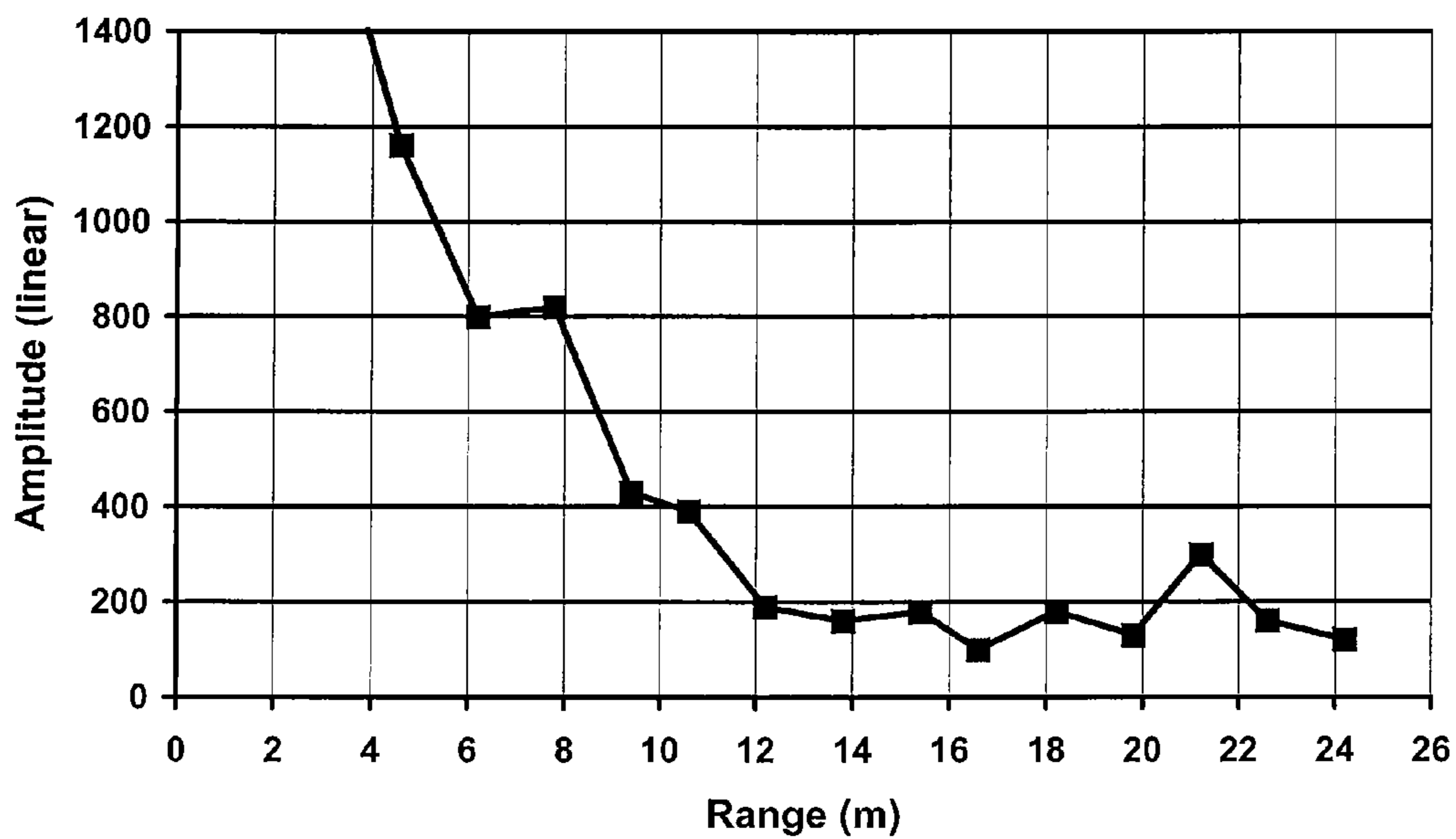
Well F2 Radar Return
