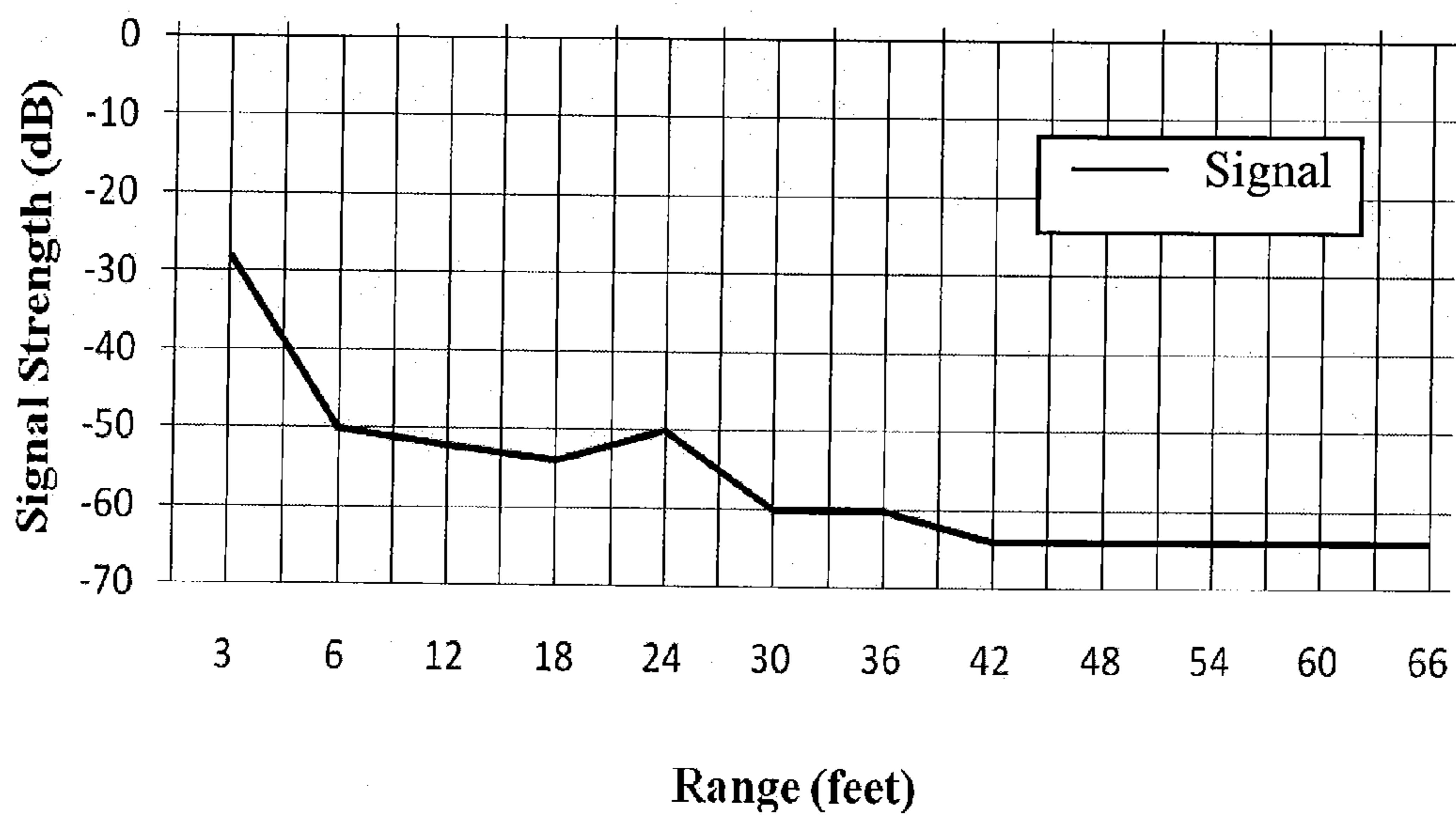
Signal Strength vs Range at 1.01 GHz
