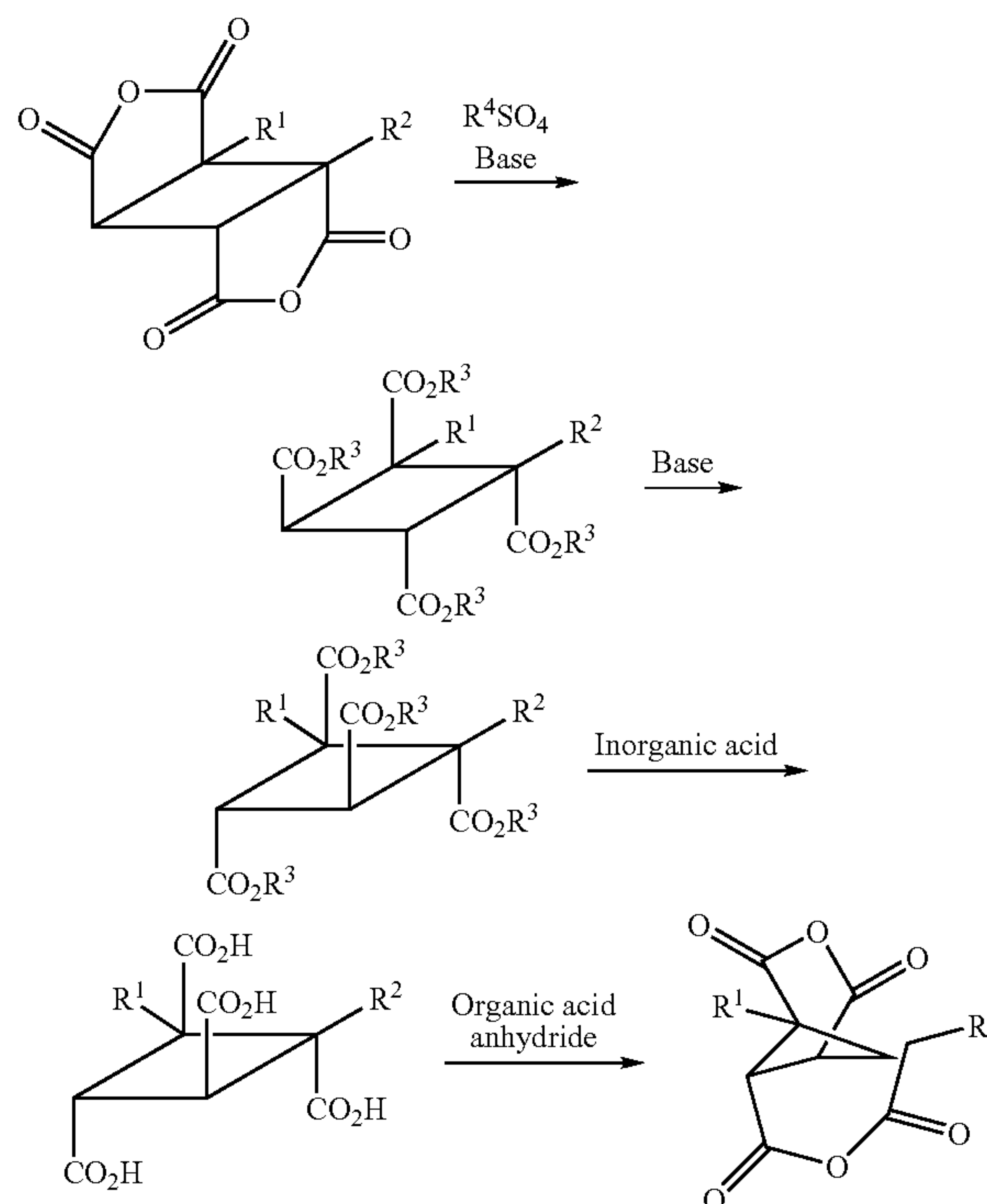
(Scheme 2)
