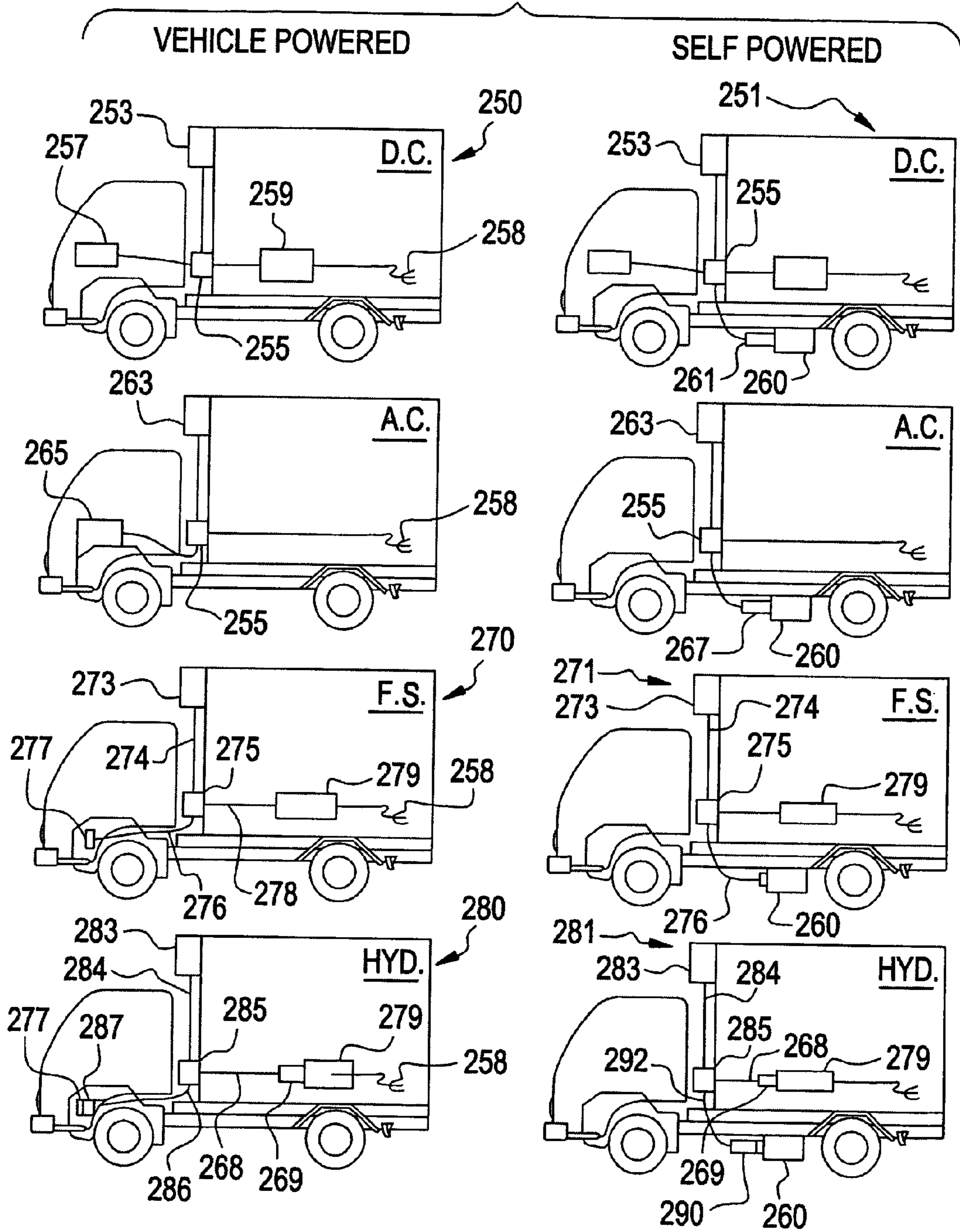
FIG. 48 STAND - BY OPTIONS
