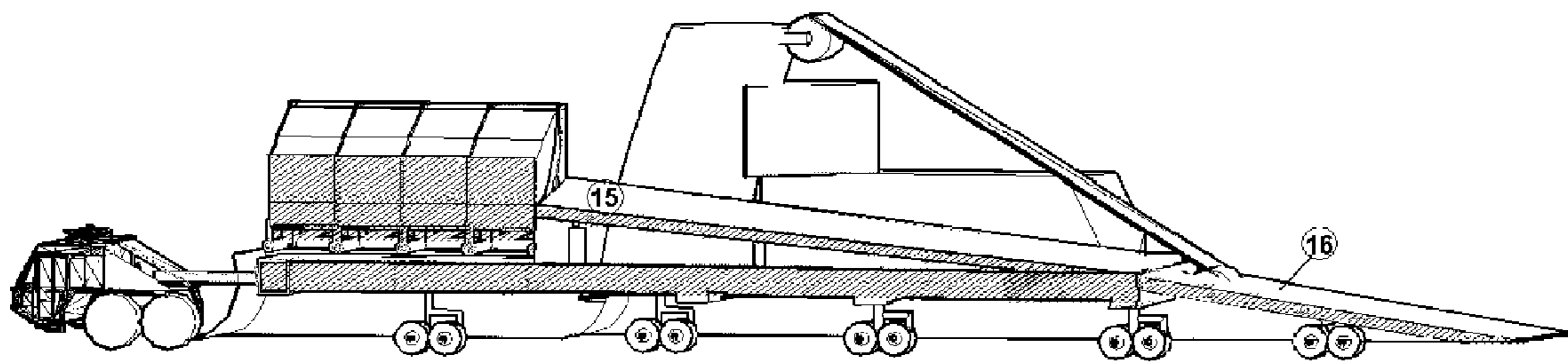
FIG. 9 is a graphical representation of a sectional view comprising ramp 15 and ramp 16.
