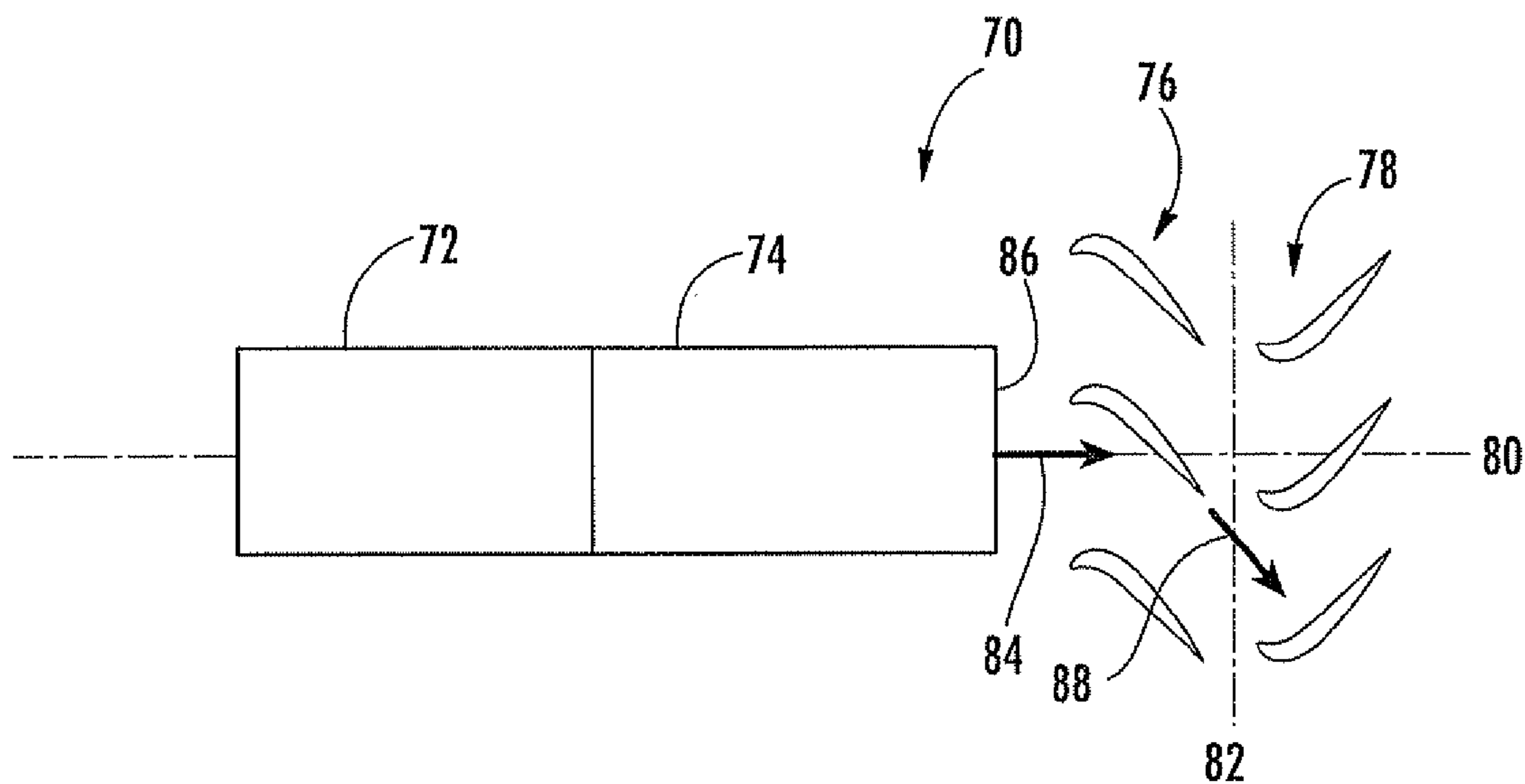
FIG. 3 (PRIOR ART)
